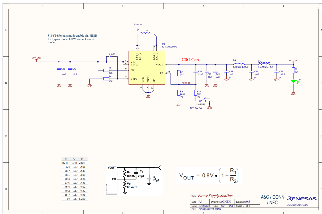
Figure 8. Schematic Sheet 3
