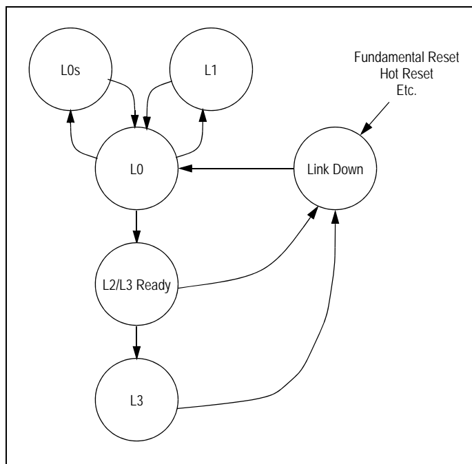
Figure 4.3 PES8T5 ASPM Link State Transitions
