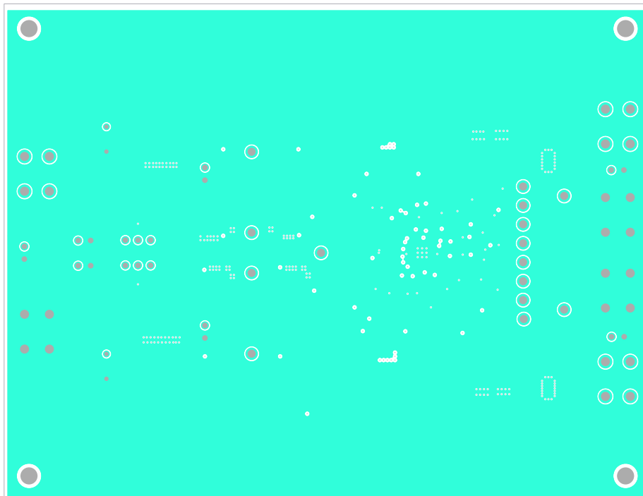
Figure 10. Third Layer
