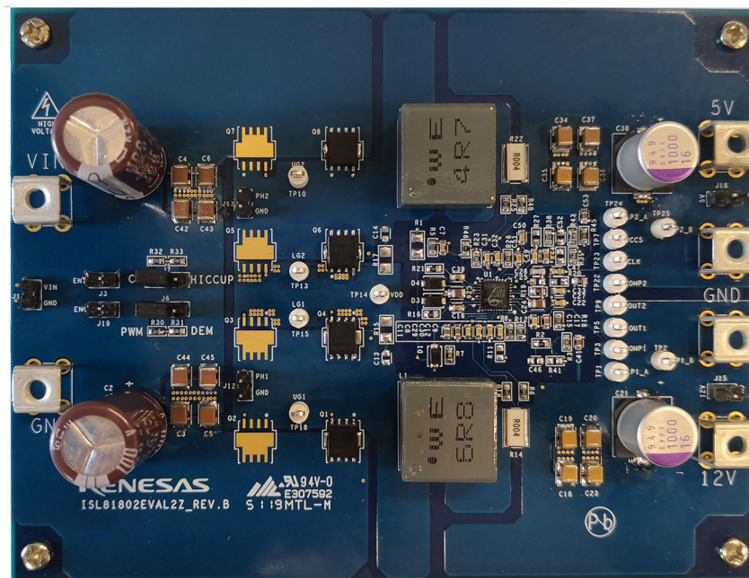
Figure 4. ISL81802EVAL2Z Evaluation Board, Top View
