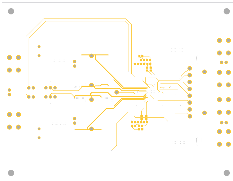
Figure 11. Bottom Layer
