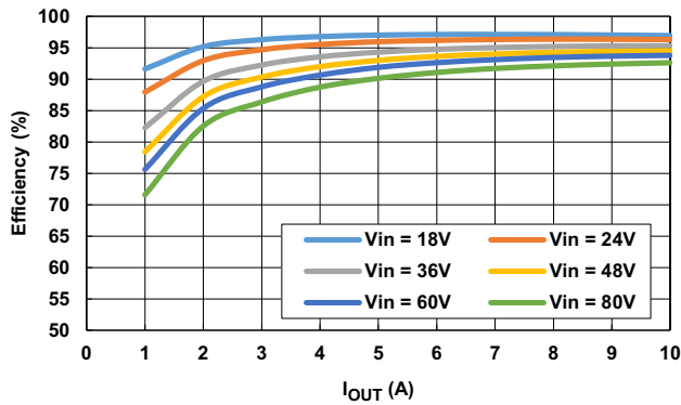
Figure 15. 12V Output Efficiency, CCM
