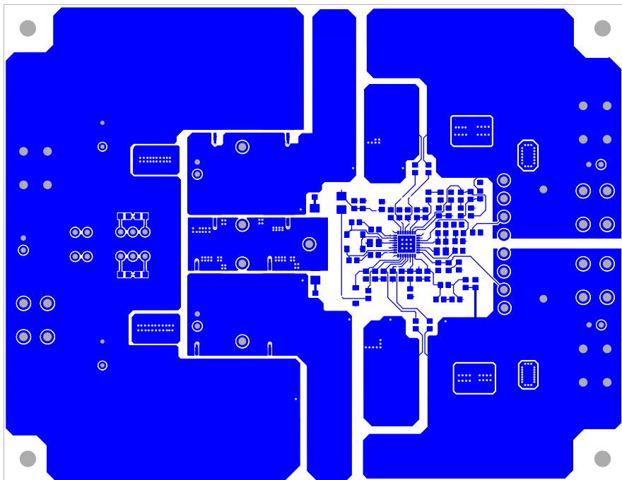
Figure 8. Top Layer
