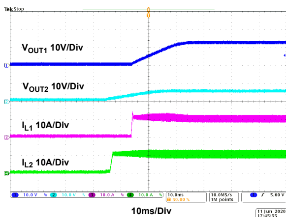
Figure 25. Start-Up Waveform, V_{IN} = 18V , V_{OUT1} = 12V , V_{OUT2} = 5V , I_{OUT1} = 10A , I_{OUT2} = 10A , CCM
