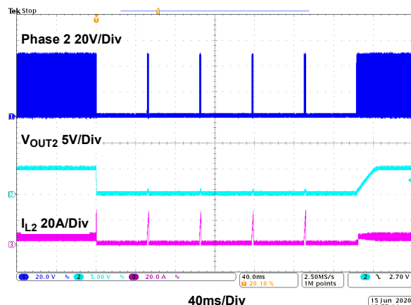
Figure 30. 5V Output Short-Circuit Waveform
