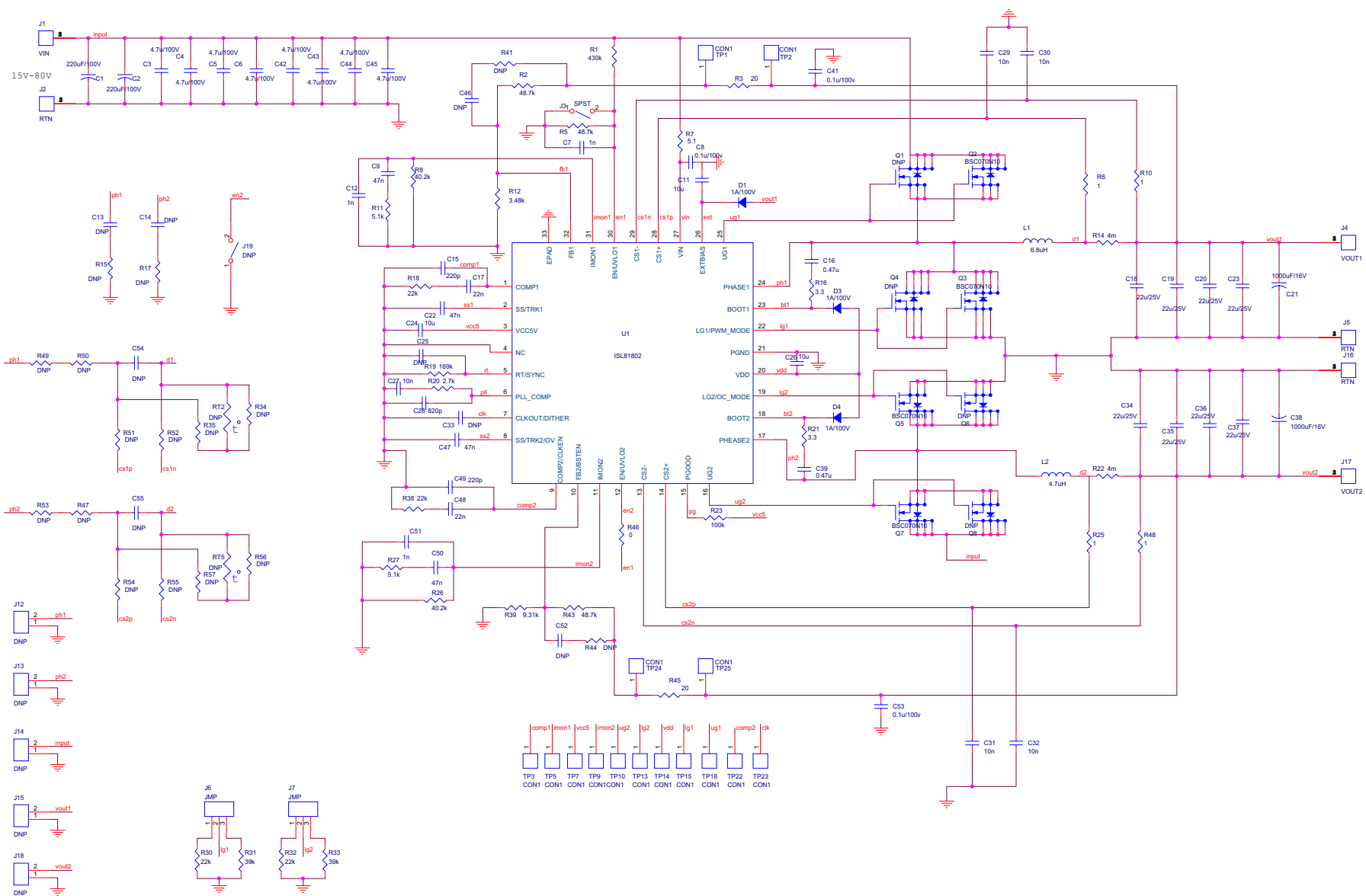
Figure 6. Schematic
