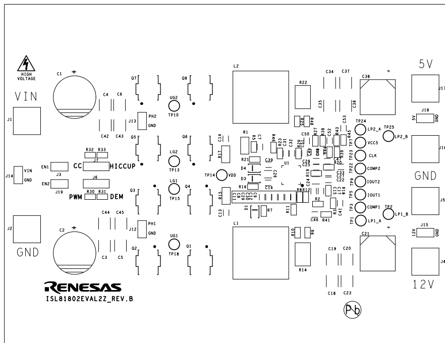
Figure 7. Silkscreen Top
