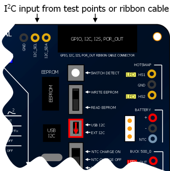
Figure 20. External I 2 C Input Switch
