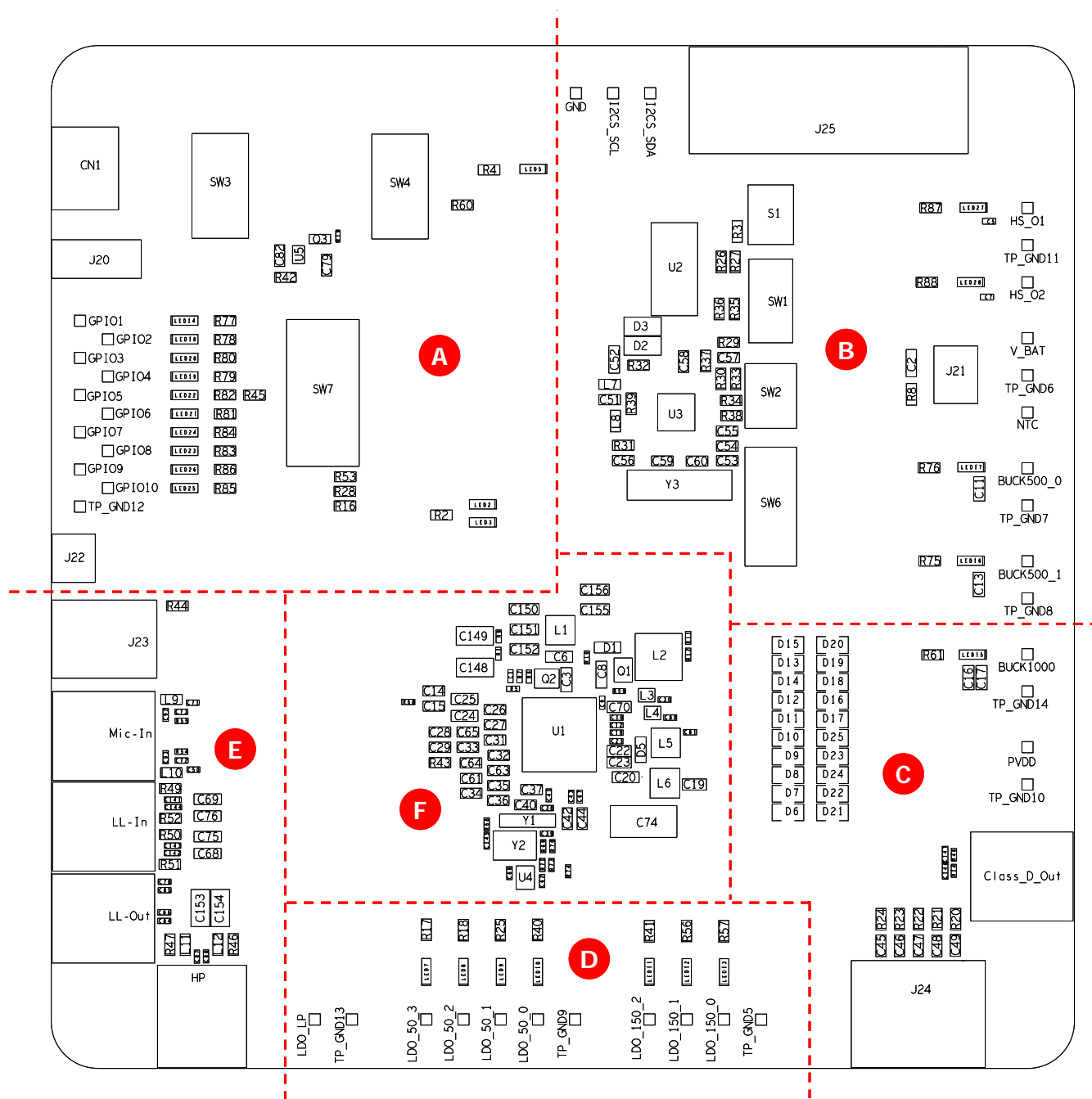
Figure 28. Component Map
