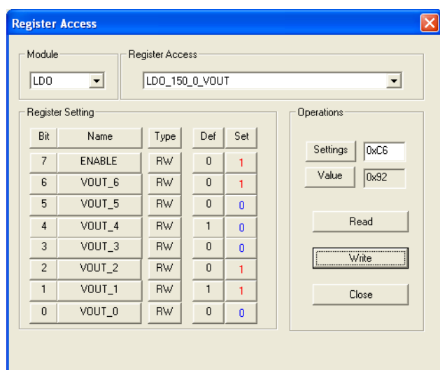
Figure 19. LDO_150_0 2.5V Output Voltage Setting
