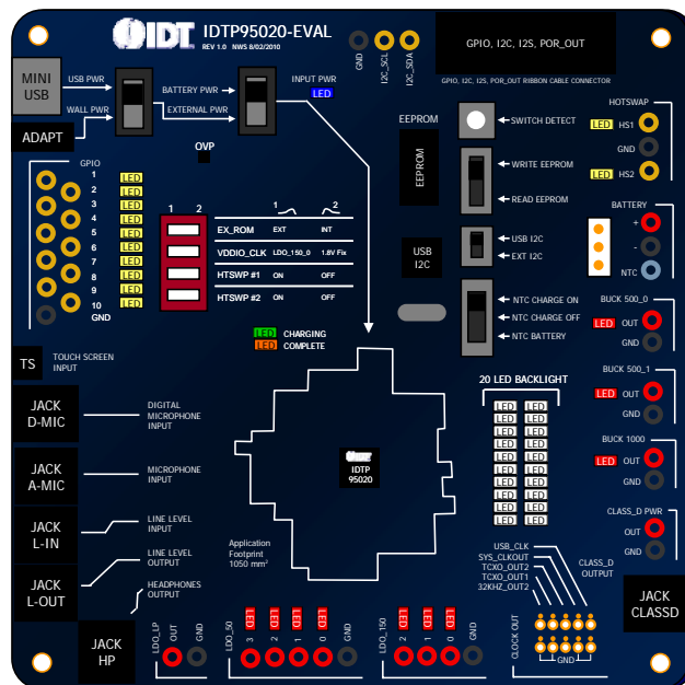
Figure 1. Evaluation Board Illustration Top Layer
