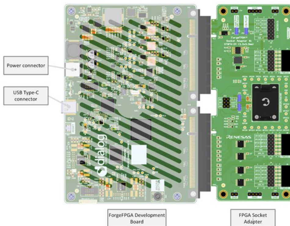
Figure 10: Development Kit
