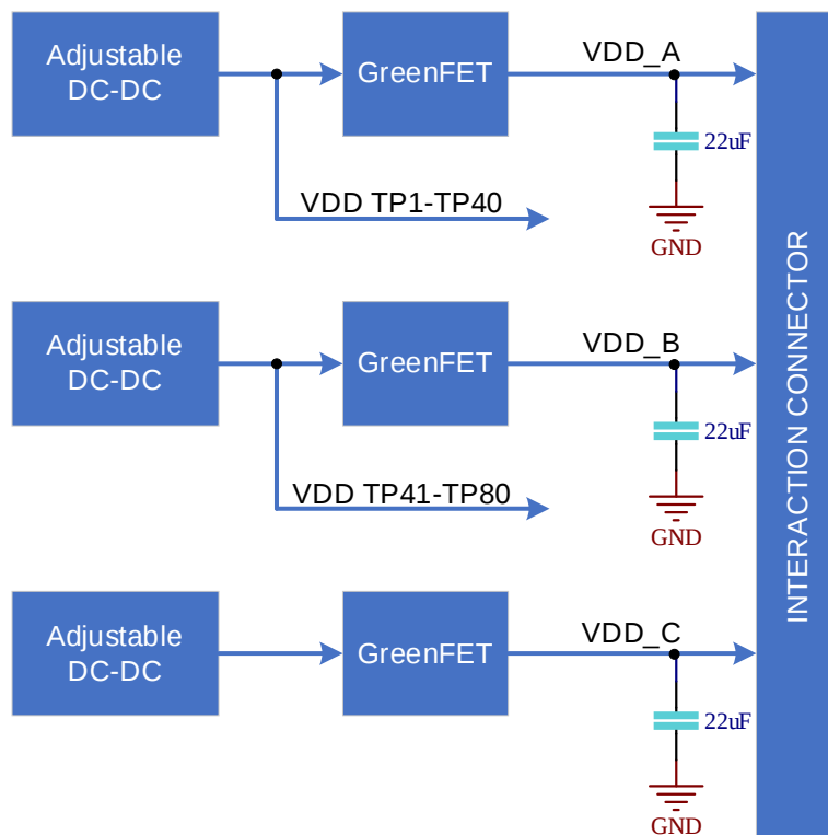
Figure 7: Power Structure
