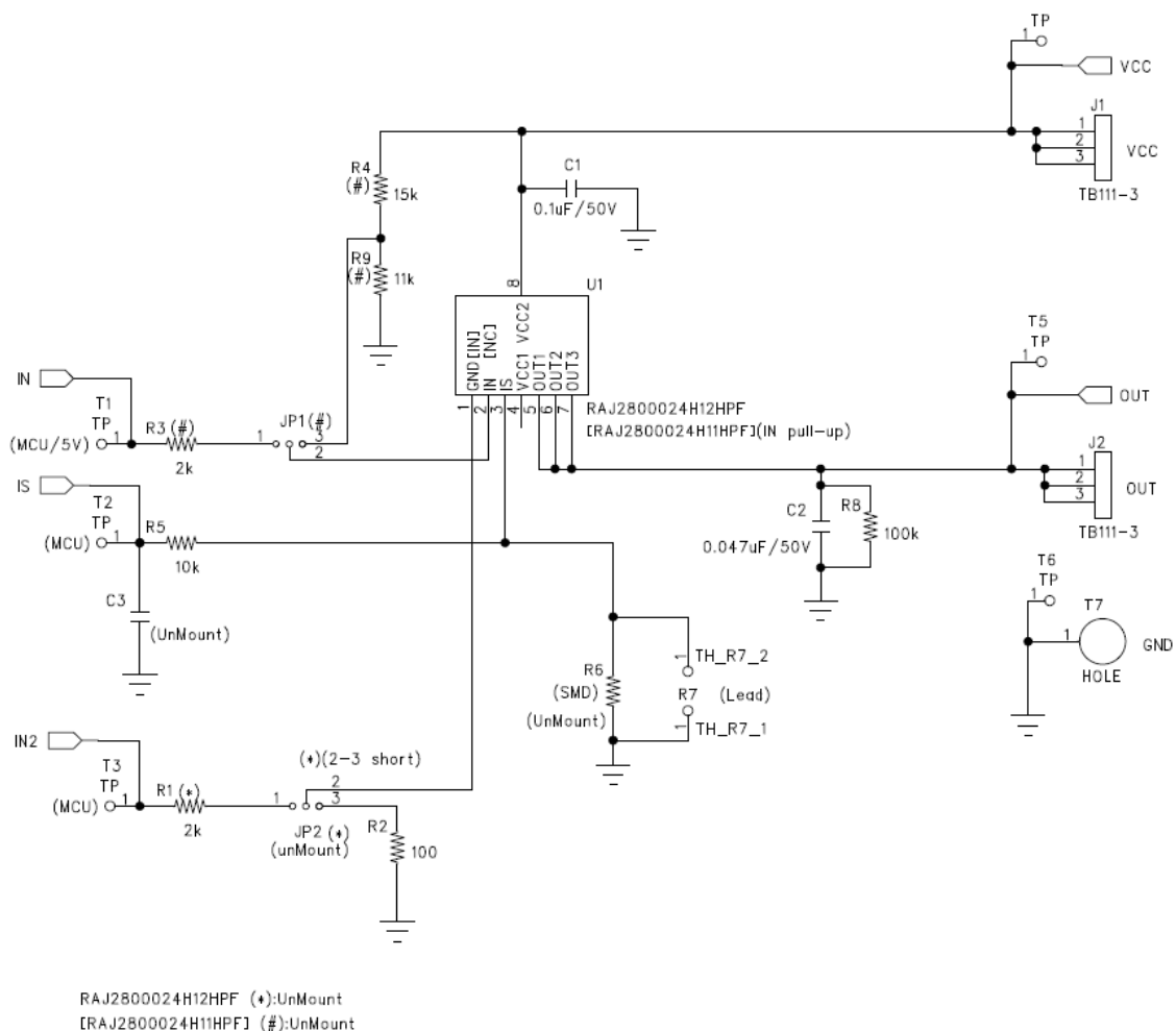
Figure 2. EV-IPD263 schematics
