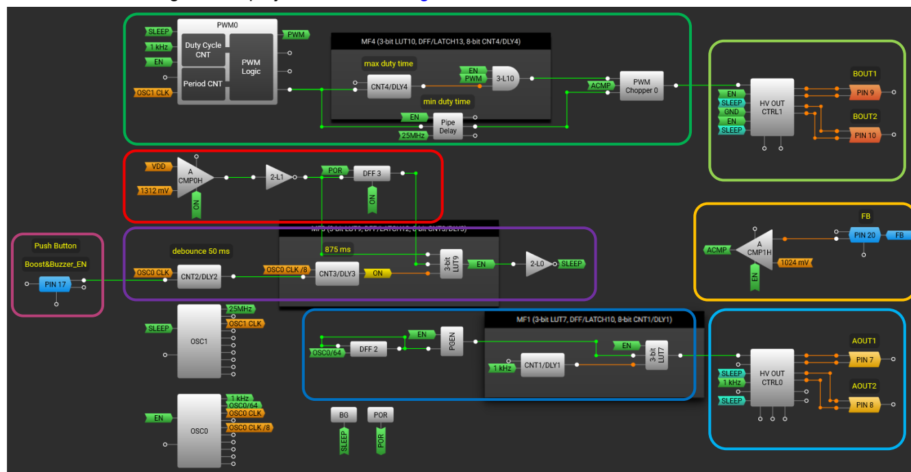
Figure 6. SLG47105V DC/DC Boost & Buzzer Driver Demo Board GreenPAK Design
