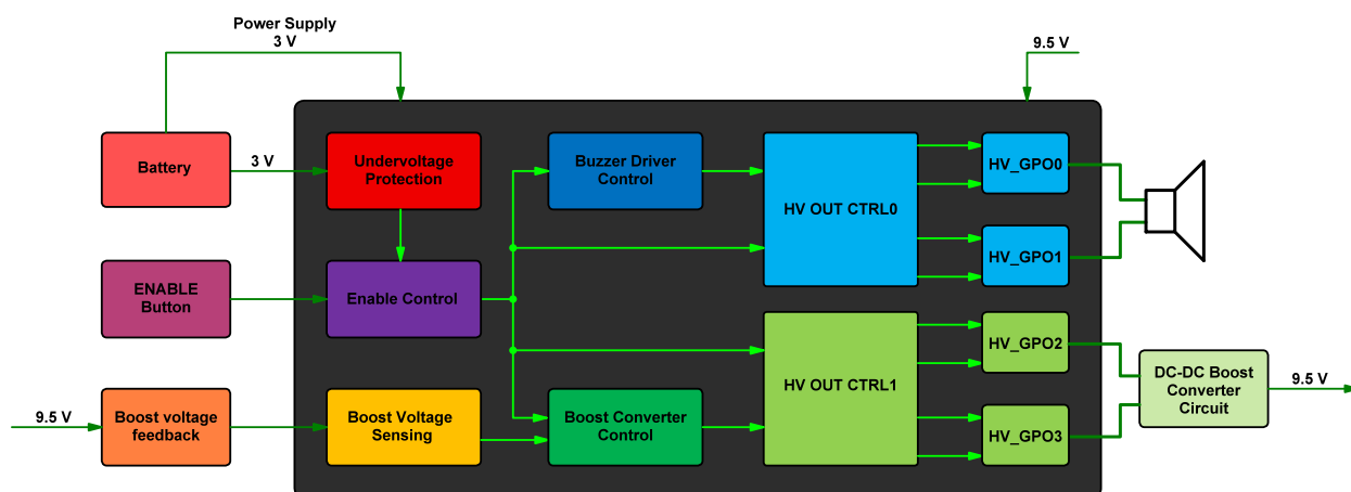
Figure 5. SLG47105V DC/DC Boost & Buzzer Driver Demo Board Block Diagram
