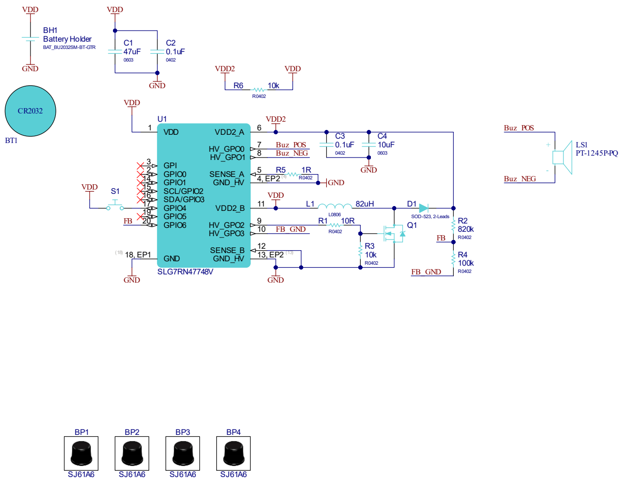
Figure 9. Board Schematic
