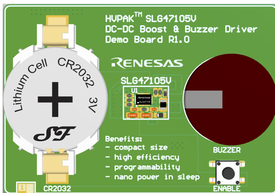
Figure 1. SLG47105V DC/DC Boost & Buzzer Driver Demo Board General View
