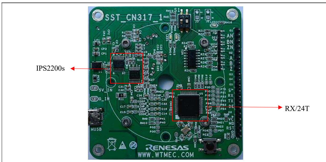
Figure 7-1: Top of Main Board
