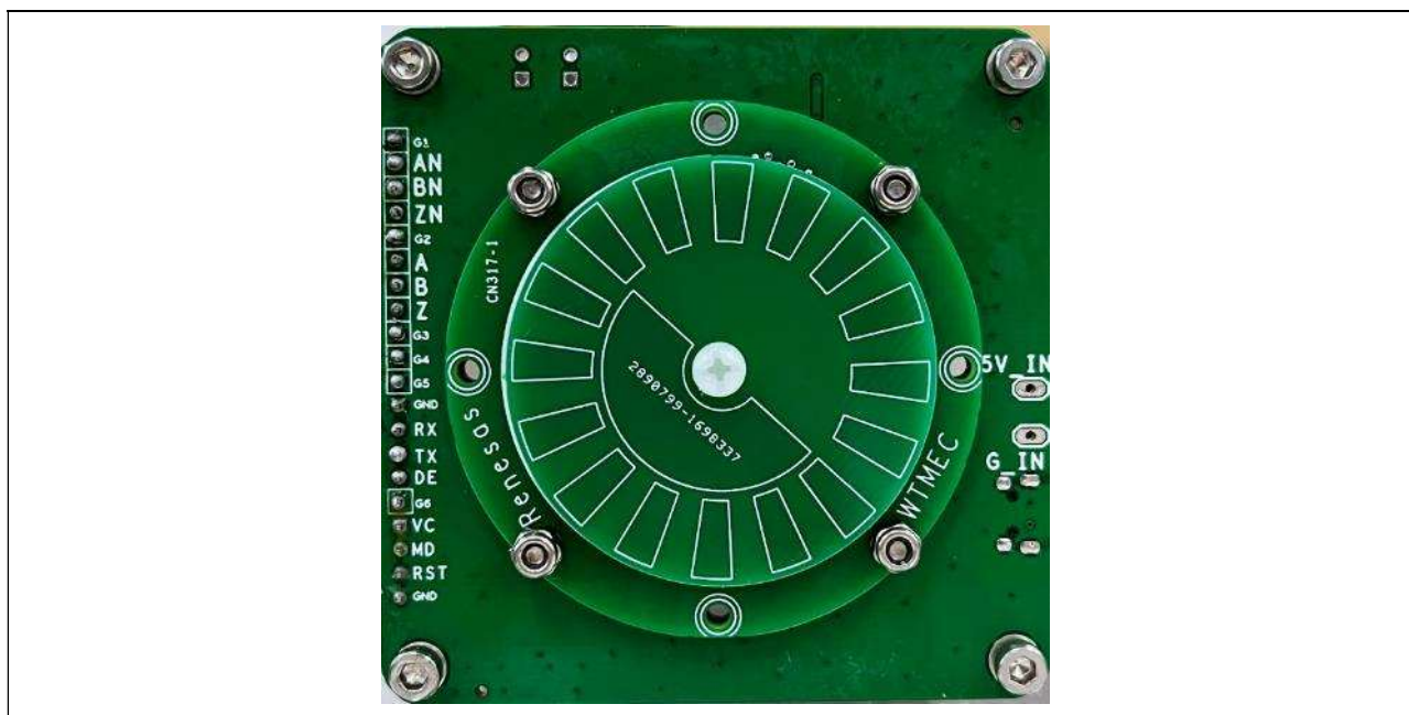
Figure 7-2: Bottom of Main Board
