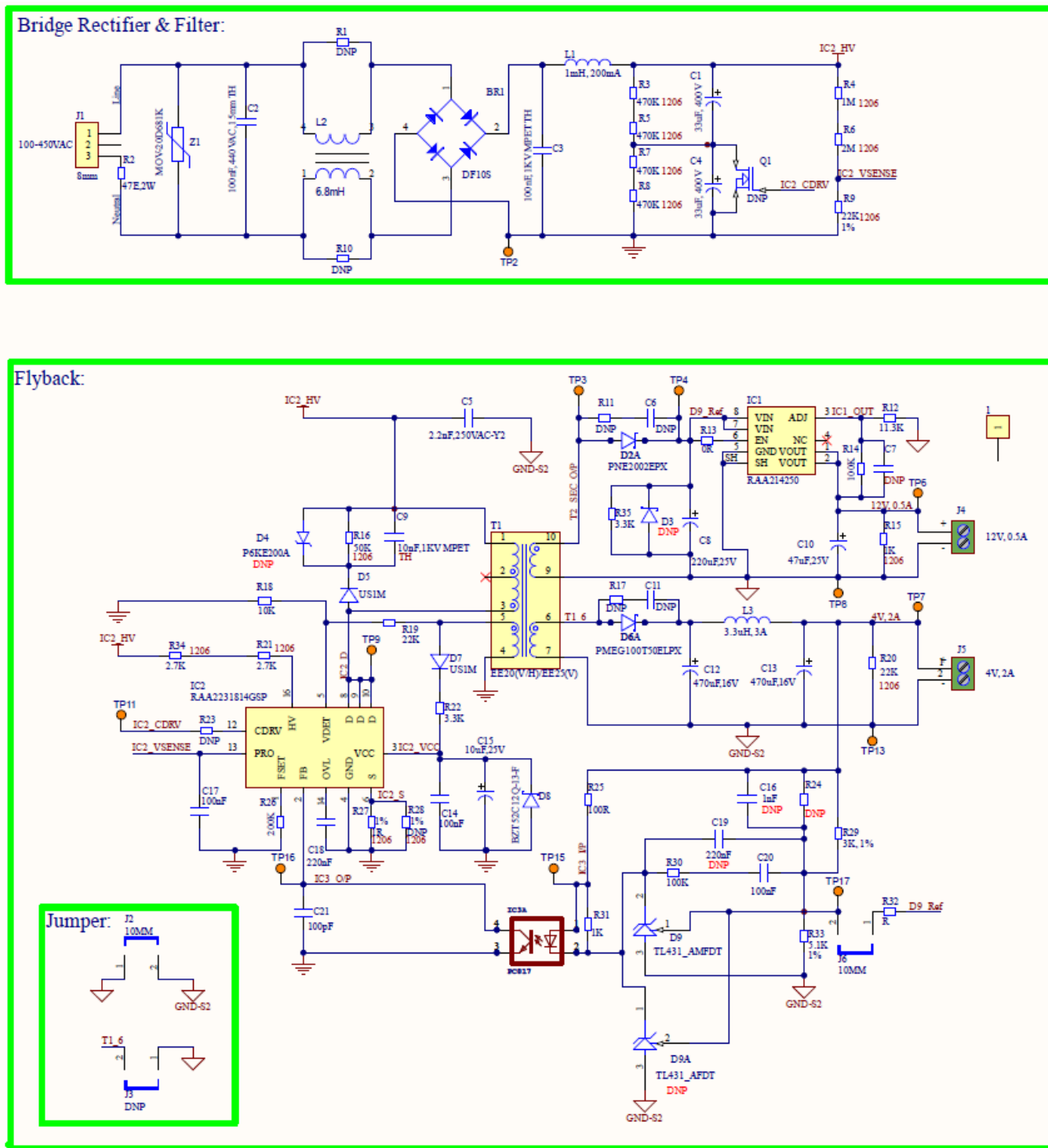
Figure 14. Schematic
