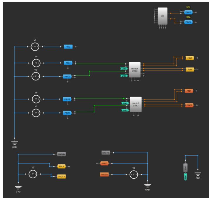
Fig. 4-16 Stepping motor driver device (U2) internal circuit
