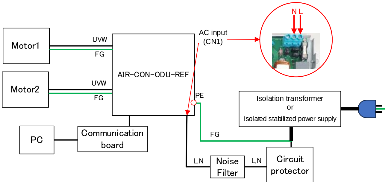
Fig. 3-7 Connection of AC power supply
