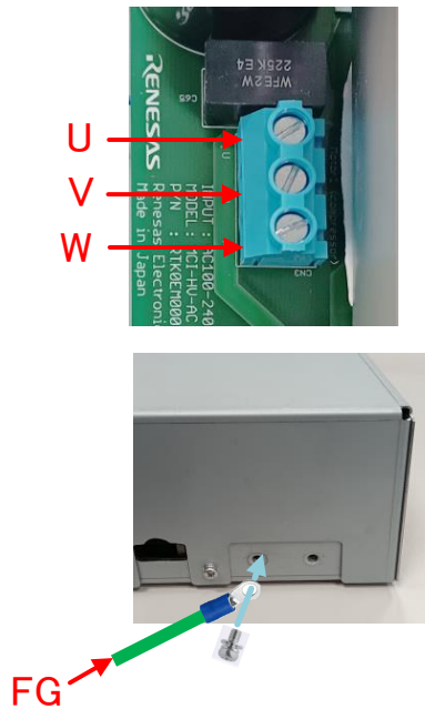
Fig. 3-3 Motor1 Connection
