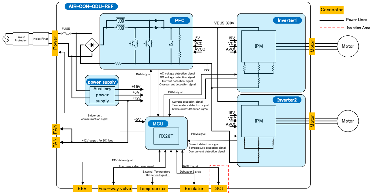
Fig. 2-1 AIR-CON-ODU-REF function block diagram
