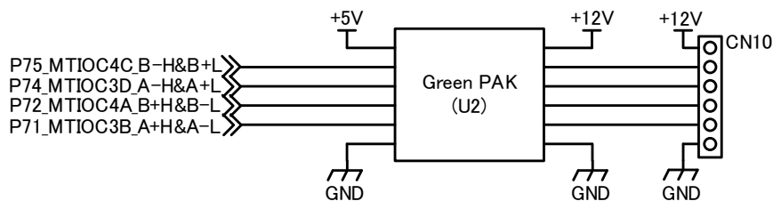
Fig. 4-12 EEV drive circuit
