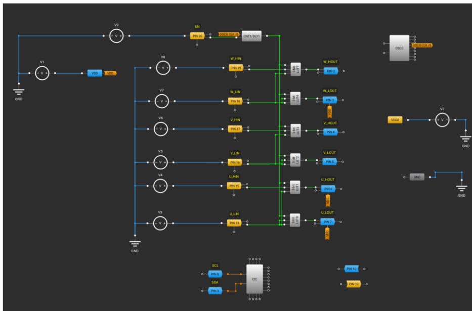
Fig. 4-15 PWM signal overlap protection device (U7) internal circuit
