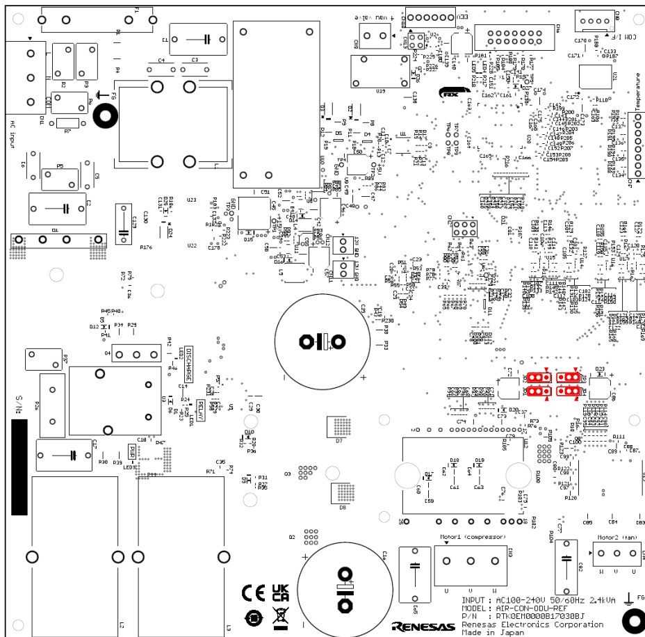
Fig. 2-3 Default jumper pin setting of inverter board
