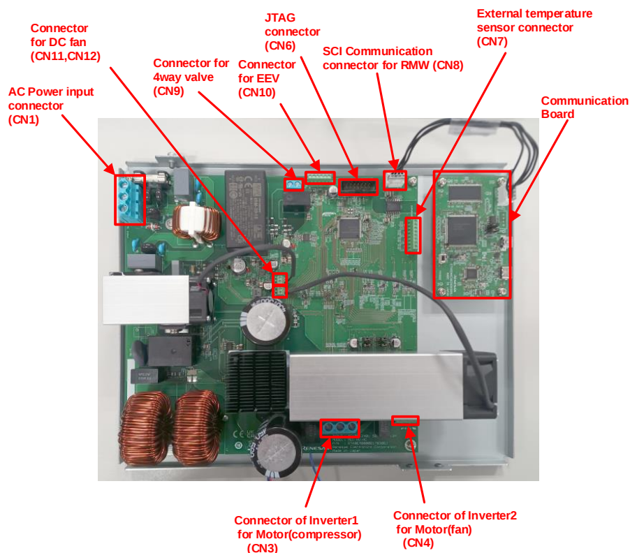
Fig. 2-2 Board layout
