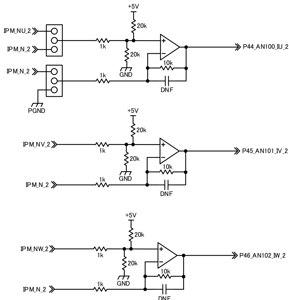
Fig. 4-6 Inverter 2, current detection circuit
