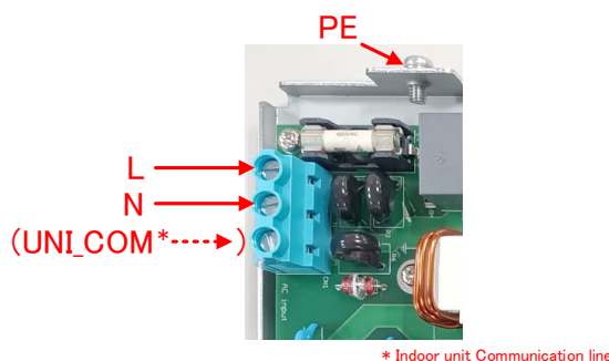
Fig. 3-6 AC power supply connector
