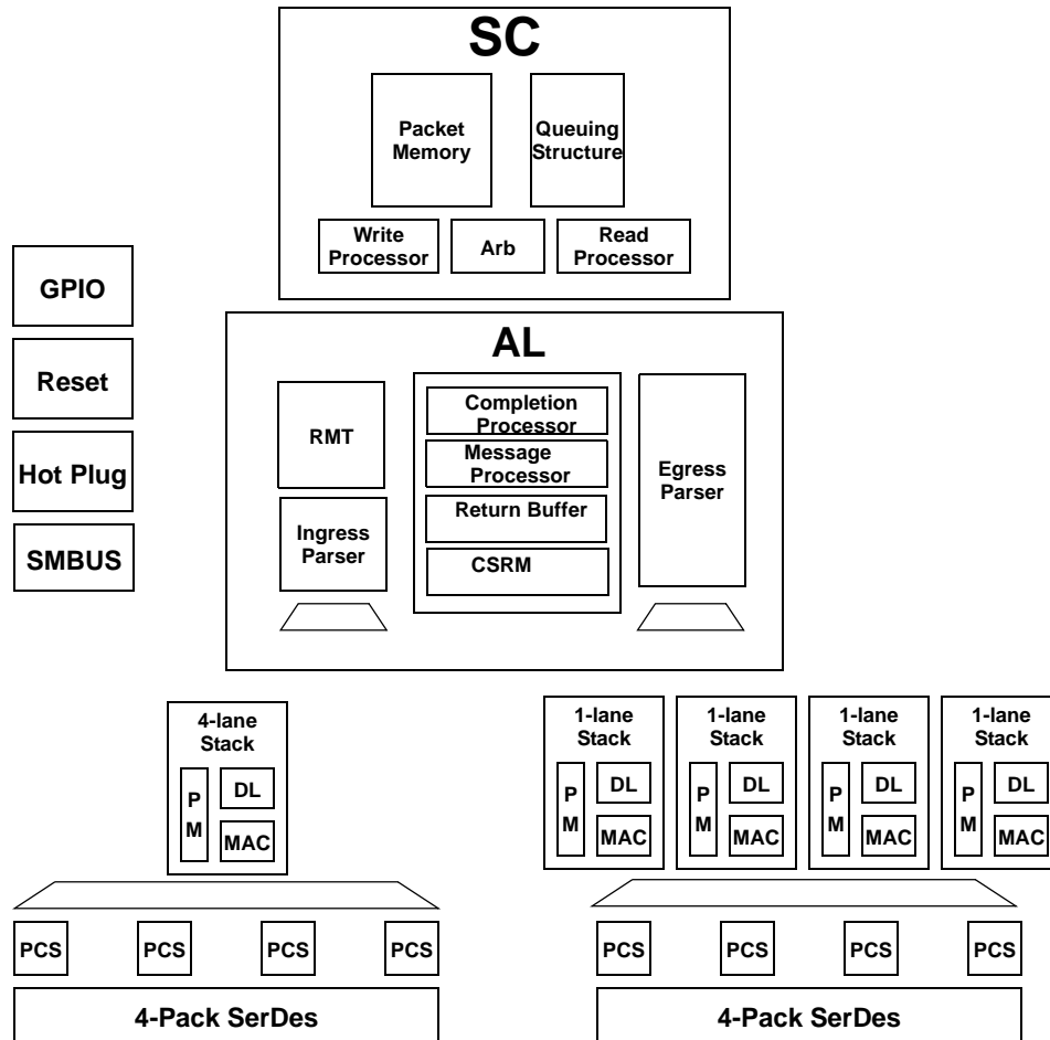
Figure 1.1 PES6T5 Architectural Block Diagram
