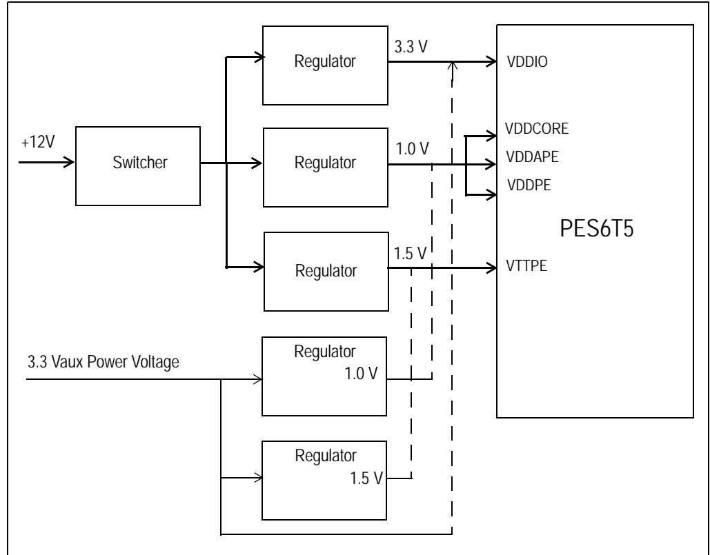
Figure 7.5 Conceptual Diagram of the PES6T5 Auxiliary Power Connection
