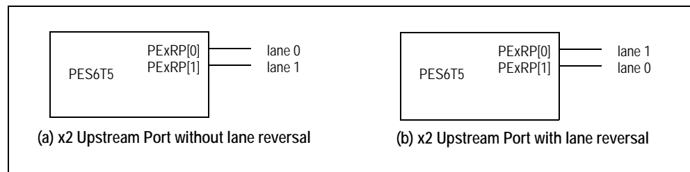
Figure 4.1 Upstream Port (x2 Lane Width) Lane Reversal
