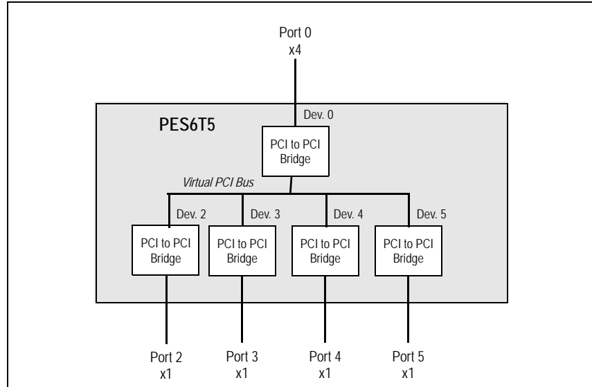
Figure 1.3 PES6T5 Port Configuration
