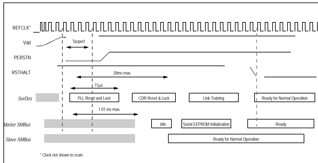
Figure 2.5 Fundamental Reset with Serial EEPROM initialization
