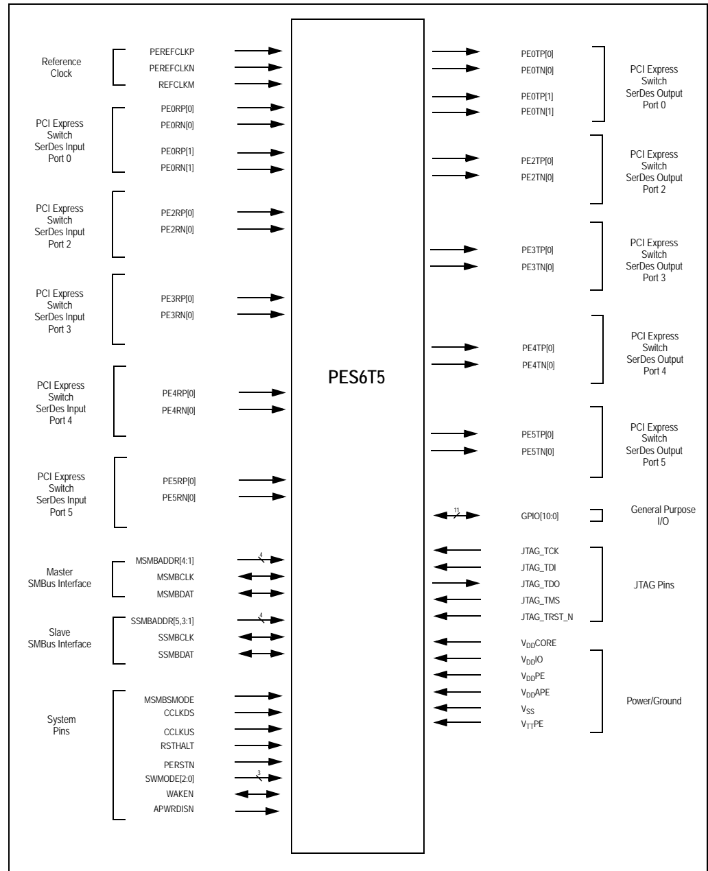
Figure 1.2 PES6T5 Logic Diagram
