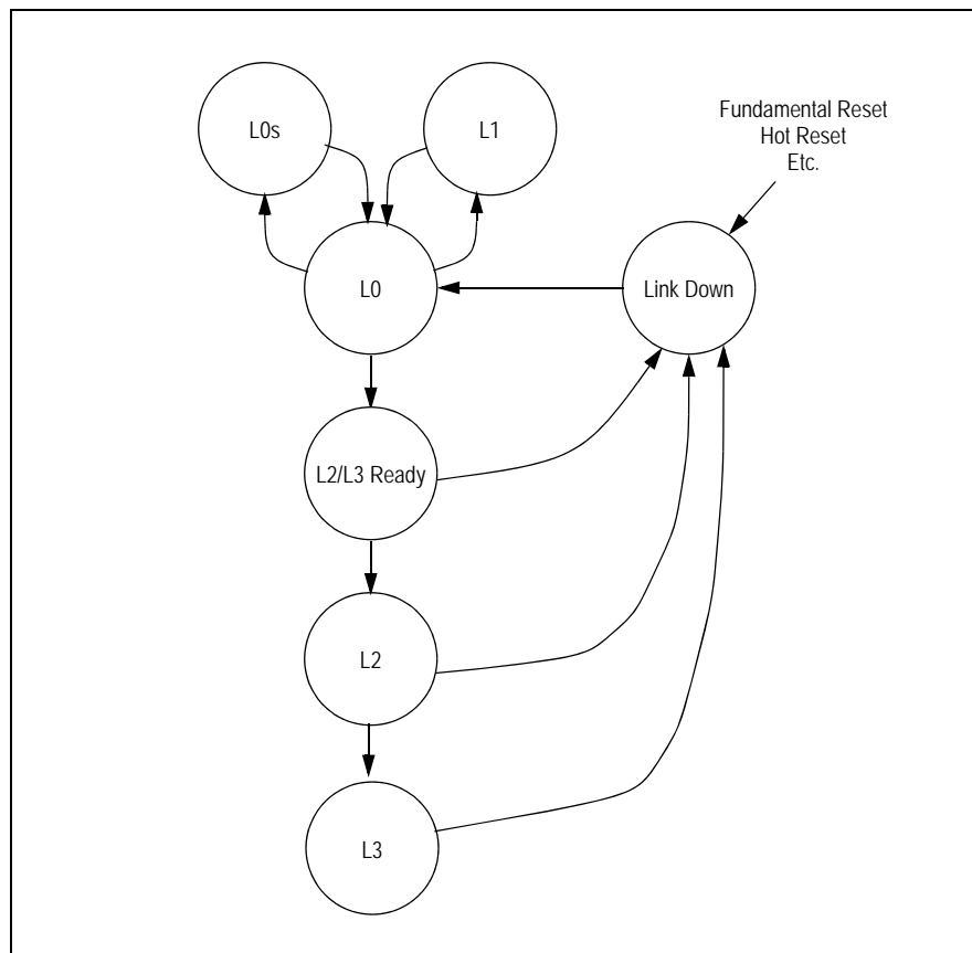
Figure 4.2 PES6T5 ASPM Link State Transitions
