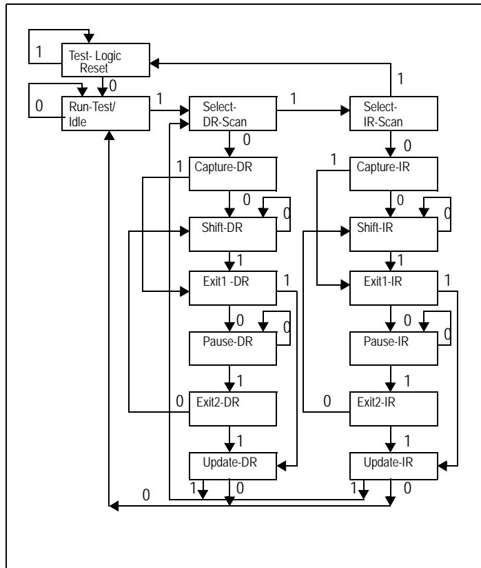
Figure 10.2 State Diagram of PES6T5's TAP Controller
