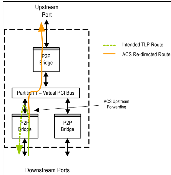
Figure 8.3 ACS Upstream Forwarding Example
