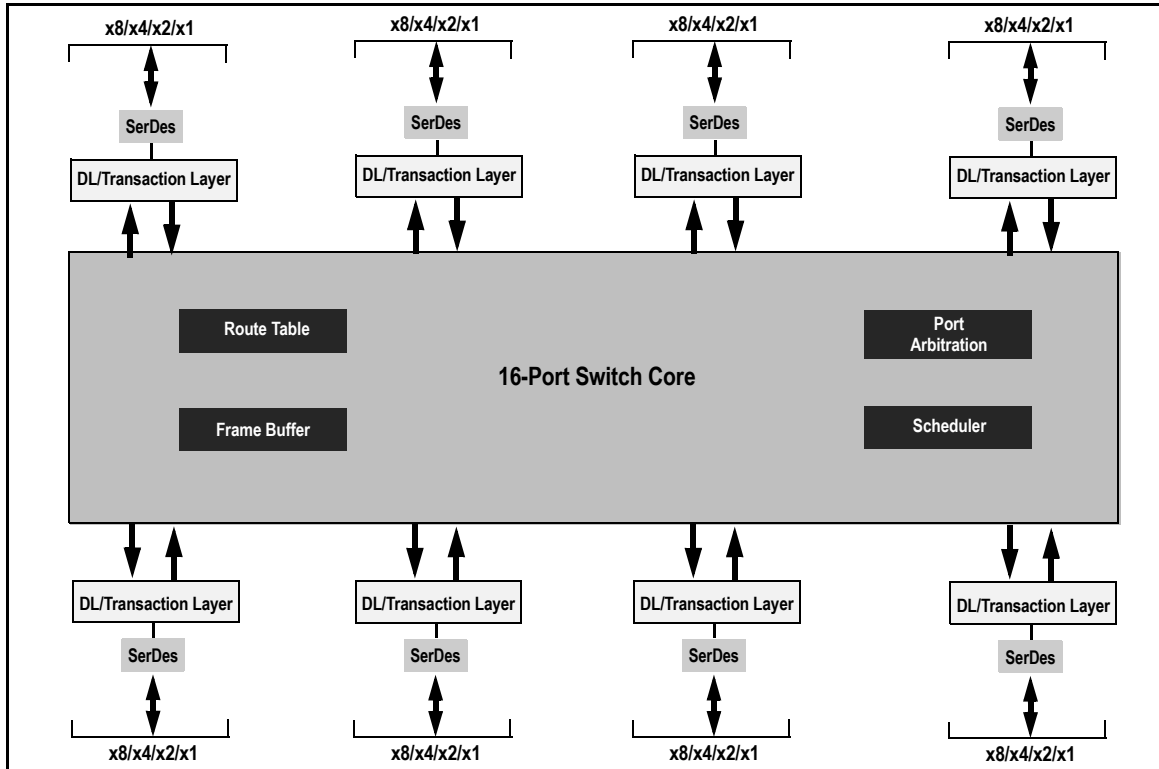
64 PCI Express Lanes Up to 8 x8 ports or 16 x4 Ports Figure 1.1 PES64H16AG2 Block Diagram
