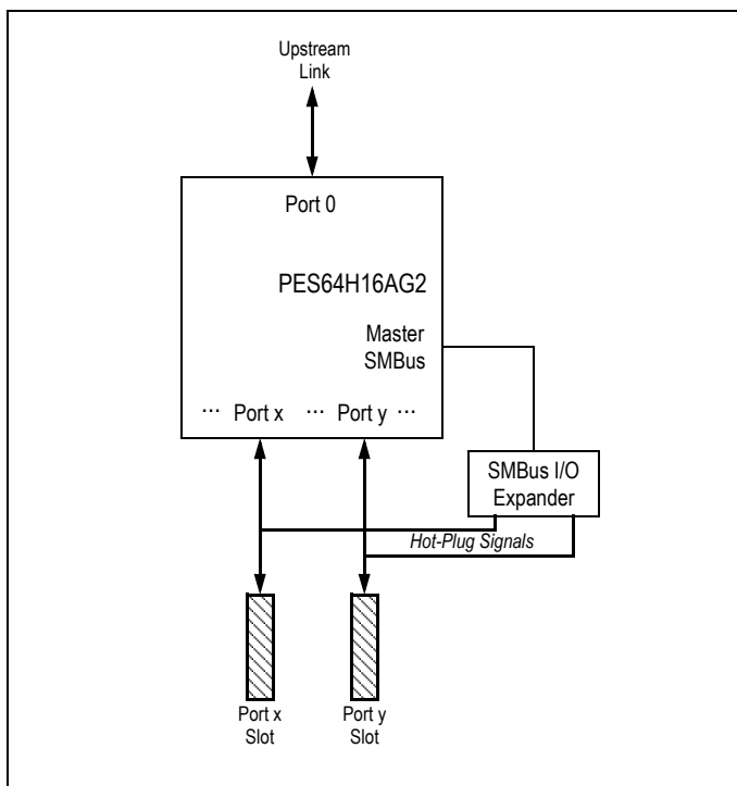
Figure 10.1 Hot-Plug on Switch Downstream Slots Application
