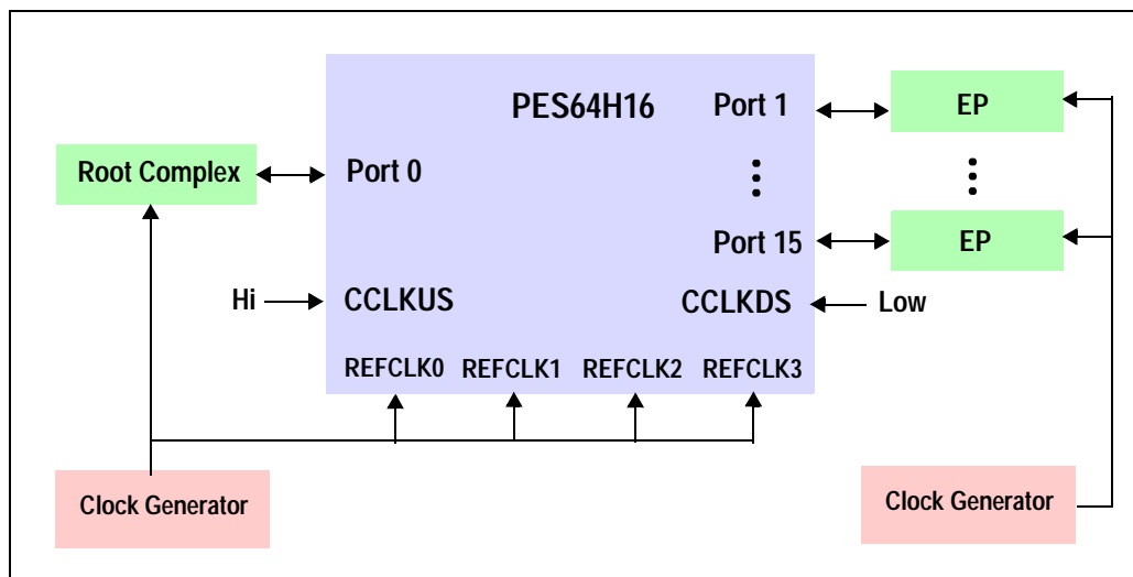
Figure 3.3 Common Clock on Upstream; Non-Common Clock on Downstream (must disable Spread Spectrum Clock)
