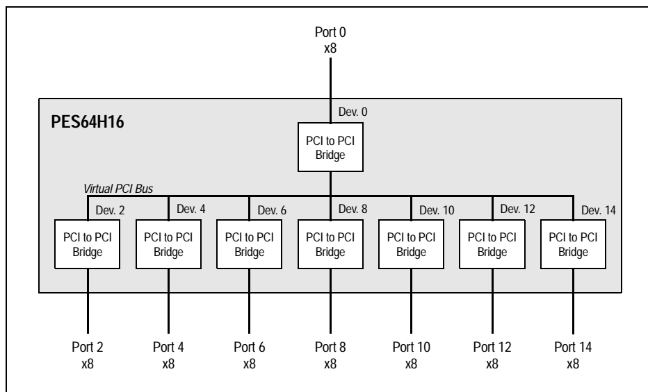
Figure 1.5 All Ports Merged Configuration
