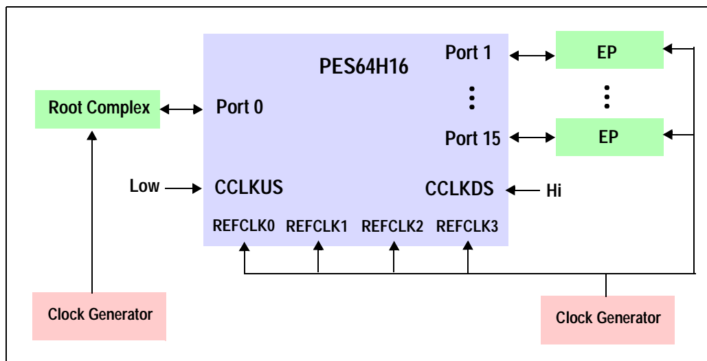
Figure 3.2 Non-Common Clock on Upstream; Common Clock on Downstream (must disable Spread Spectrum Clock)
