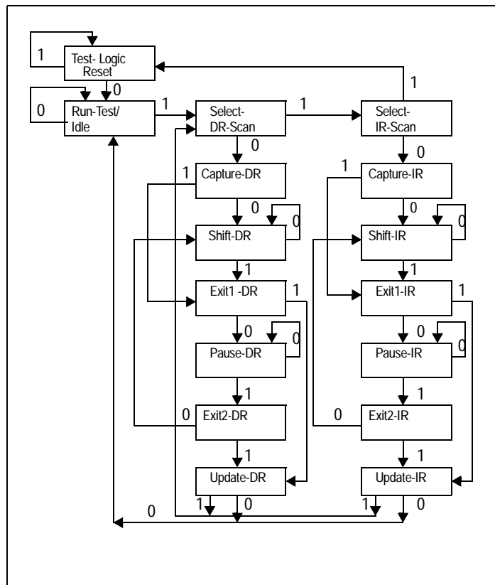
Figure 10.2 State Diagram of PES34H16's TAP Controller
