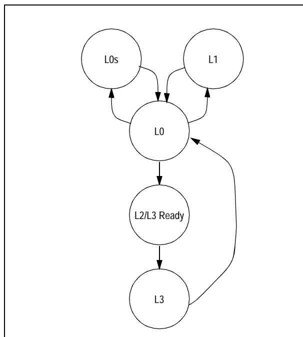
Figure 4.6 PES34H16 ASPM Link State Transitions
