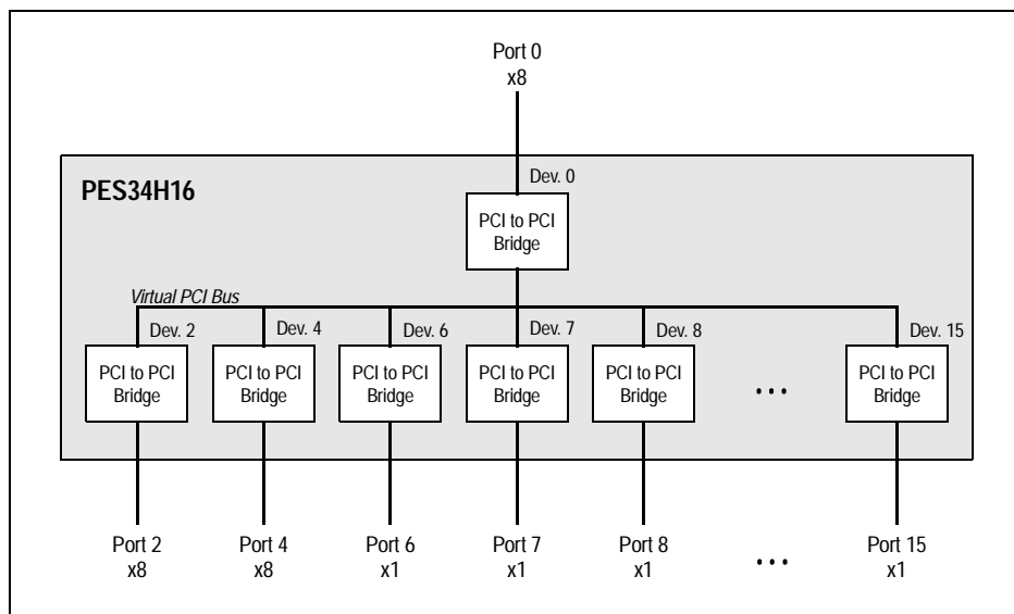
Figure 1.4 Three Ports Merged Configuration
