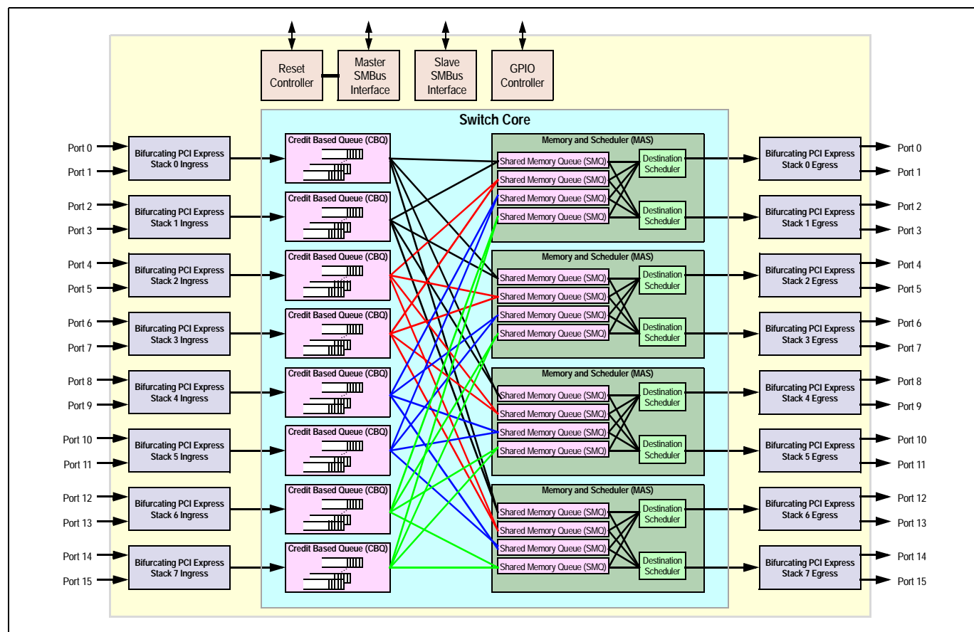
Figure 1.1 PES34H16 Architectural Block Diagram
