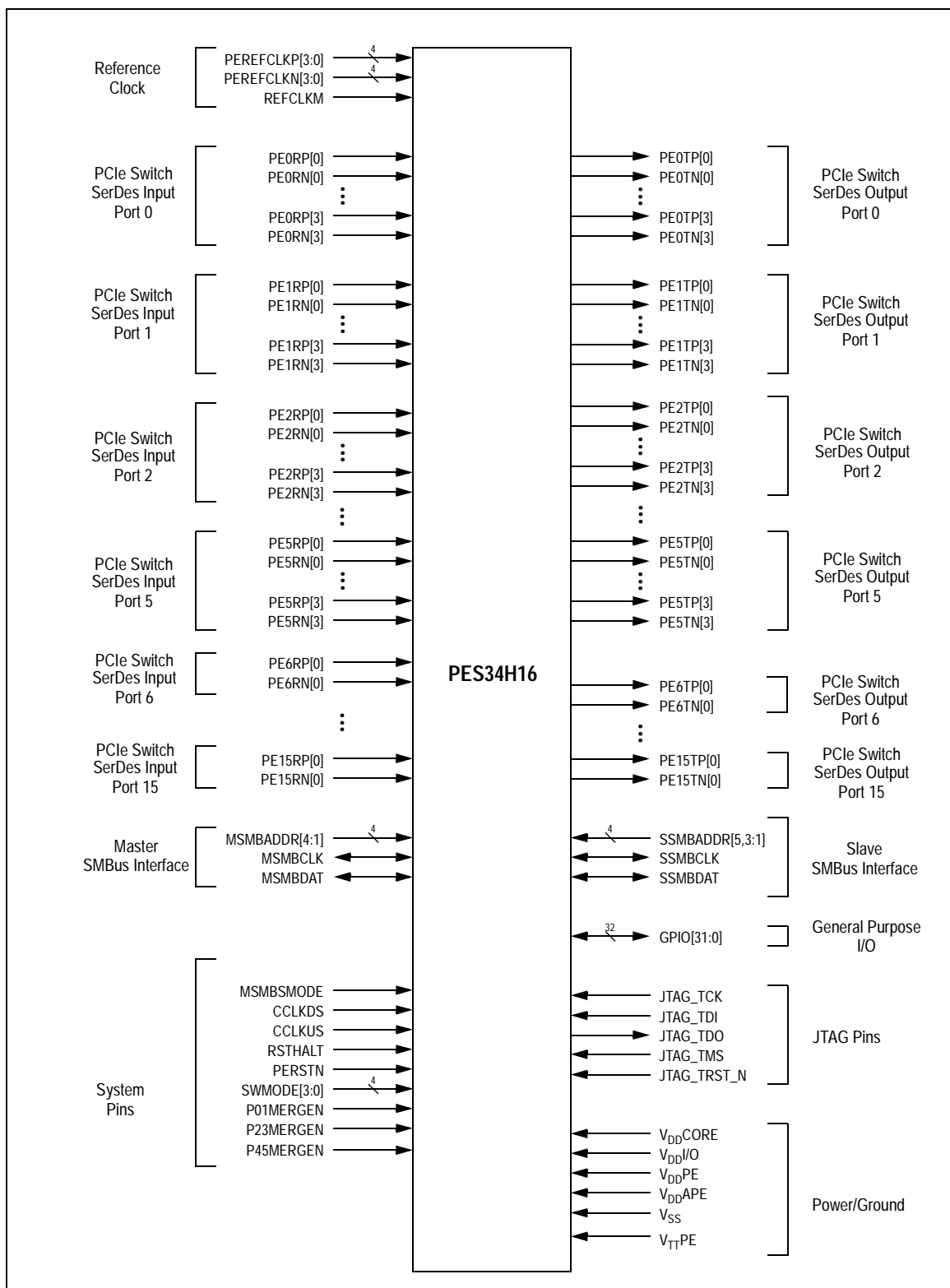
Figure 1.2 PES34H16 Logic Diagram
