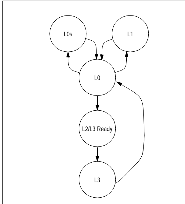
Figure 4.6 PES32H8 ASPM Link State Transitions
