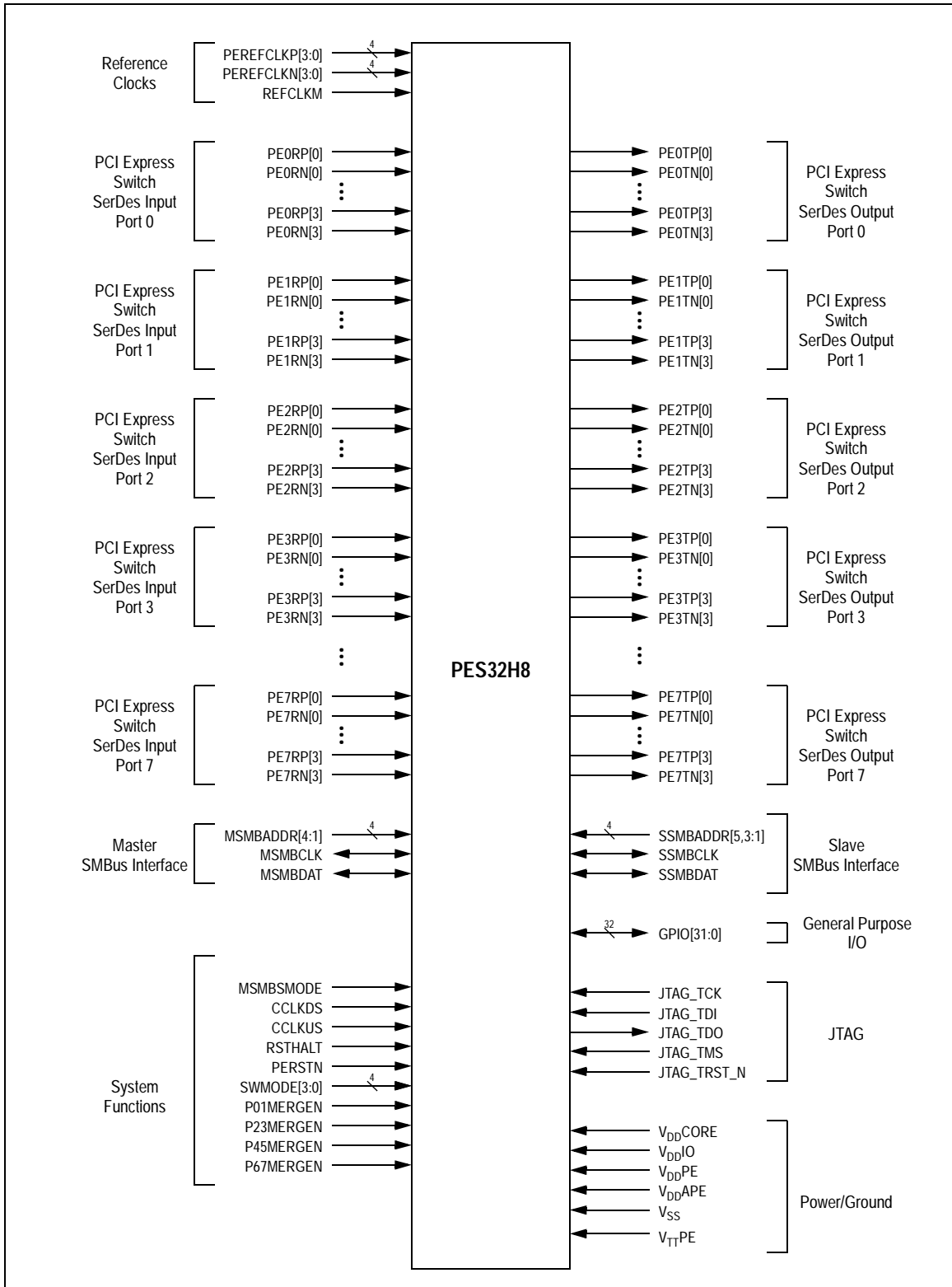
Figure 1.2 PES32H8 Logic Diagram
