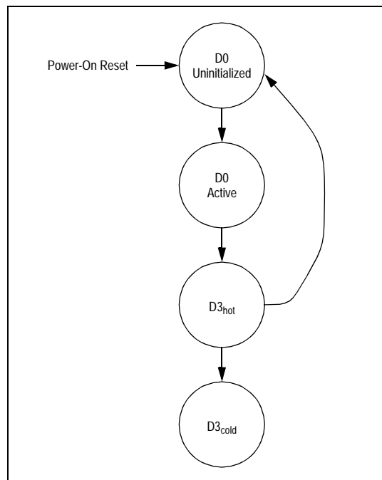
Figure 7.1 PES32H8 Power Management State Transition Diagram
