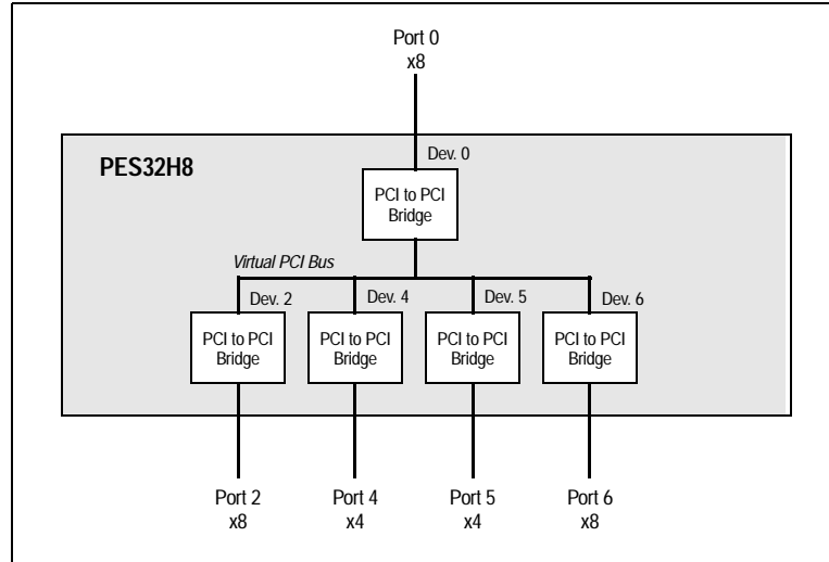
Figure 1.4 Some Ports Merged Configuration
