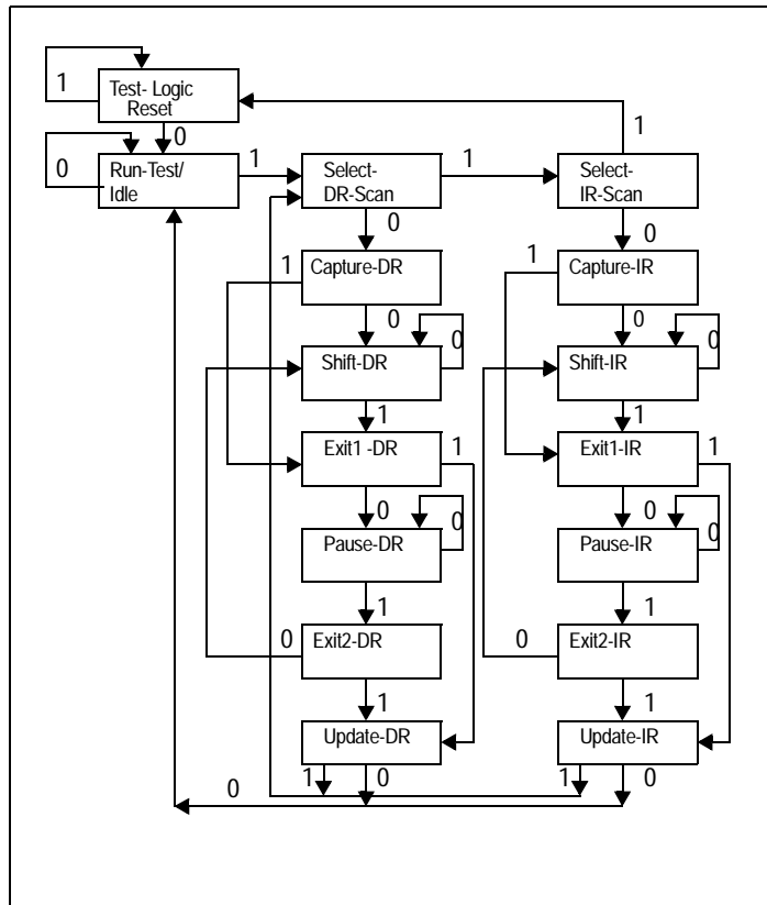
Figure 10.2 State Diagram of PES32H8's TAP Controller
