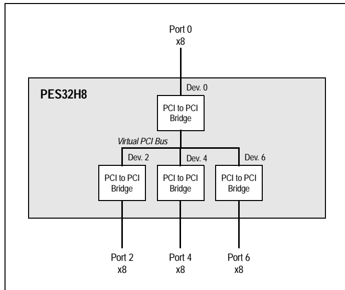
Figure 1.5 All Ports Merged Configuration
