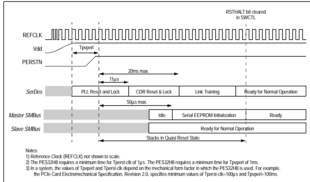
Figure 3.5 Fundamental Reset in Transparent Mode with Serial EEPROM Initialization
