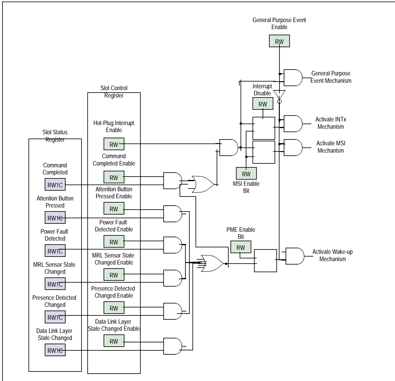
Figure 8.4 PES32H8 Hot-Plug Event Signalling
