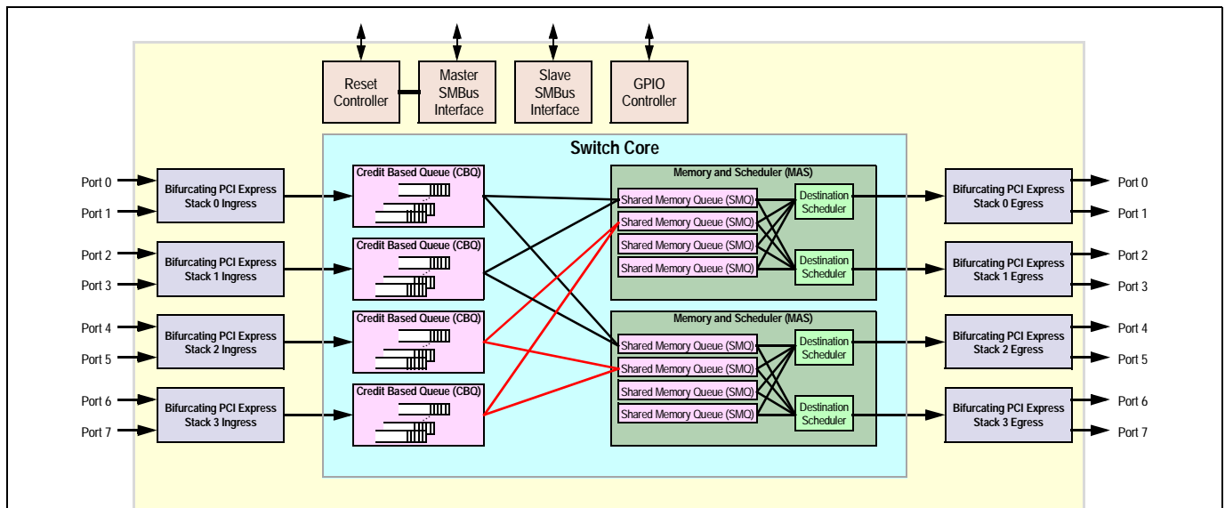
Figure 1.1 PES32H8 Architectural Block Diagram
