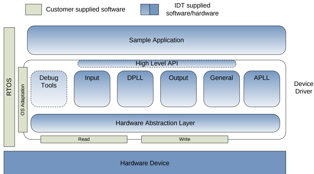
Figure 1 Device driver architecture
