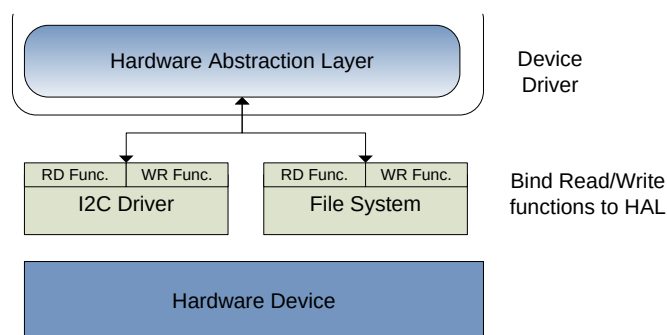
Figure 2 Hardware abstraction layer (HAL)
