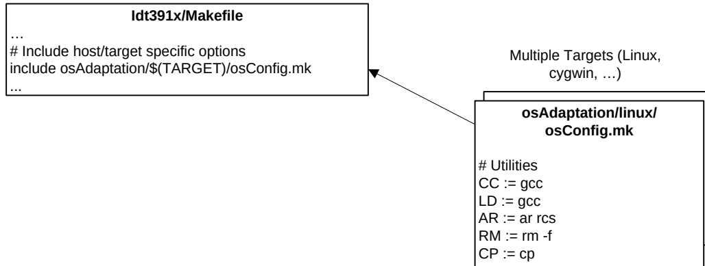
Figure 3 Makefile Hierarchy
