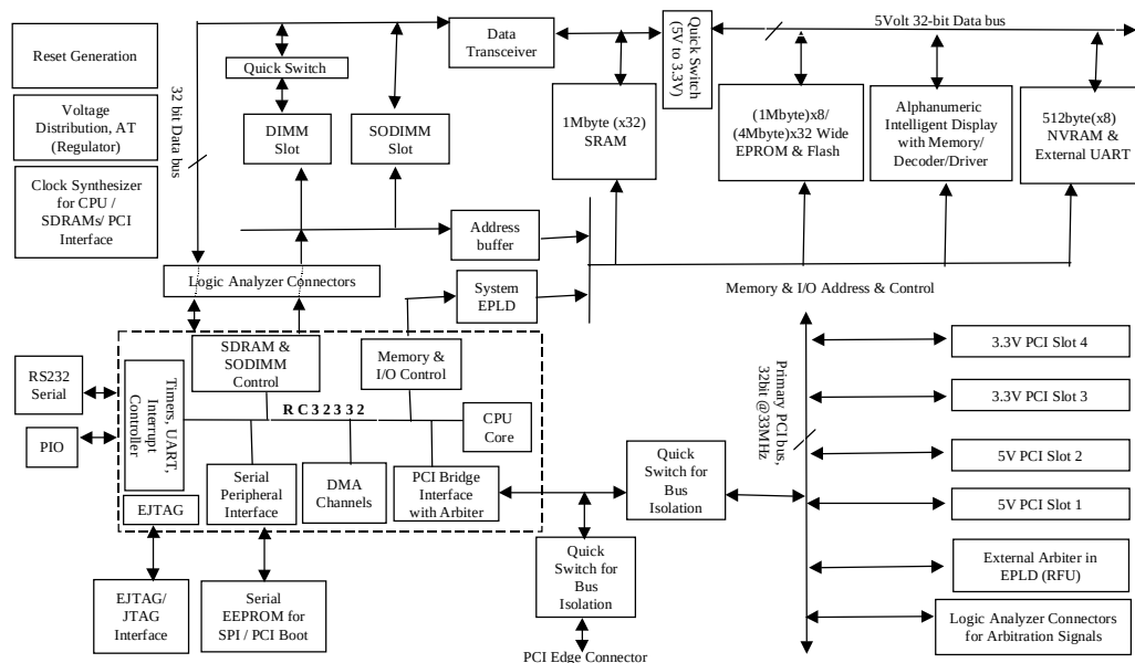
Figure 1.1 79S332 Evaluation Board Block Diagram
