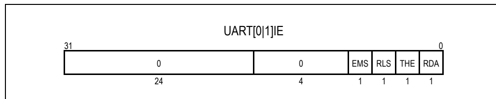
Figure 13.4 UART [0|1] Interrupt Enable Register (UART[0|1]IE)
