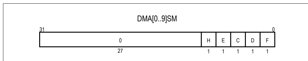
Figure 9.8 DMA [0..9] Status Mask Register (DMA[0..9]SM)
