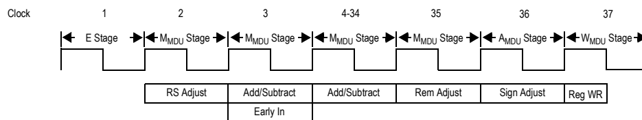
Figure 2.12 MDU Pipeline Flow During a 32-bit Divide (DIV) Operation
