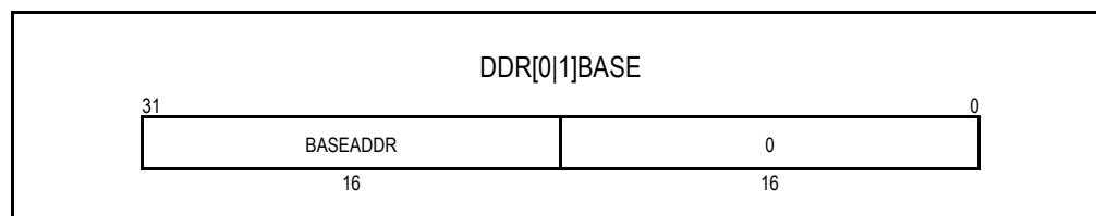
Figure 7.5 DDR [0|1] Base Register (DDR[0|1]BASE)
