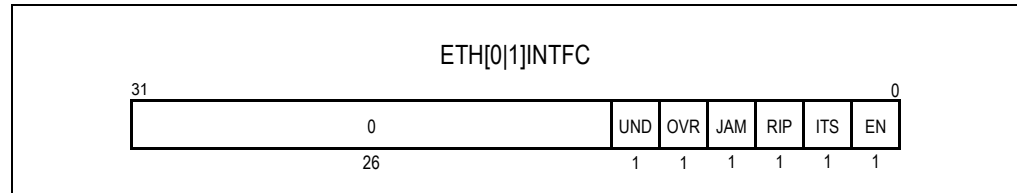
Figure 11.2 Ethernet Interface Control Register (ETH[0]INTFC)
