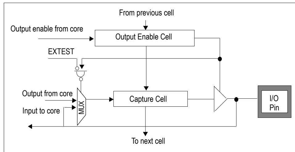
Figure 19.7 Diagram of Bidirectional Cell
