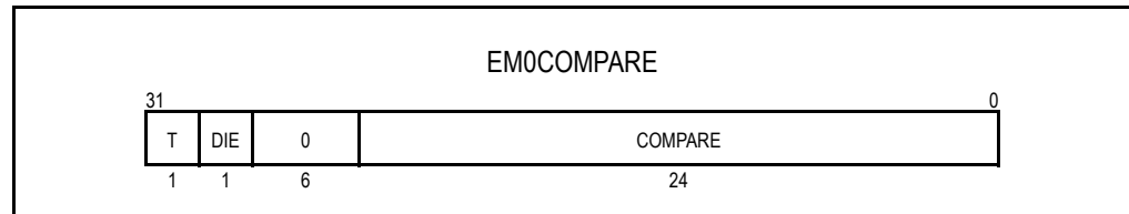
Figure 18.20 Event Monitor 0 Compare Register (EM0COMPARE)
