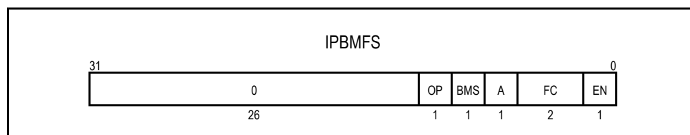
Figure 18.9 IPBus Monitor Filter Select Register (IPBMFS)
