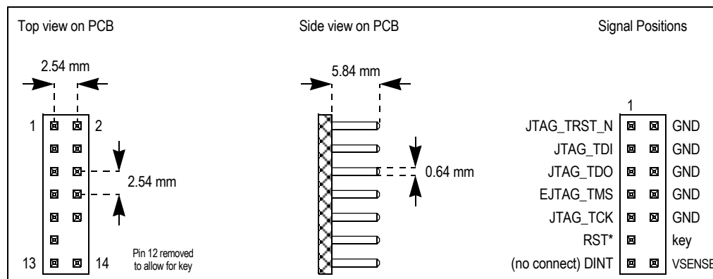
Figure 20.37 EJTAG Connector Mechanical Dimensions
