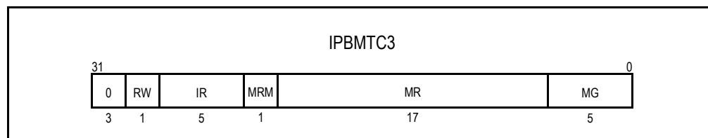
Figure 18.8 IPBus Monitor Trigger Condition 3 Register (IPBMT C3)
