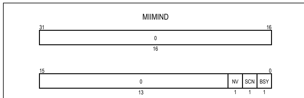
Figure 11.34 MII Management Indicators Register (MIIMIND)
