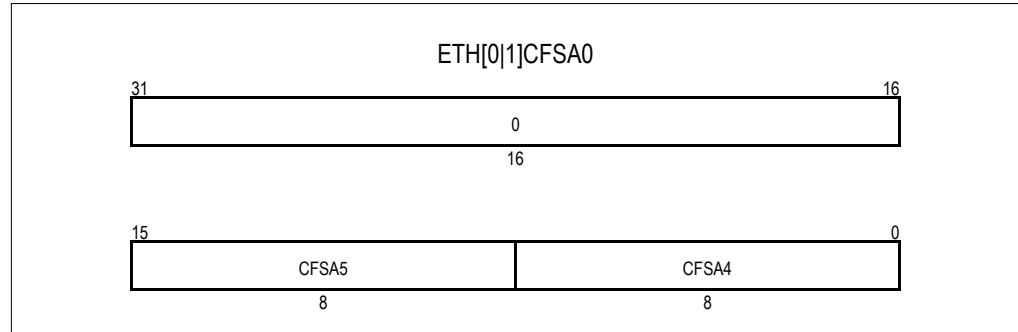
Figure 11.19 Ethernet Control Frame Station Address 0 (ETH[0][1]CFSA0)
