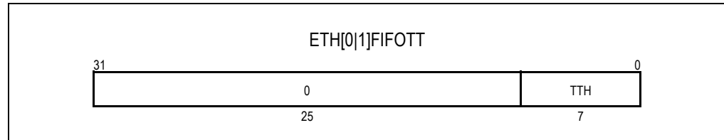
Figure 11.3 Ethernet FIFO Transmit Threshold Register (ETH[0]FIFOTT)
