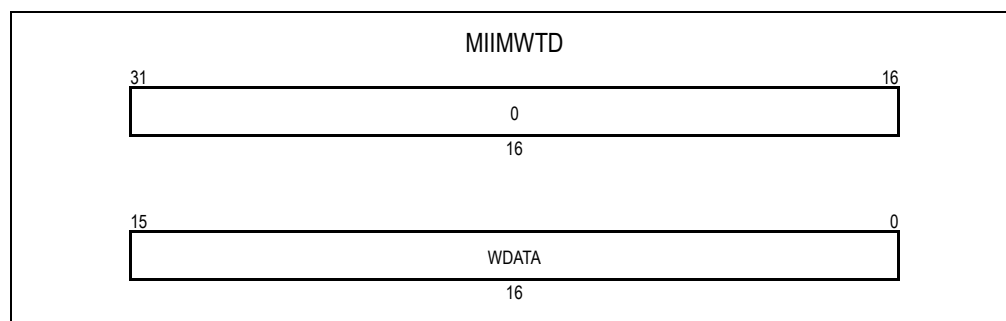
Figure 11.32 MII Management Write Data Register (MIIMWTD)
