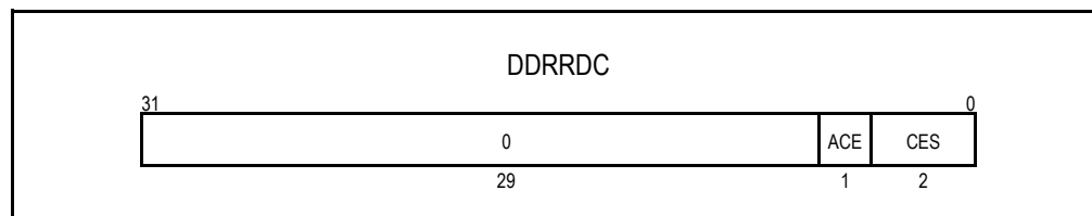
Figure 7.3 DDR Read Data Capture Register (DDRRDC)
