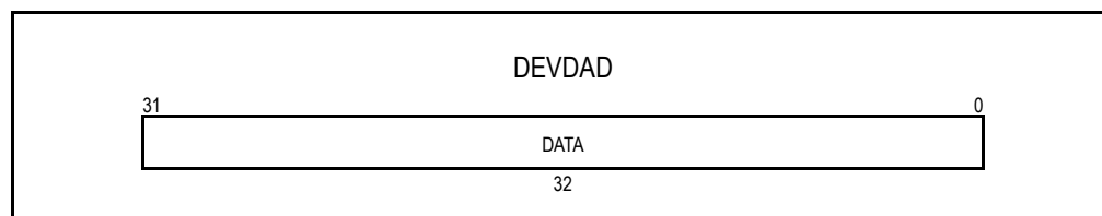
Figure 6.18 Device Decoupled Access Data Register (DEVDAAR)
