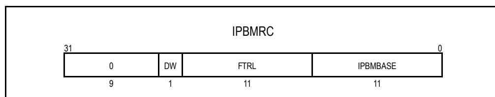
Figure 18.13 IPBus Monitor Record Control Register (IPBMRC)
