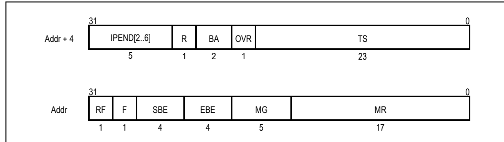
Figure 18.16 IPBus Monitor Transaction Summary Record Format
