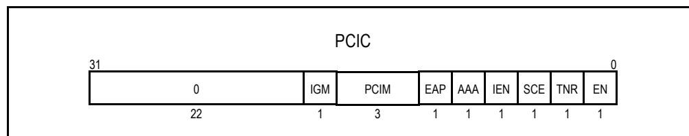
Figure 10.2 PCI Control Register (PCIC)
