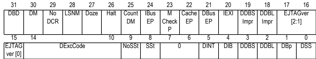
Figure 20.3 Debug Register Format
