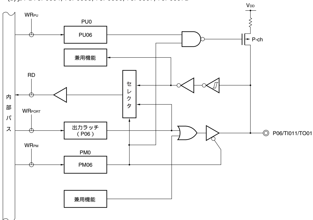
(b) \mu PD78F0394, 78F0395, 78F0396, 78F0397, 78F0397D
