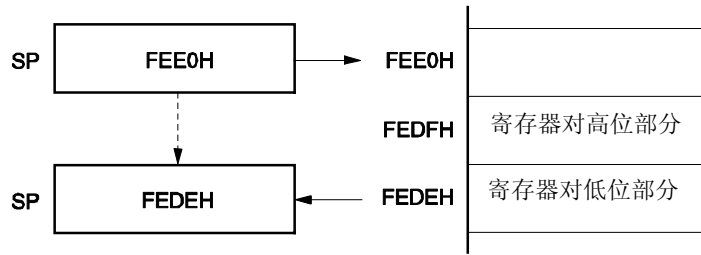
(b) CALL, CALLE, CALLT 指令 (当 SP = FEE0H)
