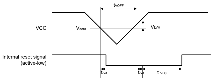
Figure 35.54 Voltage detection circuit timing ( V_{det0} )
