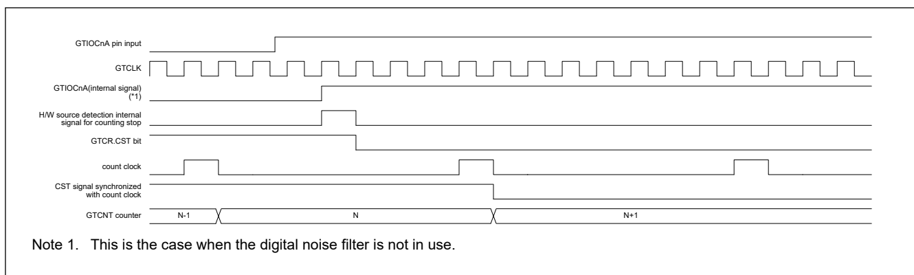
Figure 20.96 Example of timing of operations to stop counting in response to a rising edge of the input on the GTIOCN pin
