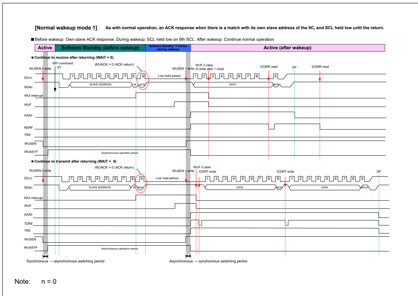
Figure 25.32 Timing of normal wakeup mode 1
