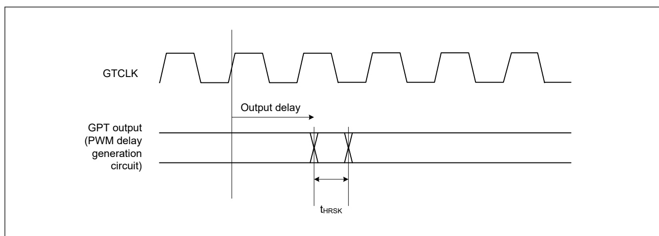
Figure 35.27 GPT (PDG) output delay skew
