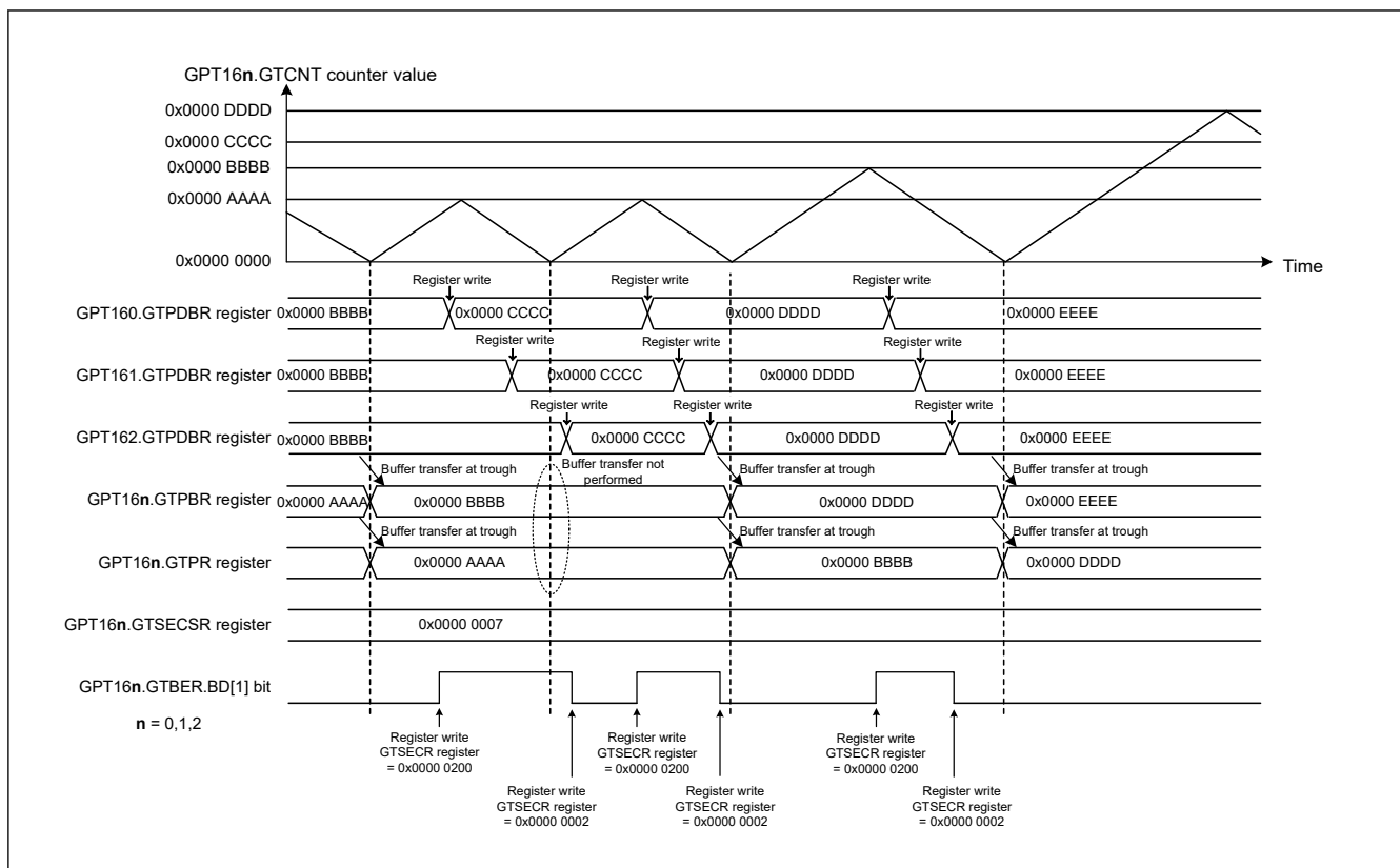
Figure 20.164 Example of multiple channel operation for disabling buffer operation (triangle-waves, double buffer operation)
