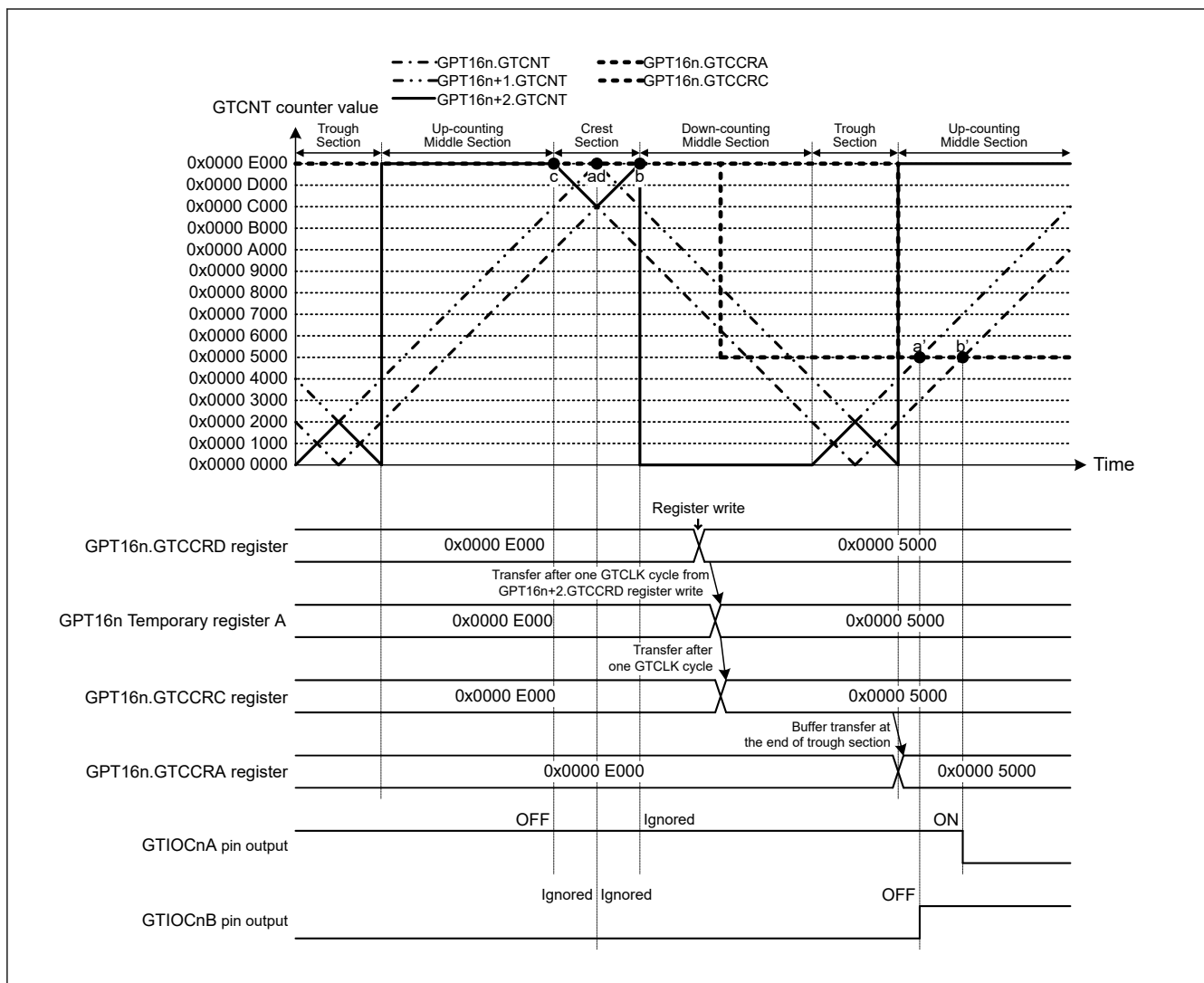
Figure 20.60 Example of compare match generation sequence operation in complementary PWM mode (complementary PWM mode 3 single buffer operation, GTIOCnA pin = low/GTIOCnB pin = high at GTCCRA register compare match during up-counting, GTIOCnA pin = high/GTIOCnB pin = low at GTCCRA register compare match during down-counting, the dead time value is 0x0000 2000, compare match generation order: c → (a, d) → b) (n = 0)
