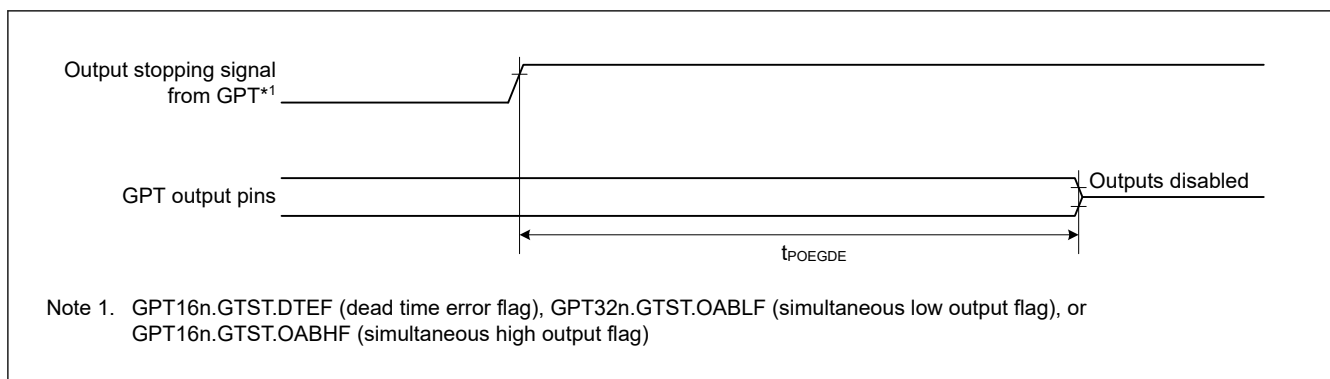
Figure 35.16 Output disable time for POEG in response to detection of the output stopping signal from GPT
