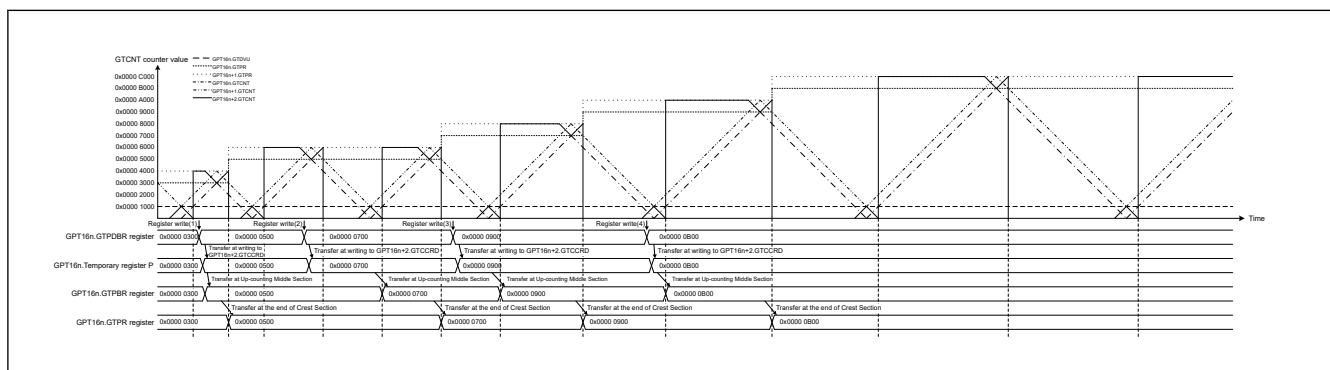
Figure 20.21 Example of GTPR double buffer operation with complementary PWM mode 1
