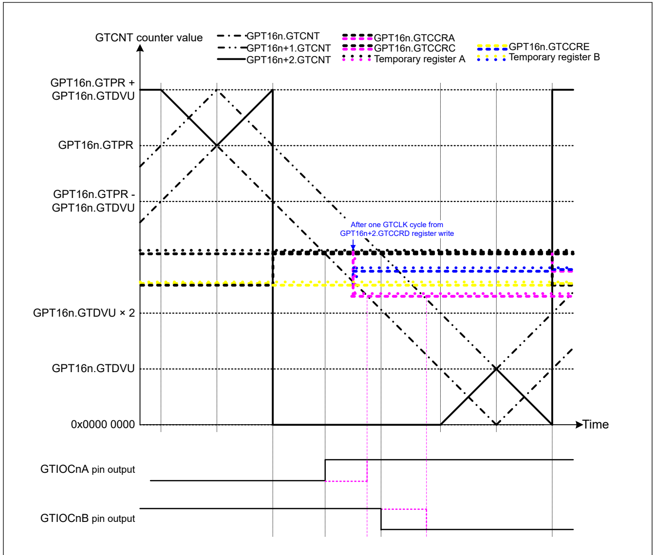
Figure 20.78 Example of complementary PWM mode 4 double buffer operation (down-counting middle section) (complementary PWM mode 4 double buffer operation, GTIOcNA pin = low/GTIOcNB pin = high at GTCCRA register compare match during up-counting, GTIOcNA pin = high/GTIOcNB pin = low at GTCCRA register compare match during down-counting, when a value is written to GTCCRD register during the down-counting dead time) (n = 0)
