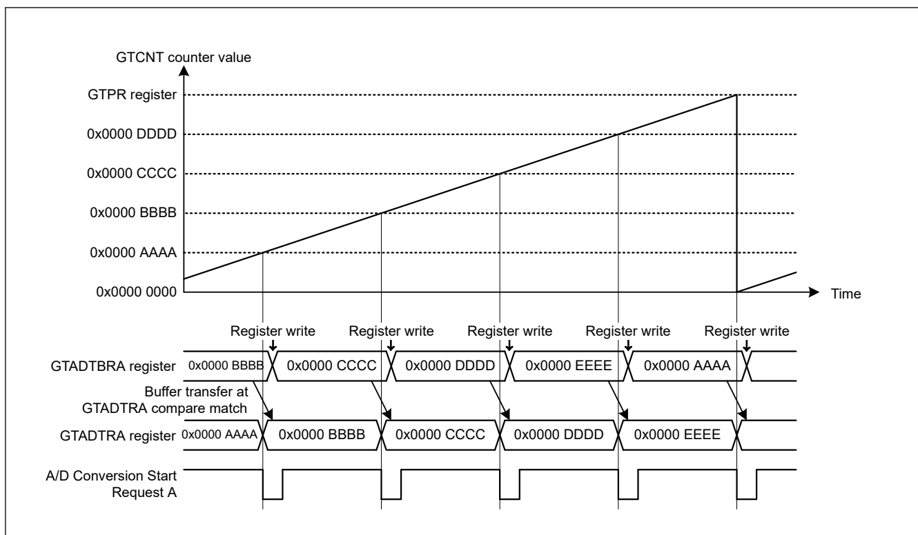
Figure 20.31 Example of buffer operation of the GTADTRA and GTADTRB registers (saw waves in up-counting, buffer transfer at GTADTRA compare match, A/D conversion start request generated by up-counting)
