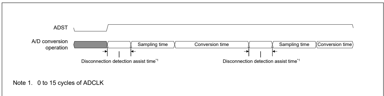
Figure 29.31 Operation of A/D conversion when disconnection detection assist function is used
