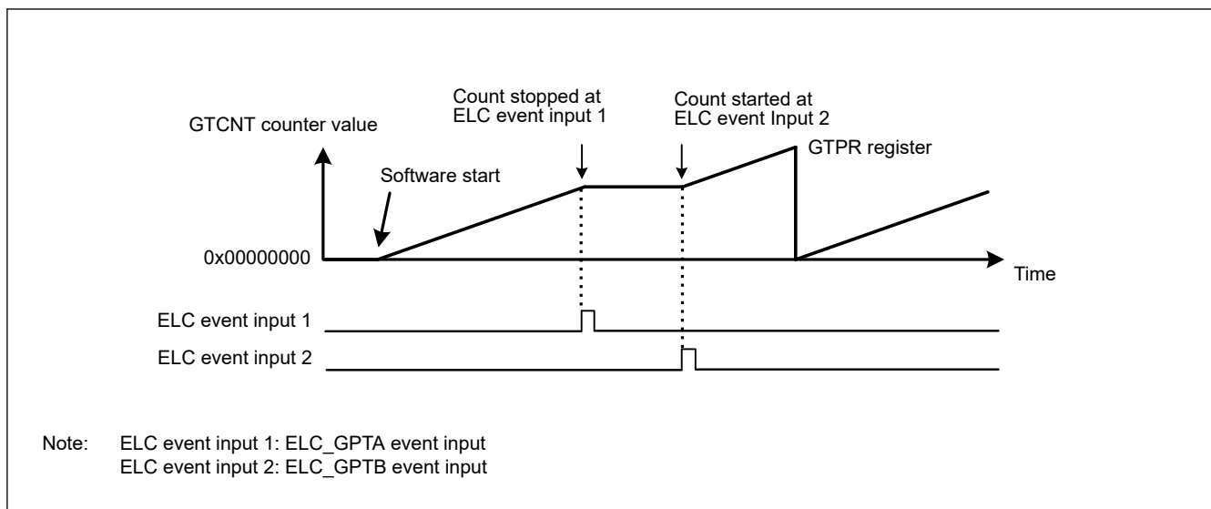
Figure 20.93 Example of count stop operation by hardware source started by software, stopped at ELC_GPTA input, and restarted at ELC_GPTB input
