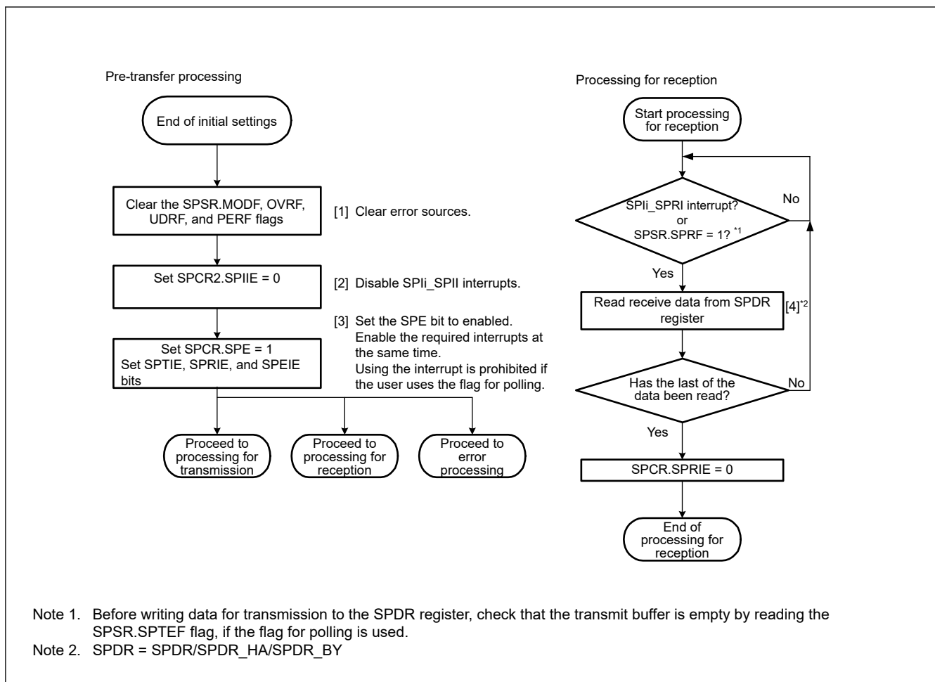
Figure 26.37 Reception flow in slave mode
