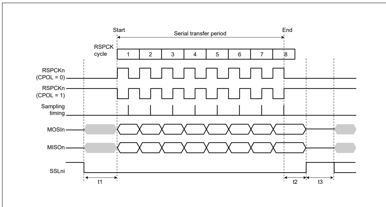
Figure 26.22 SPI transfer format when CPHA = 1
