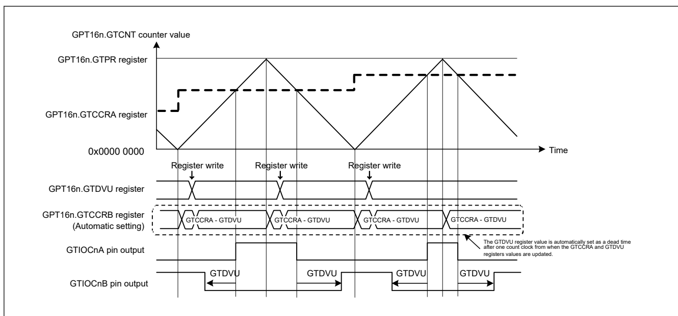
Figure 20.84 Example of automatic compare-match value setting function with dead time in triangle-wave PWM mode 1 and active-high in GPT163
