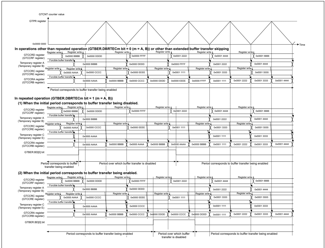
Figure 20.169 Example of repeated double-buffer operation when GTCCR buffer transfer is disabled (triangle-wave PWM mode 3, updating the GTBER.BD[0] bit)
