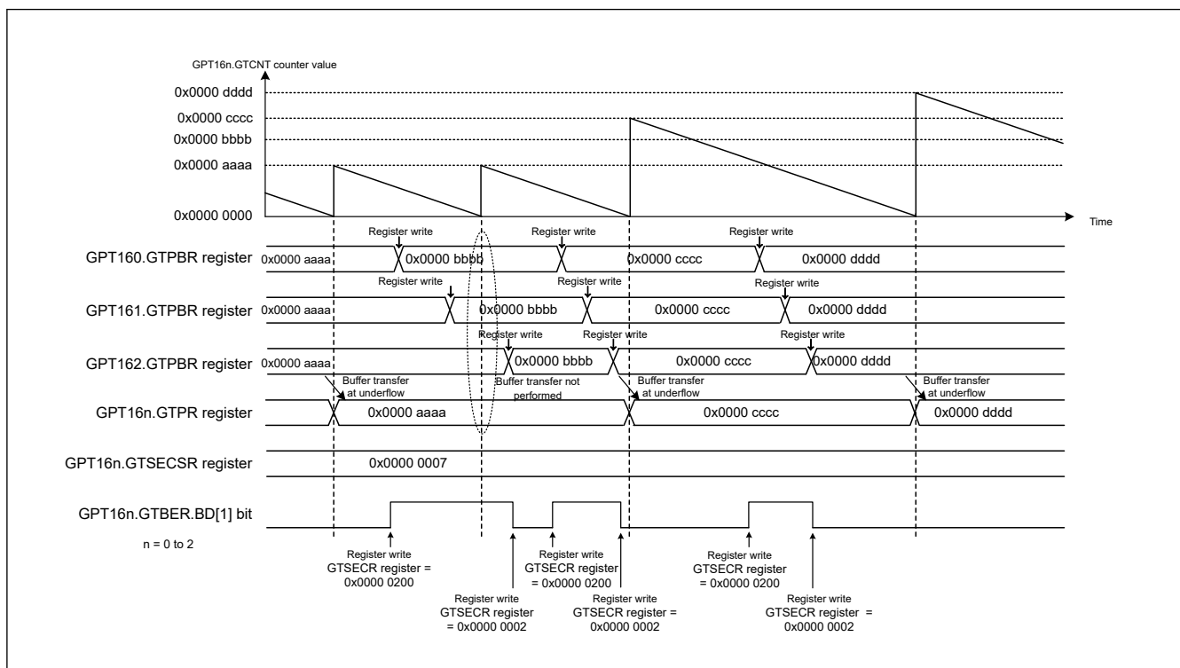
Figure 20.165 Example of multiple channel operation for disabling buffer operation (saw-waves, single buffer operation)
