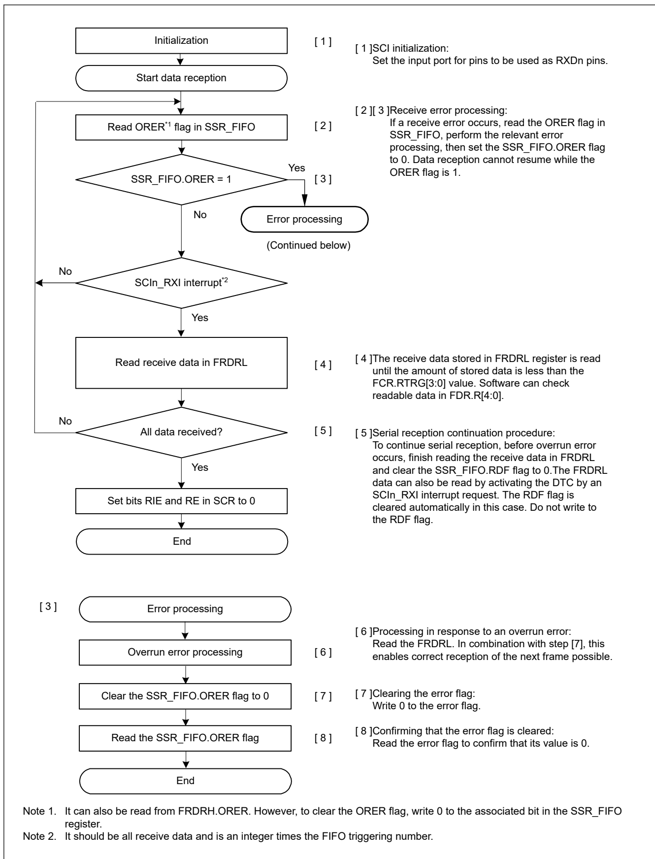
Figure 24.44 Example flow of serial reception in clock synchronous mode with FIFO selected
