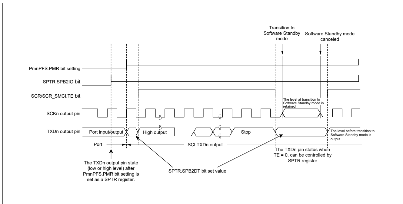
Figure 24.73 Port pin states during transition to Software Standby mode with internal clock and asynchronous transmission
