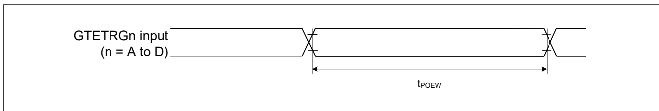
Figure 35.14 POEG input trigger timing
