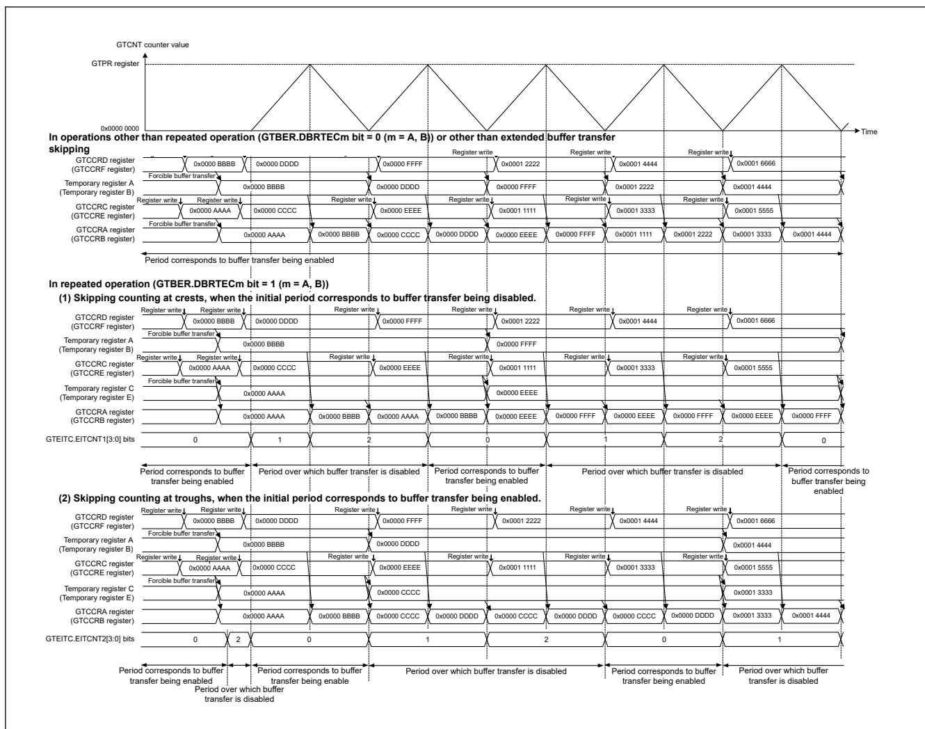
Figure 20.168 Example of repeated double-buffer operation when GTCCR buffer transfer is disabled (triangle-wave PWM mode 3, using extended buffer transfer skipping, GTBER.BD[0] is constantly 0)
