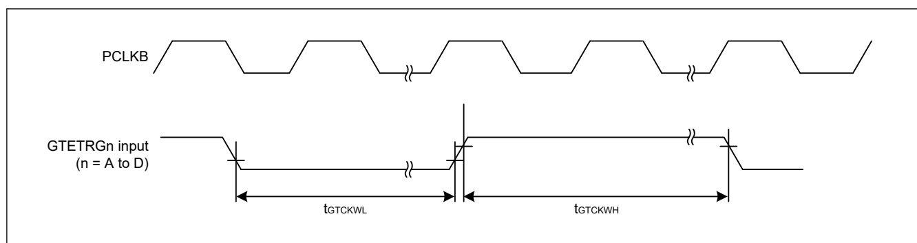
Figure 35.26 GPT clock input timing
