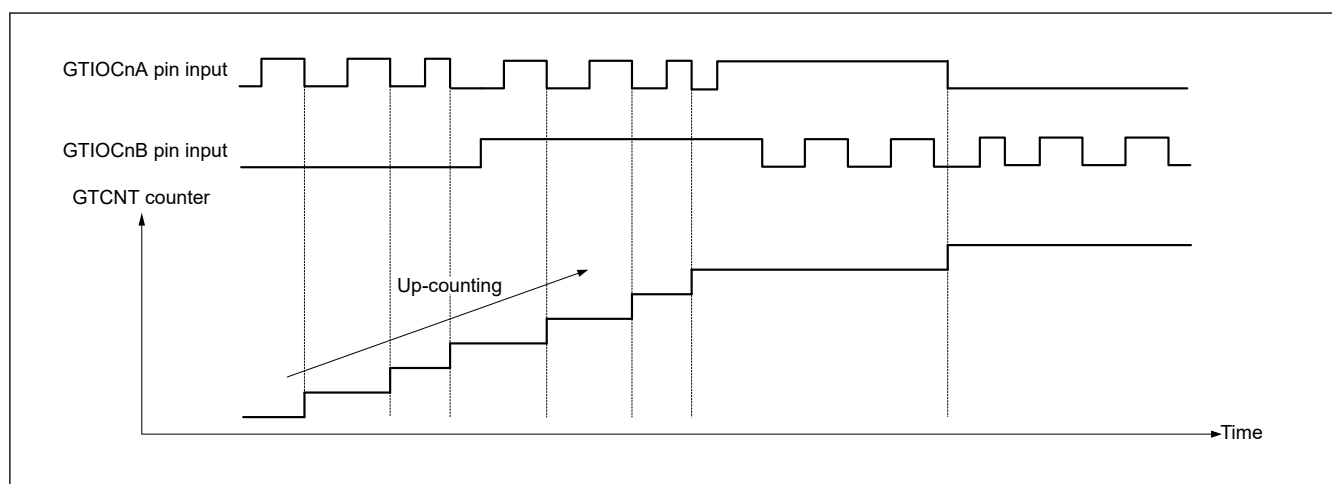
Figure 20.131 Example of phase counting mode 5 (A)
