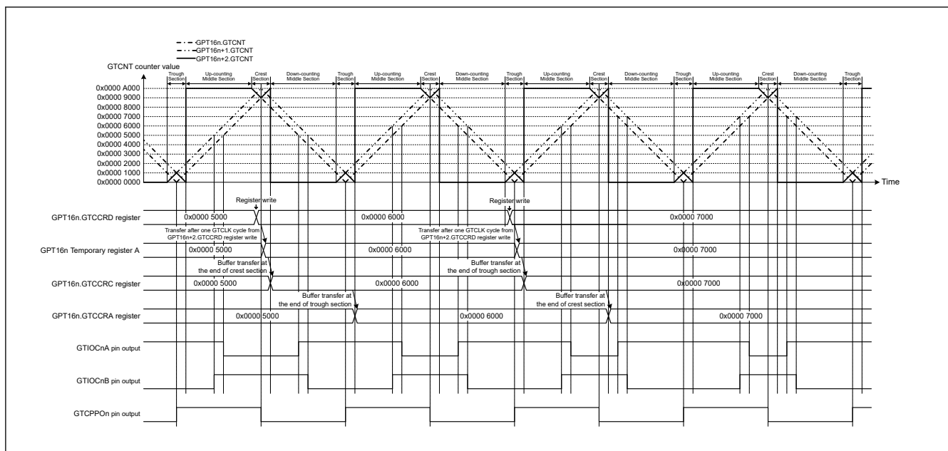
Figure 20.52 Example of complementary PWM mode 3 operation (single buffer operation, GTIOCnA pin = low/GTIOCnB pin = high at GTCCRA register compare match during up-counting, GTIOCnA pin = high/GTIOCnB pin = low at GTCCRA register compare match during down-counting, the dead time value is 0x0000 1000 and updating GTCRD register in crest and trough sections) (n = 0)
