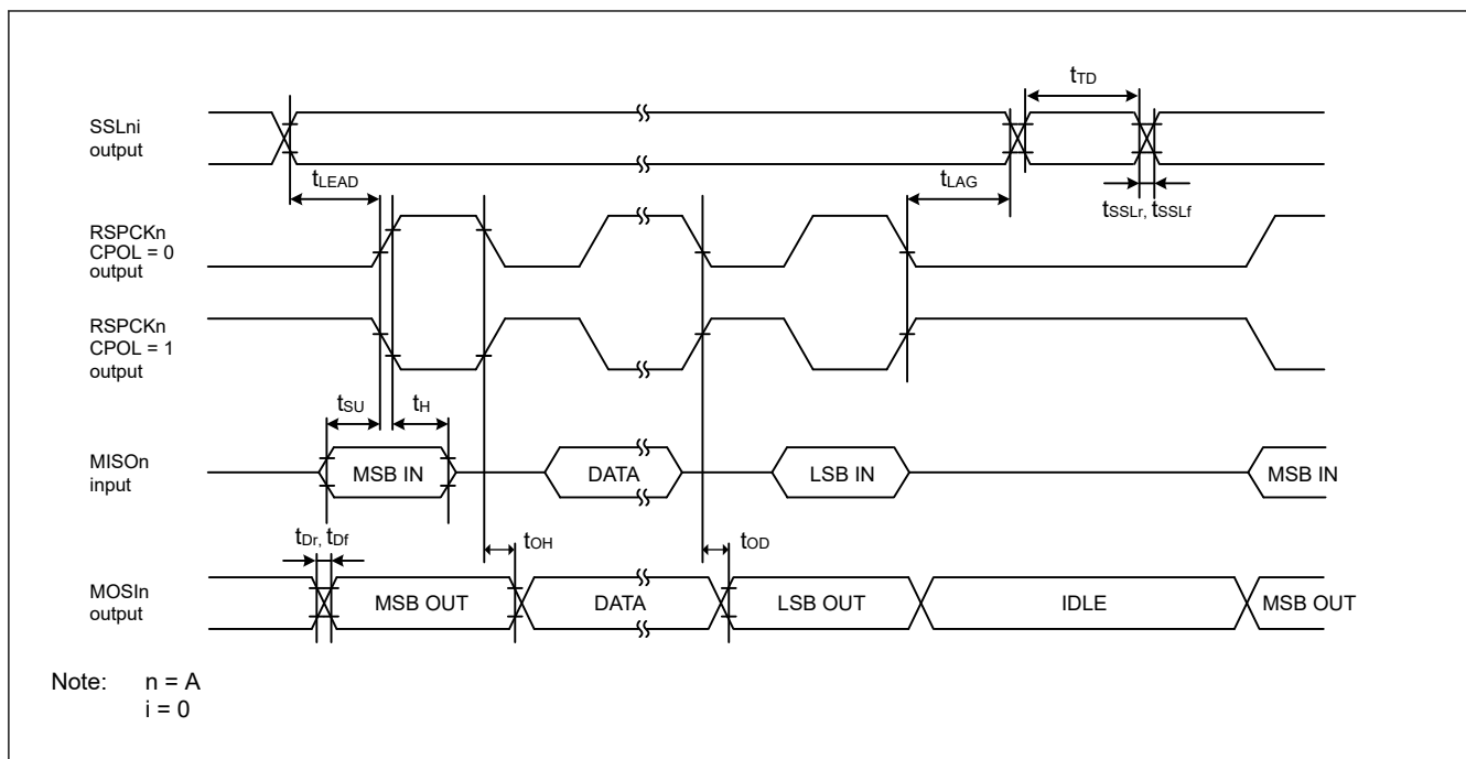
Figure 35.40 SPI timing (master, CPHA = 0) (bit rate: PCLKB division ratio is set to any value other than 1/2)
