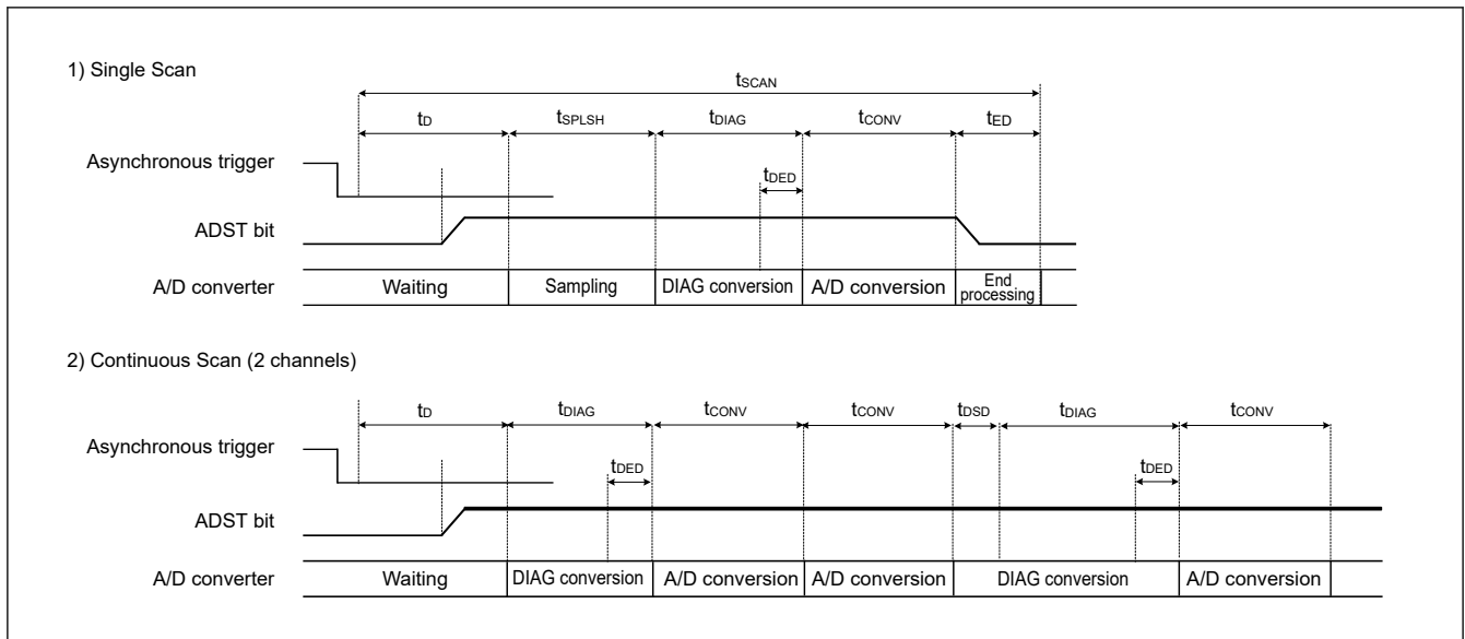
Figure 29.30 Scan conversion timing when activated by an asynchronous trigger input (ADTRG0)
