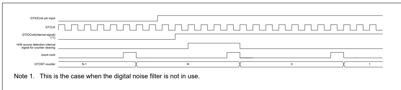
Figure 20.102 Examples of timing of operations for counter clearing in response to a rising edge of the input on the GTIOCnA pin (during the counting of cycles of clock signal produced by dividing the GTCLK frequency)
