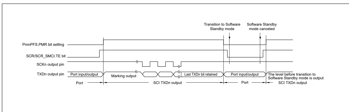
Figure 24.74 Port pin states during transition to Software Standby mode with internal clock and clock synchronous transmission
