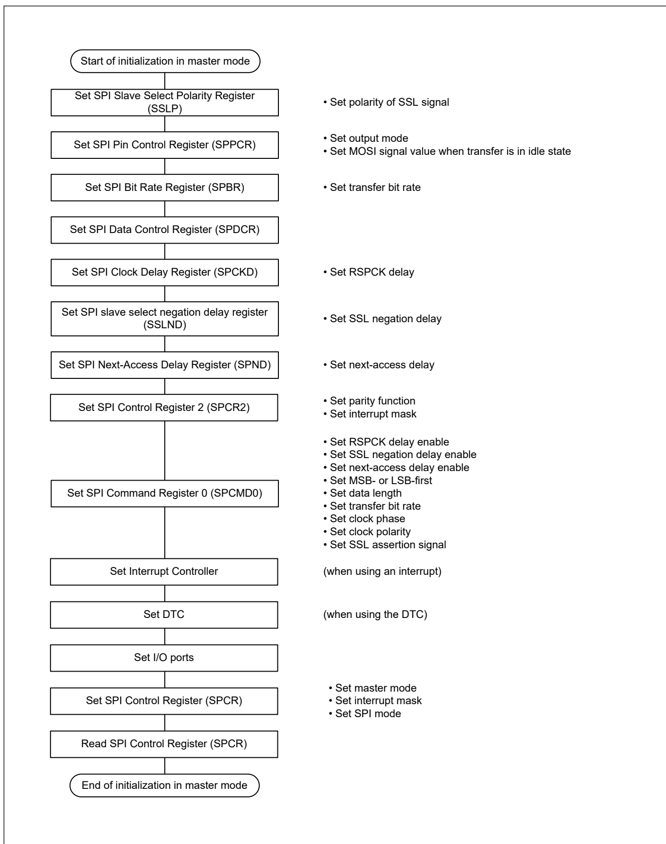
Figure 26.31 Example of initialization flow in master mode for SPI operation
