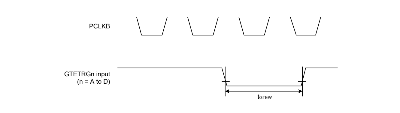
Figure 35.25 GPT external trigger input timing
