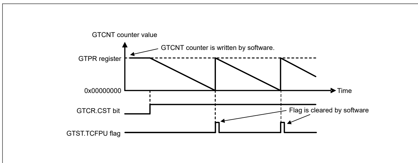
Figure 20.5 Example of periodic count operation in down-counting by the count clock
