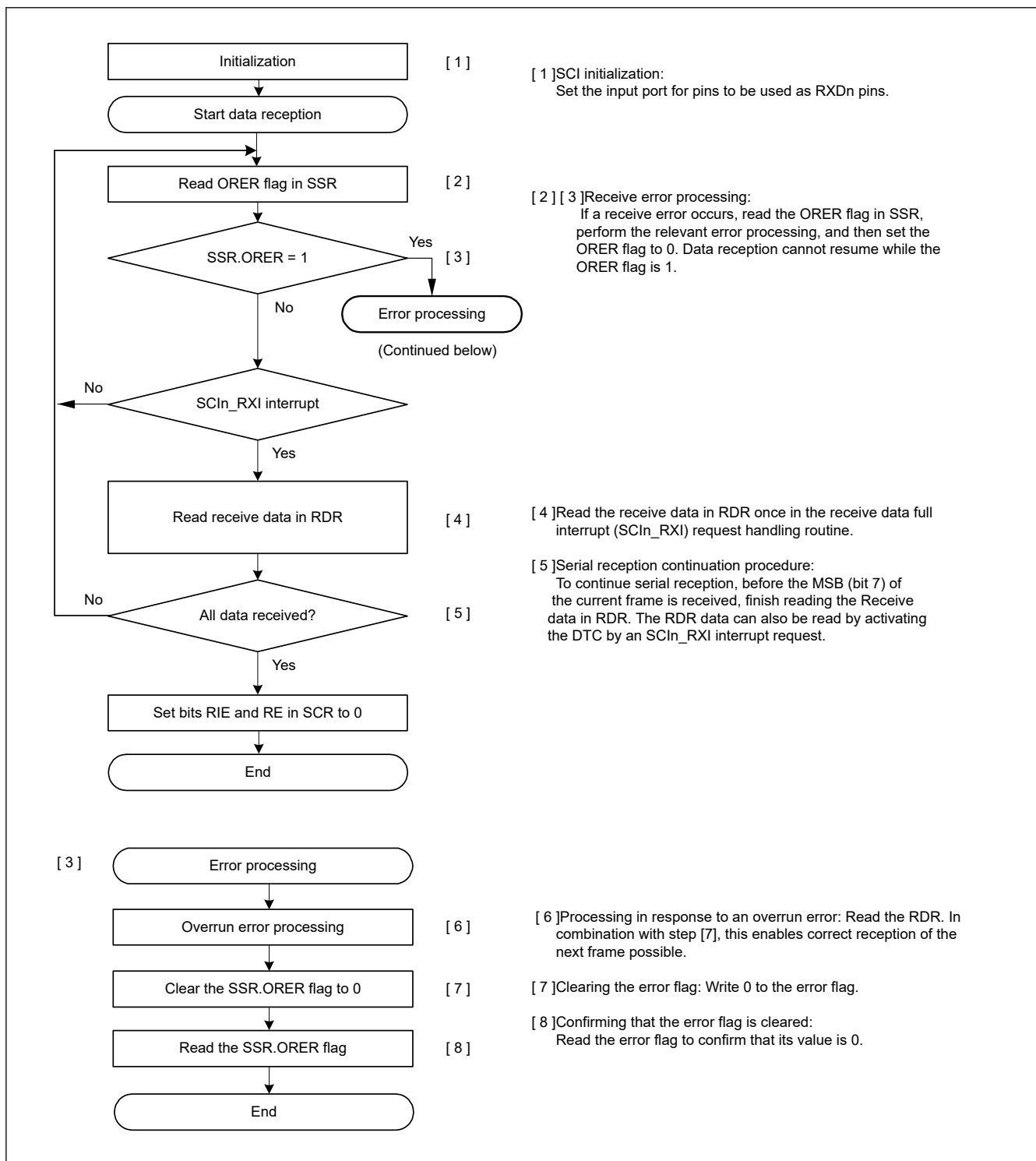
Figure 24.43 Example flow of serial reception in clock synchronous mode with non-FIFO selected
