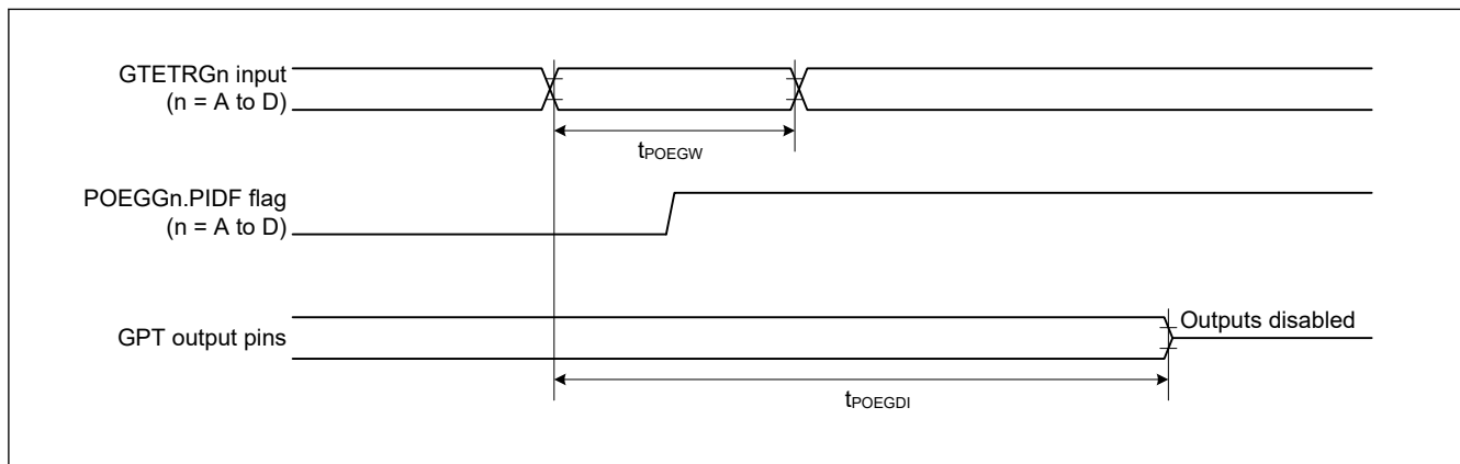
Figure 35.15 Output disable time for POEG via detection flag in response to the input level detection of the GTETRn pin
