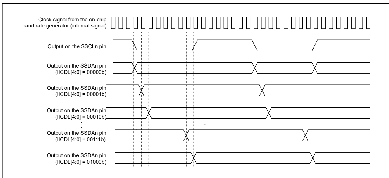
Figure 24.62 Timing of delays in SDAn output
