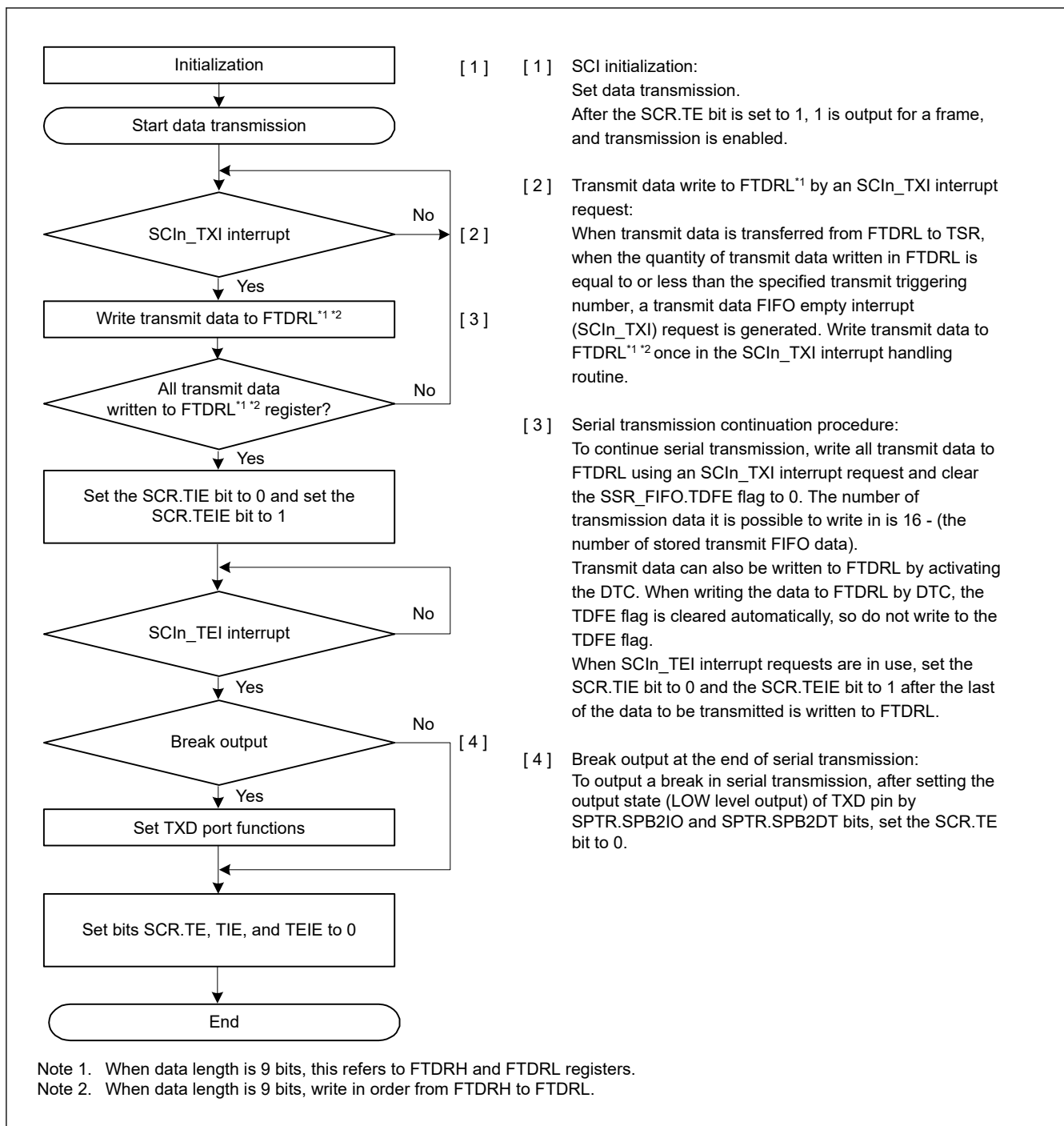
Figure 24.12 Example flow of serial transmission in asynchronous mode with FIFO selected
