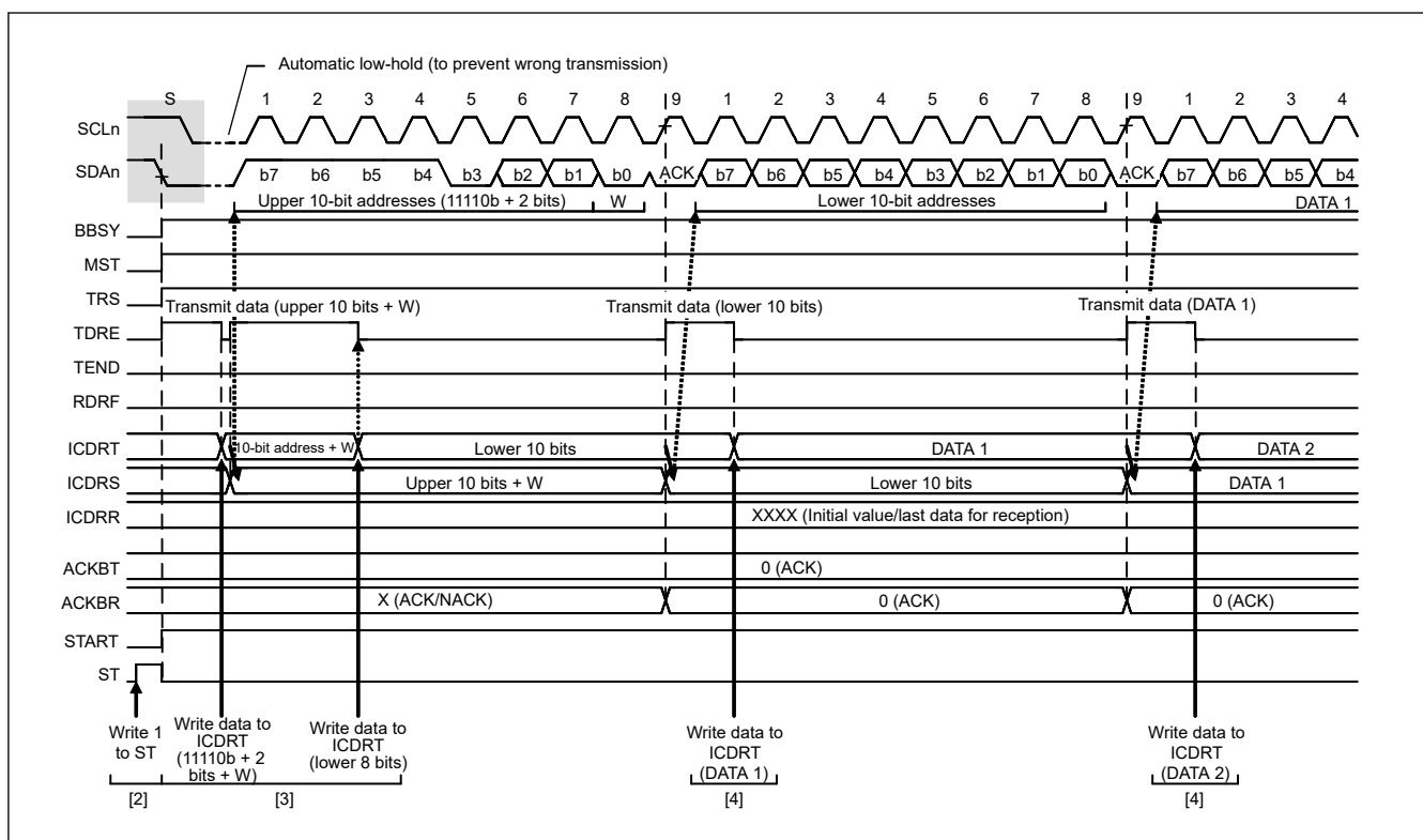
Figure 25.8 Master transmit operation timing (2) with 10-bit address format
