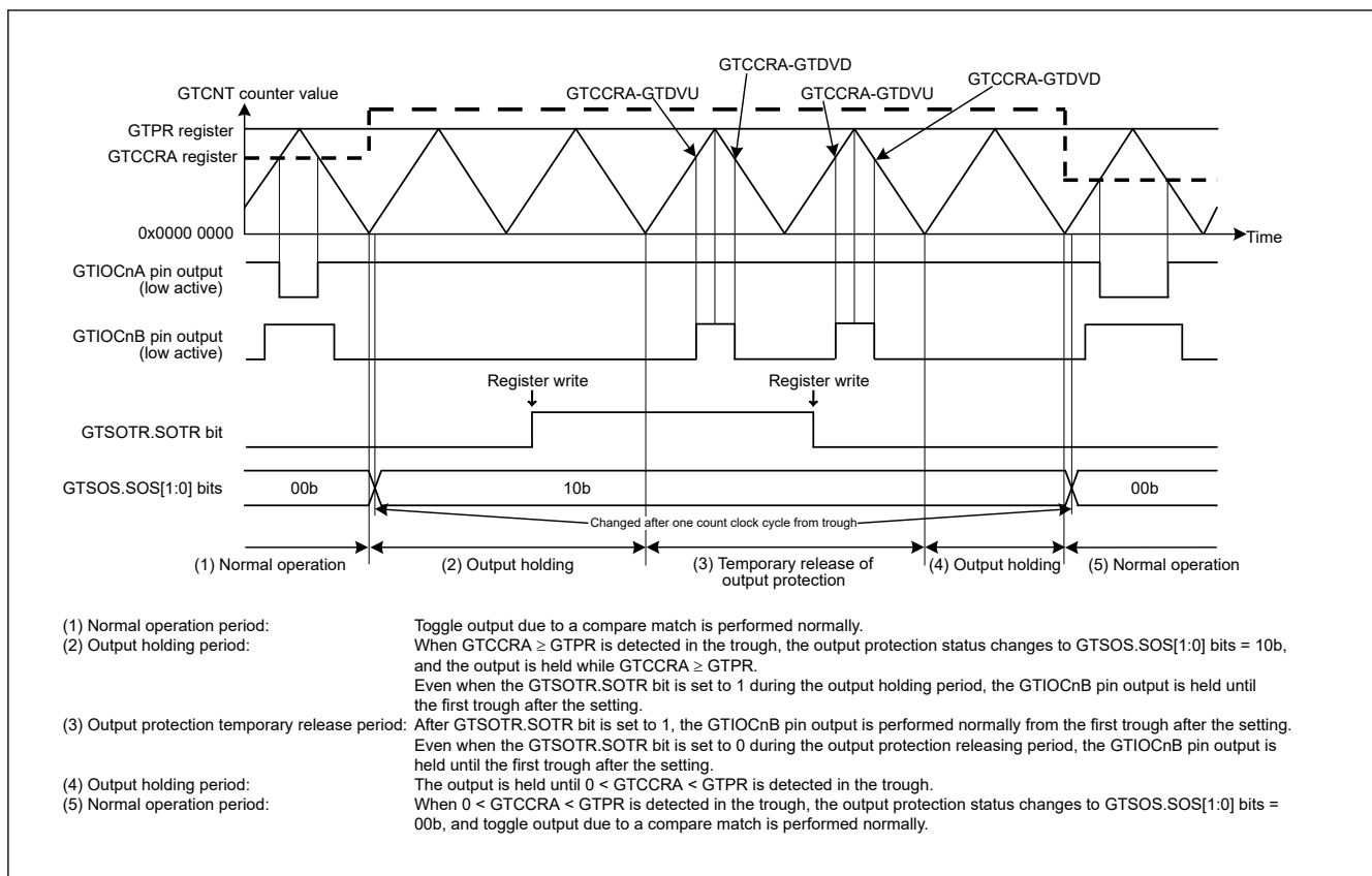
Figure 20.180 Example of temporary release of output protection when the setting of the GTCCRA \geq GTPR during buffer transfer at troughs (restored to 0 < \text{GTCCRA} < \text{GTPR} during buffer transfer at troughs, active level: low) (n = 0 to 2)
