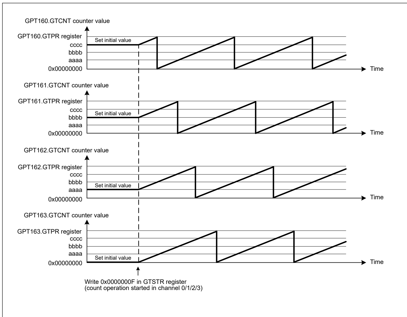
Figure 20.108 Example of software phase start with the same count cycle (GTPR register value)
