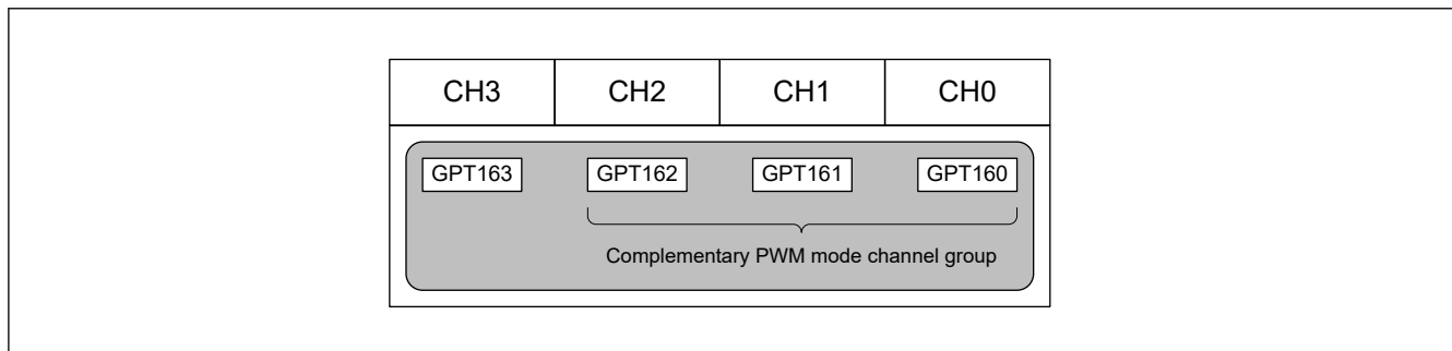
Figure 20.3 Association between GPT channels and module names
