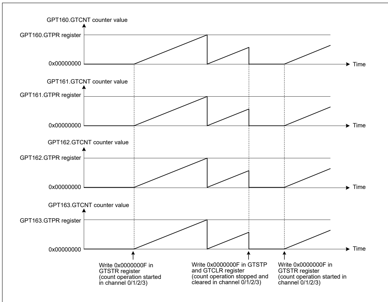
Figure 20.107 Example of a simultaneous start, stop, and clear by software with the same count cycle (GTPR register value)
