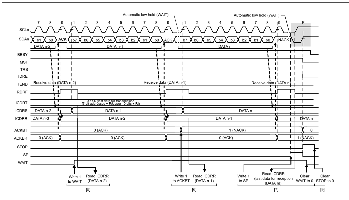
Figure 25.14 Master receive operation timing (3) when RDRFS = 0
