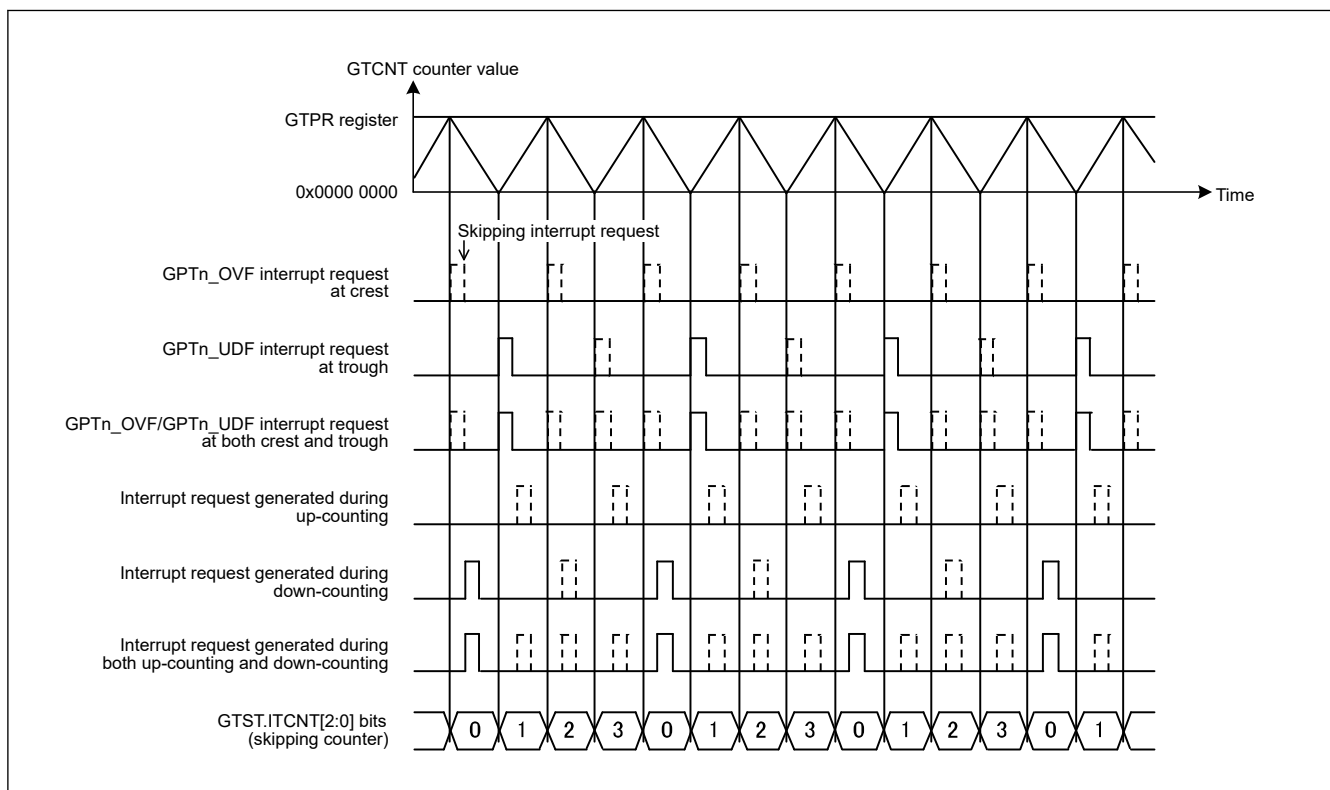
Figure 20.142 Example of Interrupt Skipping Function Operation (Triangle Waves, Counting and Skipping Both Troughs and Crests, Skipping Count: 3, Skipping Started at Up-Counting)
