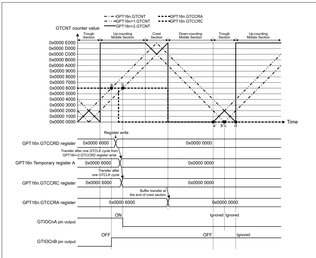
Figure 20.66 Example of compare match generation sequence operation in complementary PWM mode (complementary PWM mode 3 single buffer operation, GTIOCnA pin = low/GTIOCnB pin = high at GTCCRA register compare match during up-counting, GTIOCnA pin = high/GTIOCnB pin = low at GTCCRA register compare match during down-counting, the dead time value is 0x0000 2000, compare match generation order: a' → (b', c) → d) (n = 0)
