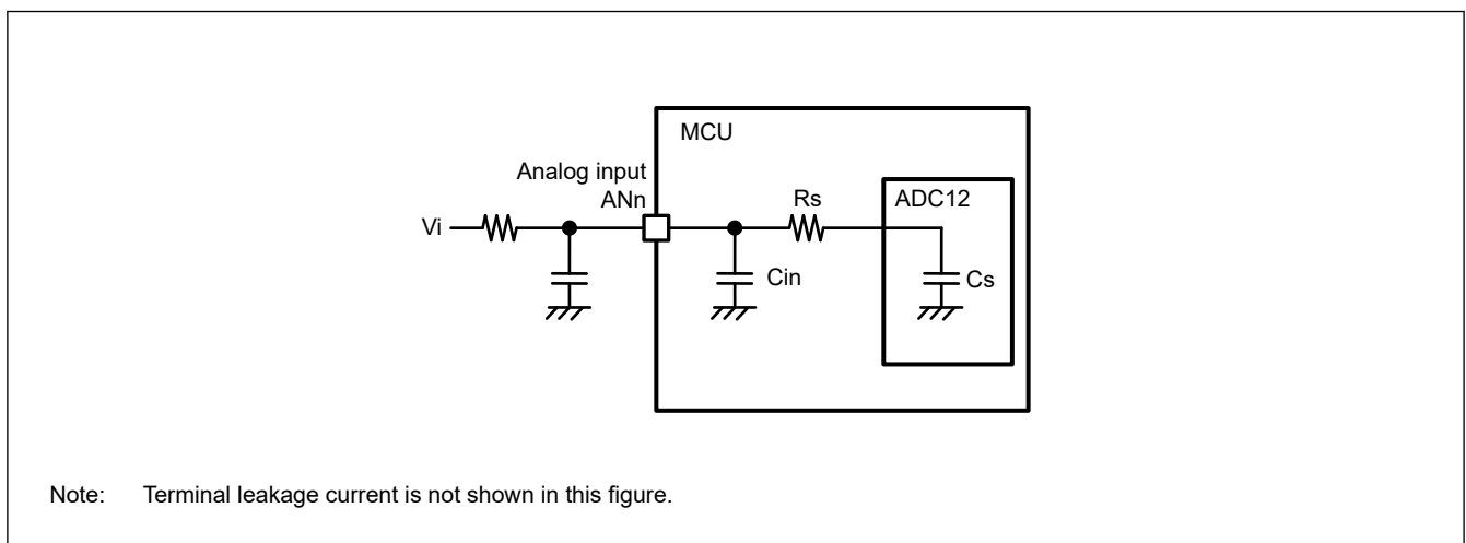
Figure 35.49 Equivalent circuit for analog input
