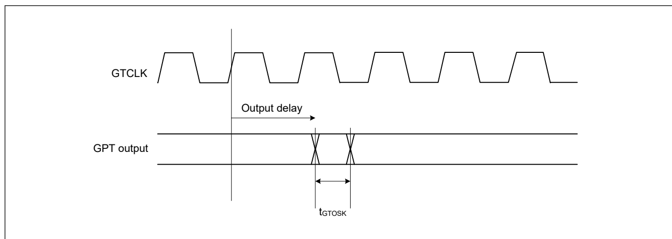
Figure 35.24 GPT output delay skew for OPS
