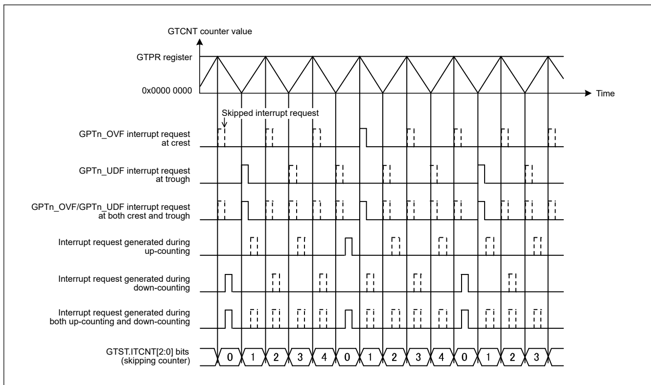
Figure 20.141 Example of Interrupt Skipping Function Operation (Triangle Waves, Counting and Skipping Both Troughs and Crests, Skipping Count: 4)
