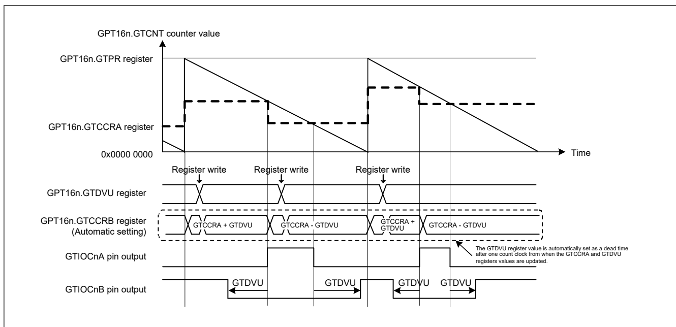
Figure 20.82 Example of automatic dead time setting function operation in saw-wave one-shot pulse mode, down-counting and active-high in GPT163
