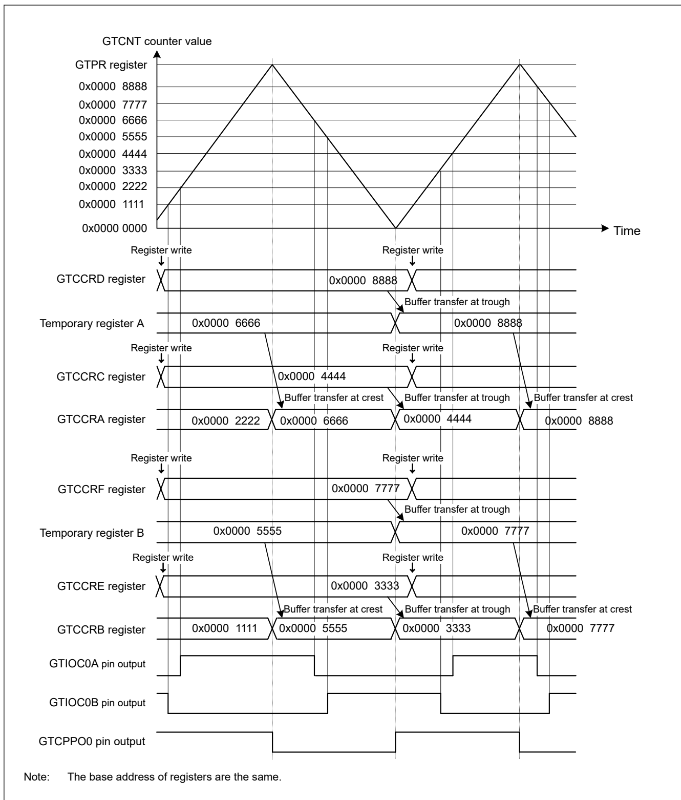
Figure 20.45 Example of triangle-wave PWM mode 3 operation with low output from the GTIOCnA pin and high output from the GTIOCnB pin at count start, output toggled at GTCCRA/GTCCRB compare match, output retained at cycle end, and GTIOR.PSYE = 1
