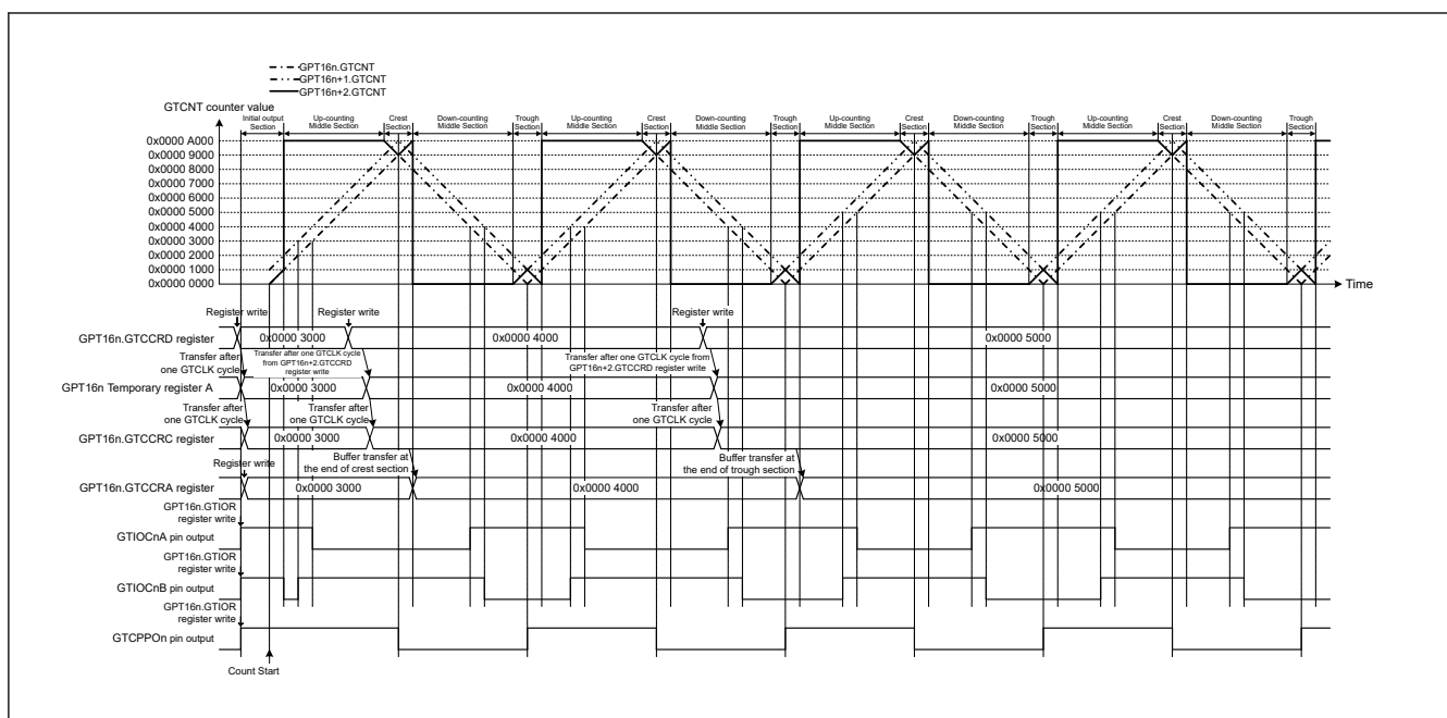
Figure 20.51 Example of complementary PWM mode 3 operation (single buffer operation, GTIOCnA pin = high/GTIOCnB pin = high as initial output, GTIOCnA pin = low/GTIOCnB pin = high at GTCCRA register compare match during up-counting, GTIOCnA pin = high/GTIOCnB pin = low at GTCCRA register compare match during down-counting, the dead time value is 0x0000 1000 and updating GTCCRD register in middle section) (n = 0)
