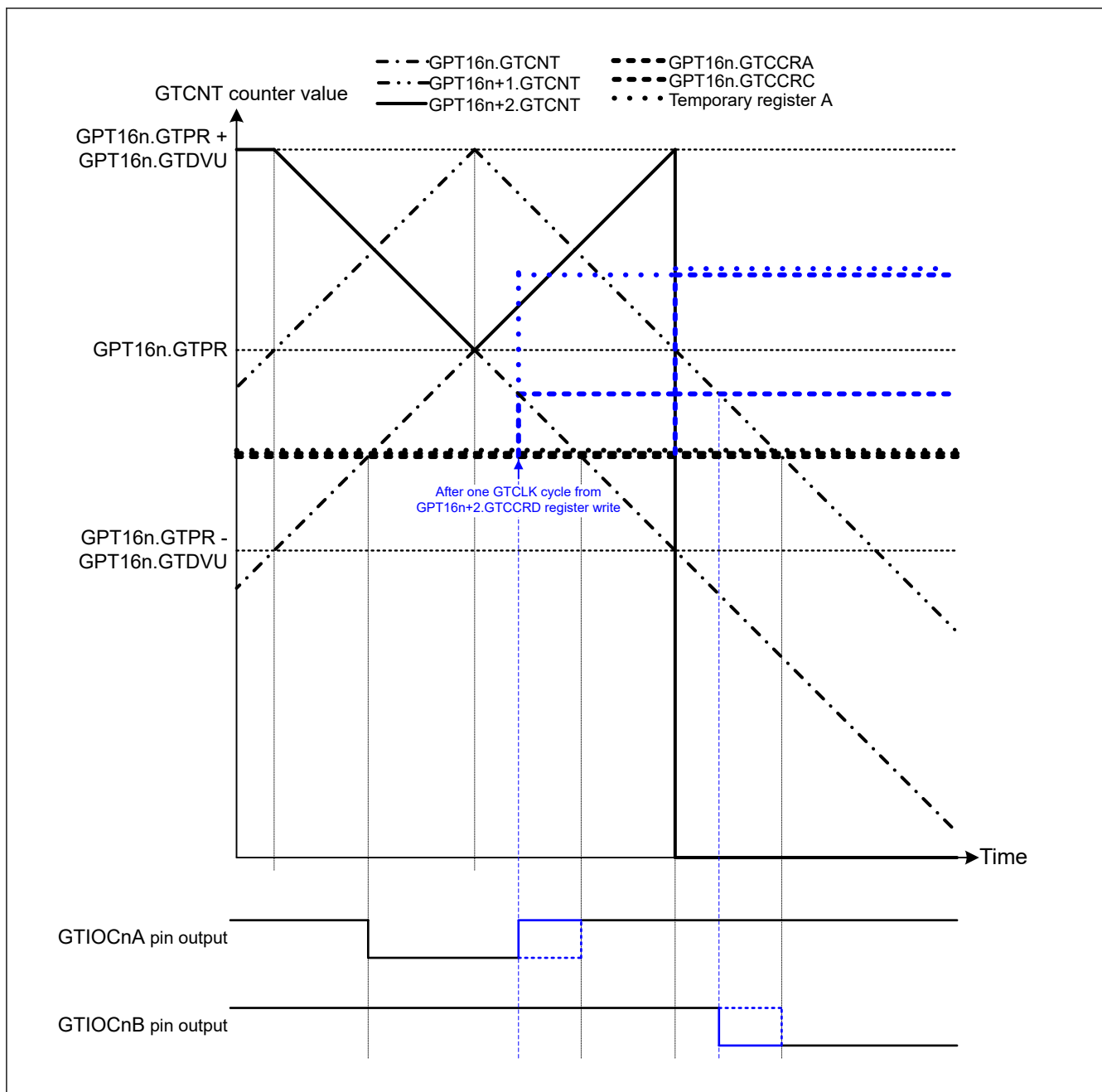
Figure 20.72 Example of complementary PWM mode 4 single buffer operation (down-counting crest section) (complementary PWM mode 4 single buffer operation, GTIOCnA pin = low/GTIOCnB pin = high at GTCCRA register compare match during up-counting, GTIOCnA pin = high/GTIOCnB pin = low at GTCCRA register compare match during down-counting, when a value not less than the GPT16n.GTCNT value is written to GTCCRD register after up-counting compare match before down-counting compare match) (n = 0)
