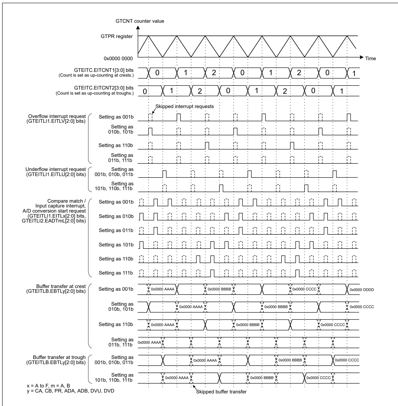
Figure 20.148 Example of extended interrupt skipping function (triangle-waves, count crests by the extended interrupt skipping 1 with skipping count: 2, count troughs by the extended interrupt skipping 2 with skipping count: 2, extended interrupt skipping counter 2 initial value: 1)
