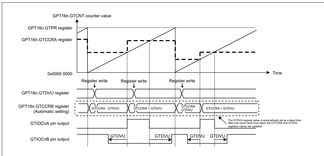
Figure 20.80 Example of automatic dead time setting function operation in saw-wave one-shot pulse mode, up-counting and active-high in GPT163
