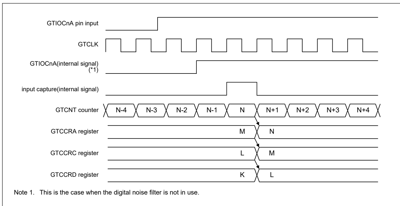
Figure 20.15 Example of the timing of input capture operation in response to a rising edge of the input on the GTIOCnA pin
