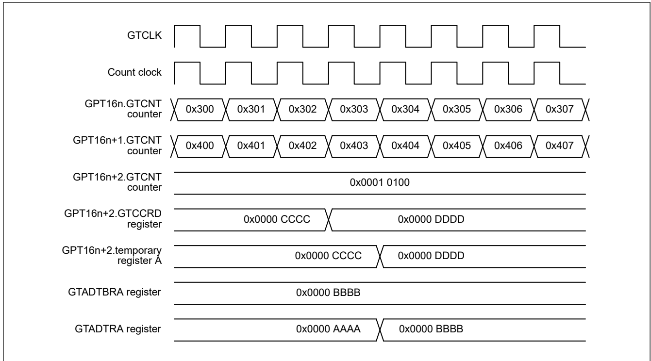
Figure 20.34 Example of buffer operation of the GTADTRA and GTADTRB registers at the GTCCRD register of slave channel 2 updating in complementary PWM mode
