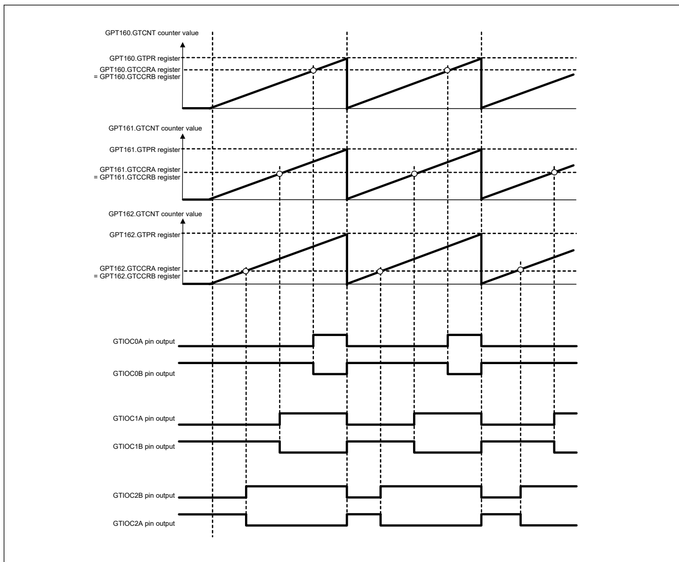
Figure 20.116 Example of 3-phase saw-wave complementary PWM output
