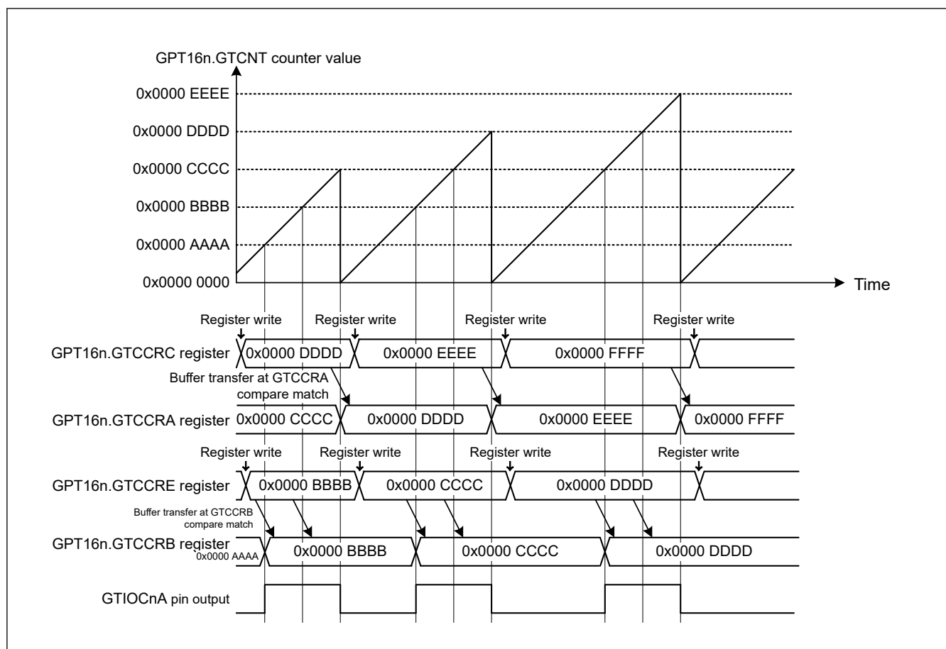
Figure 20.25 Example of GTCCRA and GTCCRB registers buffer operation (output compare, saw-wave PWM mode 2, buffer transfer at GTCCRA register compare match, counter clearing, low output, buffer transfer at GTCCRB register compare match, high output) (n = 0 to 2)
