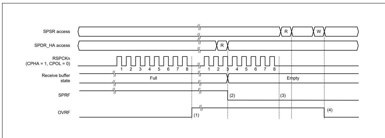
Figure 26.27 Operation example of the OVRF and SPRF flags
