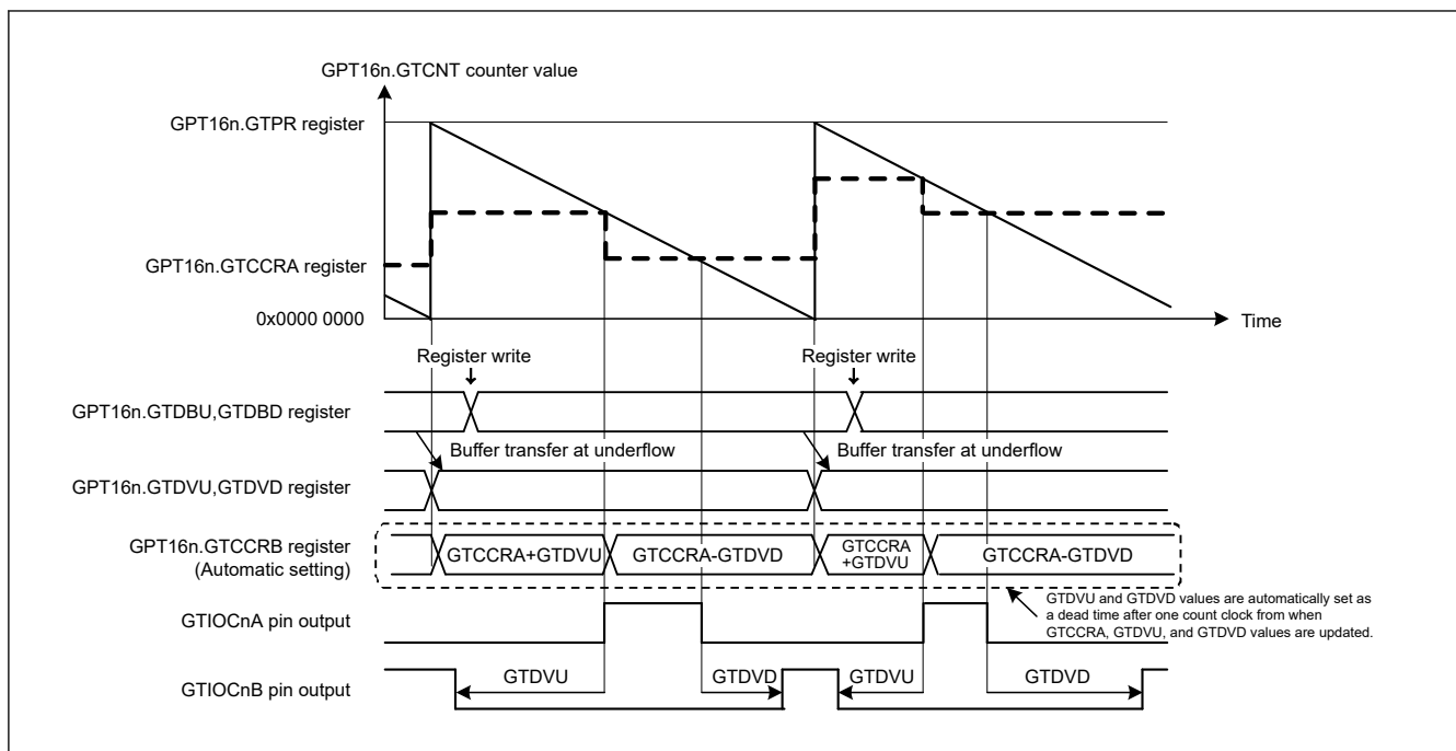
Figure 20.81 Example of automatic dead time setting function operation in saw-wave one-shot pulse mode, down-counting, GTDVU and GTDVD set to buffer operation, and active-high in GPT160 to GPT162
