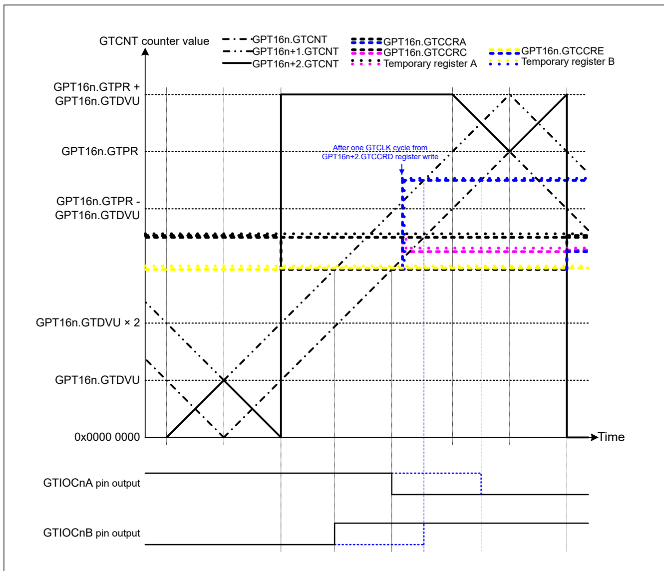
Figure 20.76 Example of complementary PWM mode 4 double buffer operation (up-counting middle section) (complementary PWM mode 4 double buffer operation, GTIOcNA pin = low/GTIOcNB pin = high at GTCCRA register compare match during up-counting, GTIOcNA pin = high/GTIOcNB pin = low at GTCCR register compare match during down-counting, when a value is written to GTCCR register after up-counting compare match) ( n = 0 )
