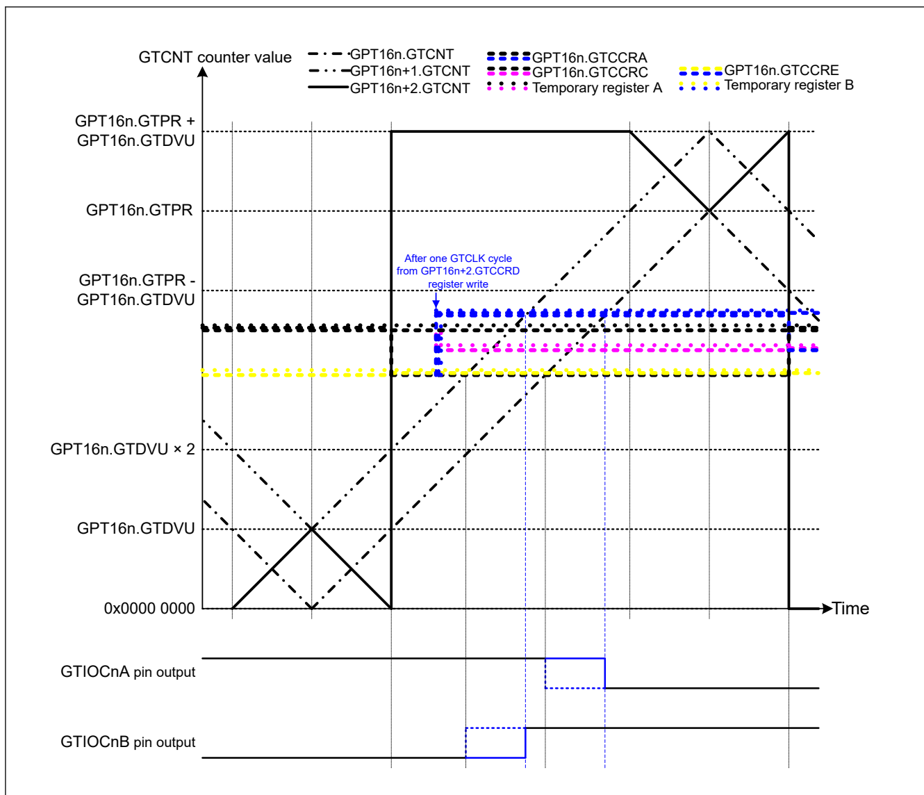
Figure 20.75 Example of complementary PWM mode 4 double buffer operation (up-counting middle section) (complementary PWM mode 4 double buffer operation, GTIOCnA pin = low/GTIOCnB pin = high at GTCCRA register compare match during up-counting, GTIOCnA pin = high/GTIOCnB pin = low at GTCCRA register compare match during down-counting, when a value larger than the GPT16n+1.GTCNT value is written to GTCCRF register before up-counting compare match) (n = 0)
