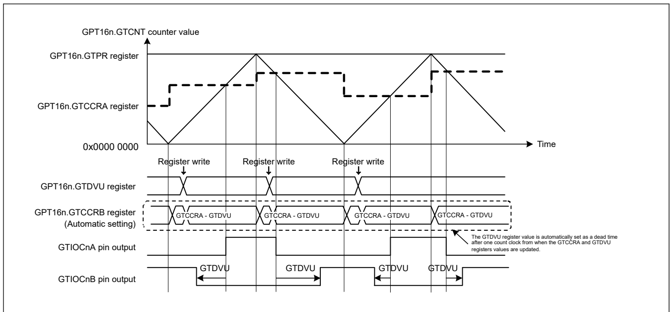
Figure 20.86 Example of automatic compare-match value setting function with dead time in triangle-wave PWM mode 2 or 3 and active-high in GPT163
