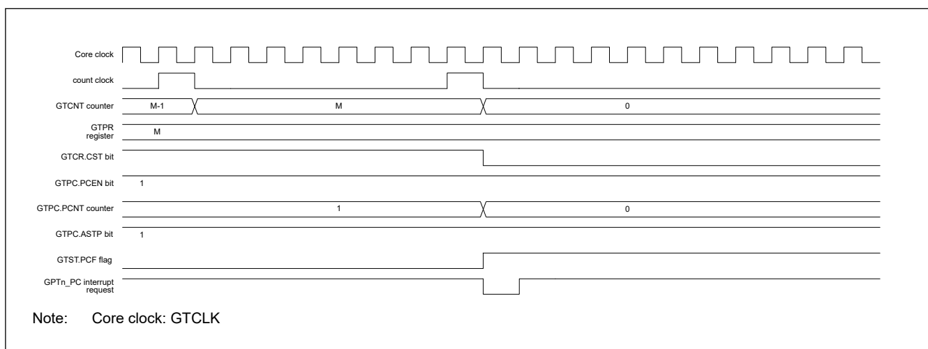
Figure 20.122 Example of the timing of operations for PWM cycle count function (saw-wave one-shot pulse mode, up-counting)
