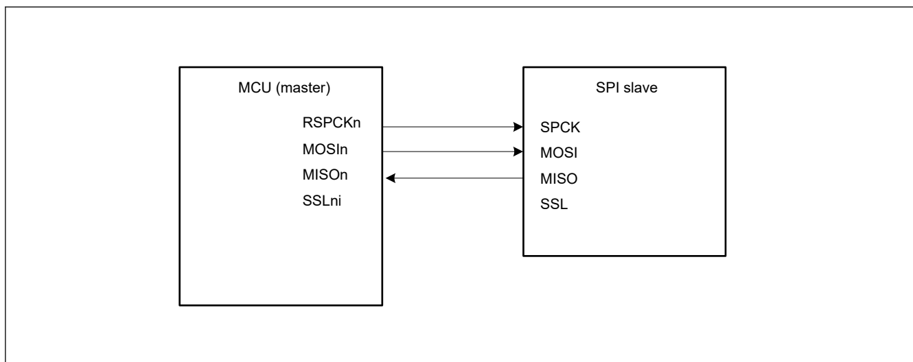
Figure 26.10 Clock synchronous master/slave configuration example with the MCU as a master
