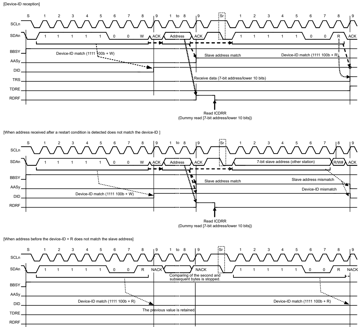
Figure 25.28 AASy and DID flag set and clear timing during reception of device ID
