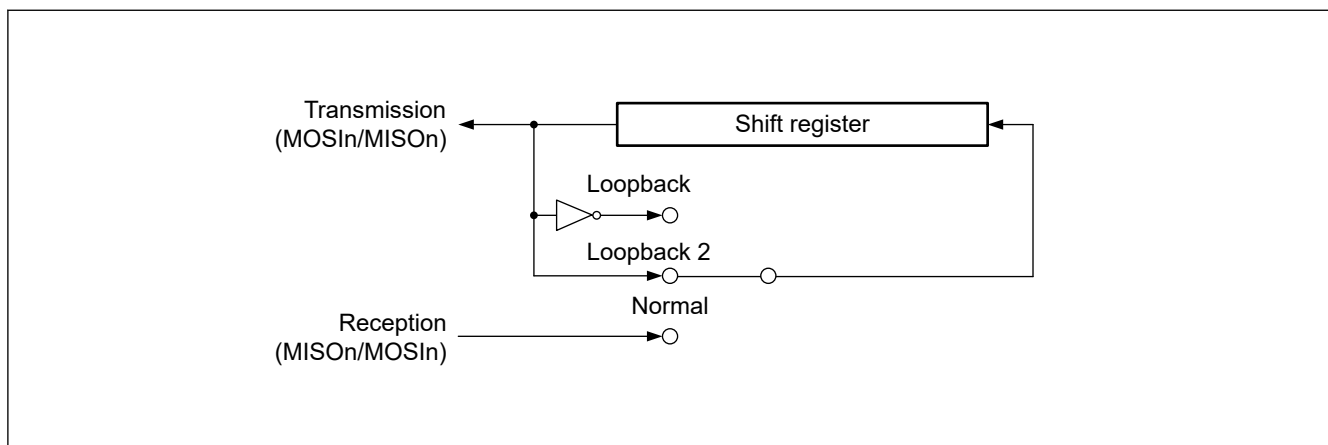
Figure 26.41 Configuration of shift register I/O paths in loopback mode for master mode
