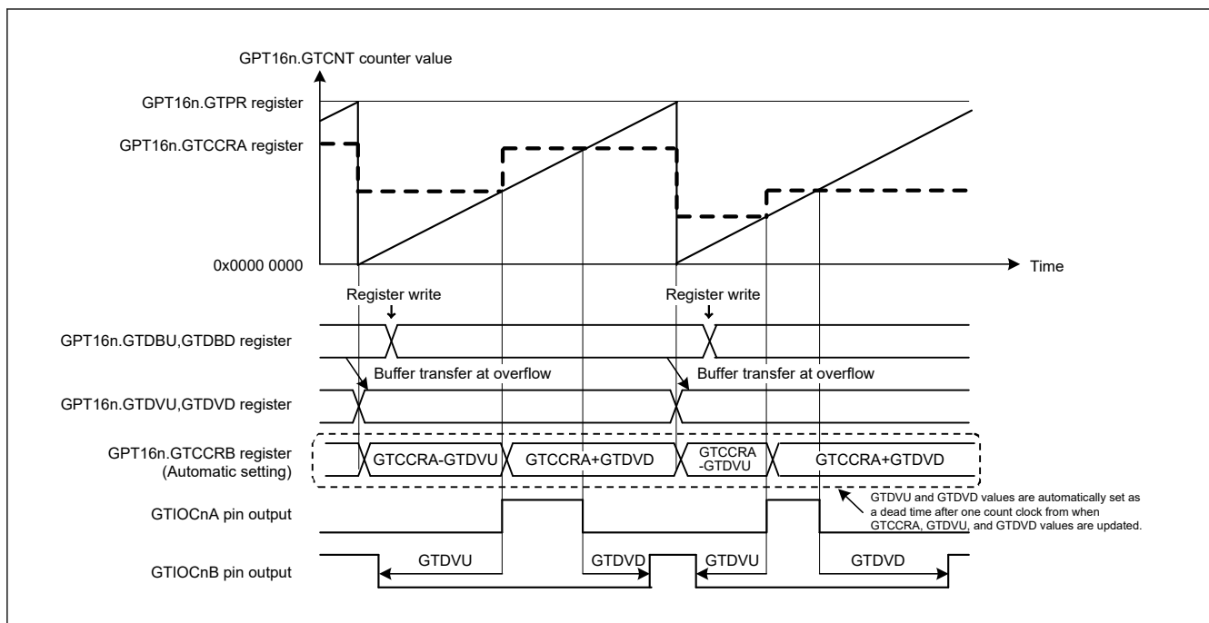
Figure 20.79 Example of automatic dead time setting function operation in saw-wave one-shot pulse mode, up-counting, GTDVU and GTDVD set to buffer operation, and active-high in GPT160 to GPT162
