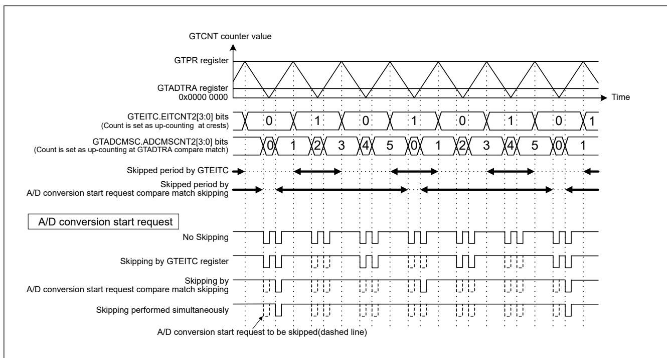
Figure 20.157 Example of A/D conversion start request compare match skipping function operation (extended interrupt skipping: EIVTC2[1:0] = 01b, EADTAL[2:0] = 010b, A/D conversion start request compare match skipping: ADCMSC2[1:0] = 01b, ADCMSAL[2:0] = 010b)
