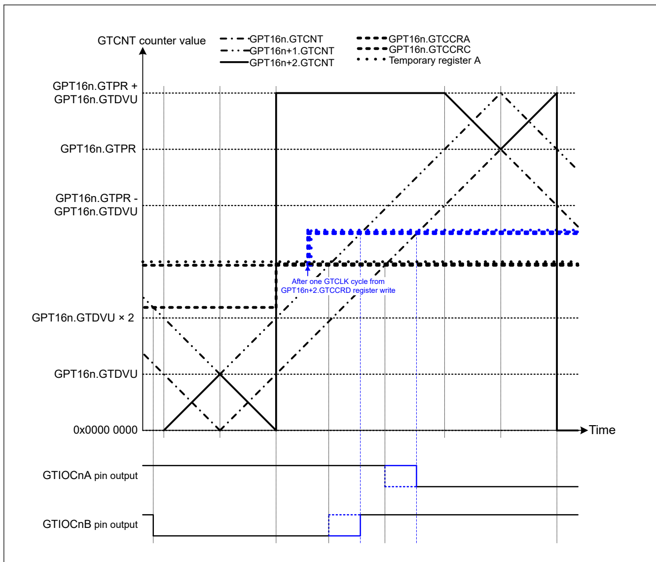
Figure 20.70 Example of complementary PWM mode 4 single buffer operation (up-counting middle section) (complementary PWM mode 4 single buffer operation, GTIOCnA pin = low/GTIOCnB pin = high at GTCCRA register compare match during up-counting, GTIOCnA pin = high/GTIOCnB pin = low at GTCCRA register compare match during down-counting, when a value larger than the GPT16n+1.GTCNT value is written to GTCCRD register before up-counting compare match) ( n = 0 )
