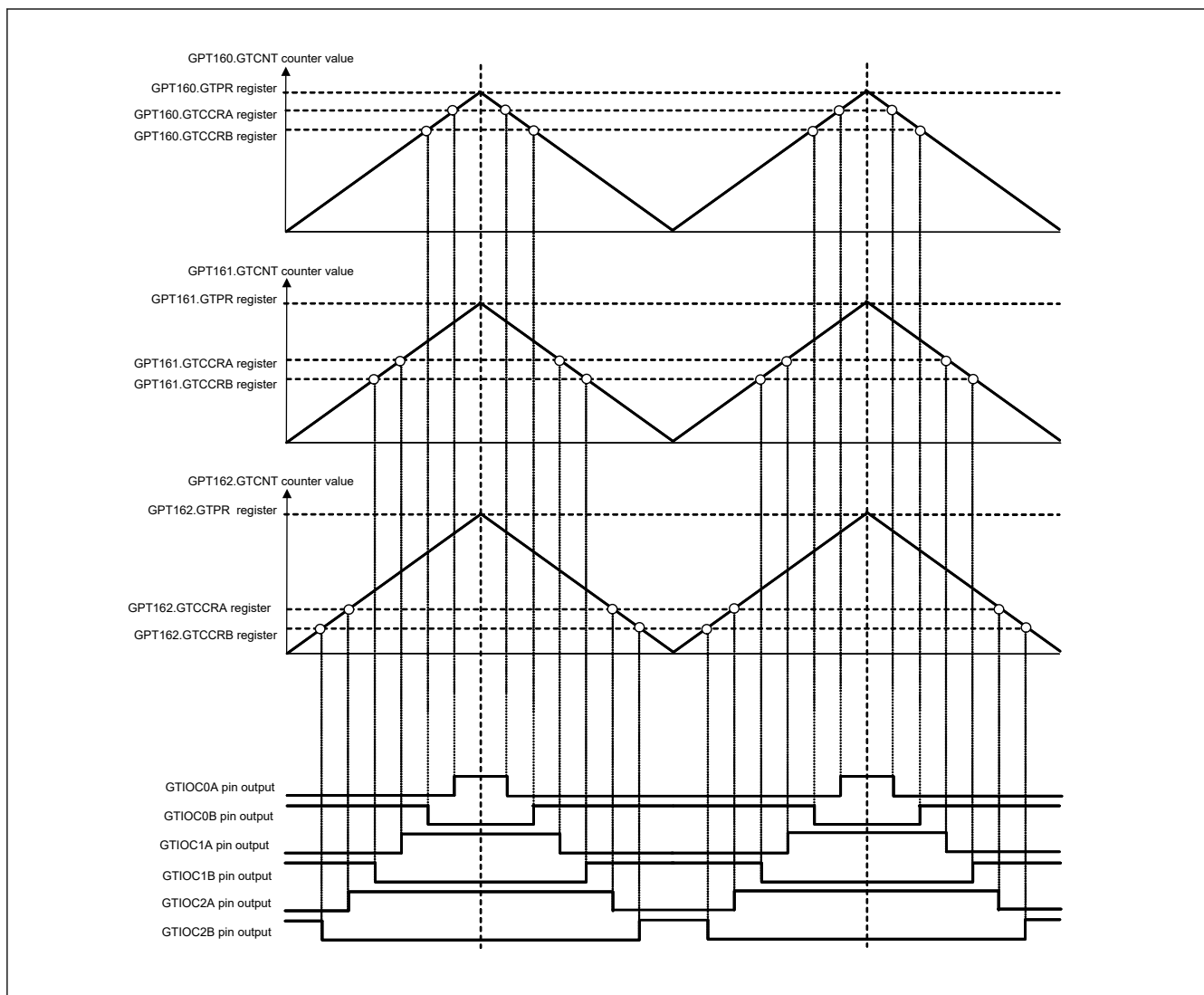
Figure 20.118 Example of 3-phase triangle-wave complementary PWM output
