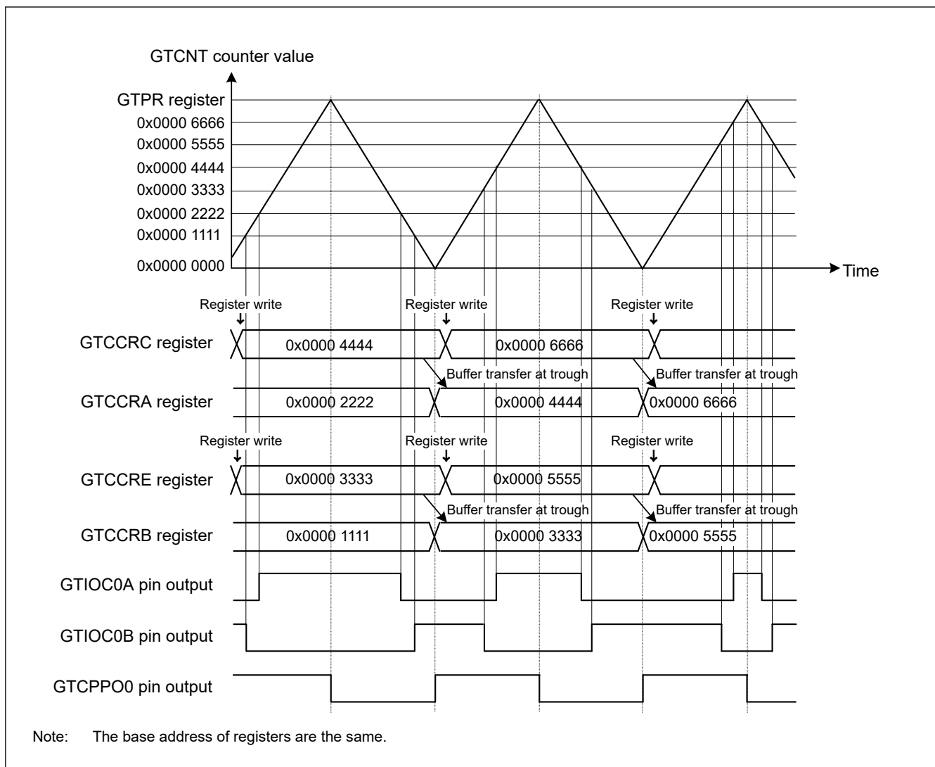
Figure 20.43 Example of triangle-wave PWM mode 1 operation with buffer operation, low output from the GTIOCnA pin and high output from the GTIOCnB pin at count start, output toggled at GTCCRA/ GTCCRB register compare match, output retained at cycle end, and GTIOR.PSYE = 1
