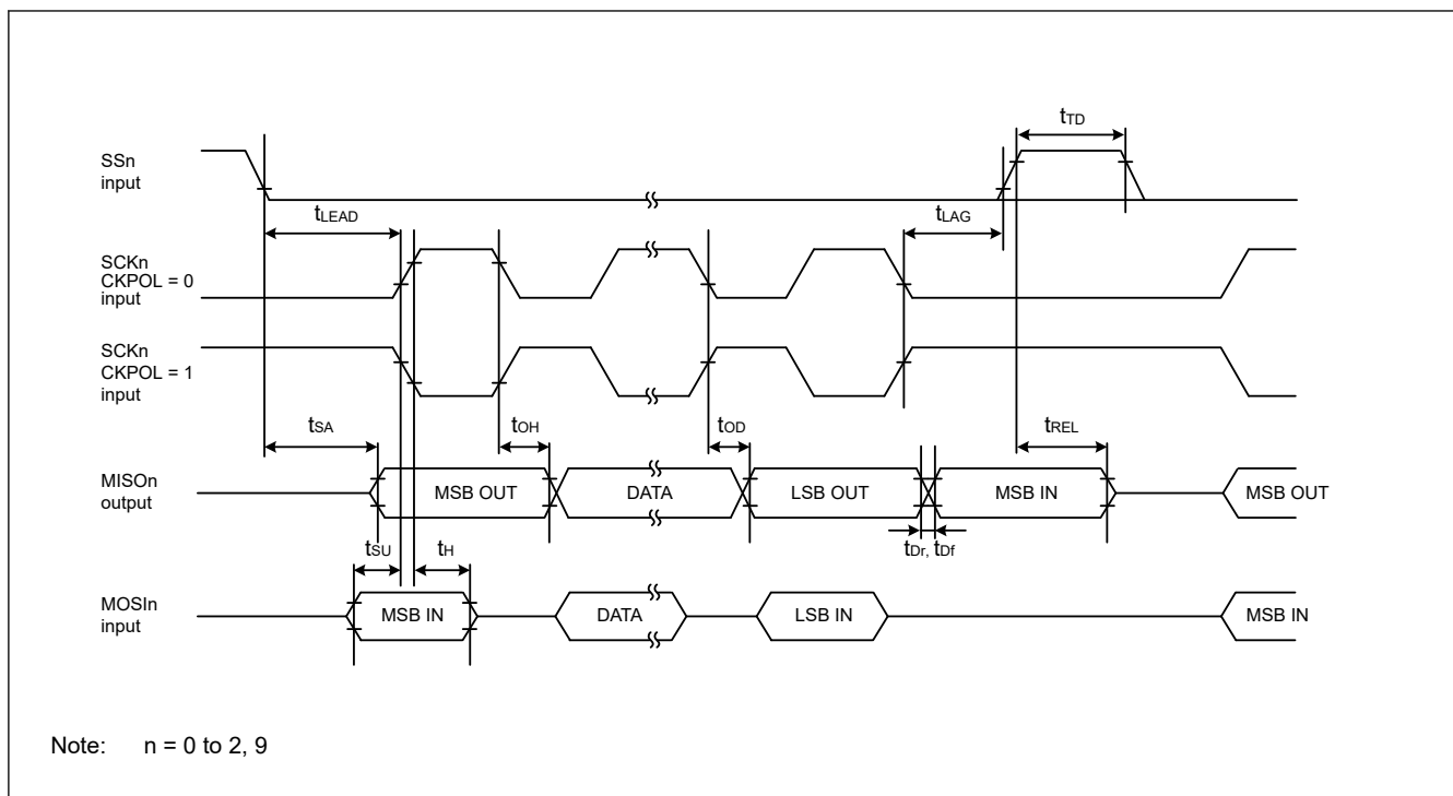
Figure 35.36 SCI simple SPI mode timing (slave, CKPH = 1)
