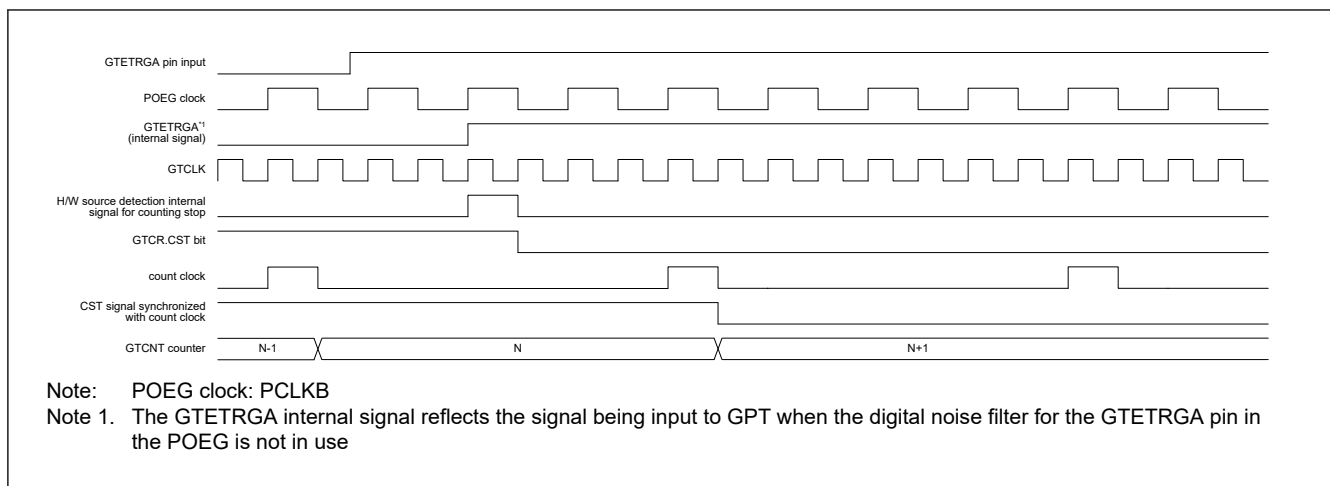
Figure 20.95 Example of timing of operations to stop counting in response to a rising edge of the input on the GTETRG pin
