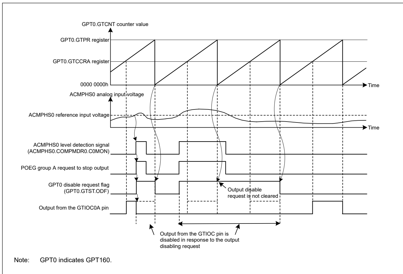
Figure 19.4 Example of Operation to Stop Output from the GTIOC Pin In Response to Level Detection by a Comparator
