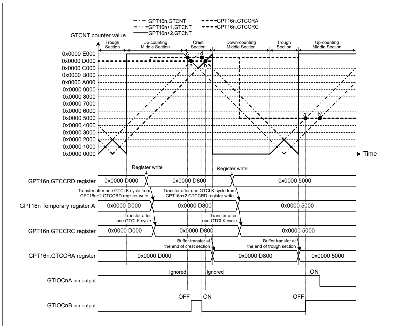
Figure 20.59 Example of compare match generation sequence operation in complementary PWM mode (complementary PWM mode 3 single buffer operation, GTIOCnA pin = low/GTIOCnB pin = high at GTCCRA register compare match during up-counting, GTIOCnA pin = high/GTIOCnB pin = low at GTCCRA register compare match during down-counting, the dead time value is 0x0000 2000, compare match generation order: c → a → d → b) (n = 0)
