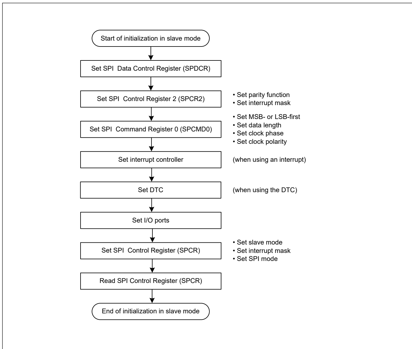
Figure 26.40 Example of initialization flow in slave mode for clock synchronous operation
