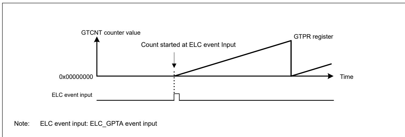
Figure 20.89 Example of count start operation by a hardware source started at the input of the signal from the ELC_GPTA event
