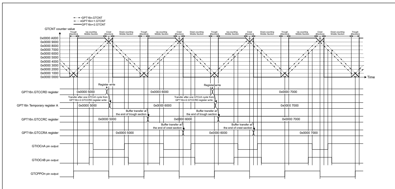
Figure 20.48 Example of complementary PWM mode 1 operation (GTIOCnA pin = low/GTIOCnB pin = high at GTCCRA register compare match during up-counting, GTIOCnA pin = high/GTIOCnB pin = low at GTCCRA register compare match during down-counting, the dead time value is 0x0000 1000 and updating GTCCRD register in crest and trough sections) (n = 0)
