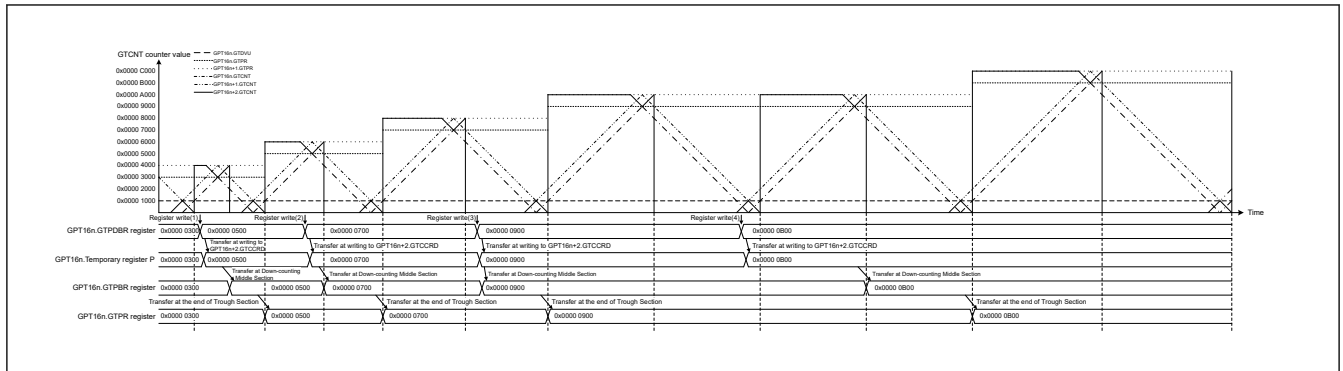
Figure 20.22 Example of GTPR double buffer operation with complementary PWM mode 2
