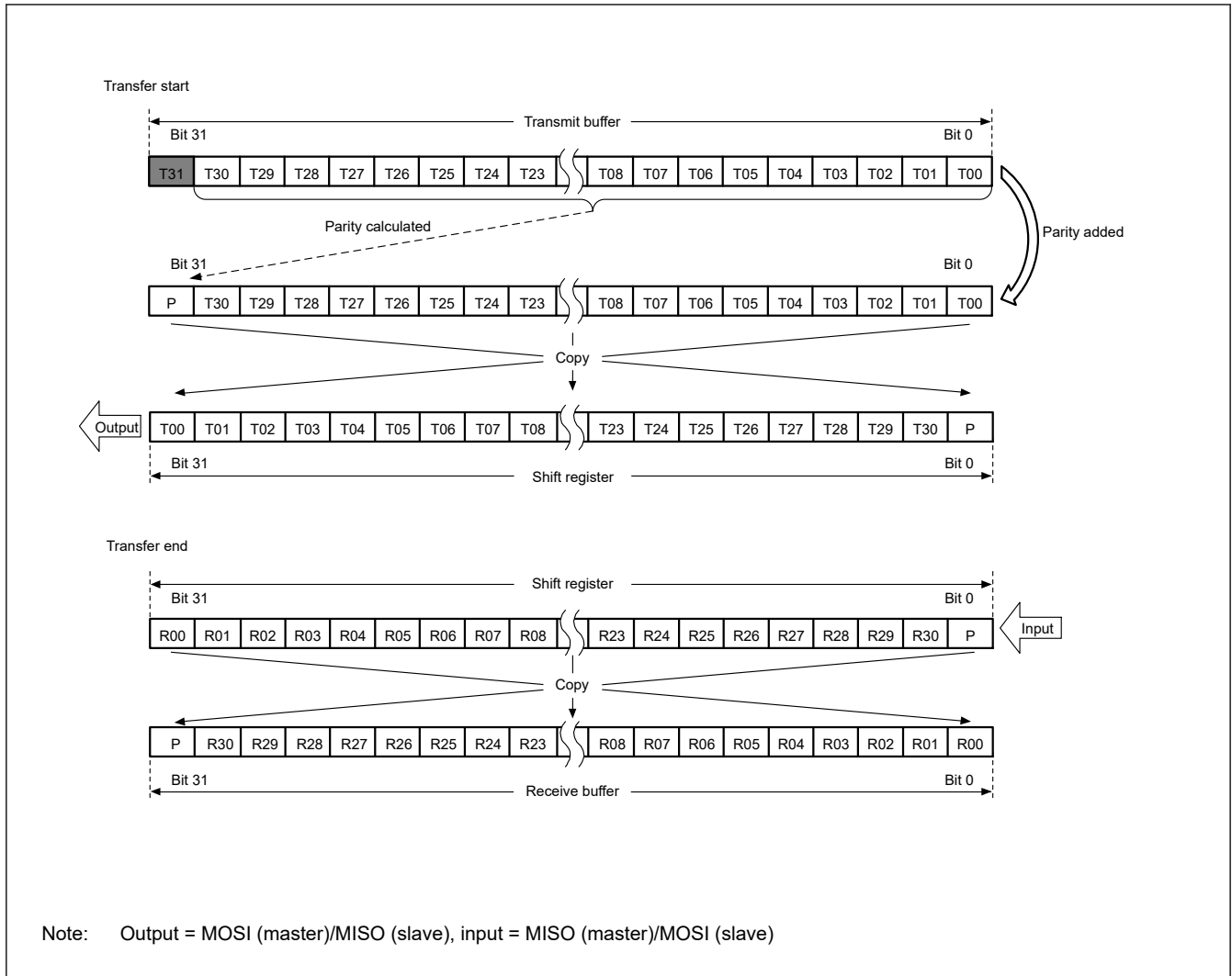
Figure 26.19 LSB-first transfer with 32-bit data and parity enabled
