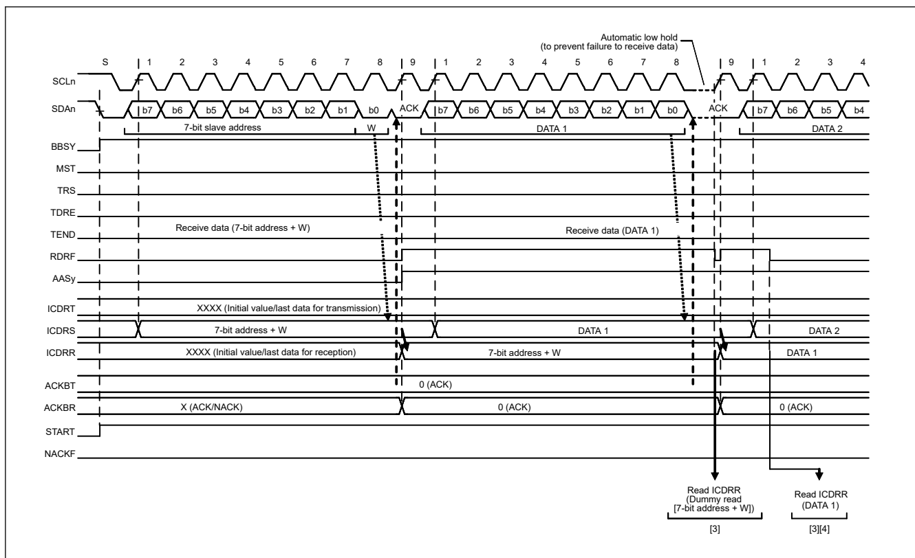
Figure 25.19 Slave receive operation timing (1) with 7-bit address format when RDRFS = 0
