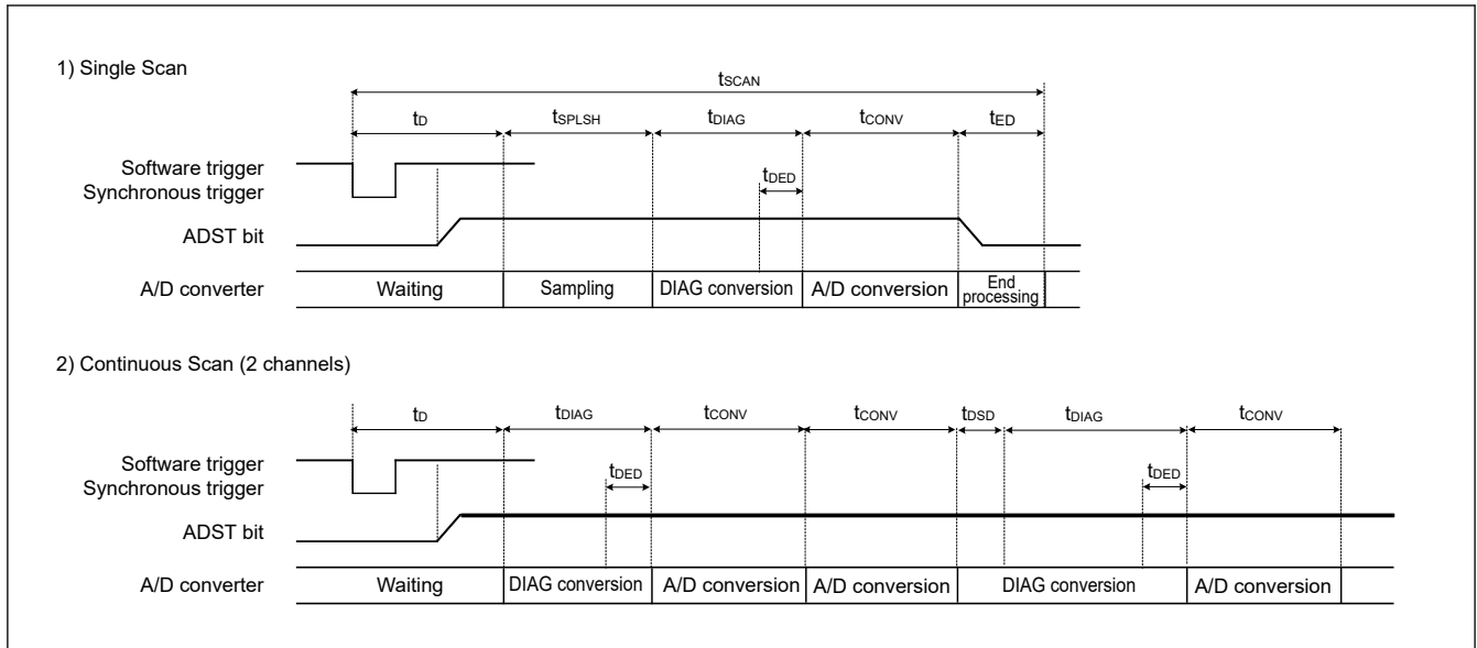
Figure 29.29 Scan conversion timing when activated by software or a synchronous trigger input (ELC)
