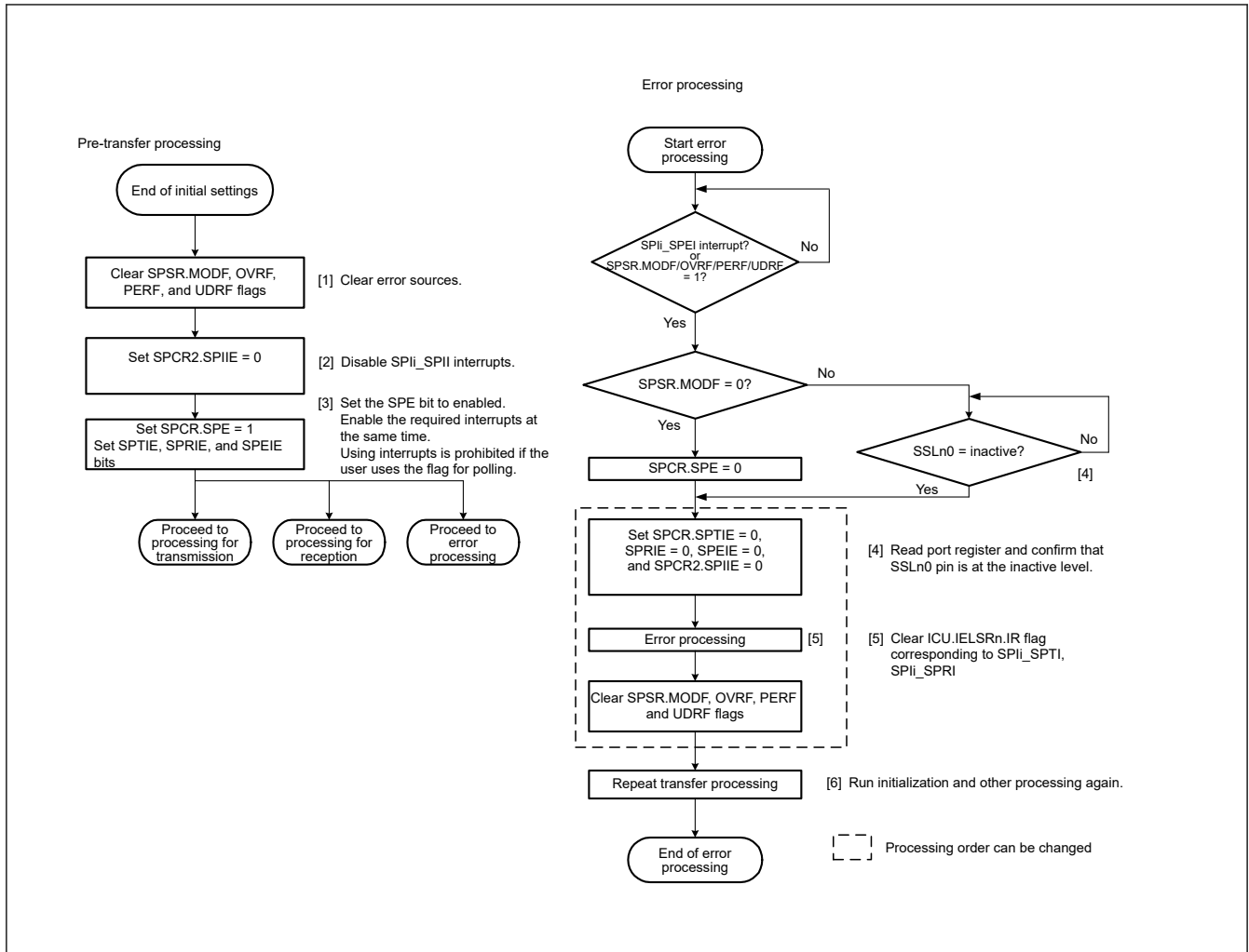
Figure 26.34 Error processing flow in master mode
