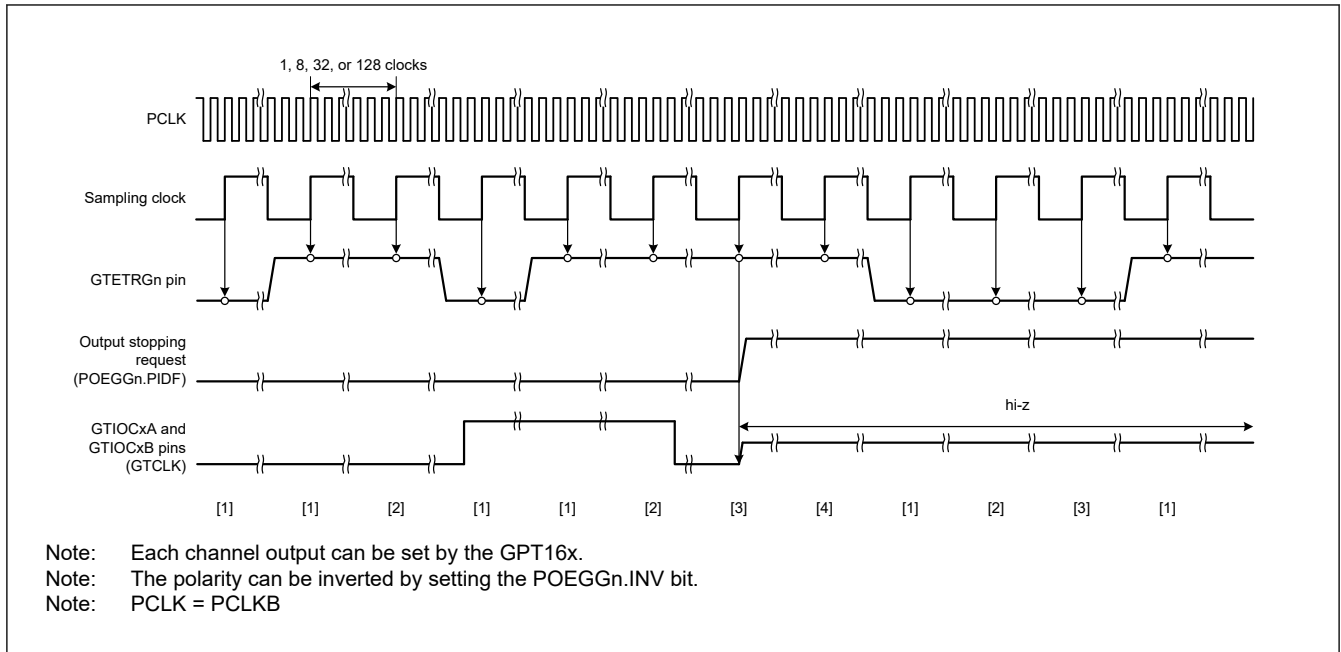
Figure 19.2 Example for Operation of Digital Noise Filter
