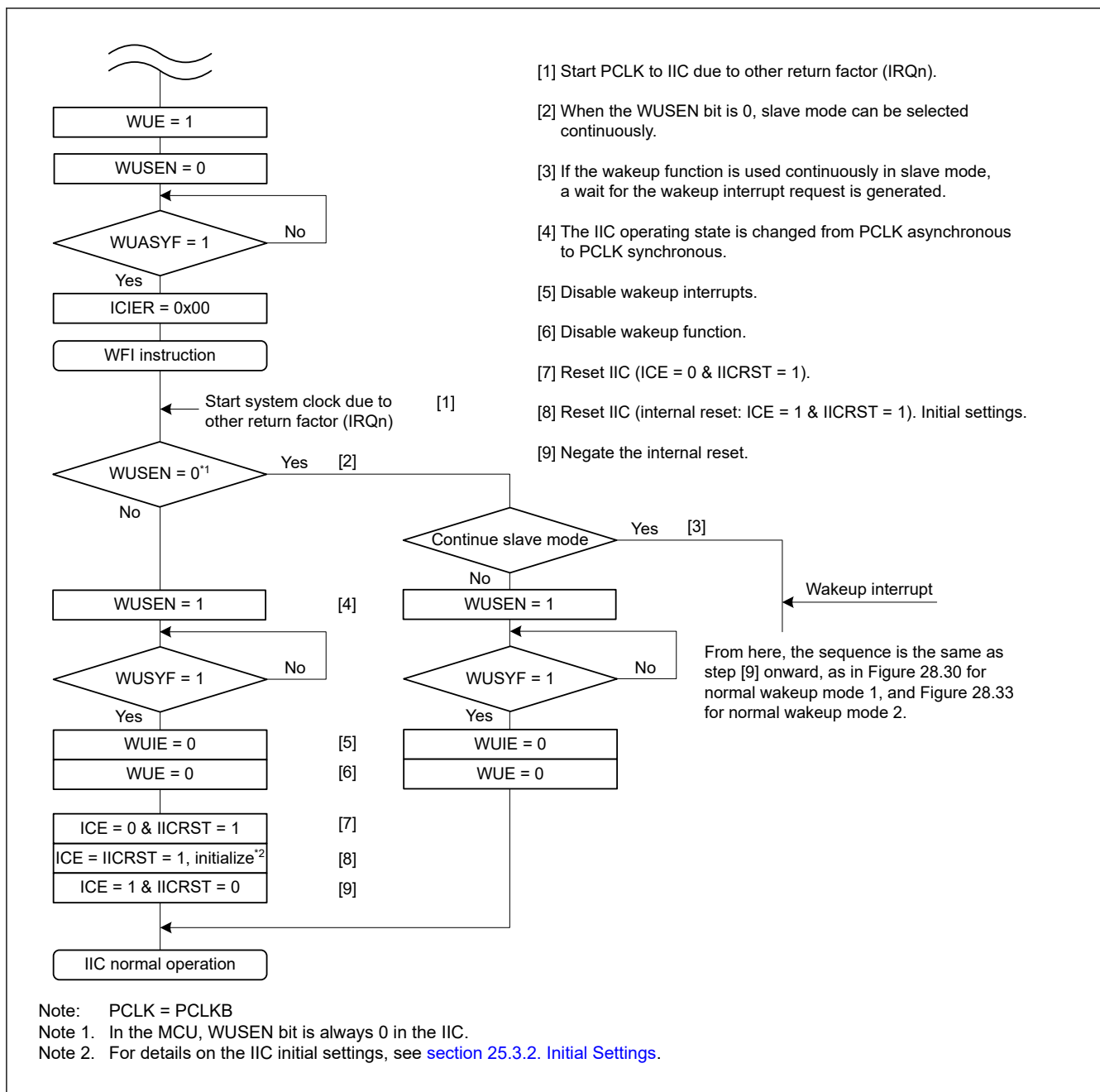
Figure 25.31 Example operation of normal wakeup modes 1 and 2 when wakeup is triggered by an interrupt other than IIC wakeup interrupt, for example, the IRQn
