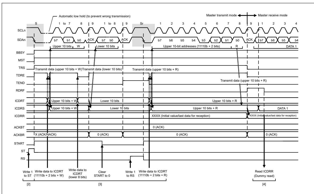
Figure 25.13 Master receive operation timing (2) with 10-bit address format when RDRFS = 0
