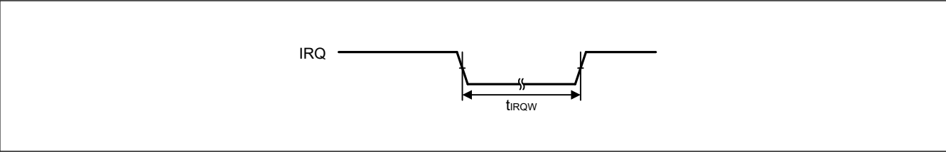
Figure 35.12 IRQ interrupt input timing
