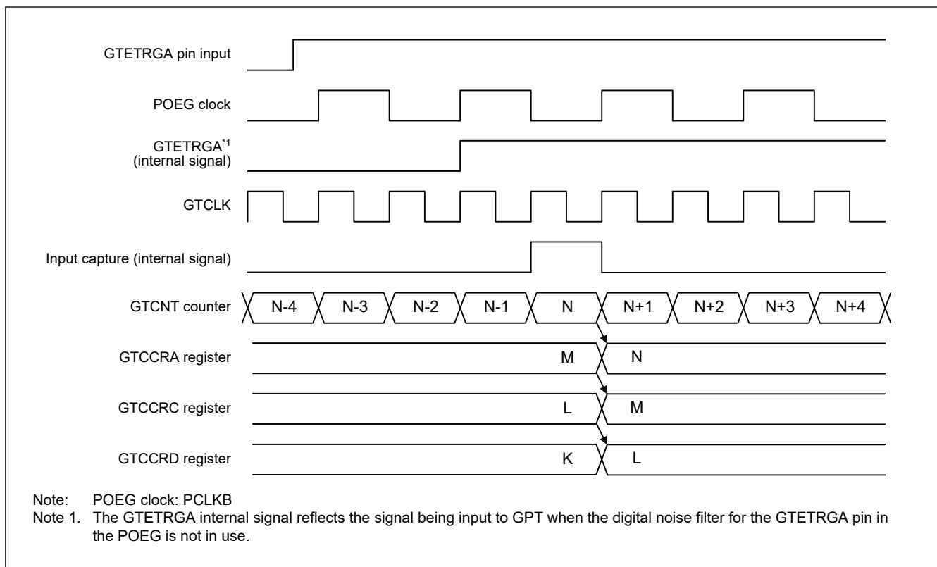
Figure 20.14 Example of the timing of input capture operation in response to a rising edge of the input on the GTETRGA pin
