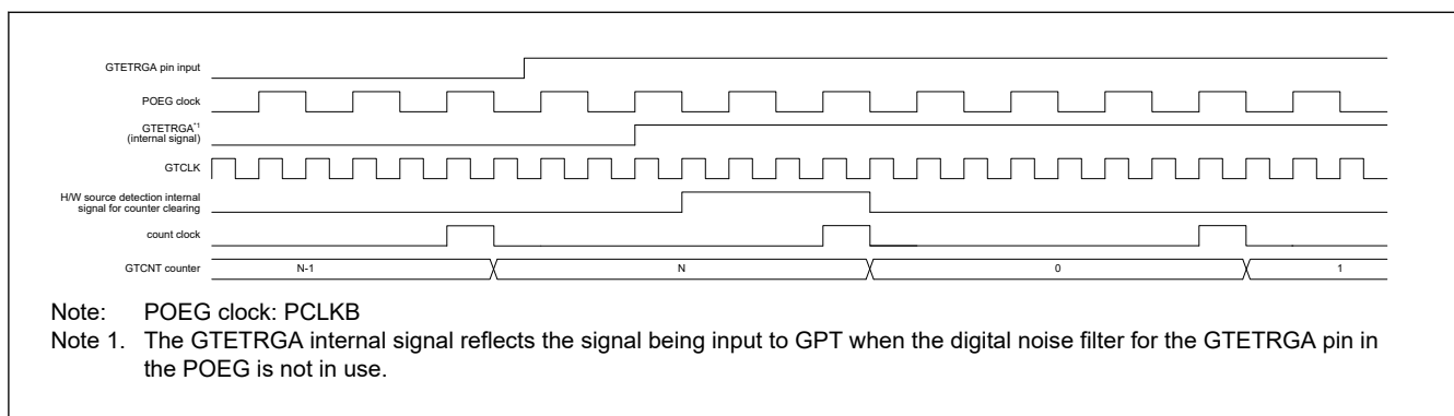
Figure 20.101 Examples of the timing of operations for counter clearing in response to a rising edge of the input on the GTETRGA pin (during the counting of cycles of clock signal produced by dividing the GTCLK frequency)
