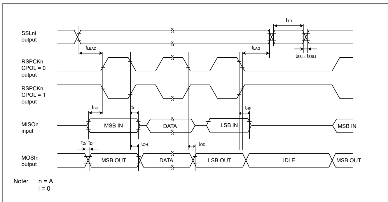
Figure 35.41 SPI timing (master, CPHA = 0) (bit rate: PCLKB division ratio is set to 1/2)
