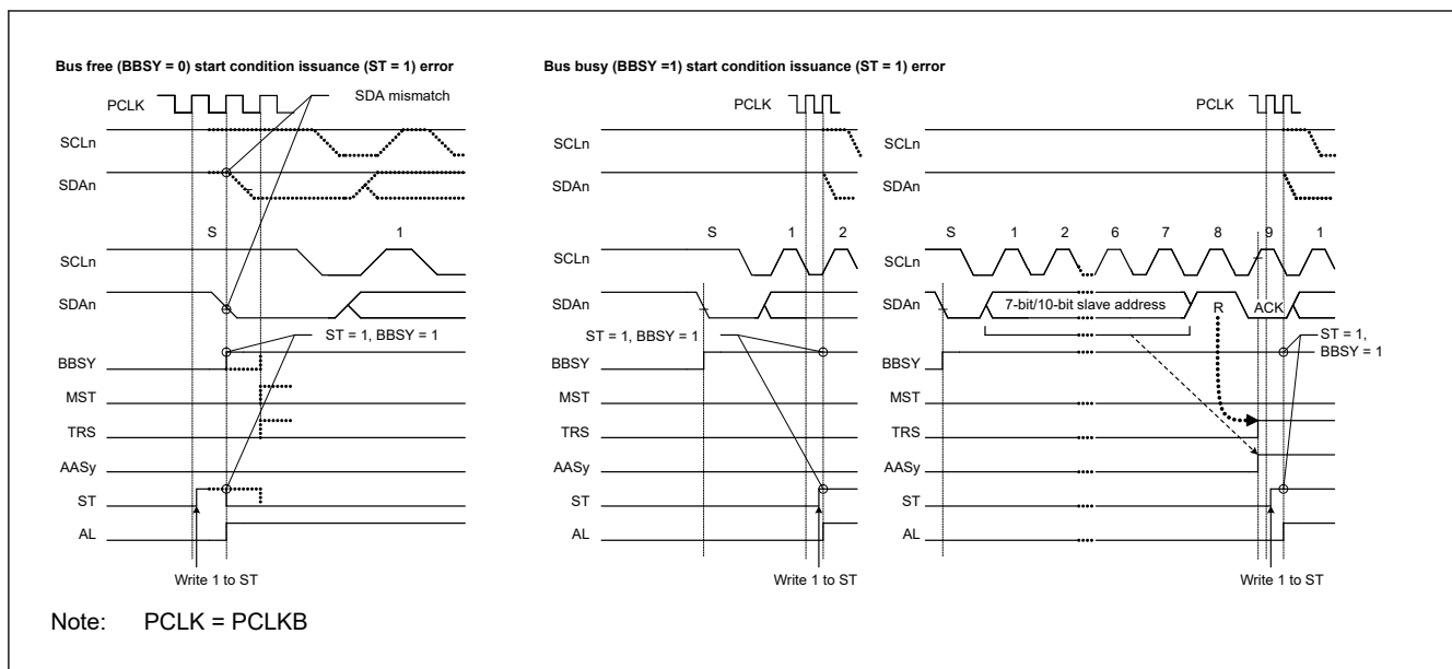
Figure 25.42 Arbitration-lost when start condition is issued when MALE = 1
