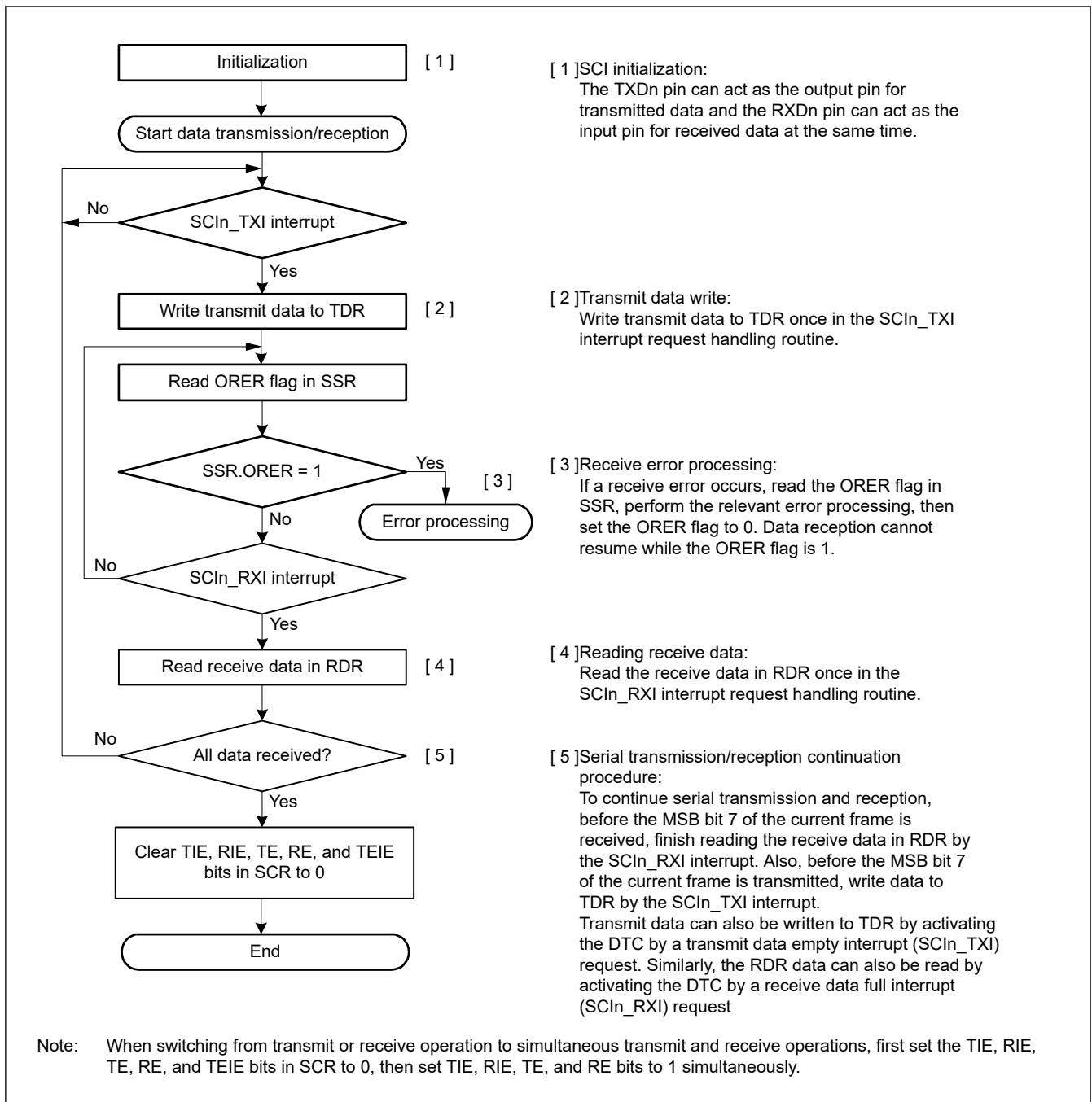
Figure 24.45 Example flow of simultaneous serial transmission and reception in clock synchronous mode with non-FIFO selected
