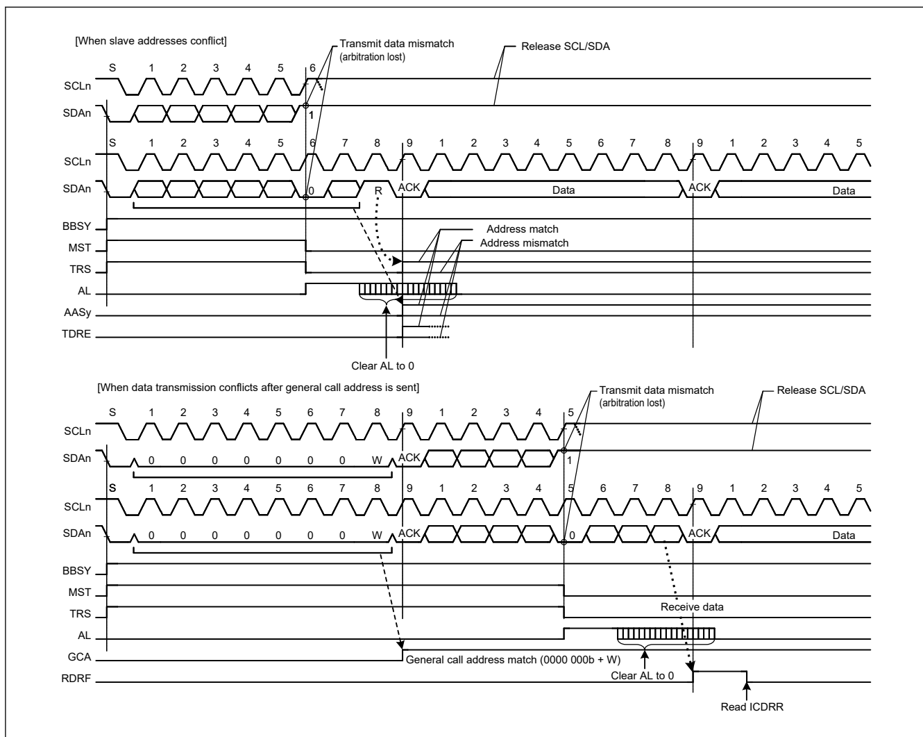
Figure 25.41 Examples of master arbitration-lost detection when MALE = 1
