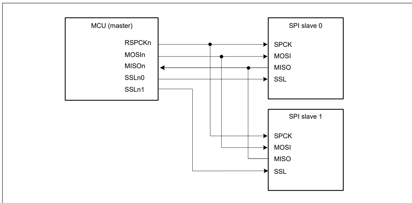
Figure 26.8 Single-master/multi-slave configuration example with the MCU as a master
