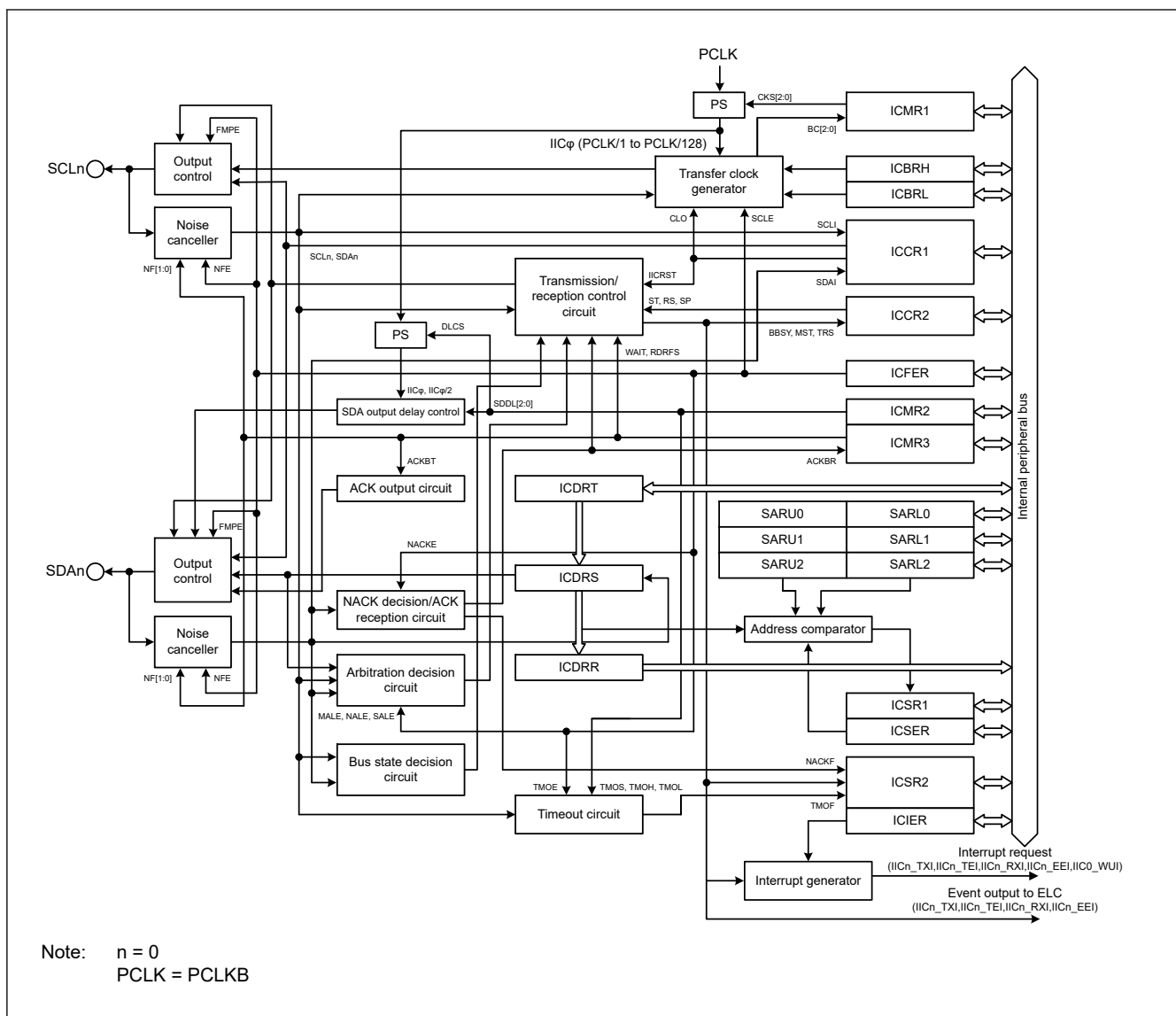
Figure 25.1 IIC block diagram
