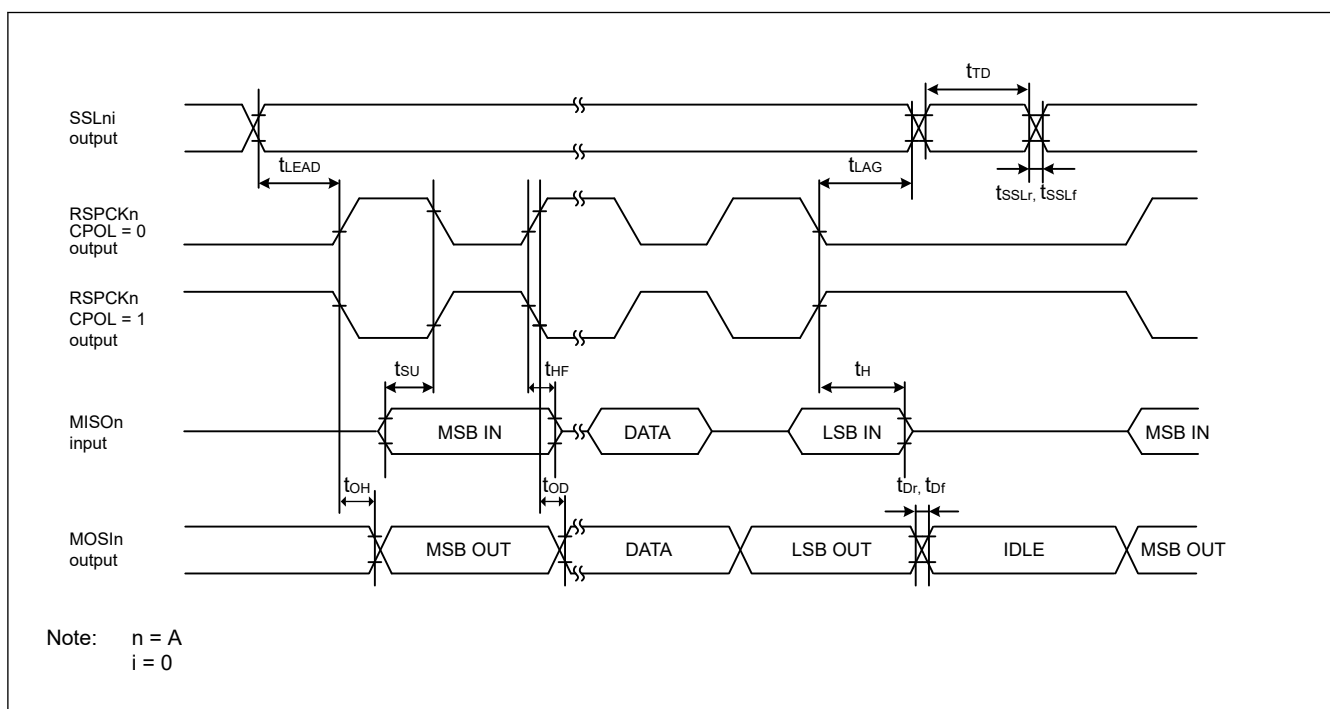
Figure 35.43 SPI timing (master, CPHA = 1) (bit rate: PCLKB division ratio is set to 1/2)
