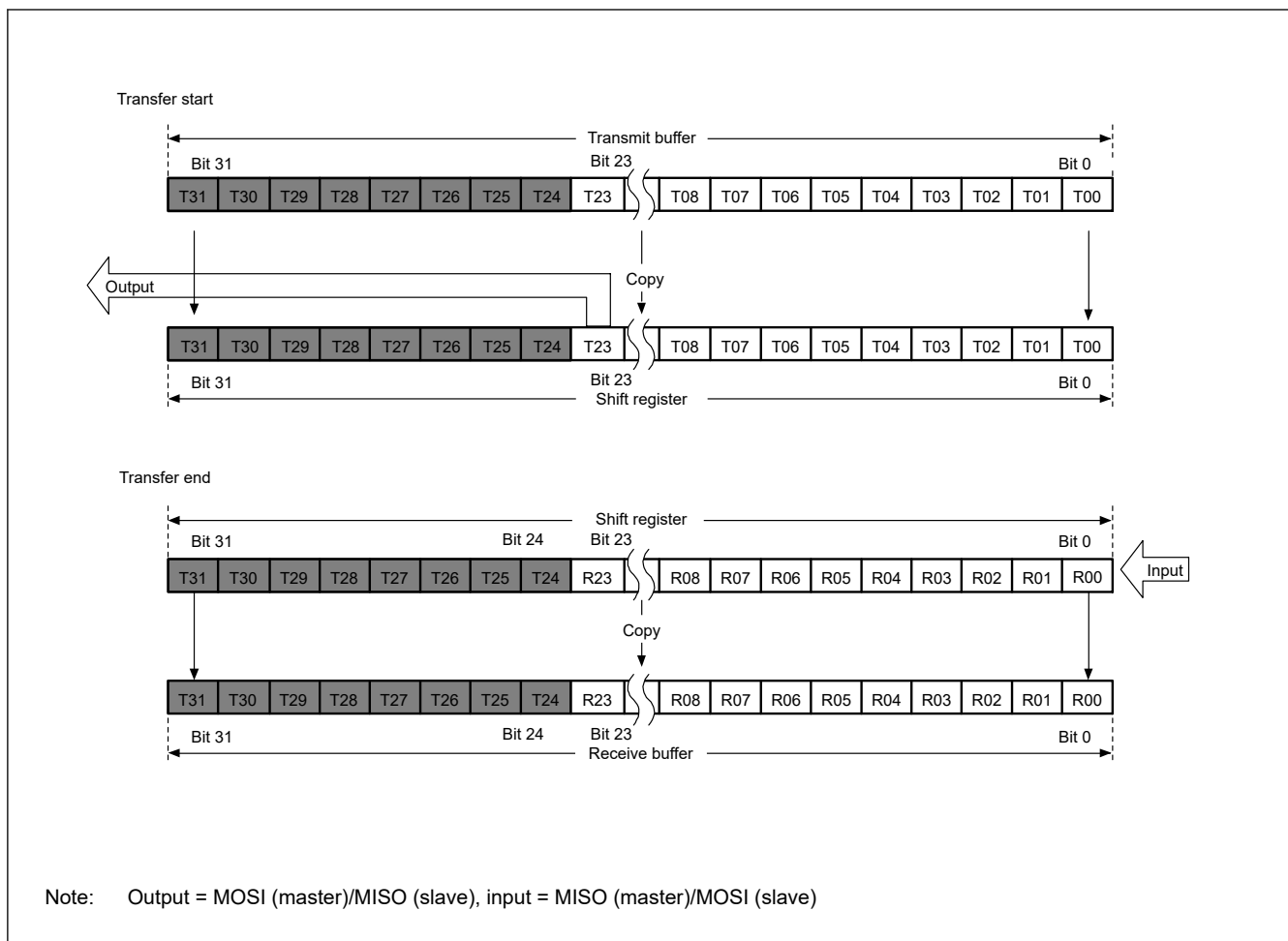
Figure 26.14 MSB-first transfer with 24-bit data and parity disabled
