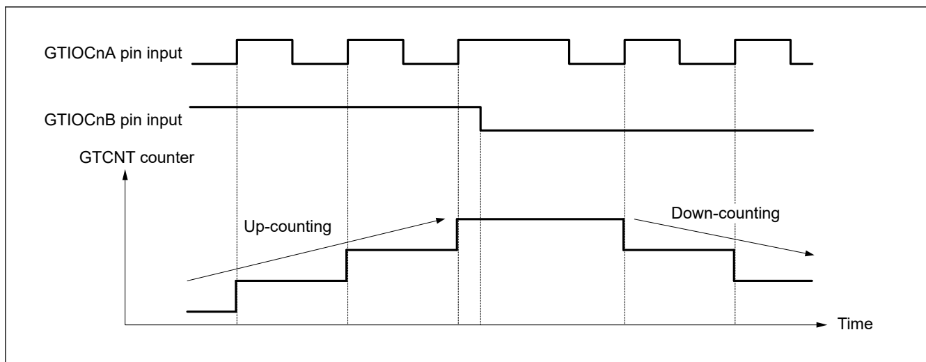
Figure 20.125 Example of phase counting mode 2 (B)
