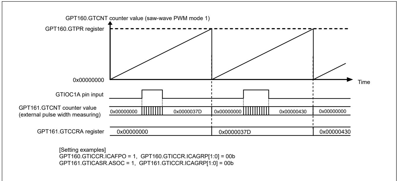
Figure 20.114 Example of input capture operation by inter channel cooperation (channel 1 is captured by the overflow of channel 0)
