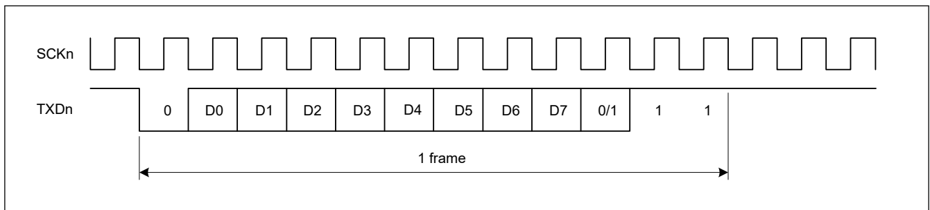
Figure 24.4 Phase relationship between output clock and transmit data in asynchronous mode when SMR.CHR = 0, PE = 1, MP = 0, and STOP = 1
