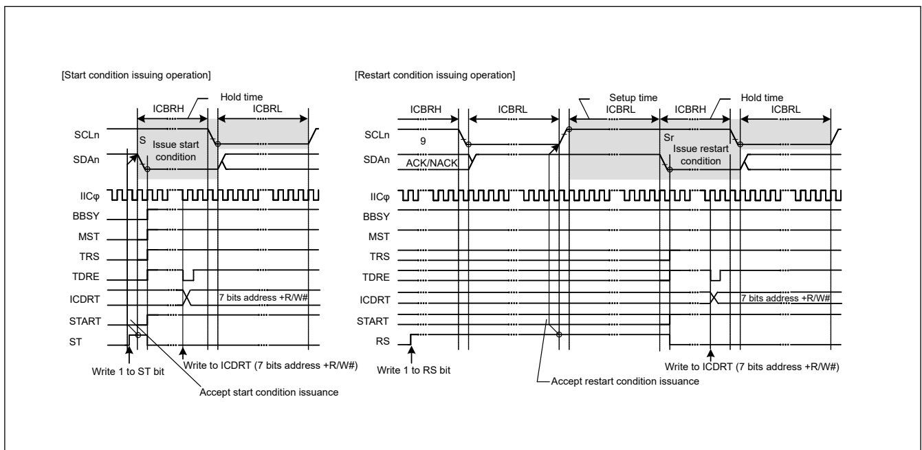
Figure 25.45 Start and restart condition issue timing using the ST and RS bits
