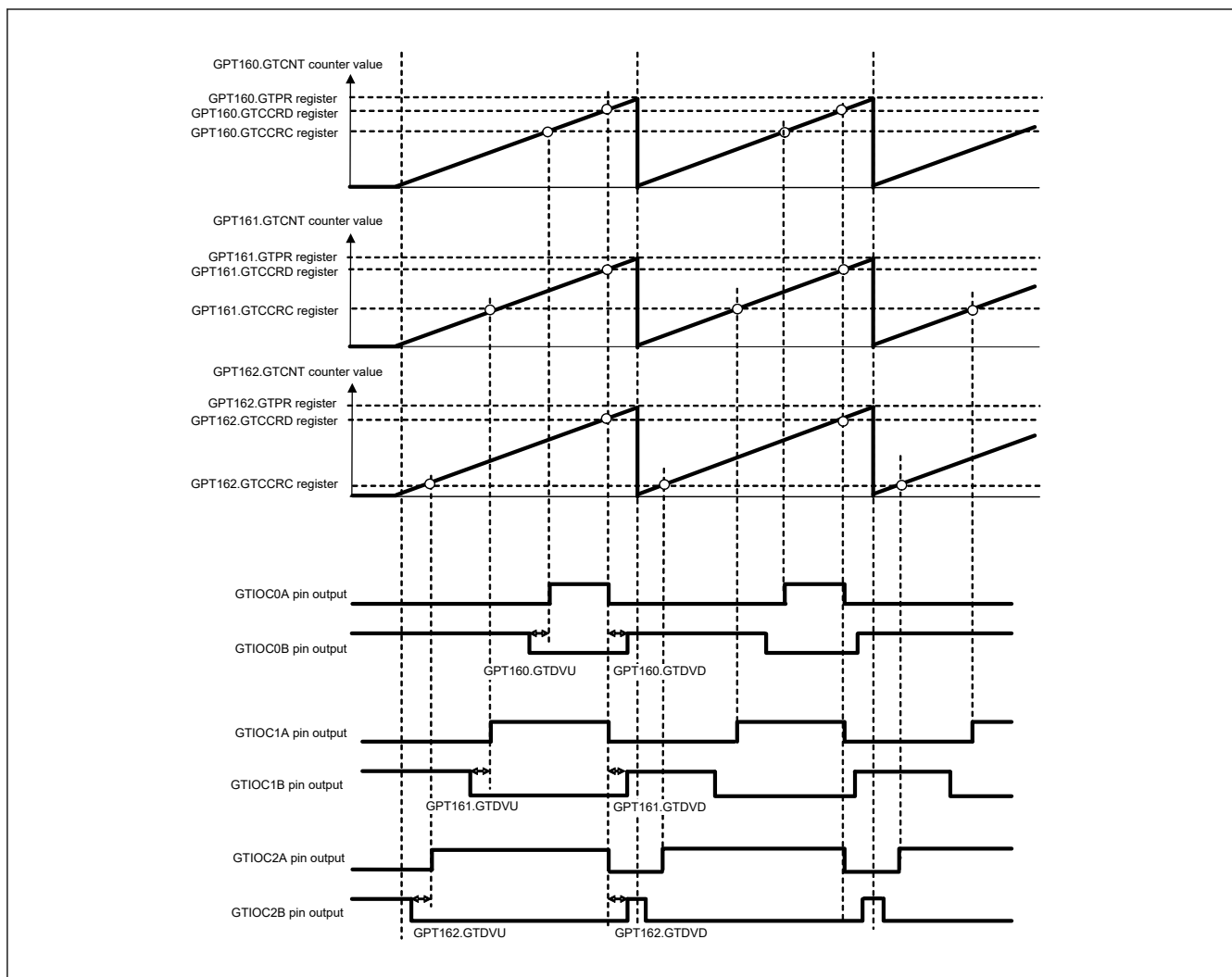
Figure 20.117 Example of 3-phase saw-wave complementary PWM output with automatic dead time setting
