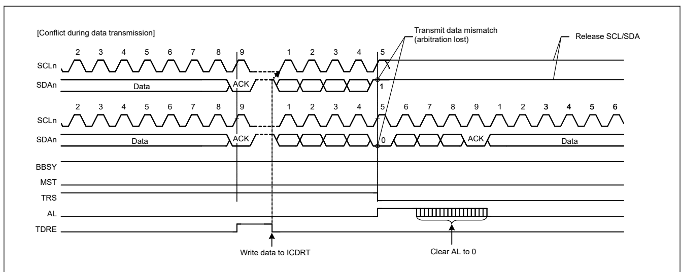
Figure 25.44 Example of slave arbitration-lost detection when SALE = 1
