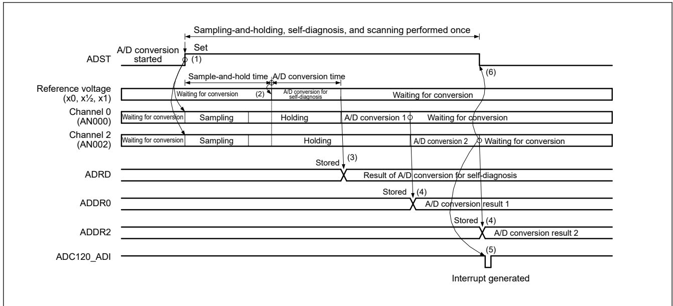
Figure 29.10 Example operation in single scan mode when channel-dedicated sample-and-hold circuits are used, AN000 and AN002 are selected with self-diagnosis
