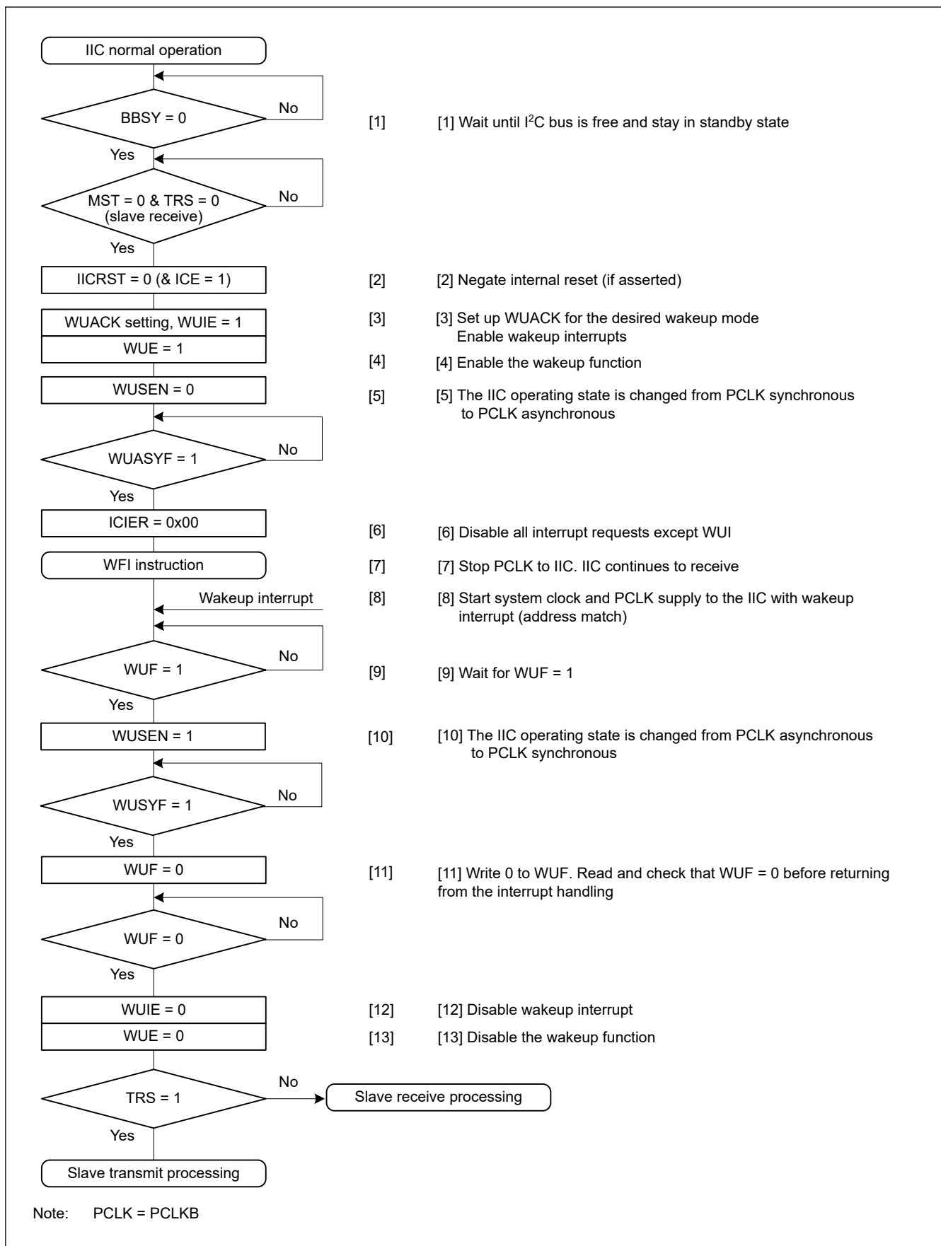
Figure 25.33 Example operation of normal wakeup mode 2 when wakeup is triggered by a wakeup interrupt on match of the slave address
