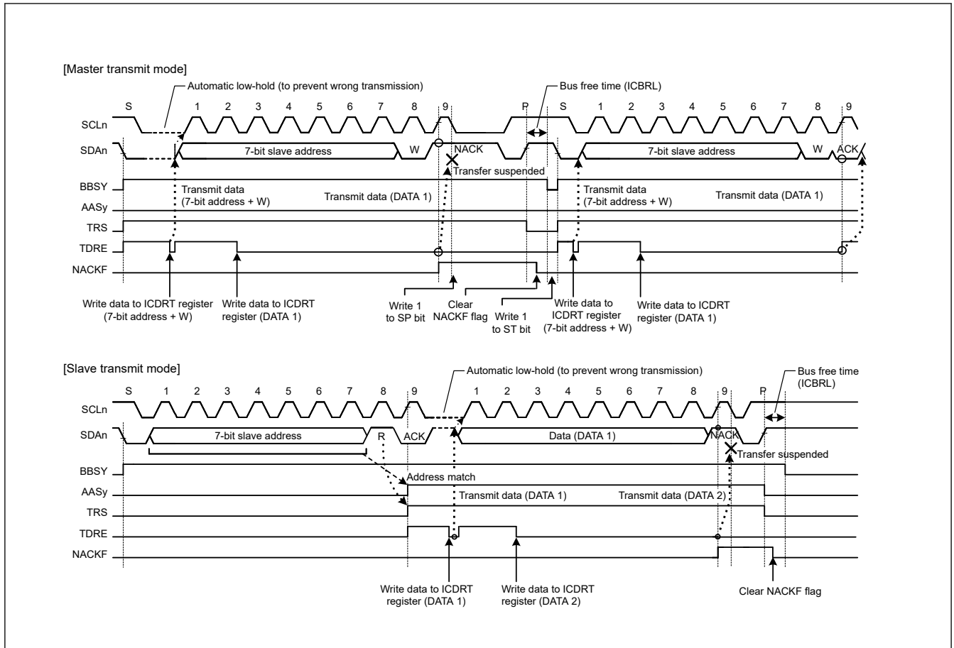
Figure 25.39 Suspension of data transfer when NACK is received, when NACK = 1
