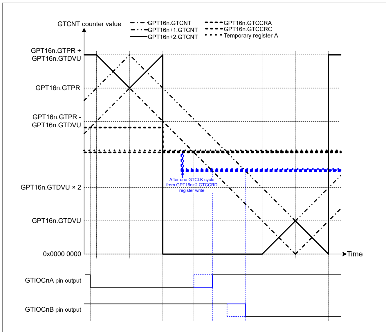
Figure 20.73 Example of complementary PWM mode 4 single buffer operation (down-counting middle section) (complementary PWM mode 4 single buffer operation, GTIOCnA pin = low/GTIOCnB pin = high at GTCCRA register compare match during up-counting, GTIOCnA pin = high/GTIOCnB pin = low at GTCCRA register compare match during down-counting, when a value smaller than the GPT16n.GTCNT value is written to GTCCRD register before down-counting compare match) ( n = 0 )
