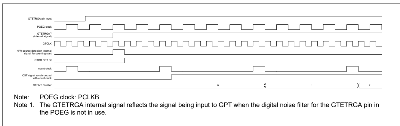
Figure 20.90 Example of timing of operations to start counting in response to a rising edge of the input on the GTETRGA pin
