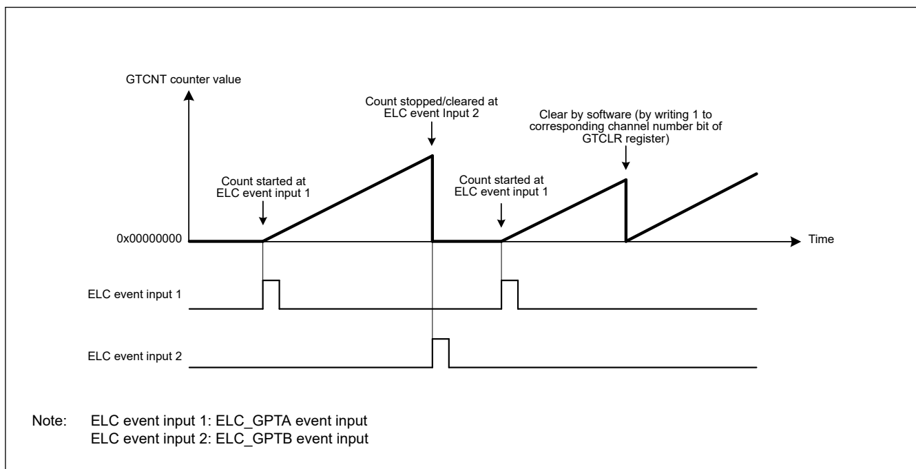
Figure 20.98 Examples of count clearing operation by hardware source in saw wave up-counting, started at ELC_GPTA input, and stopped/cleared at ELC_GPTB input
