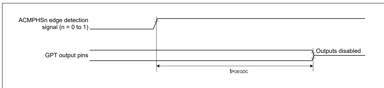
Figure 35.17 Output disable time for POEG in response to edge detection signal from ACMPHS
