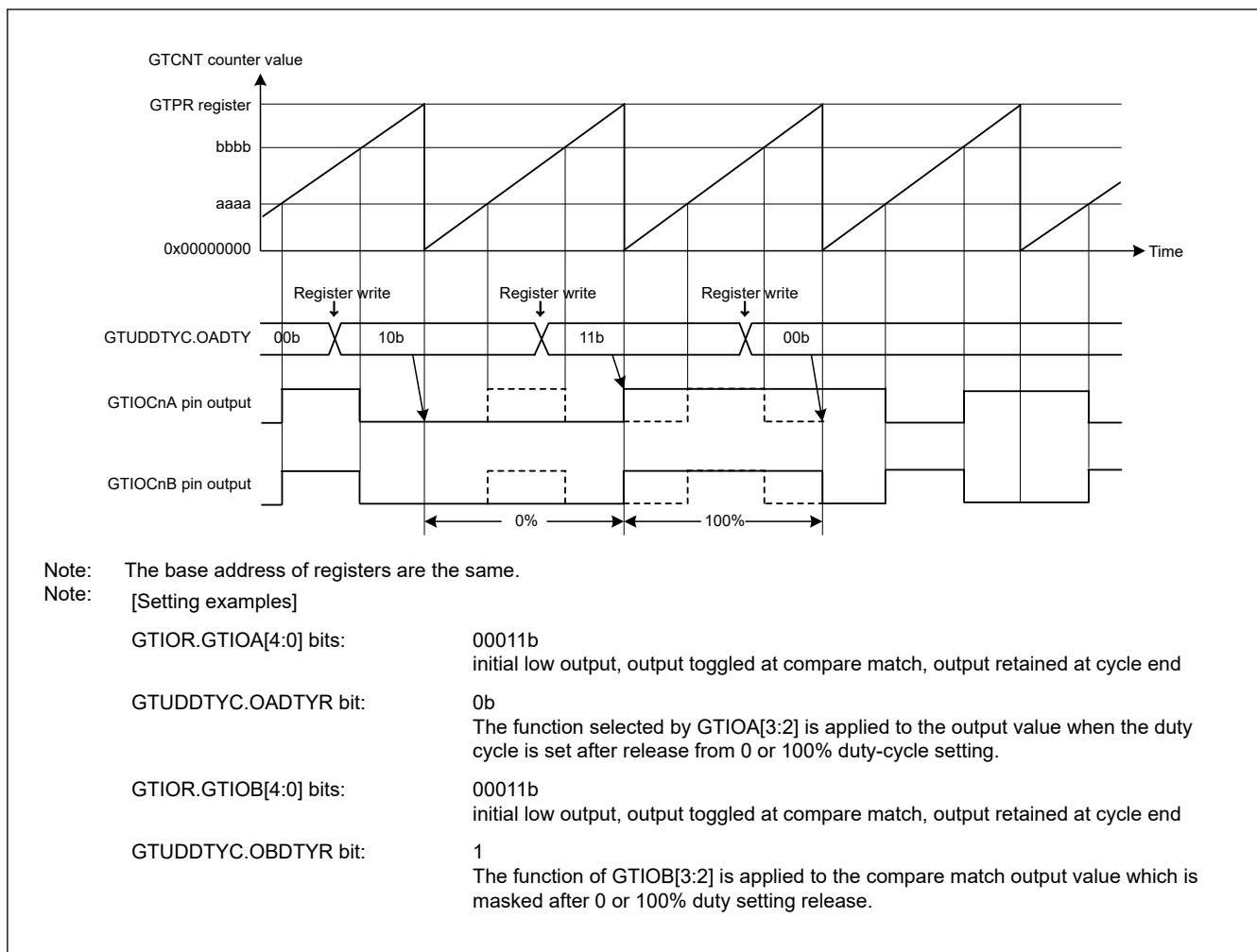
Figure 20.88 Example of output duty 0% and 100% function
