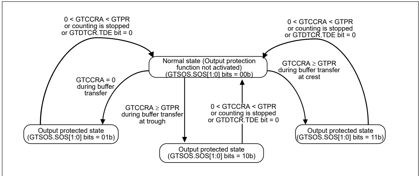
Figure 20.171 Output Protection Function
