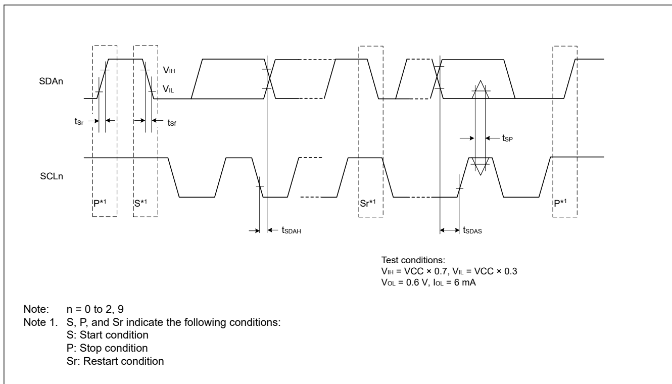
Figure 35.38 SCI simple IIC mode timing
