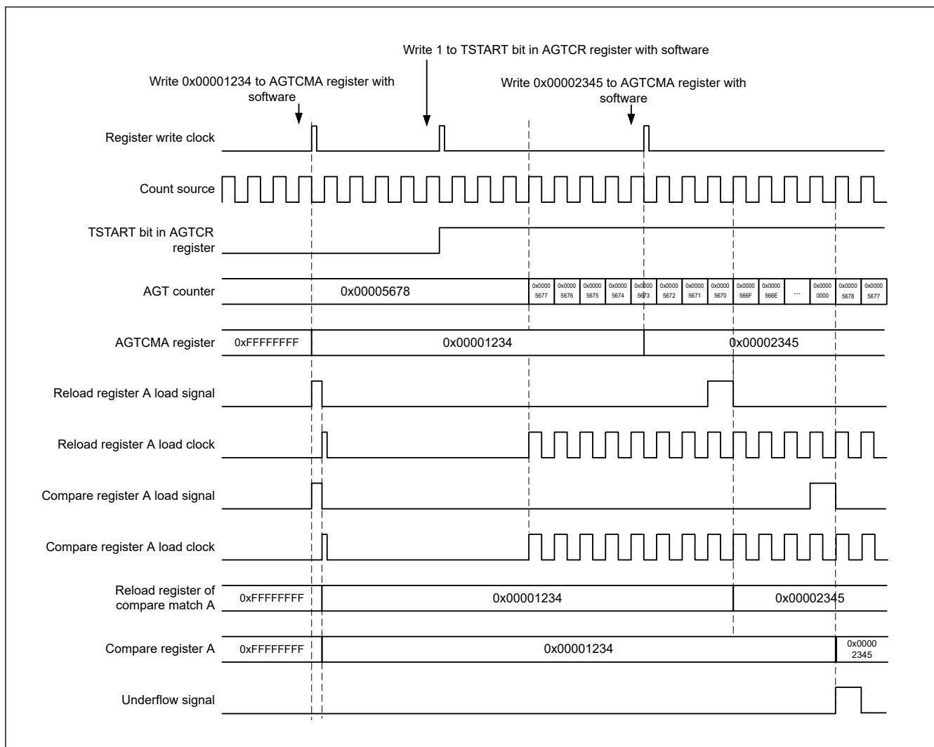
Figure 21.5 Timing of rewrite operation with the TSTART bit value for AGT compare register A
