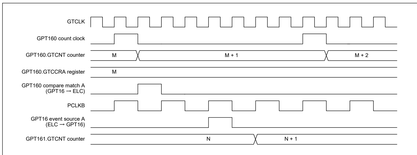
Figure 20.8 Example of event count operation (up-counting the number of event signals input from ELC_GPTA)
