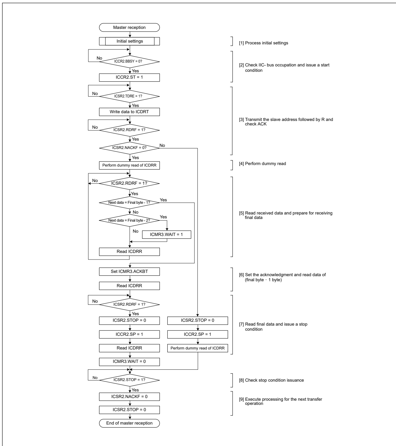
Figure 25.11 Example master reception flow with 7-bit address format of 3 or more bytes
