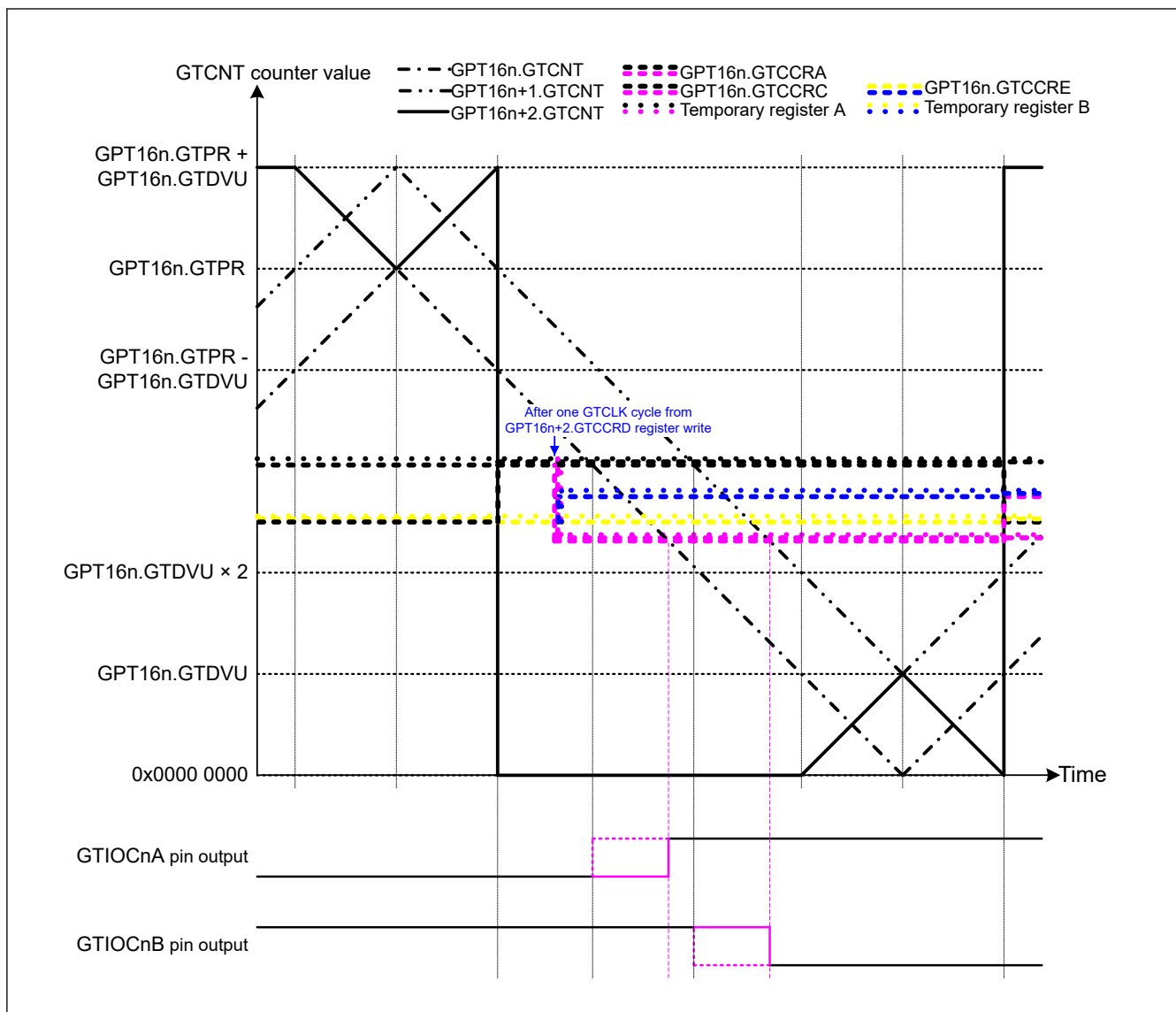
Figure 20.77 Example of complementary PWM mode 4 double buffer operation (down-counting middle section) (complementary PWM mode 4 double buffer operation, GTIOCnA pin = low/GTIOCnB pin = high at GTCCRA register compare match during up-counting, GTIOCnA pin = high/GTIOCnB pin = low at GTCCRA register compare match during down-counting, when a value smaller than the GPT16n.GTCNT value is written to GTCCRD register before down-counting compare match) ( n = 0 )
