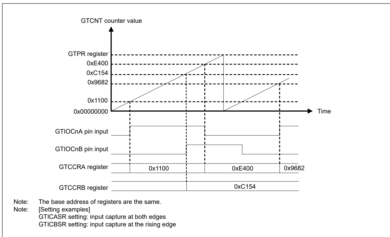
Figure 20.13 Example of input capture operation
