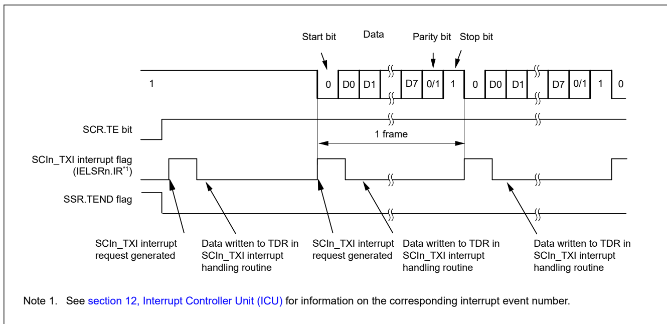
Figure 24.7 Example operation for serial transmission in asynchronous mode (1) with 8-bit data, parity bit, 1 stop bit, CTS function not used, and at the beginning of transmission
