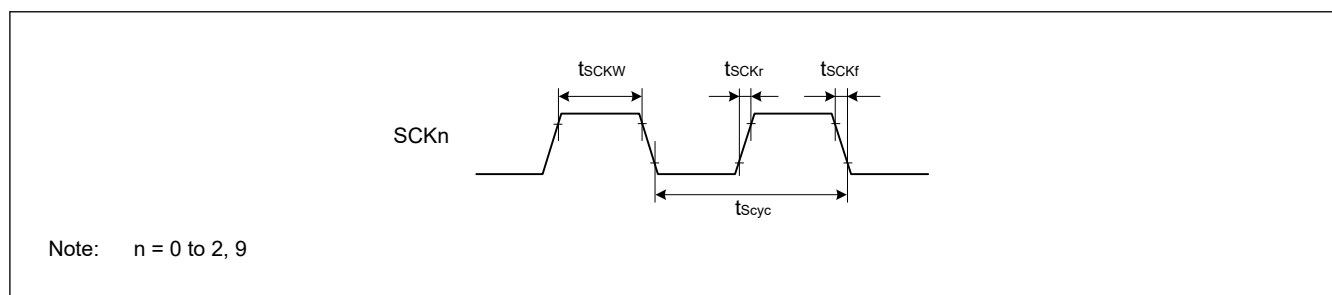
Figure 35.31 SCK clock input timing
