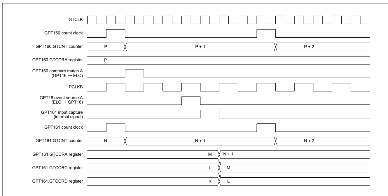
Figure 20.16 Example of the timing of input capture operation in response to ELC_GPTA event input
