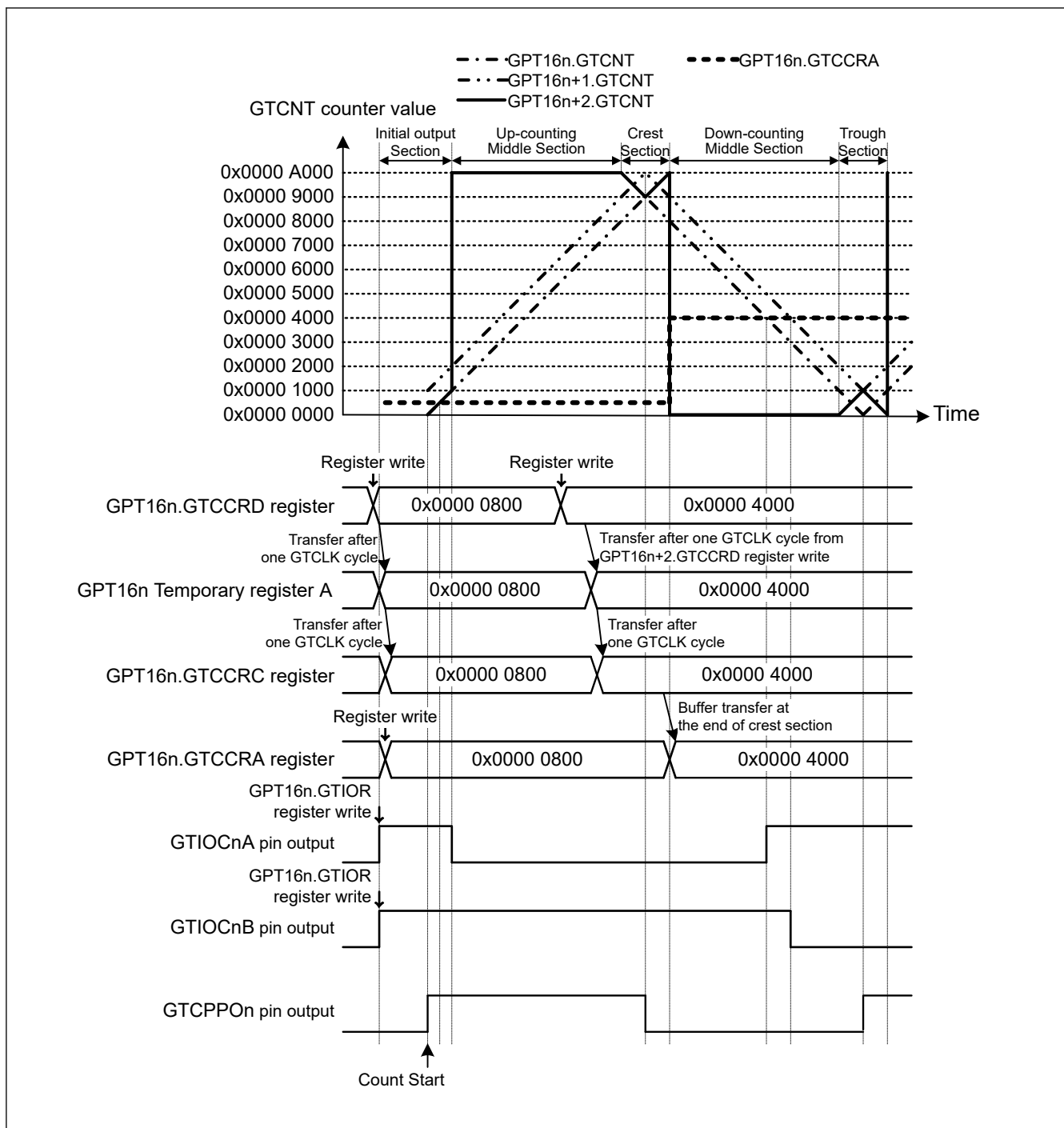
Figure 20.68 Example of complementary PWM mode initial output operation (complementary PWM mode 1 operation, GTIOCnA pin = low/GTIOCnB pin = high at GTCCRA register compare match during up-counting, GTIOCnA pin = high/GTIOCnB pin = low at GTCCRA register compare match during down-counting, the dead time value is 0x0000 1000, in the case that the initial GTCCRA register value is equal to or less than the dead time value) (n = 0)
