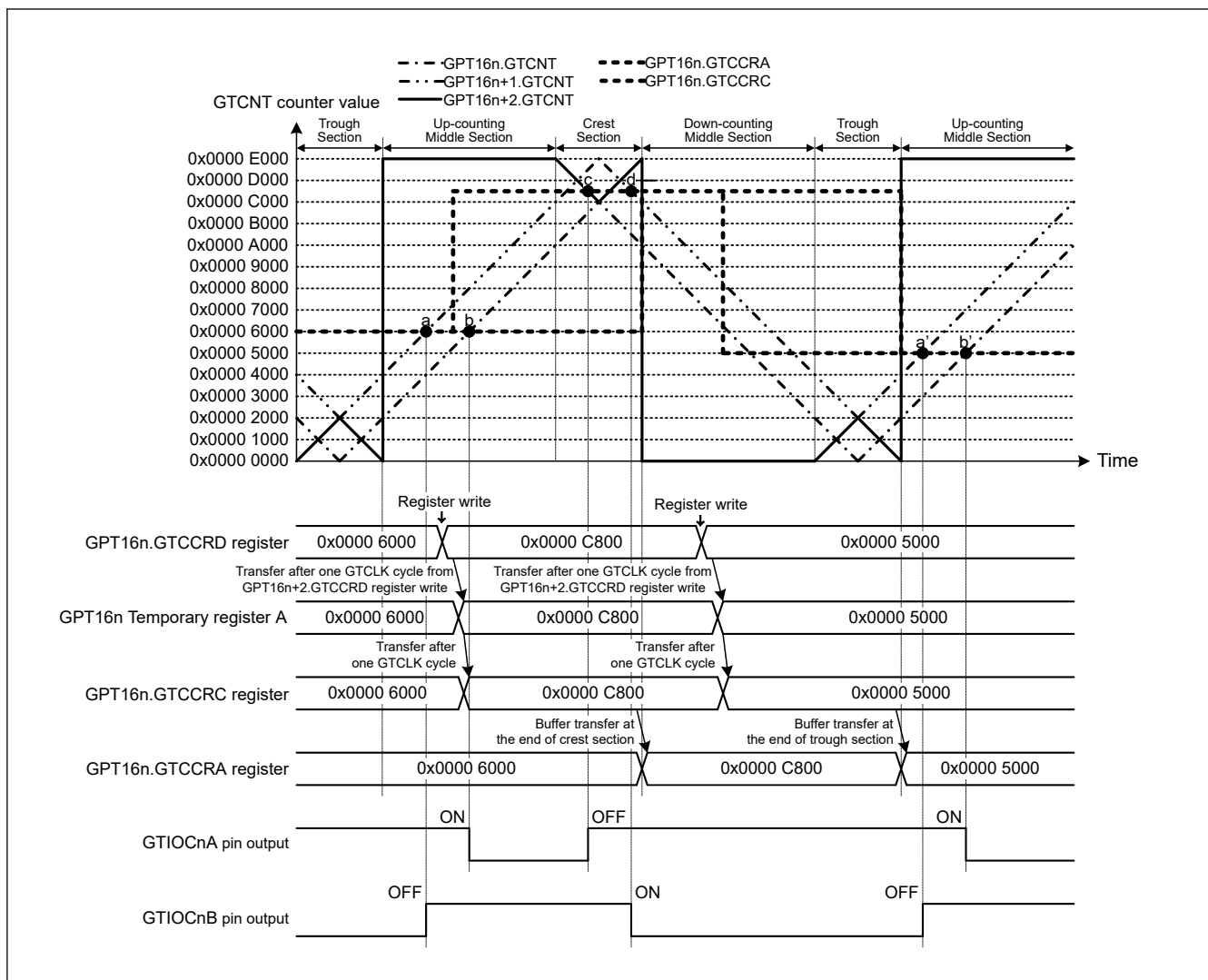
Figure 20.55 Example of compare match generation sequence operation in complementary PWM mode (complementary PWM mode 3 single buffer operation, GTIOCnA pin = low/GTIOCnB pin = high at GTCCRA register compare match during up-counting, GTIOCnA pin = high/GTIOCnB pin = low at GTCCRA register compare match during down-counting, the dead time value is 0x0000 2000, compare match generation order: a → b → c → d) (n = 0)
