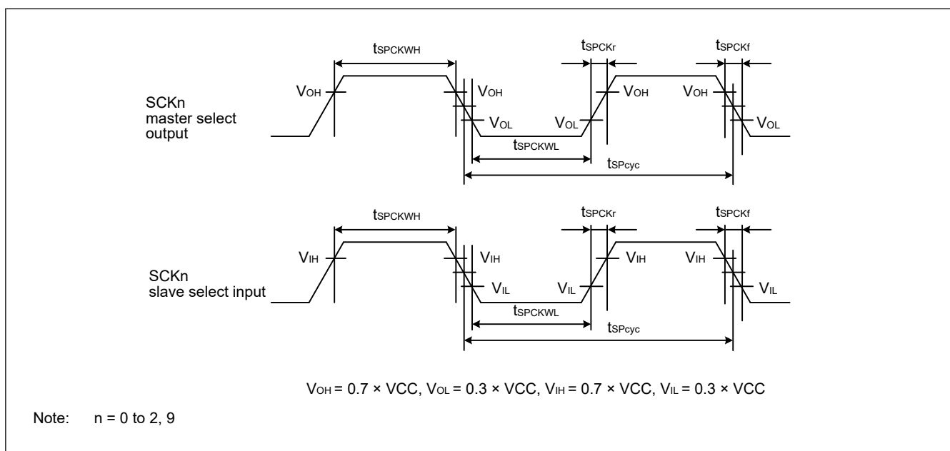
Figure 35.33 SCI simple SPI mode clock timing
