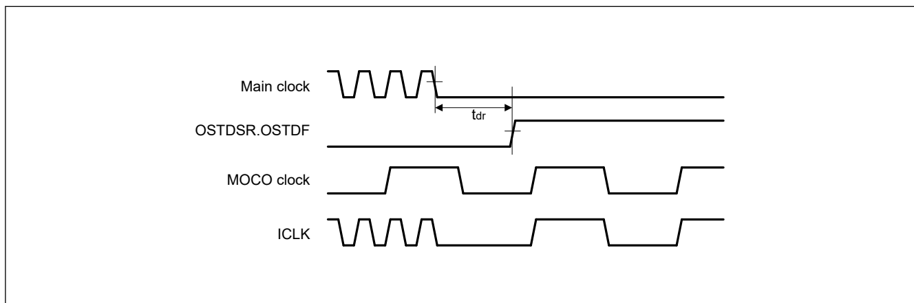
Figure 35.51 Oscillation stop detection timing
