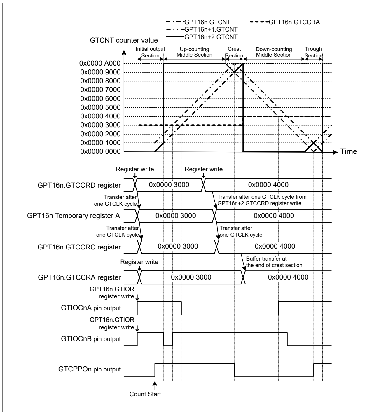
Figure 20.67 Example of complementary PWM mode initial output operation (complementary PWM mode 1 operation, GTIOcNA pin = low/GTIOcNB pin = high at GTCCRA register compare match during up-counting, GTIOcNA pin = high/GTIOcNB pin = low at GTCCRA register compare match during down-counting, the dead time value is 0x0000 1000, in the case that the initial GTCCRA register value is larger than the dead time value) (n = 0)
