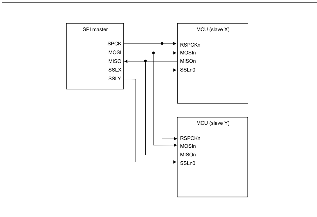
Figure 26.9 Single-master/multi-slave configuration example with the MCU as a slave
