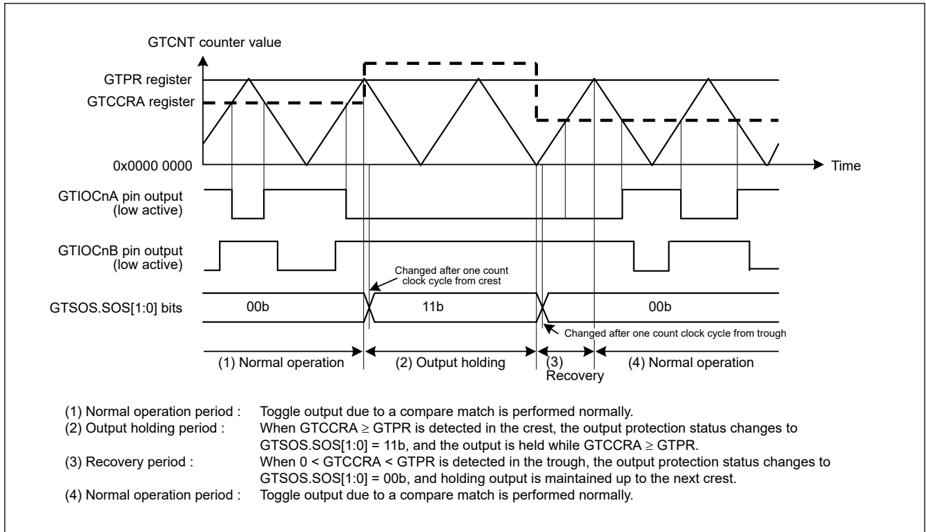
Figure 20.179 Example of output protection function operation when GTCCRA \geq GTPR is set during buffer transfer at crests (restored to 0 < GTCCRA < GTPR during buffer transfer at troughs, active level: low) (n = 0 to 2)
