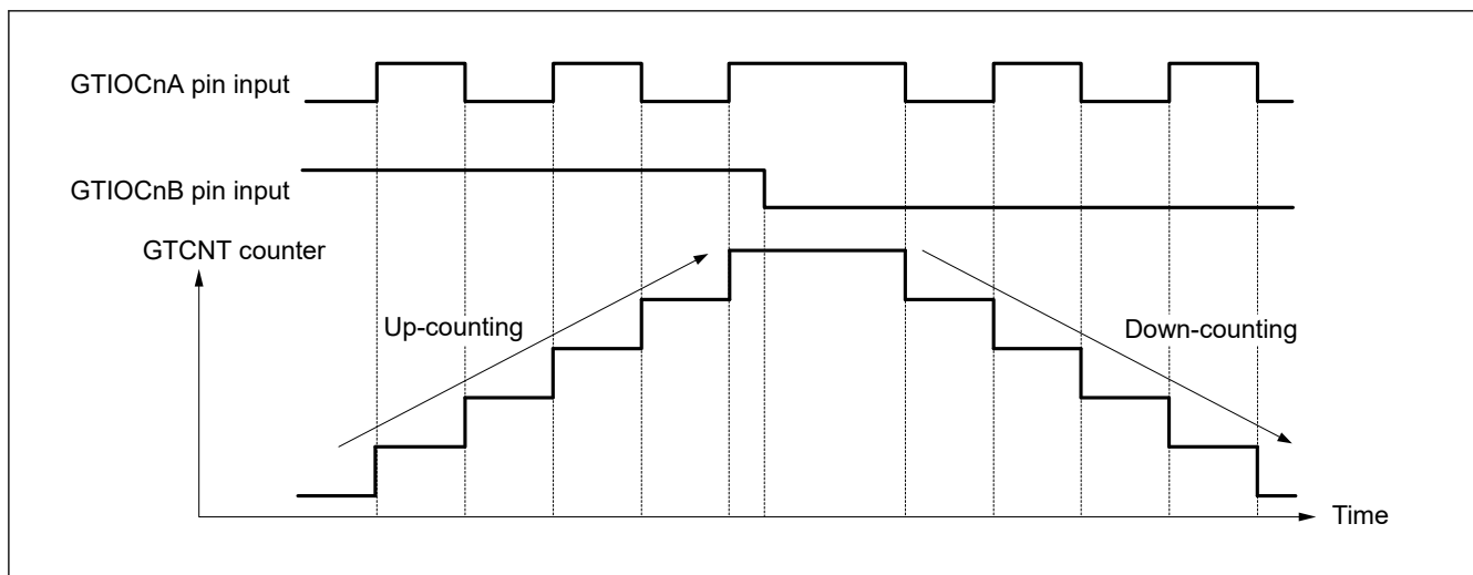
Figure 20.126 Example of phase counting mode 2 (C)
