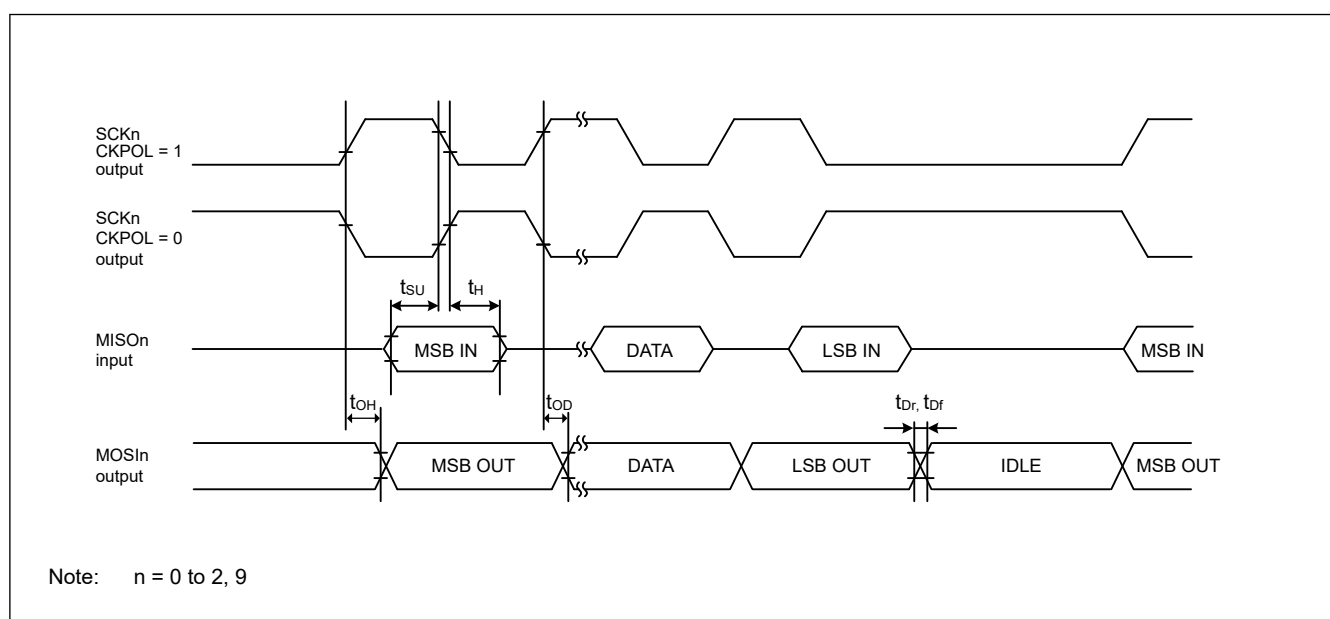
Figure 35.35 SCI simple SPI mode timing (master, CKPH = 0)
