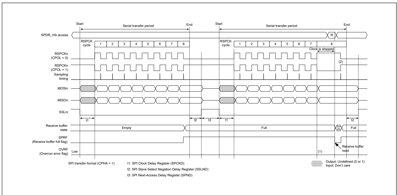
Figure 26.28 Clock stop waveform when serial transfer continues while receive buffer is full in master mode (CPHA = 1)
