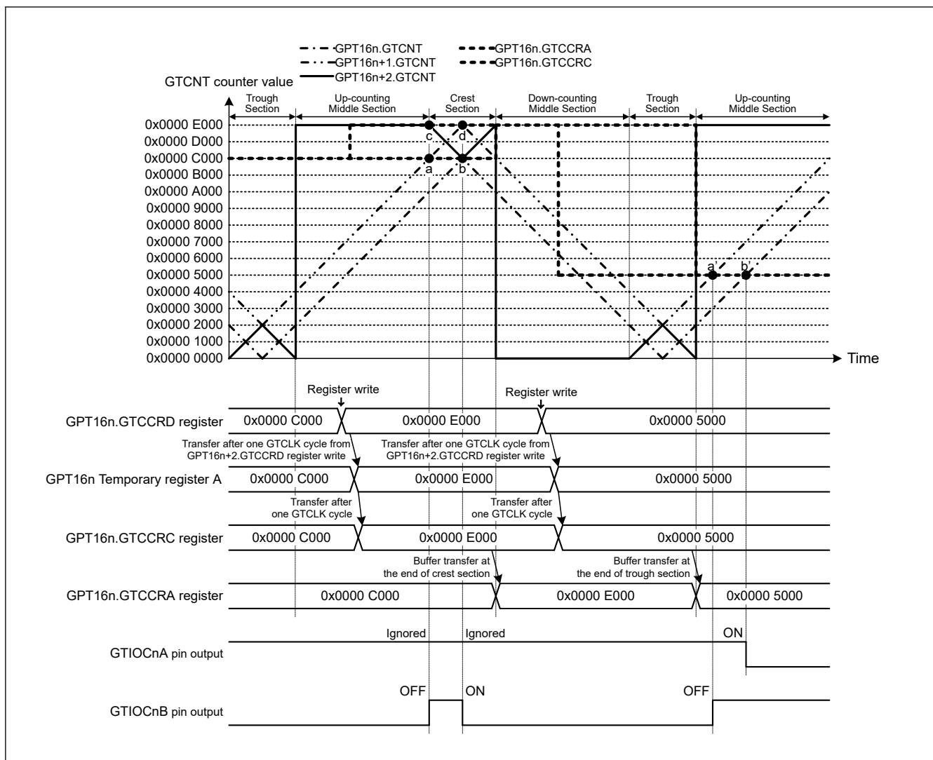
Figure 20.58 Example of compare match generation sequence operation in complementary PWM mode (complementary PWM mode 3 single buffer operation, GTIOCnA pin = low/GTIOCnB pin = high at GTCCRA register compare match during up-counting, GTIOCnA pin = high/GTIOCnB pin = low at GTCCRA register compare match during down-counting, the dead time value is 0x0000 2000, compare match generation order: (a, c) → (b, d)) (n = 0)
