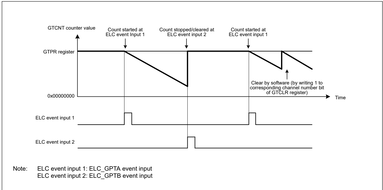
Figure 20.99 Examples of count clearing operation by hardware source in saw wave down-counting, started at ELC_GPTA input, and stopped/cleared at ELC_GPTB input
