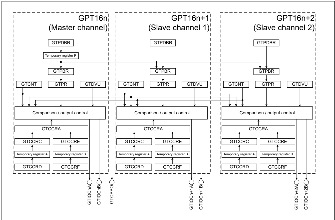
Figure 20.46 Block diagram in complementary PWM mode 1, 2, 3 ( n = 0 )
