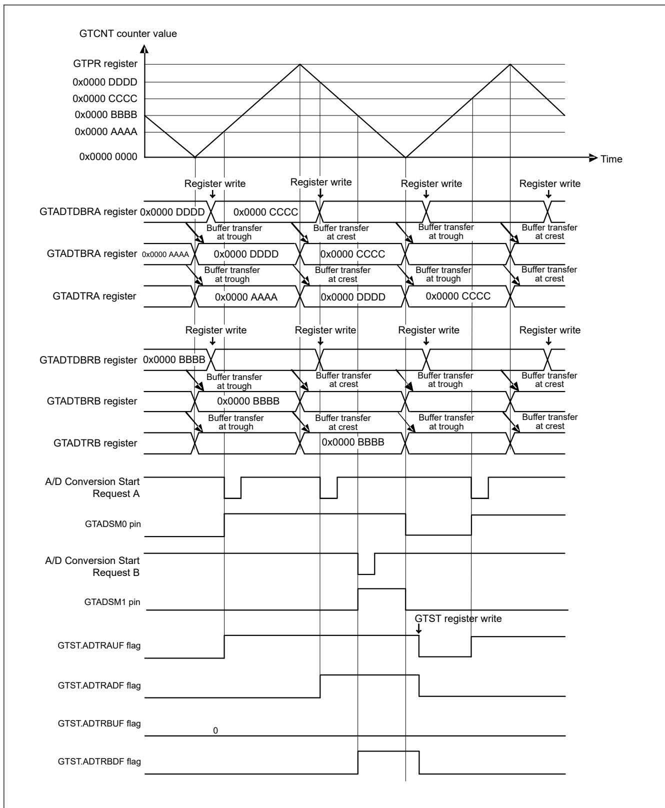
Figure 20.160 Example of A/D conversion start request timing operation (triangle-waves, double buffer operation, buffer transfer at both troughs and crests, A/D conversion start request by GTADTRA register at both up-counting and down-counting, A/D conversion start request by GTADTRB register at down-counting, monitoring of the GTADTRA register up-counting by the GTADSM0 pin, monitoring of the GTADTRB register down-counting by the GTADSM1 pin)
