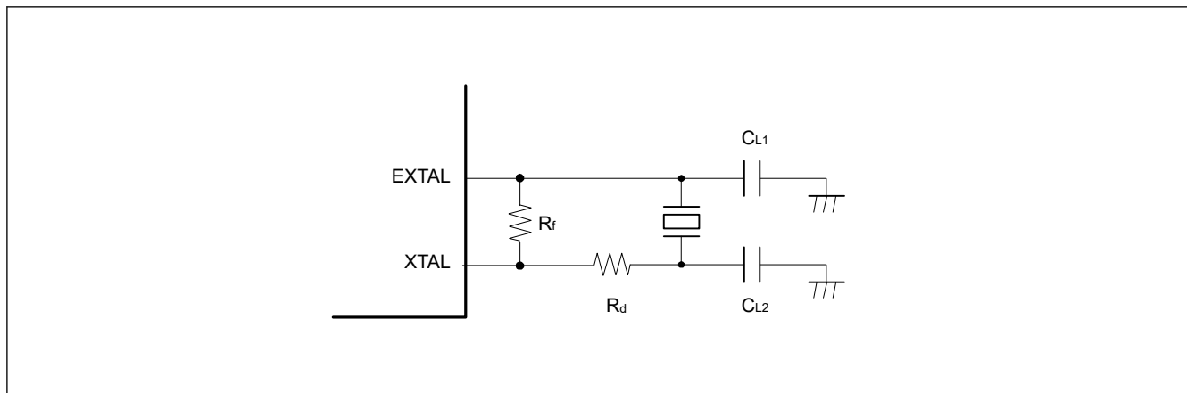
Figure 8.5 Example of a crystal resonator connection
