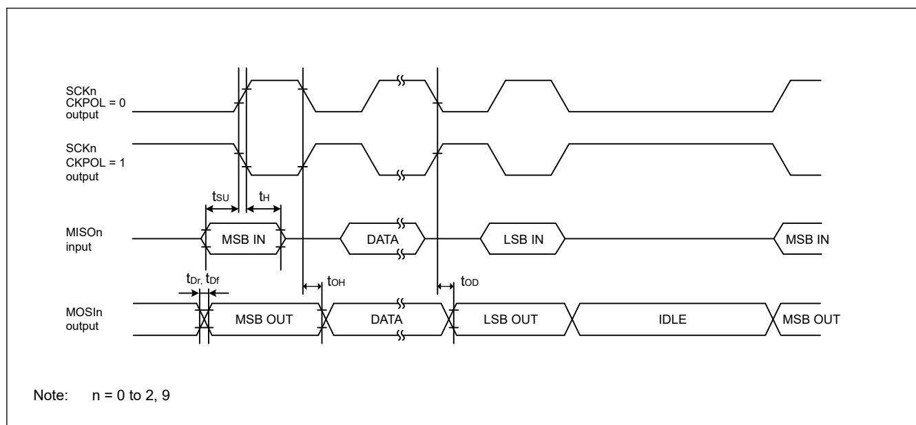
Figure 35.34 SCI simple SPI mode timing (master, CKPH = 1)
