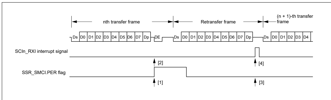
Figure 24.55 Data re-transfer operation in smart card interface reception mode
