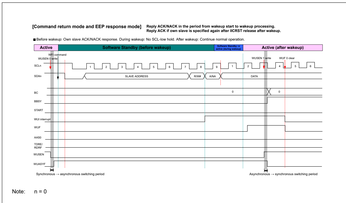
Figure 25.37 Timing of command recovery and EEP response modes
