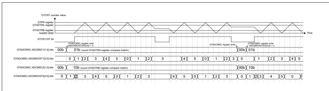
Figure 20.156 Example of A/D conversion start request compare match skipping function operation
