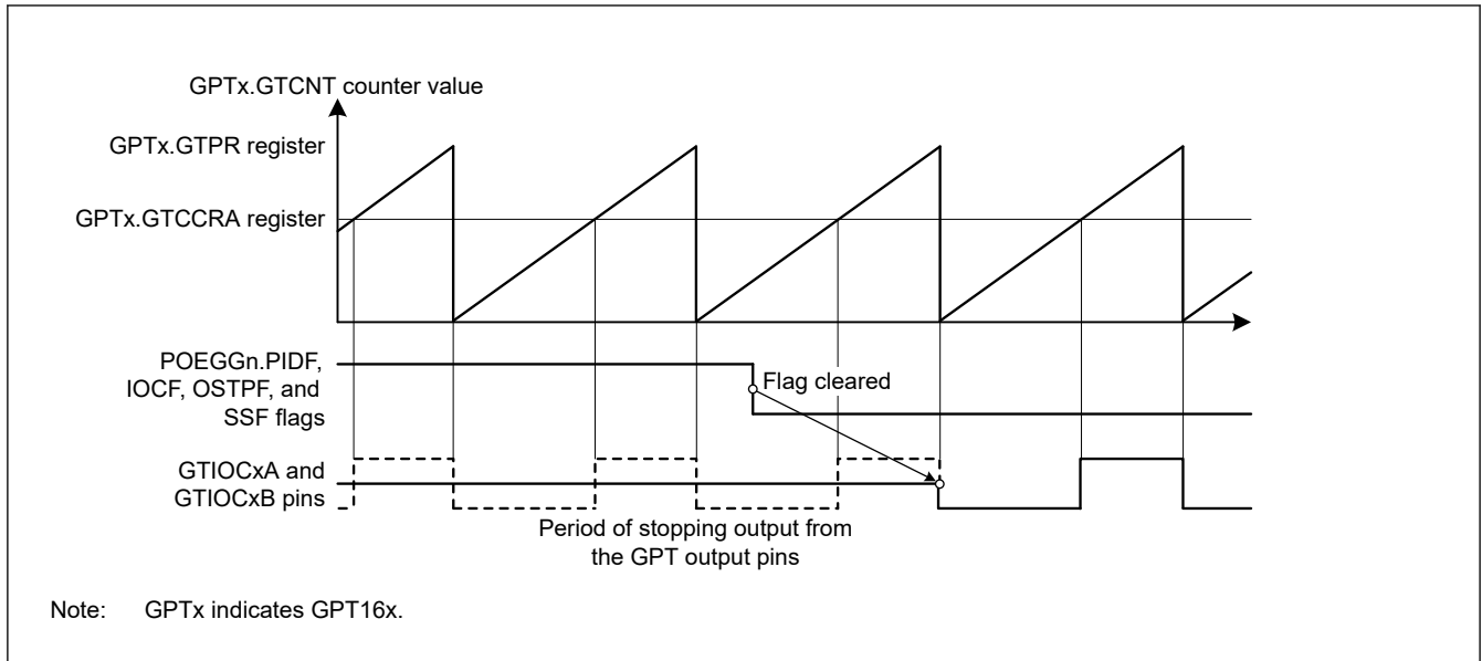
Figure 19.3 Timing of reenabling output from the GPT output pins following cancellation of a request to stop output
