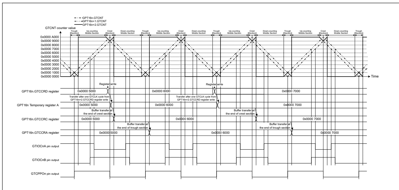
Figure 20.50 Example of complementary PWM mode 2 operation (GTIOCnA pin = low/GTIOCnB pin = high at GTCCRA register compare match during up-counting, GTIOCnA pin = high/GTIOCnB pin = low at GTCCRA register compare match during down-counting, the dead time value is 0x0000 1000 and updating GTCCRD register in crest and trough sections) (n = 0)
