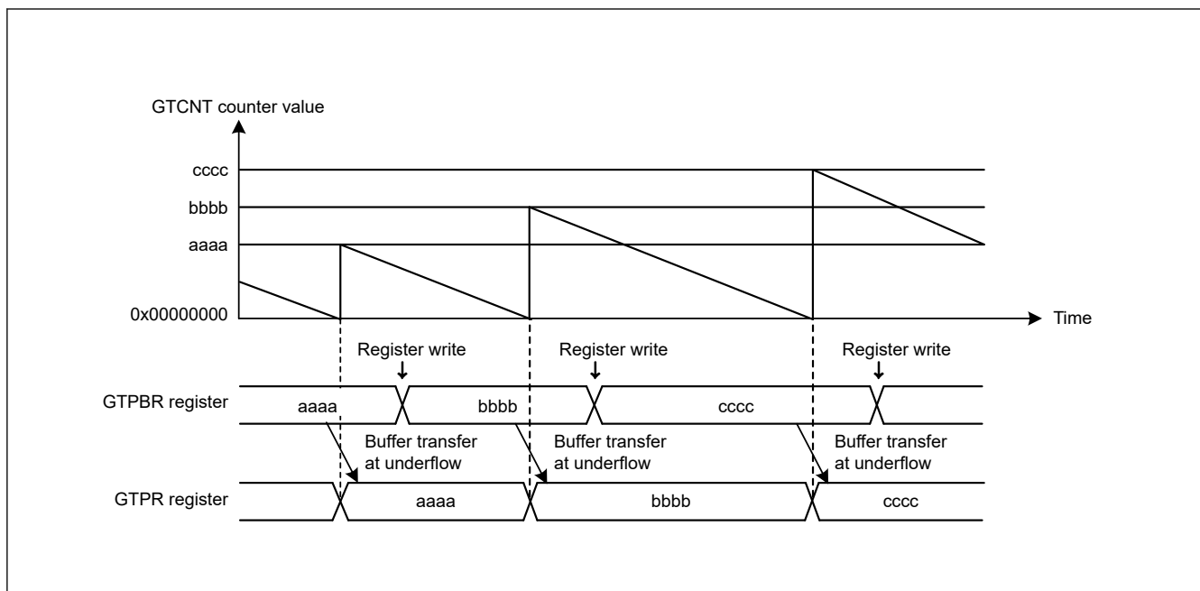
Figure 20.19 Example of GTPR buffer operation with saw waves in down-counting
