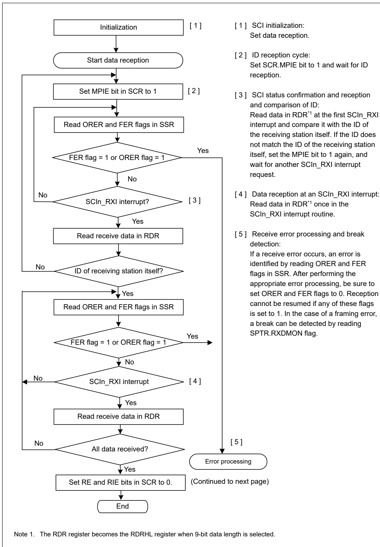
Figure 24.31 Example flow of multi-processor serial reception with non-FIFO selected (1)
