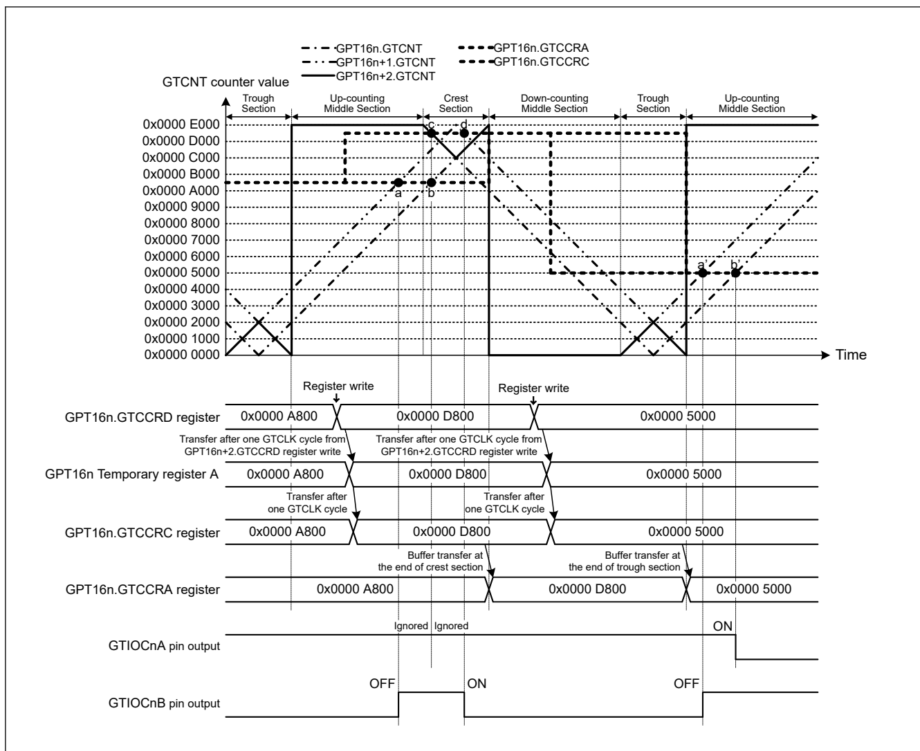
Figure 20.56 Example of compare match generation sequence operation in complementary PWM mode (complementary PWM mode 3 single buffer operation, GTIOCnA pin = low/GTIOCnB pin = high at GTCCRA register compare match during up-counting, GTIOCnA pin = high/GTIOCnB pin = low at GTCCRA register compare match during down-counting, the dead time value is 0x0000 2000, compare match generation order: a → (b, c) → d) (n = 0)
