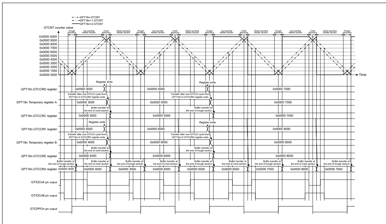
Figure 20.54 Example of complementary PWM mode 3 operation (double buffer operation, GTIOCnA pin = low/GTIOCnB pin = high at GTCCRA register compare match during up-counting, GTIOCnA pin = high/GTIOCnB pin = low at GTCCRA register compare match during down-counting, the dead time value is 0x0000 1000 and updating GTCCRD register in crest and trough sections) (n = 0)
