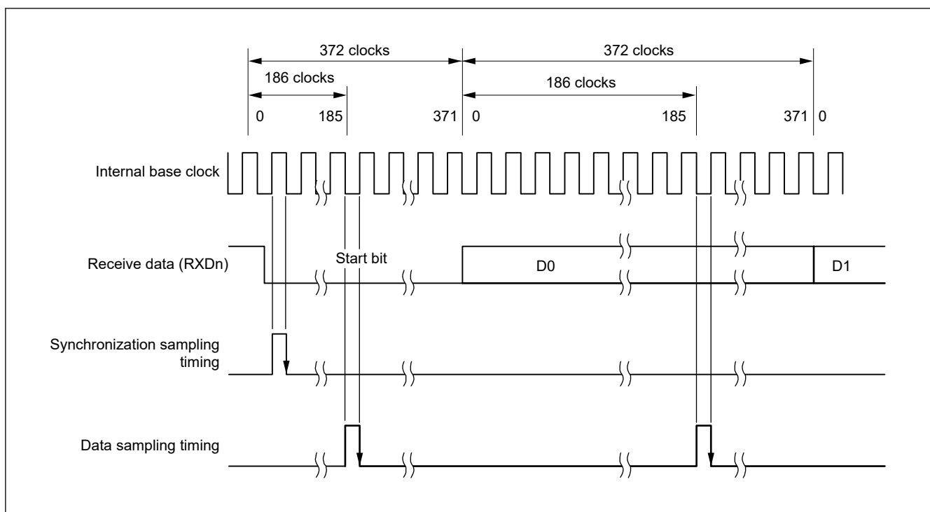
Figure 24.51 Receive data sampling timing in smart card interface mode when the clock frequency is 372 times the bit rate
