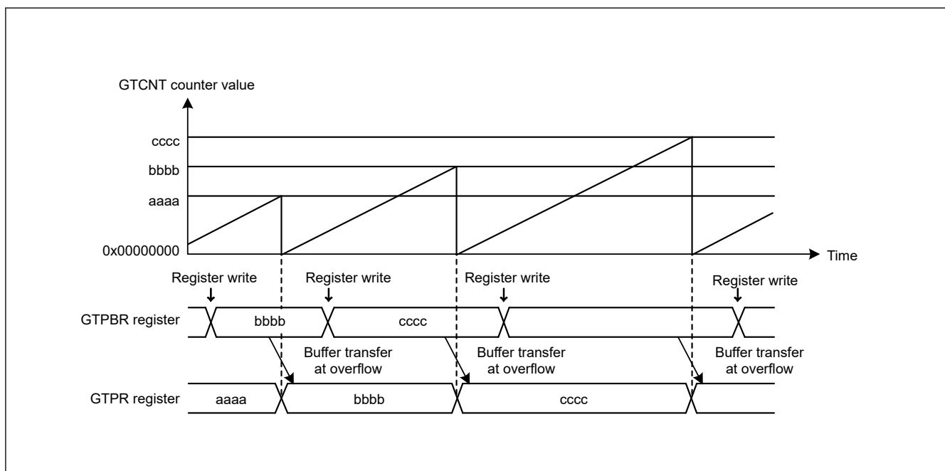
Figure 20.18 Example of GTPR buffer operation with saw waves in up-counting
