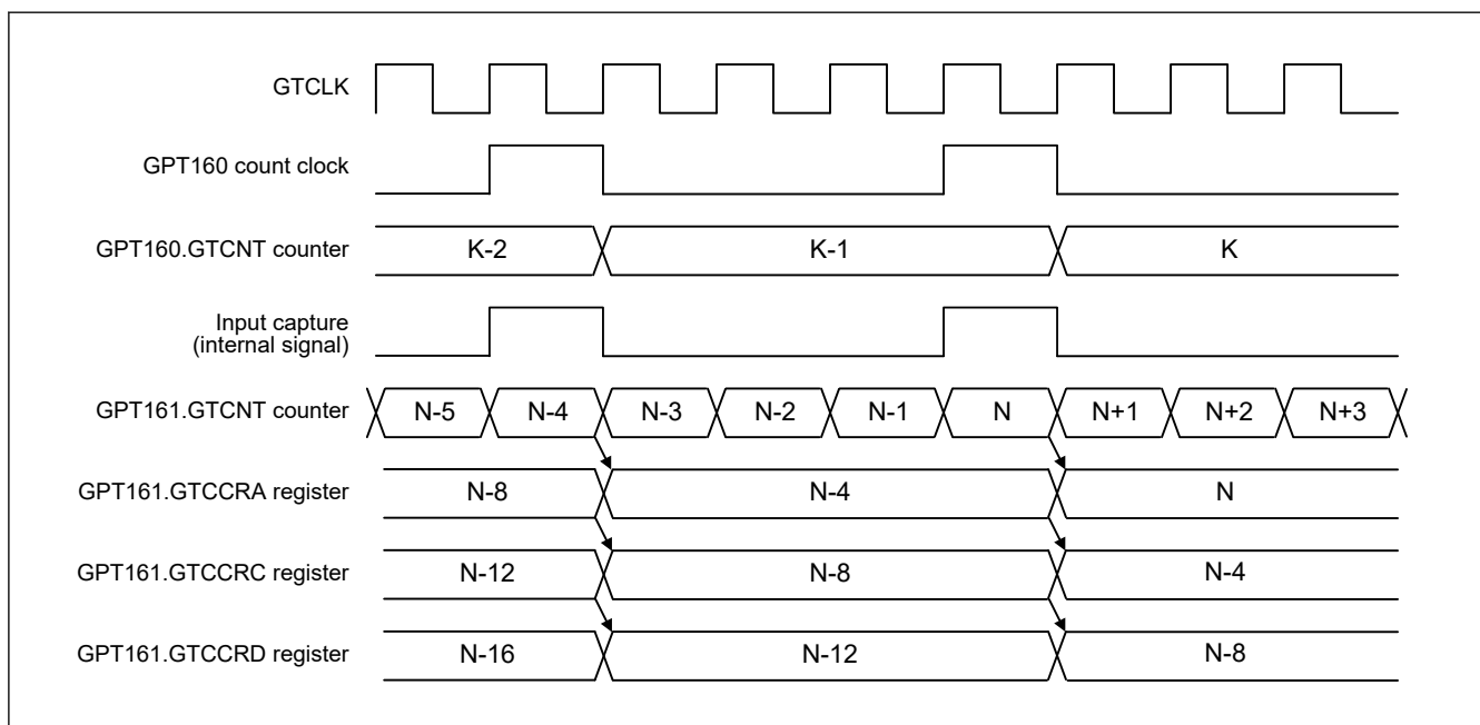
Figure 20.17 Example of the timing of input capture operation in response to count clock from other channel
