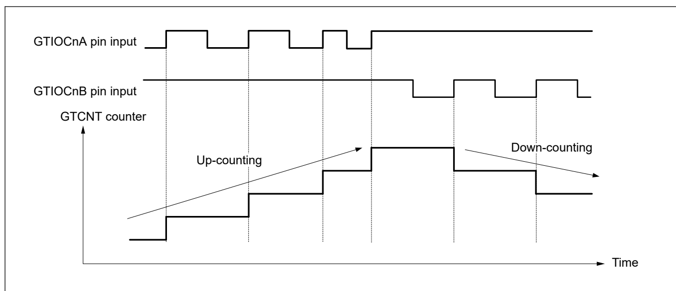
Figure 20.128 Example of phase counting mode 3 (B)
