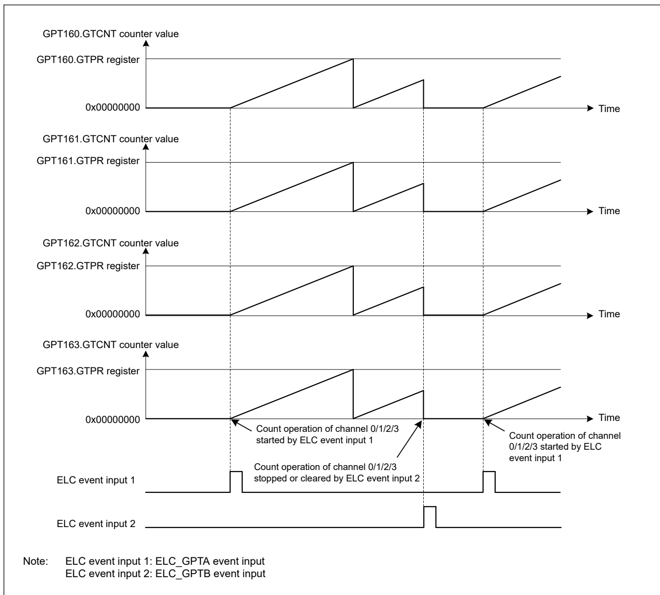
Figure 20.112 Example of a simultaneous start, stop, and clear by a hardware source with the same count cycle (GTPR register value)
