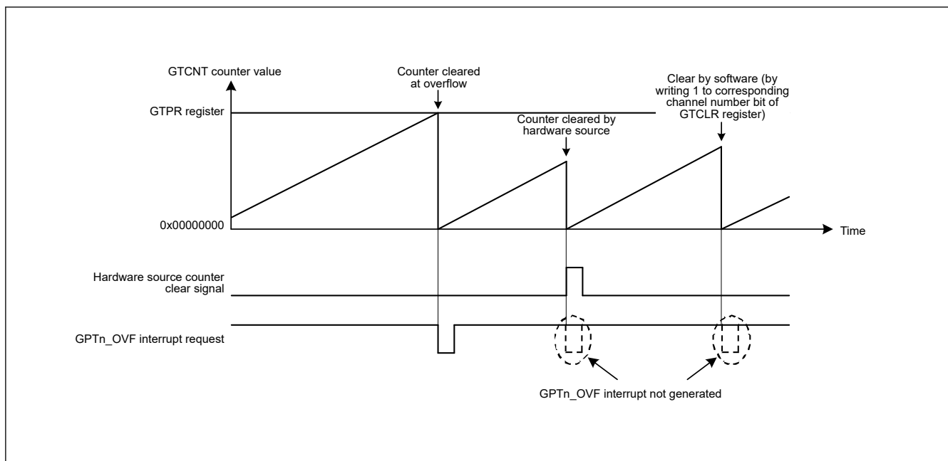
Figure 20.100 Relationship between counter clearing by hardware source and GPTn_OVF (n = 0 to 3) interrupt
