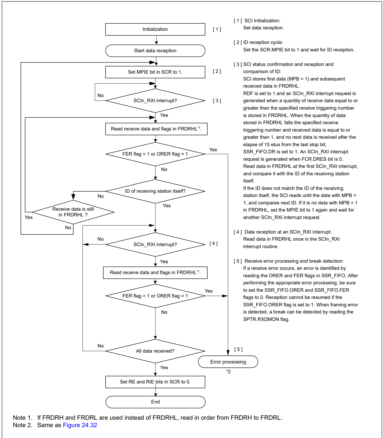
Figure 24.34 Example flow of serial reception in multi-processor mode with FIFO selected
