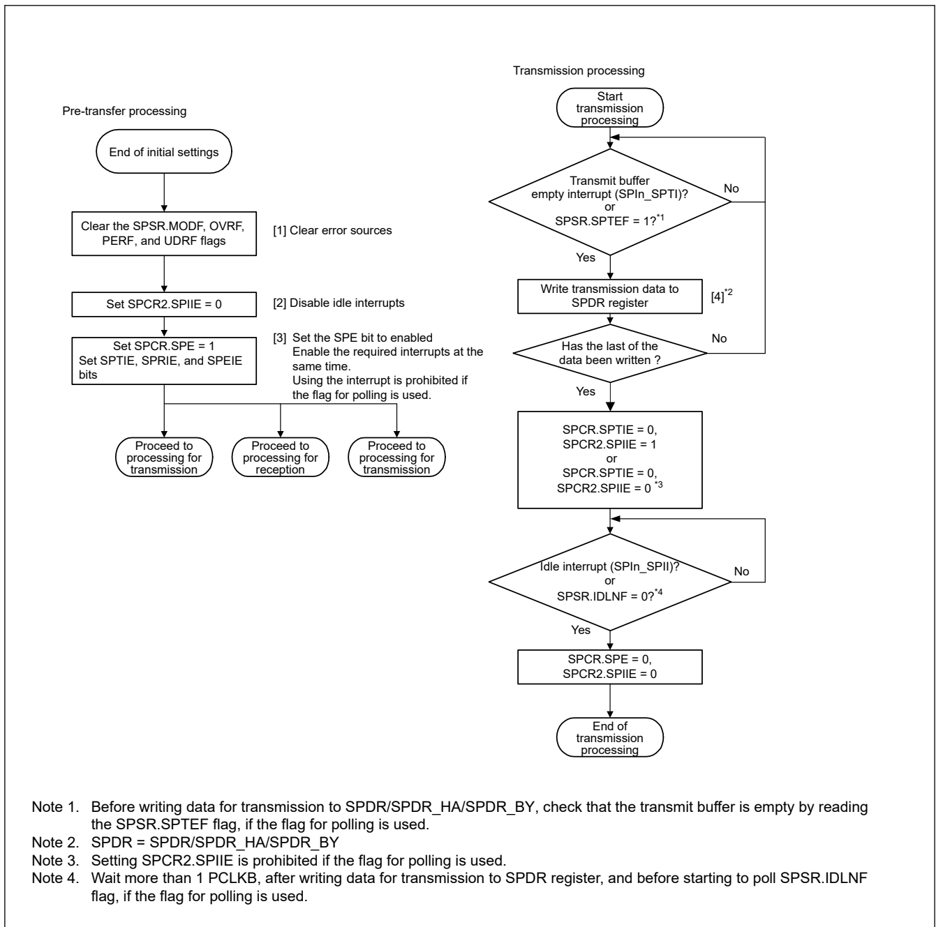
Figure 26.32 Transmission flow in master mode
