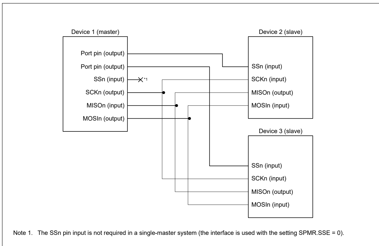
Figure 24.68 Example connections using simple SPI mode in single master mode with SPMR.SSE bit = 0
