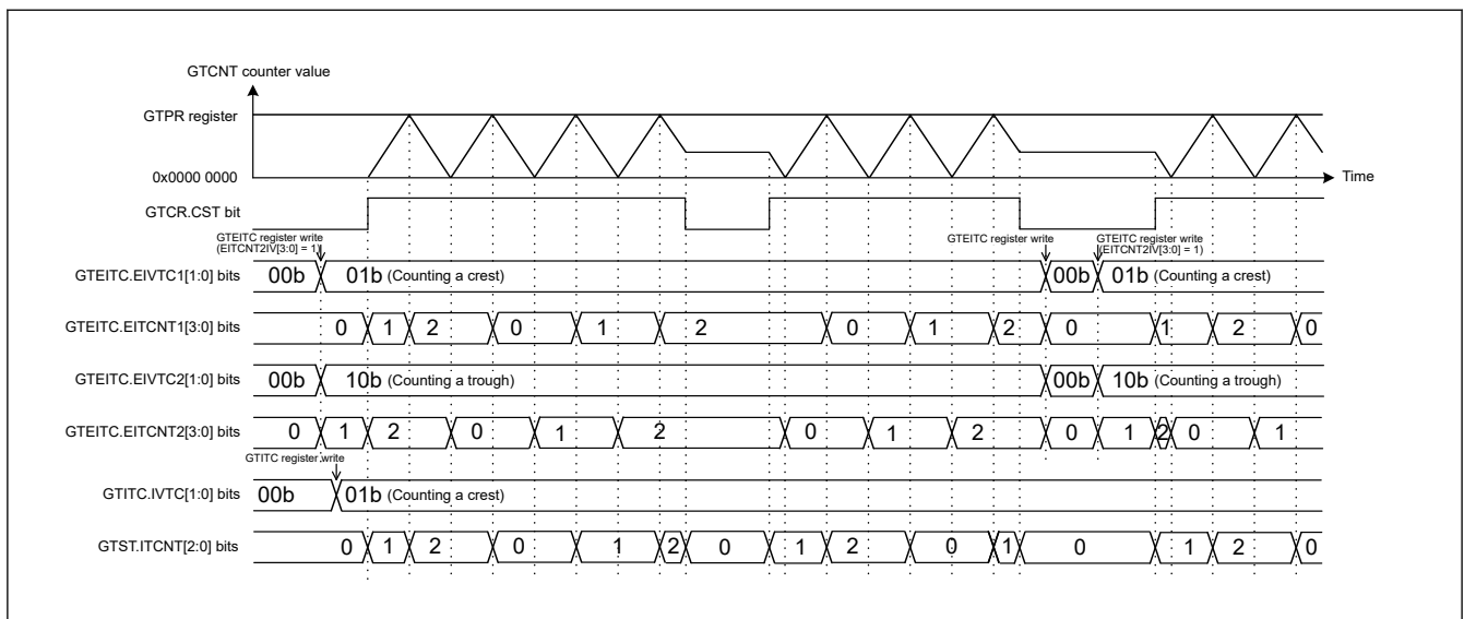
Figure 20.145 Example of counter operation for interrupt skipping
