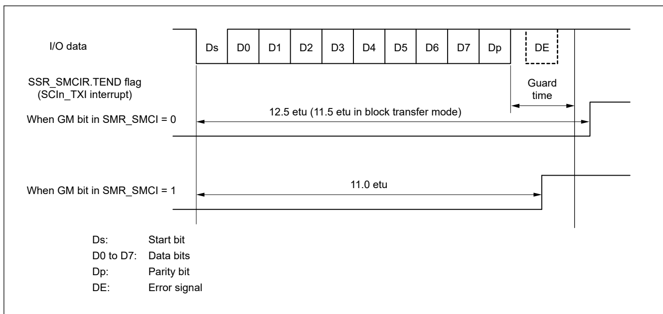
Figure 24.53 SSR.TEND flag generation timing during transmission
