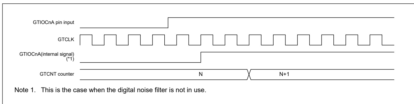
Figure 20.7 Example of event count operation (up-counting of rising edges of the input on the GTIOCnA pin)
