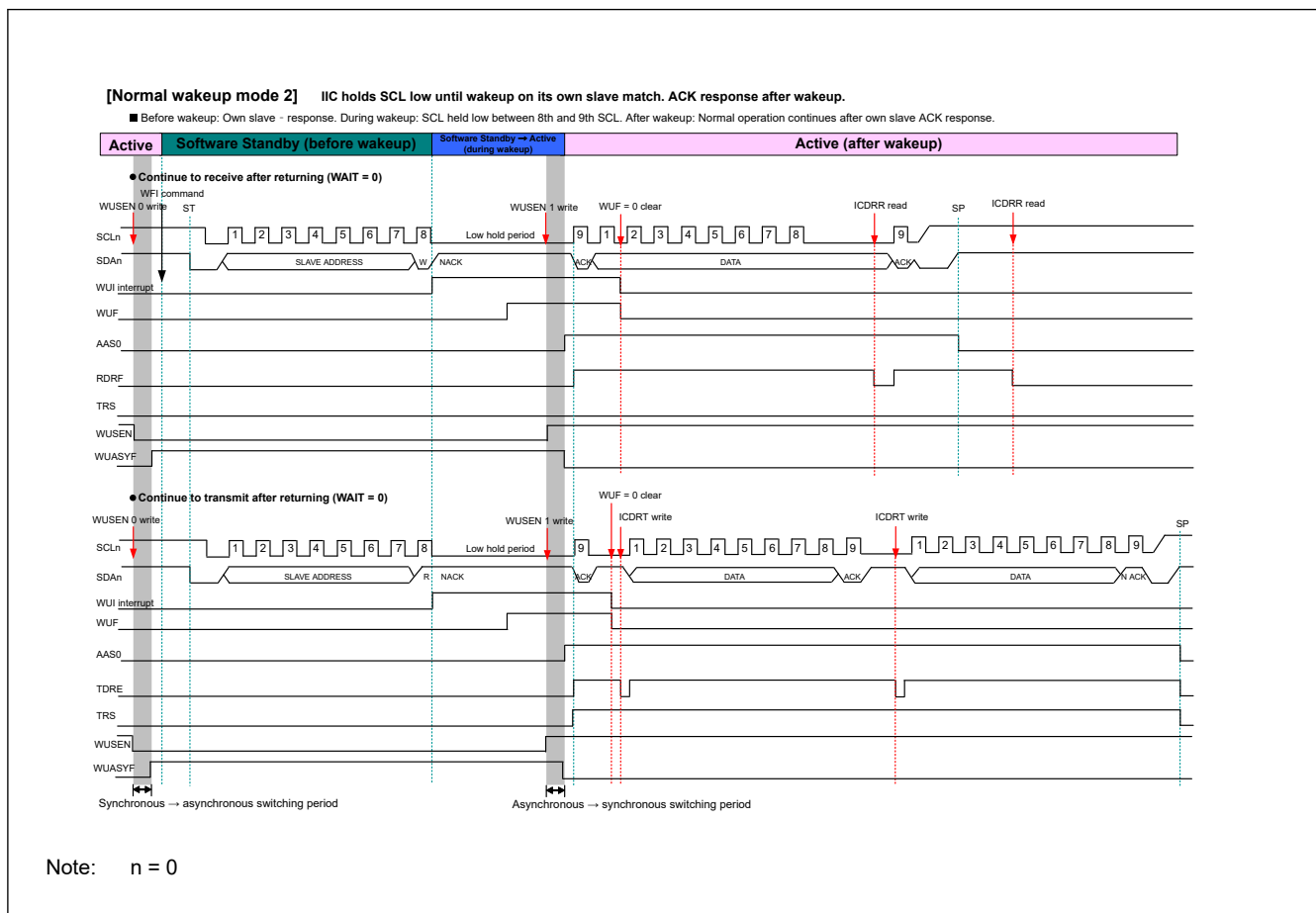
Figure 25.34 Timing of normal wakeup mode 2
