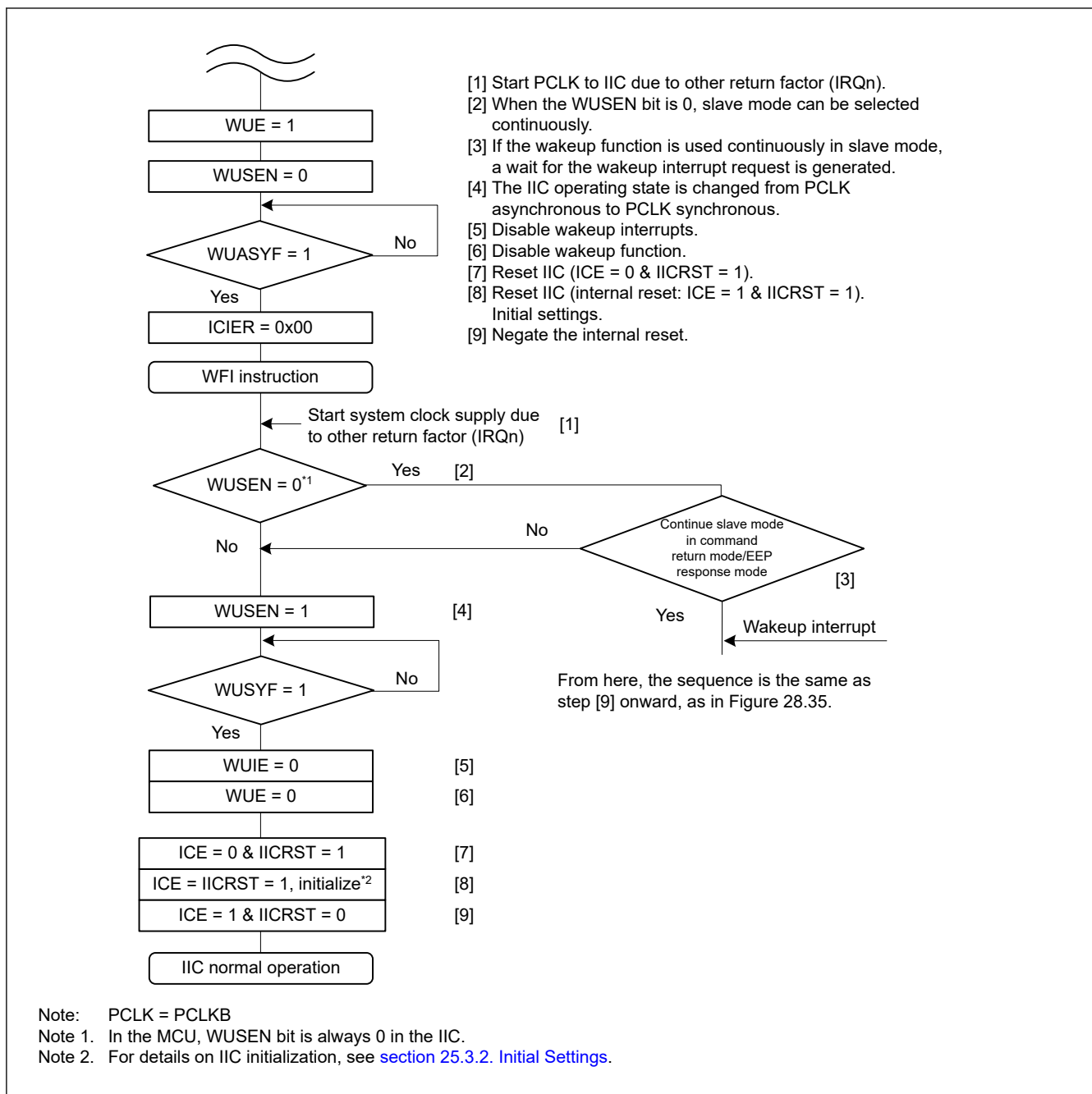
Figure 25.36 Example operation of command recovery and EEP response modes when wakeup is triggered by an interrupt other than IIC wakeup interrupt, for example, the IRQn
