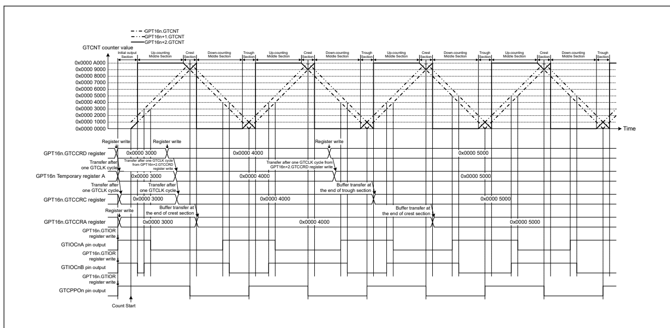
Figure 20.47 Example of complementary PWM mode 1 operation (GTIOCN A pin = high/GTIOCN B pin = high as initial output, GTIOCN A pin = low/GTIOCN B pin = high at GTCCRA register compare match during up-counting, GTIOCN A pin = high/GTIOCN B pin = low at GTCCRA register compare match during down-counting, the dead time value is 0x0000 1000 and updating GTCCRD register in middle section) (n = 0)
