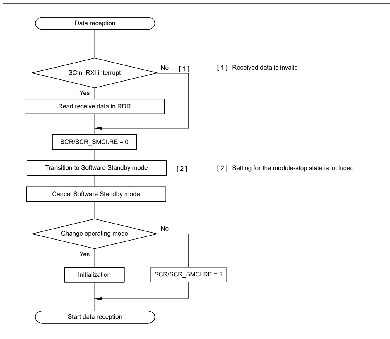
Figure 24.75 Example flow of transition to Software Standby mode during reception
