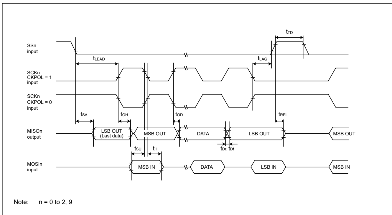
Figure 35.37 SCI simple SPI mode timing (slave, CKPH = 0)
