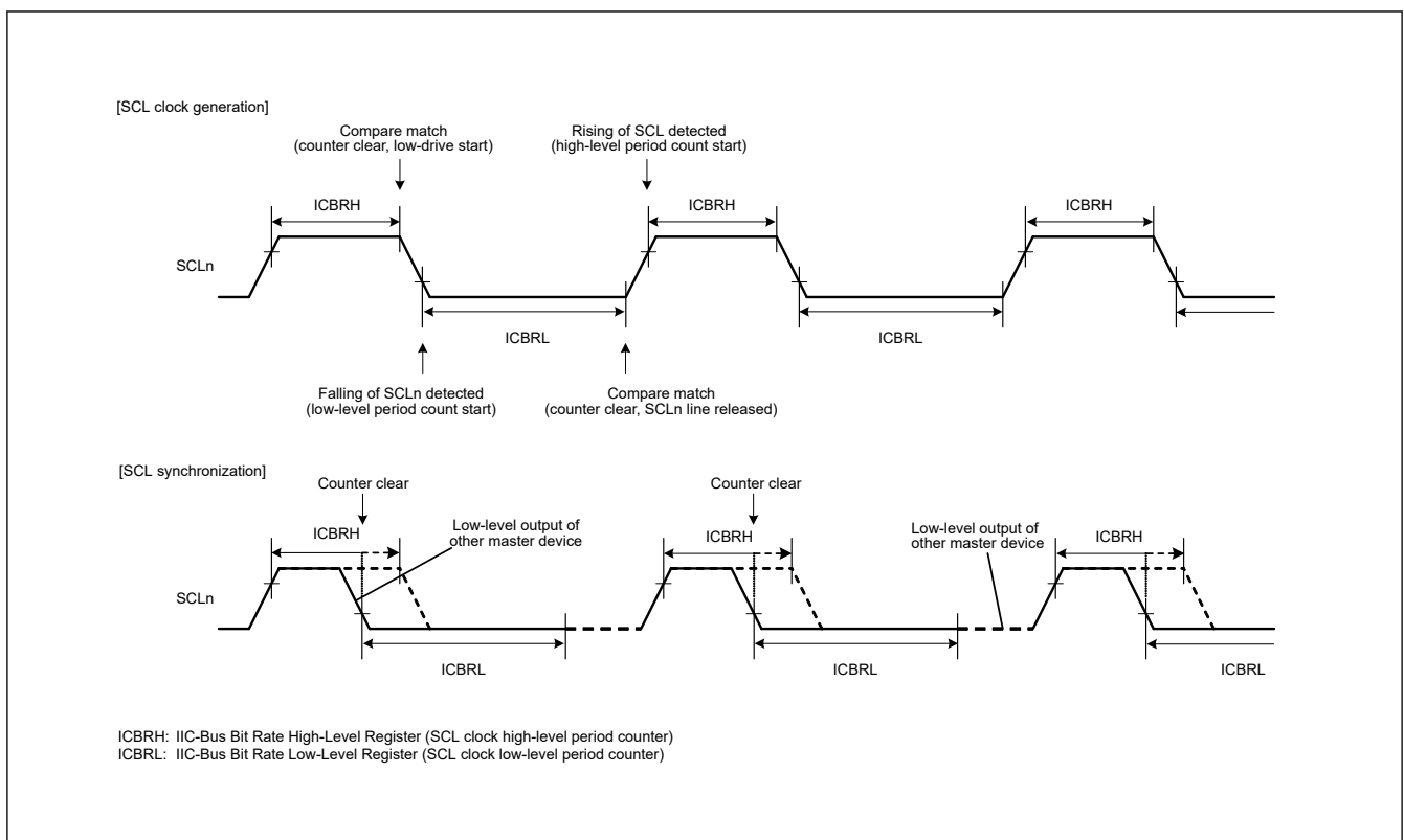
Figure 25.21 Generation and synchronization of SCL signal from IIC
