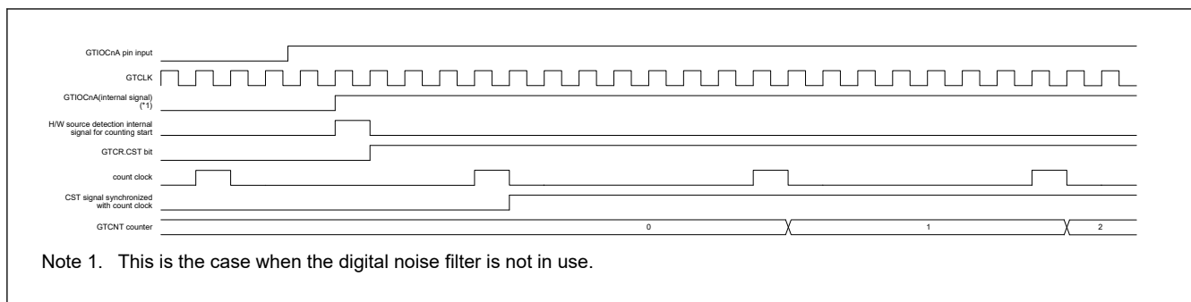
Figure 20.91 Example of timing of operations to start counting in response to a rising edge of the input on the GTIOCnA pin
