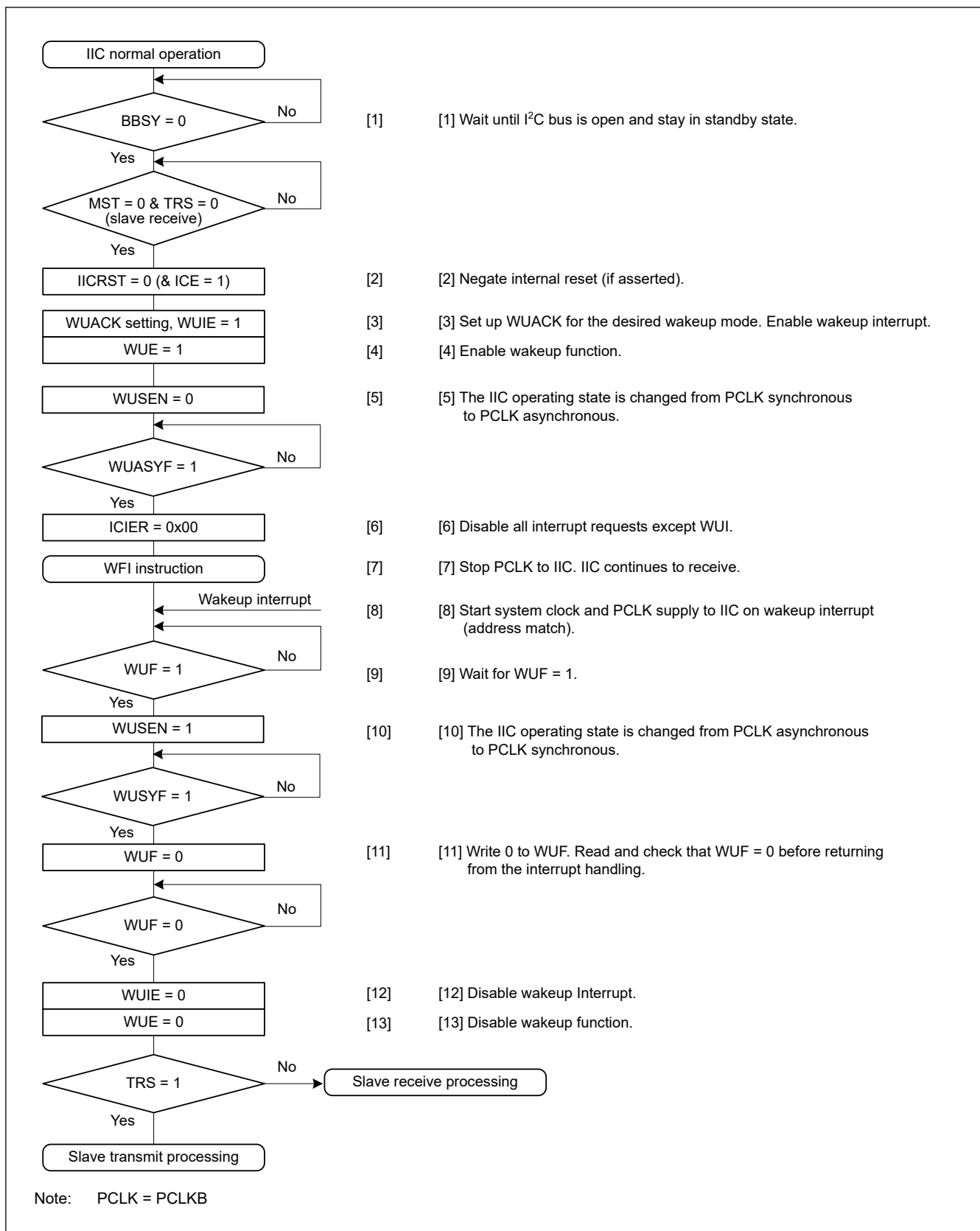
Figure 25.30 Example operation of normal wakeup mode 1 when wakeup is triggered by a wakeup interrupt on match of the slave address
