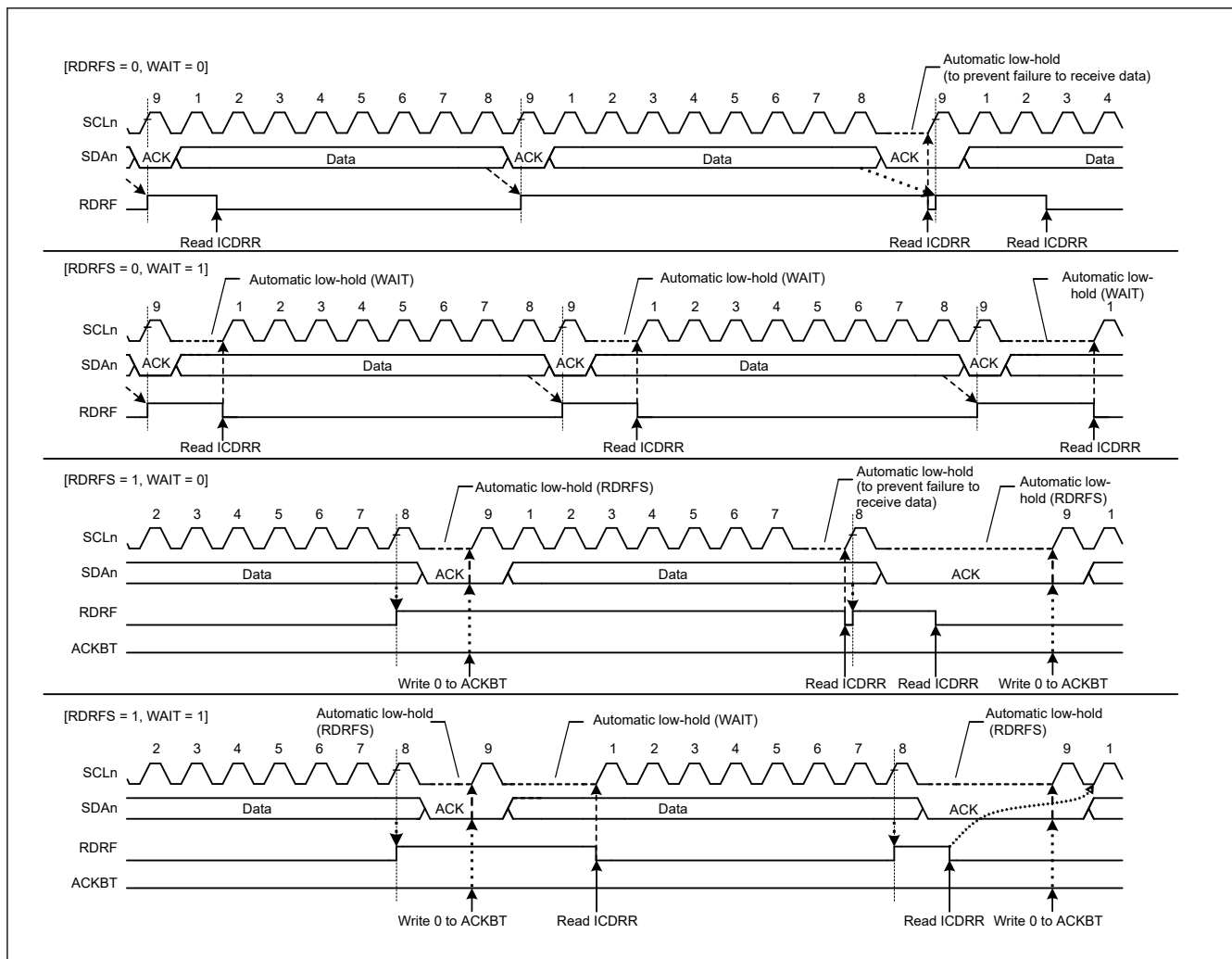
Figure 25.40 Automatic low-hold operation in receive mode using the RDRFS and WAIT bits
