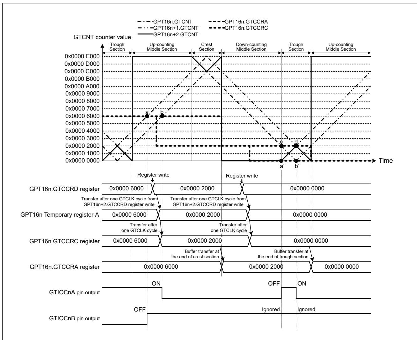
Figure 20.64 Example of compare match generation sequence operation in complementary PWM mode (complementary PWM mode 3 single buffer operation, GTIOCnA pin = low/GTIOCnB pin = high at GTCCRA register compare match during up-counting, GTIOCnA pin = high/GTIOCnB pin = low at GTCCRA register compare match during down-counting, the dead time value is 0x0000 2000, compare match generation order: (c, a') → (d, b')) (n = 0)
