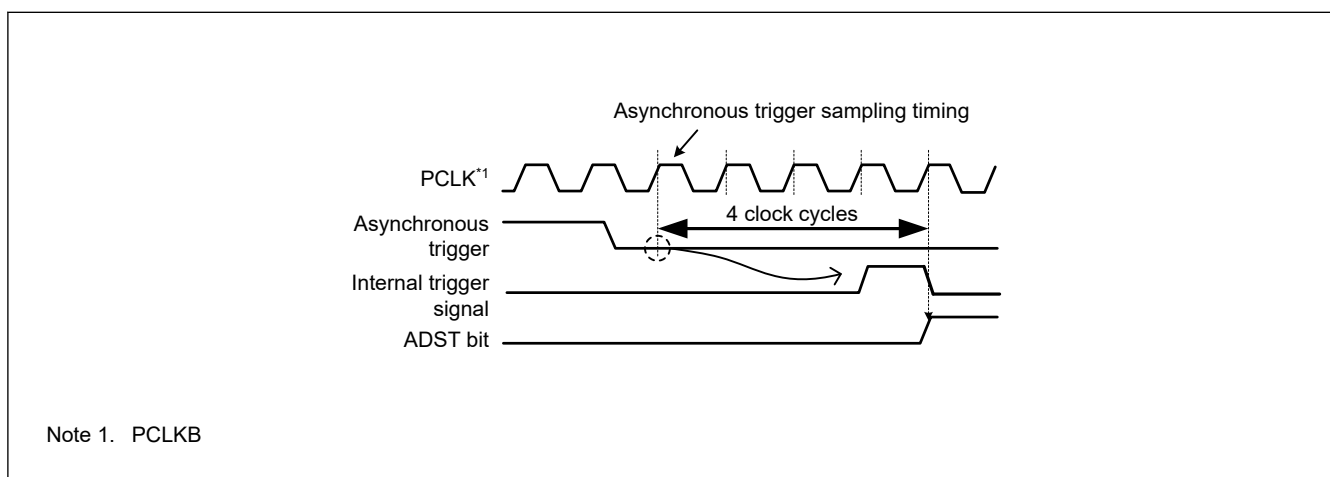
Figure 29.34 Asynchronous trigger input timing
