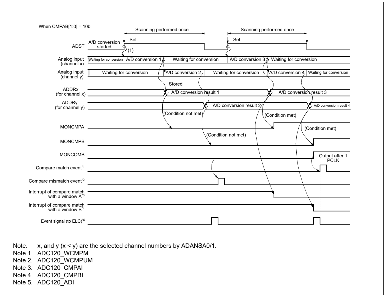
Figure 29.28 Example operation of the compare function event output, when the analog inputs (channel x and y) are compared
