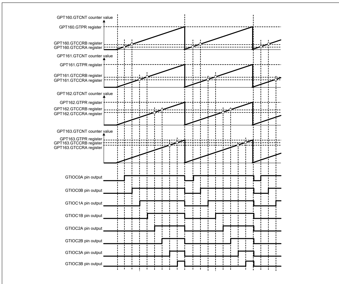
Figure 20.115 Example of synchronized PWM output
