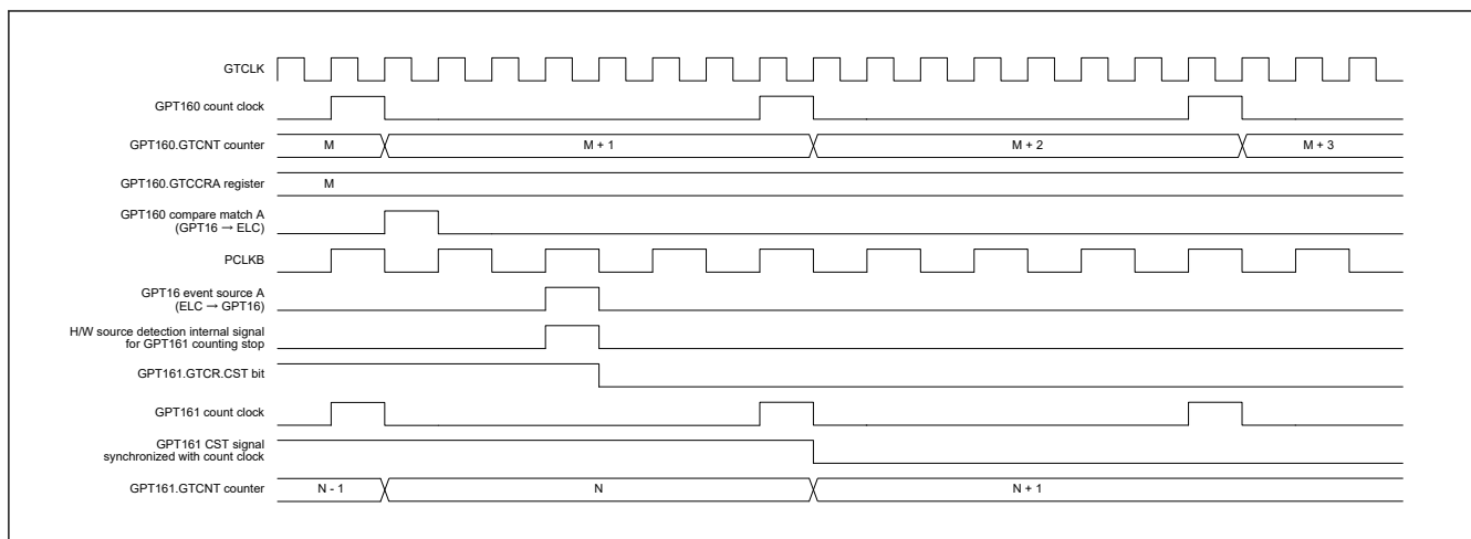
Figure 20.97 Example of timing of operations to stop counting in response to event input from ELC_GPTA
