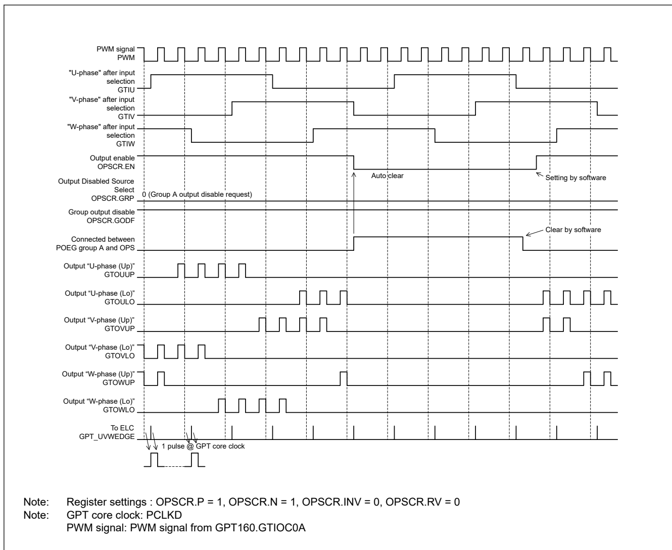
Figure 20.138 Example of group output disable control operation
