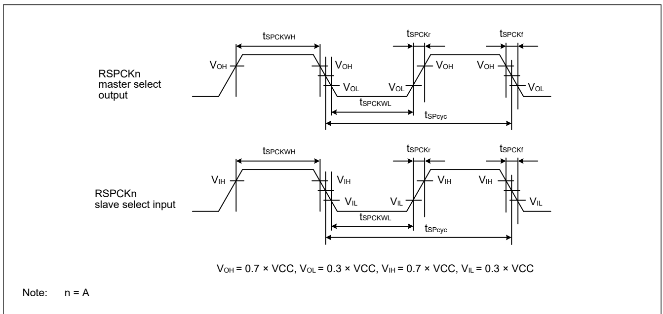
Figure 35.39 SPI clock timing
