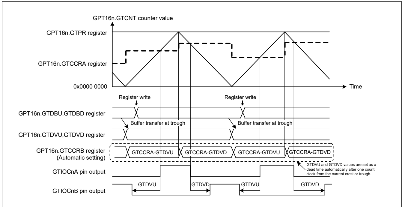
Figure 20.85 Example of automatic compare-match value setting function with dead time in triangle-wave PWM mode 2 or 3, GTDVU and GTDVD set to buffer operation, and active-high in GPT160 to GPT162
