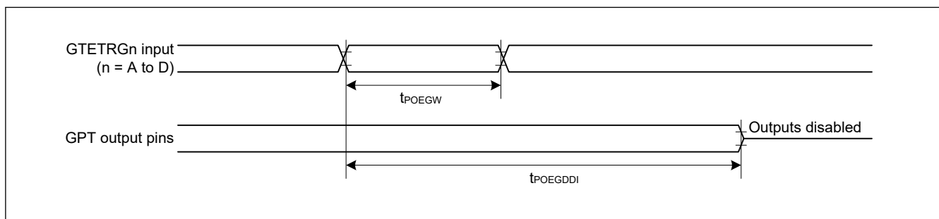
Figure 35.20 Output disable time for POEG in direct response to the input level detection of the GTETRn pin
