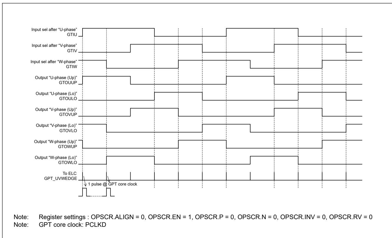
Figure 20.136 Example of 6-phase level output operation
