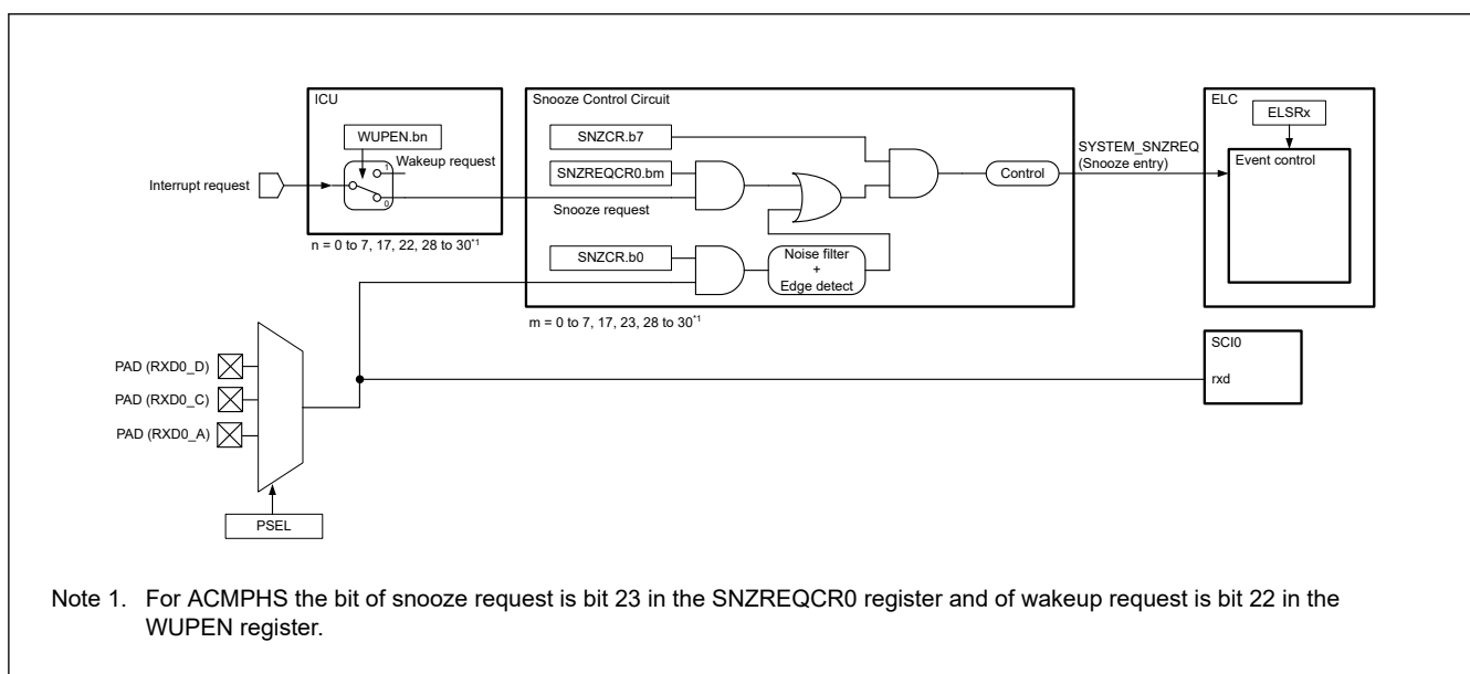
Figure 10.7 Snooze mode entry configuration
