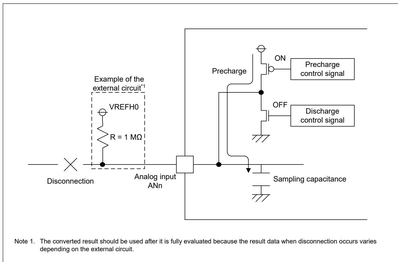
Figure 29.32 Example of disconnection detection when precharge is selected
