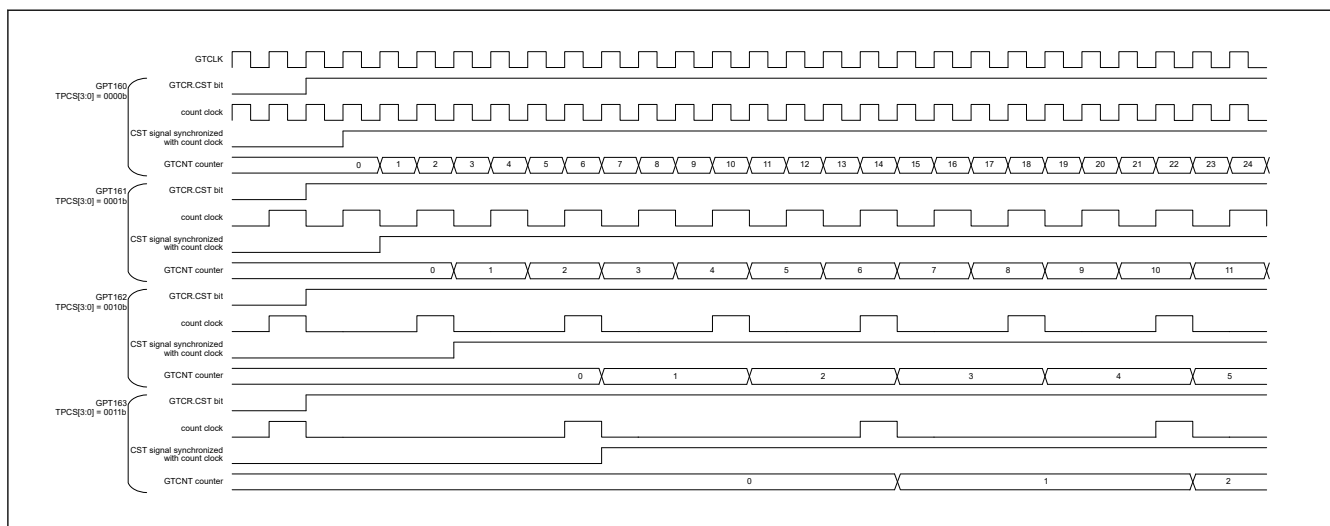
Figure 20.109 Example of simultaneous start operation by software (with different count period)
