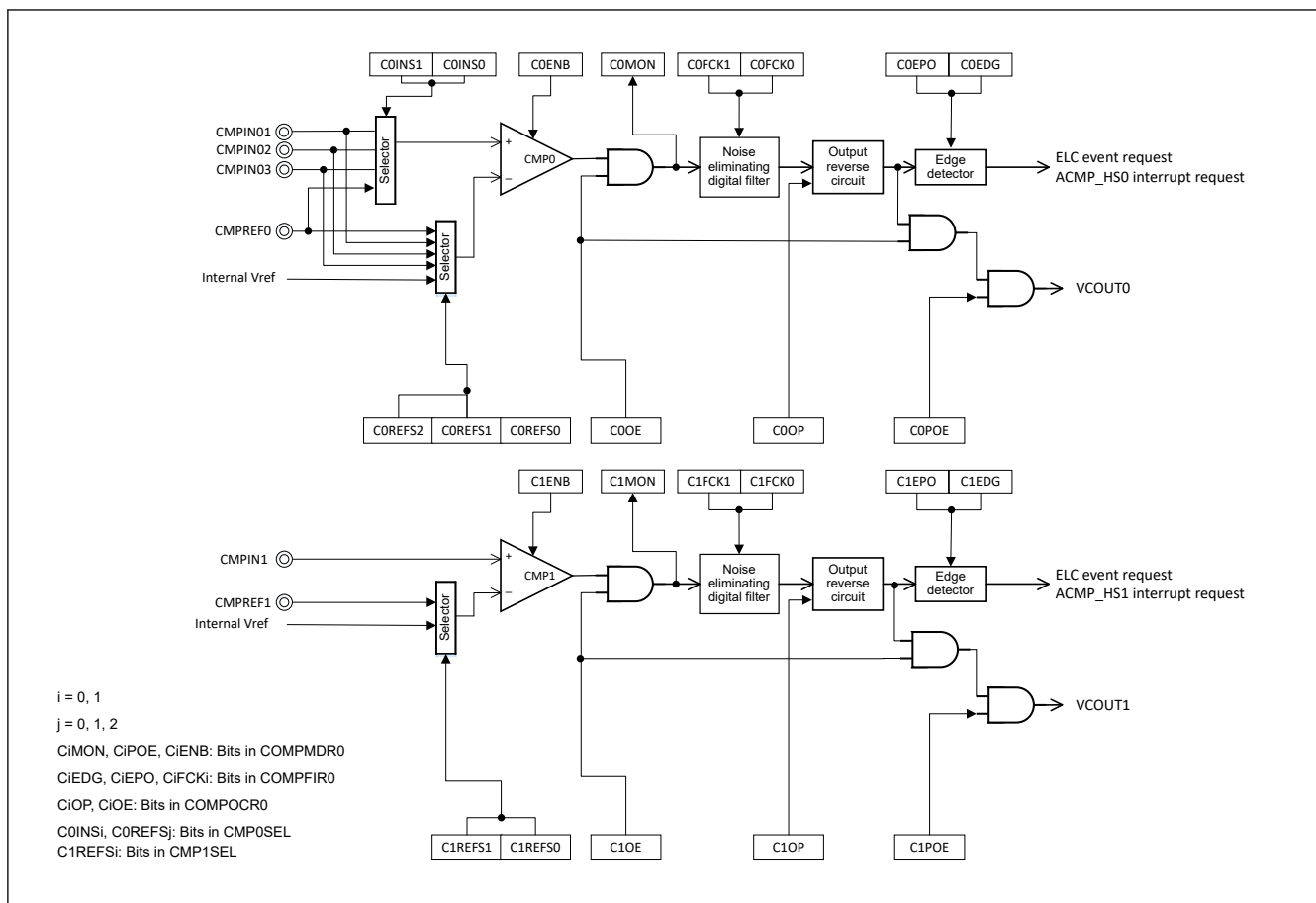
Figure 28.1 ACMPHS block diagram
