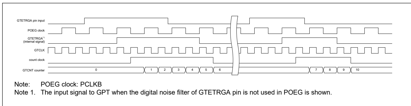
Figure 20.133 Example of external pulse width measuring function (up-counting)
