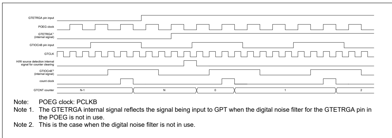
Figure 20.104 Examples of the timing of operations for counter clearing in response to a rising edge of the input on the GTETRGA pin (during counting triggered by hardware source)
