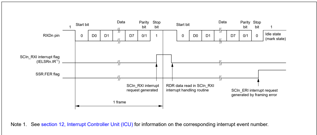
Figure 24.13 Example of SCI operation for serial reception in asynchronous mode (1) when the RTS function is not used, and with 8-bit data, parity bit, and 1 stop bit
