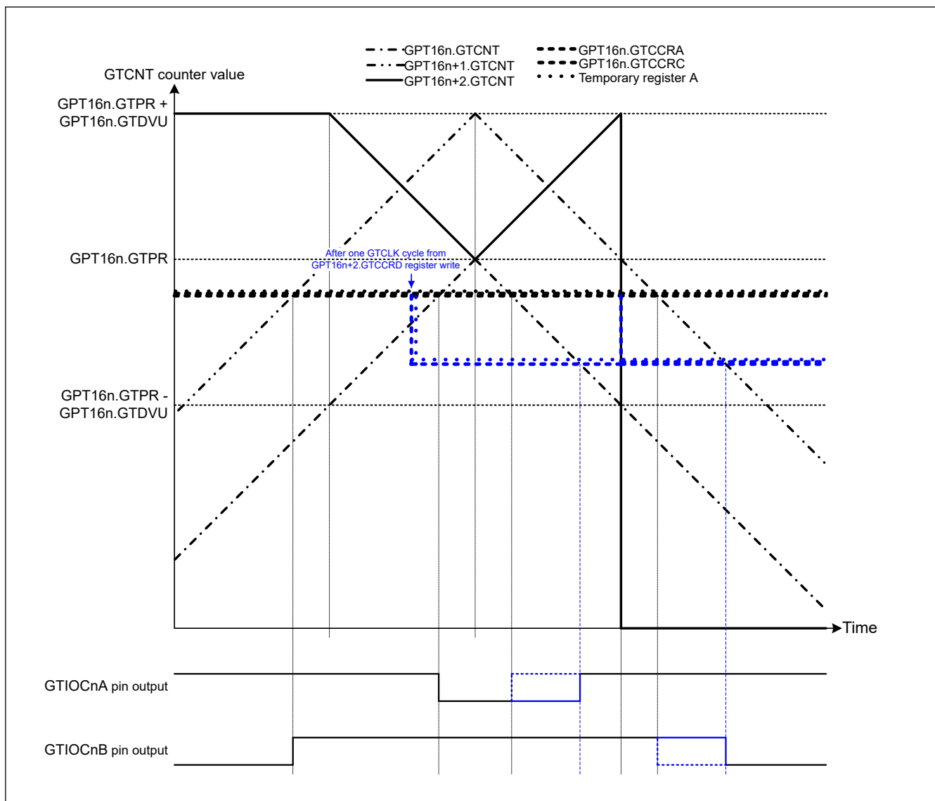
Figure 20.71 Example of complementary PWM mode 4 single buffer operation (up-counting crest section) (complementary PWM mode 4 single buffer operation, GTIOCnA pin = low/GTIOCnB pin = high at GTCCRA register compare match during up-counting, GTIOCnA pin = high/GTIOCnB pin = low at GTCCRA register compare match during down-counting, when a value is written to GTCCRD register during the up-counting dead time) (n = 0)
