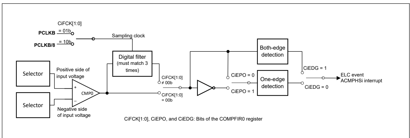
Figure 28.3 Noise filter and edge detection configuration
