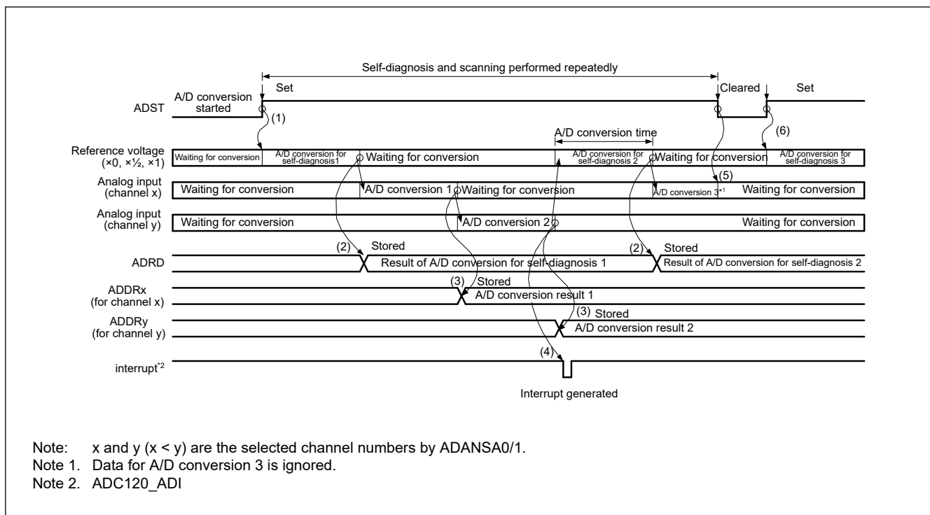
Figure 29.16 Example basic operation in continuous scan mode when the analog inputs (channel x and y) are selected with self-diagnosis
