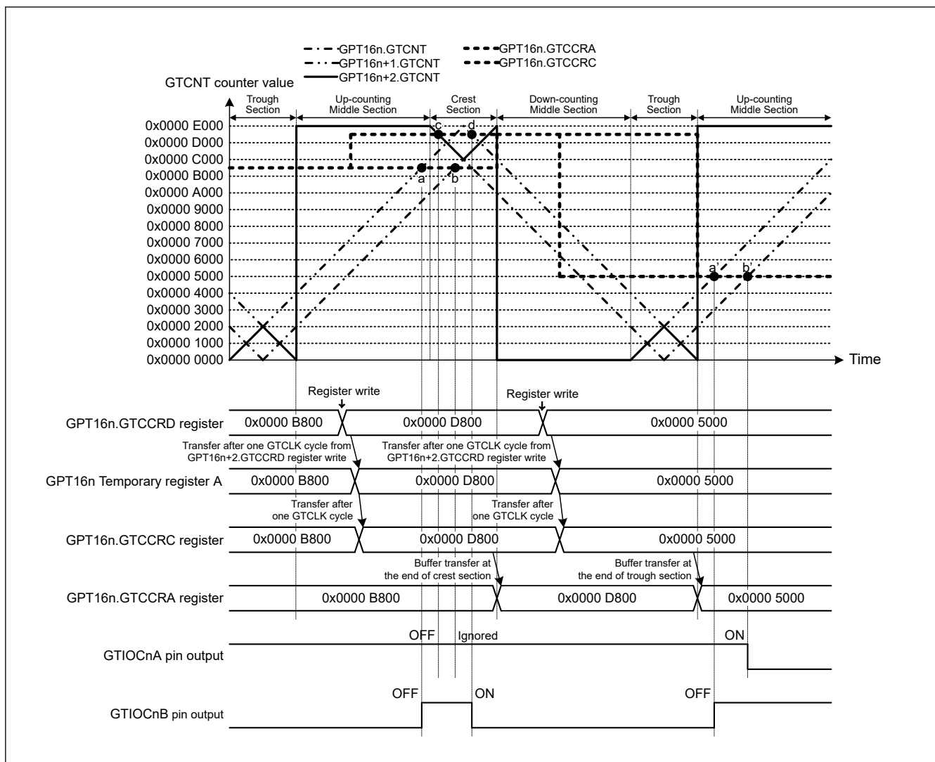
Figure 20.57 Example of compare match generation sequence operation in complementary PWM mode (complementary PWM mode 3 single buffer operation, GTIOCnA pin = low/GTIOCnB pin = high at GTCCRA register compare match during up-counting, GTIOCnA pin = high/GTIOCnB pin = low at GTCCRA register compare match during down-counting, the dead time value is 0x0000 2000, compare match generation order: a → c → b → d) (n = 0)
