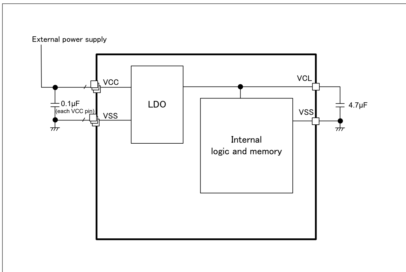
Figure 34.1 LDO settings
