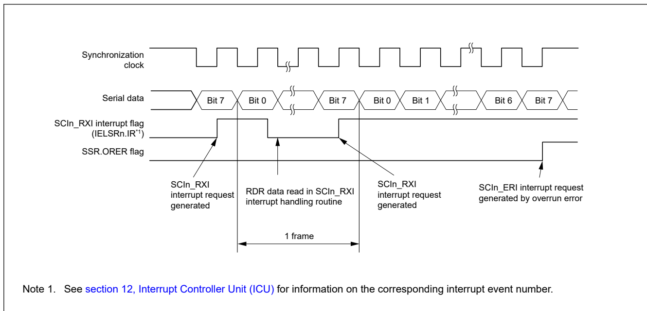
Figure 24.41 Example operation for serial reception in clock synchronous mode (1) when the RTS function is not used
