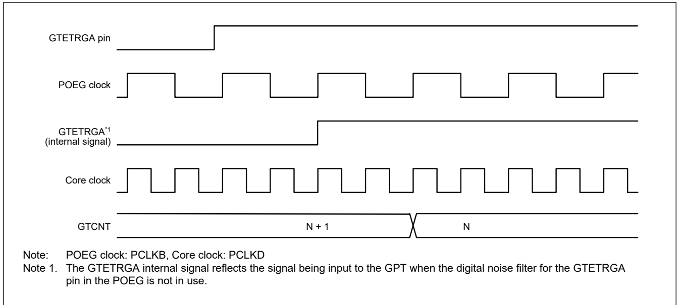
Figure 20.9 Example of event count operation in down-counting using hardware sources
