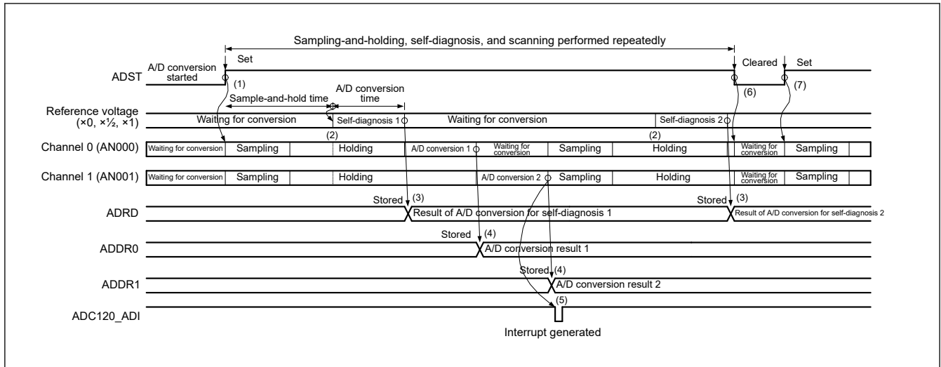
Figure 29.17 Example operation in continuous scan mode when channel-dedicated sample-and-hold circuits are used and AN000 and AN001 are selected with self-diagnosis
