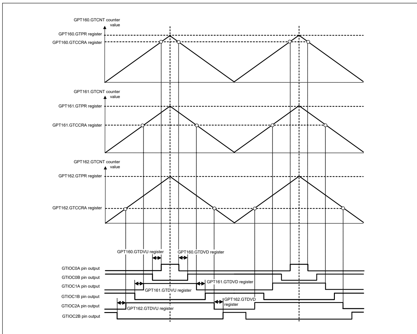
Figure 20.119 Example of 3-phase triangle-wave complementary PWM output with automatic dead time setting
