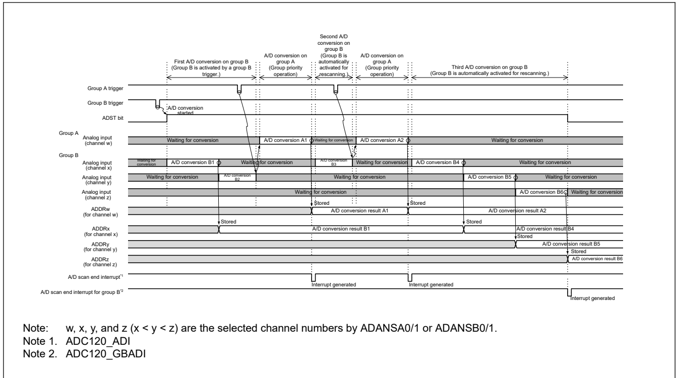
Figure 29.22 Example of group priority operation 1-2: Group A trigger input during rescanning of group B when rescanning is enabled (when ADGSPCR.GBRSCN = 1, ADGSPCR.GBRP = 0)
