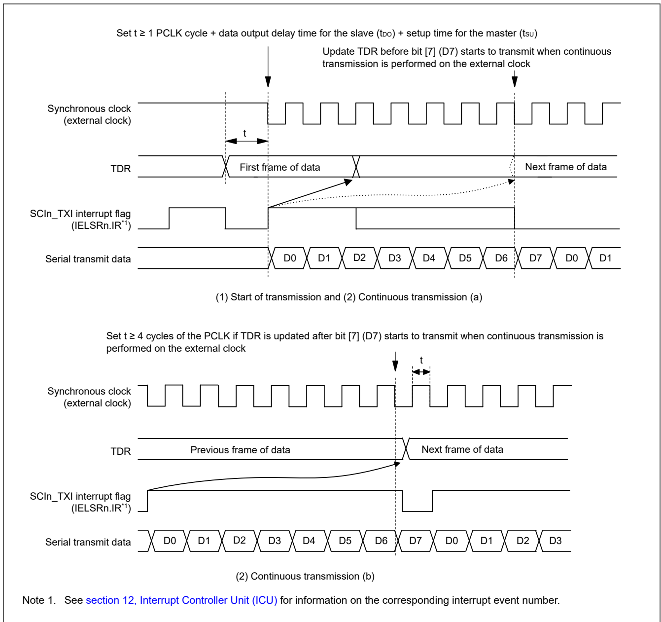
Figure 24.77 Restraints on use of external clock in clock synchronous transmission
