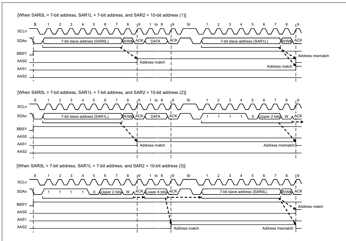
Figure 25.26 AASy flag set and clear timing with mixed 7-bit and 10-bit address formats
