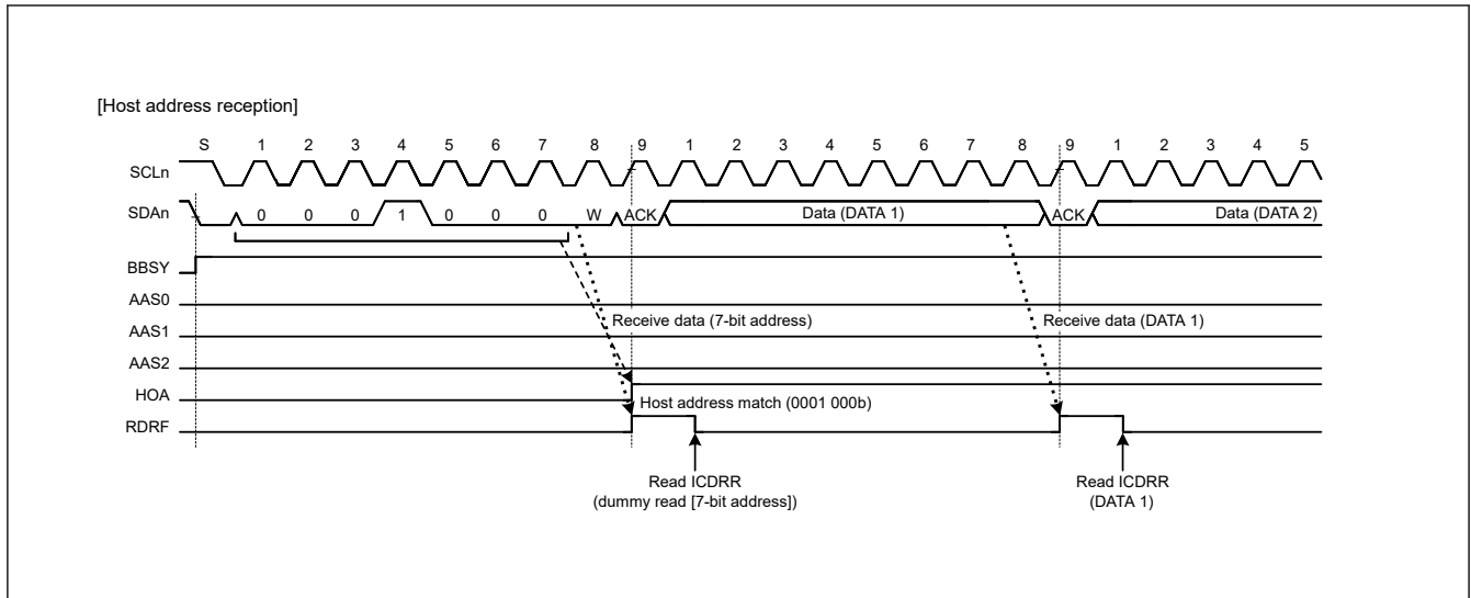
Figure 25.29 HOA flag set timing during reception of host address
