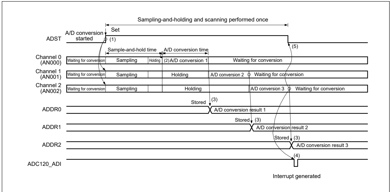
Figure 29.8 Example operation in single scan mode when the channel-dedicated sample-and-hold circuits are used and AN000 to AN002 are selected
