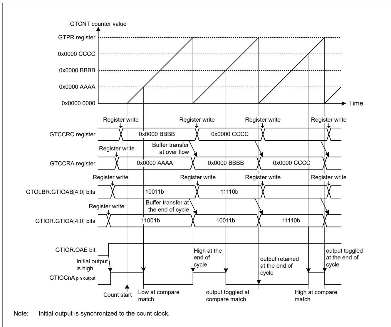
Figure 20.35 Example of buffer operation of the GTIOA and GTIOB bits (up-counting in saw-wave PWM mode 1, buffer transfer at the end of cycle)
