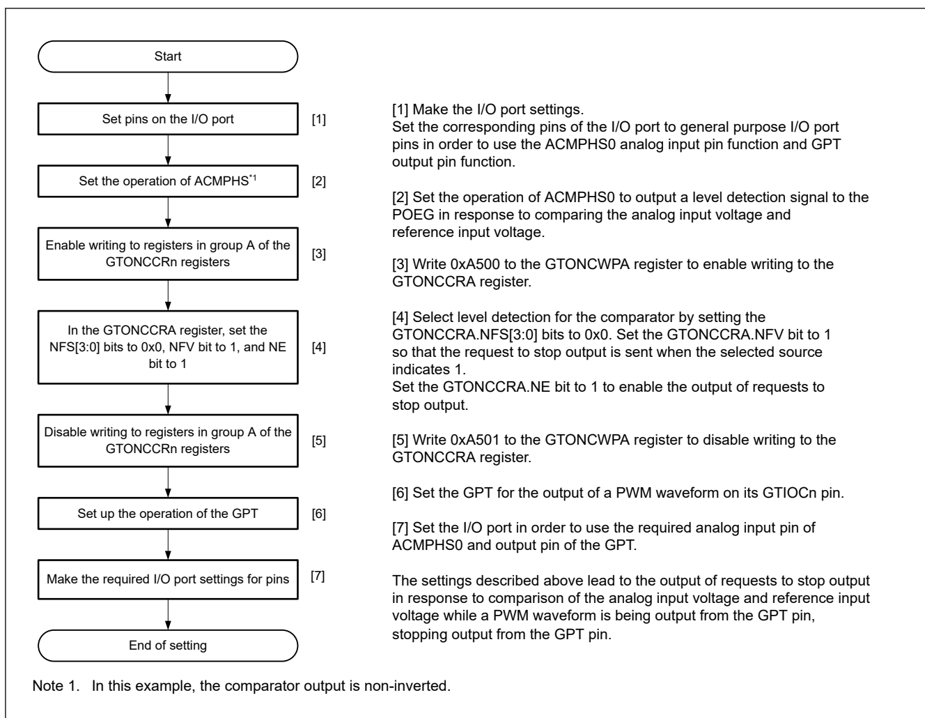
Figure 19.5 Example of Settings to Stop Output on the GTIOC Pin in Response to Level Detection by a Comparator
