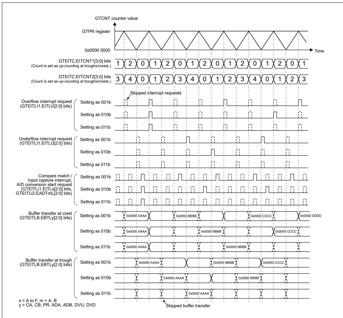
Figure 20.151 Example of extended interrupt skipping function operation (triangle-waves, counting both crests and troughs, extended interrupt skipping 1 skipping count: 2, counting both crests and troughs, extended interrupt skipping 2 skipping count: 4, extended interrupt skipping counter 2 initial value: 0, skipped in the period other than GTEITC.EITCNTk bits (k = 1, 2) as 0)
