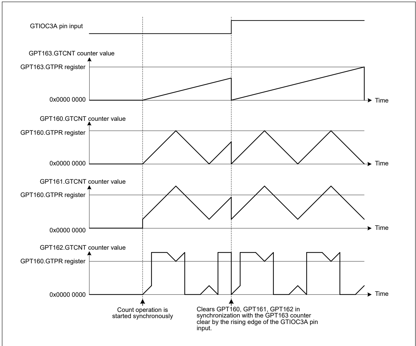
Figure 20.113 Example of synchronous clear operation by inter channel cooperation (clear caused by GTIOCN A /GTIOCN B pin) (GPT163 is saw-wave and counter is cleared by the rising edge of the GTIOC3A, GPT160, 1, 2 are complementary PWM mode. GPT160, 1, 2, 3 are the same synchronous set/clear group)
