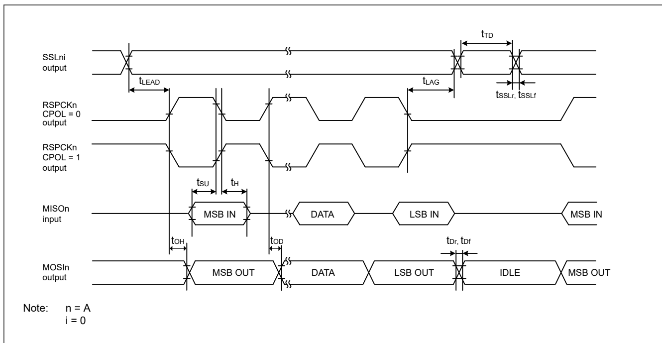
Figure 35.42 SPI timing (master, CPHA = 1) (bit rate: PCLKB division ratio is set to any value other than 1/2)
