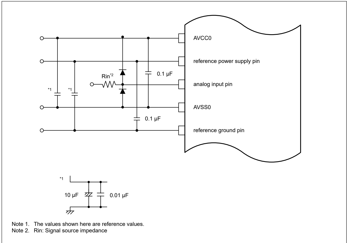
Figure 29.37 Example protection circuit for analog inputs
