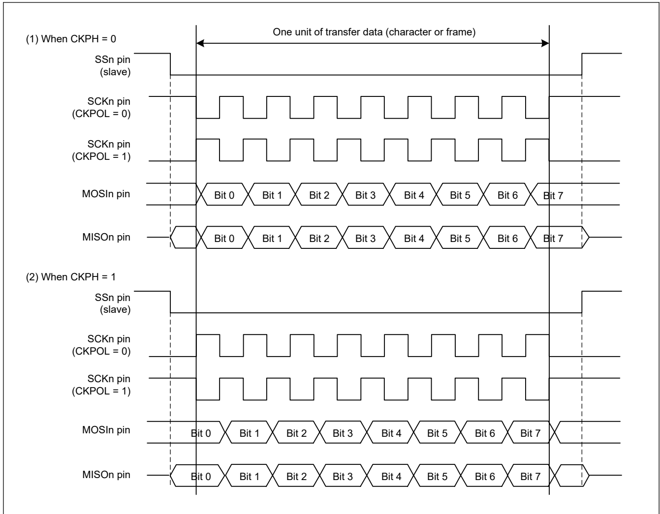
Figure 24.69 Relation between clock signal and transmit or receive data in simple SPI mode
