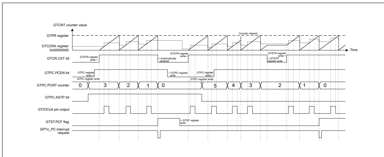
Figure 20.121 Example of PWM cycle count function (saw-wave one-shot pulse mode)
