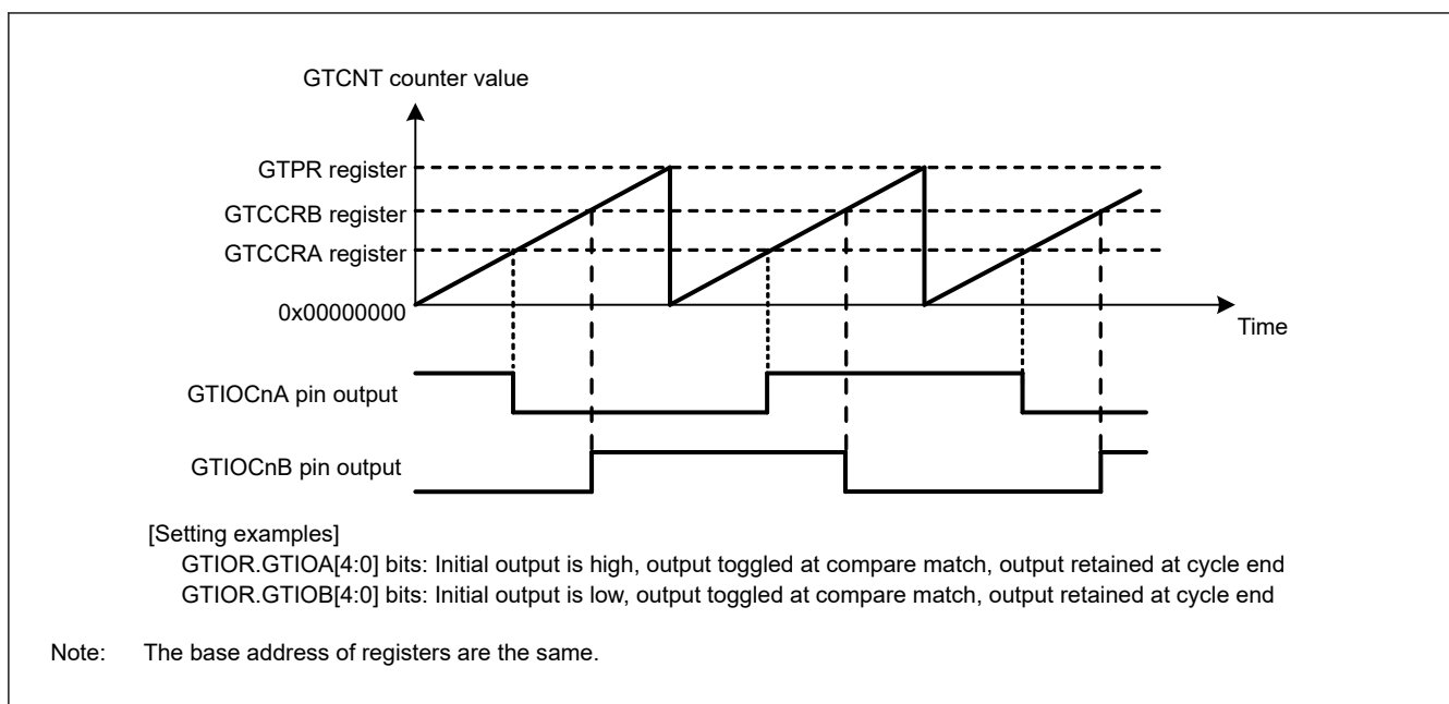
Figure 20.11 Example of toggled output operation (1)
