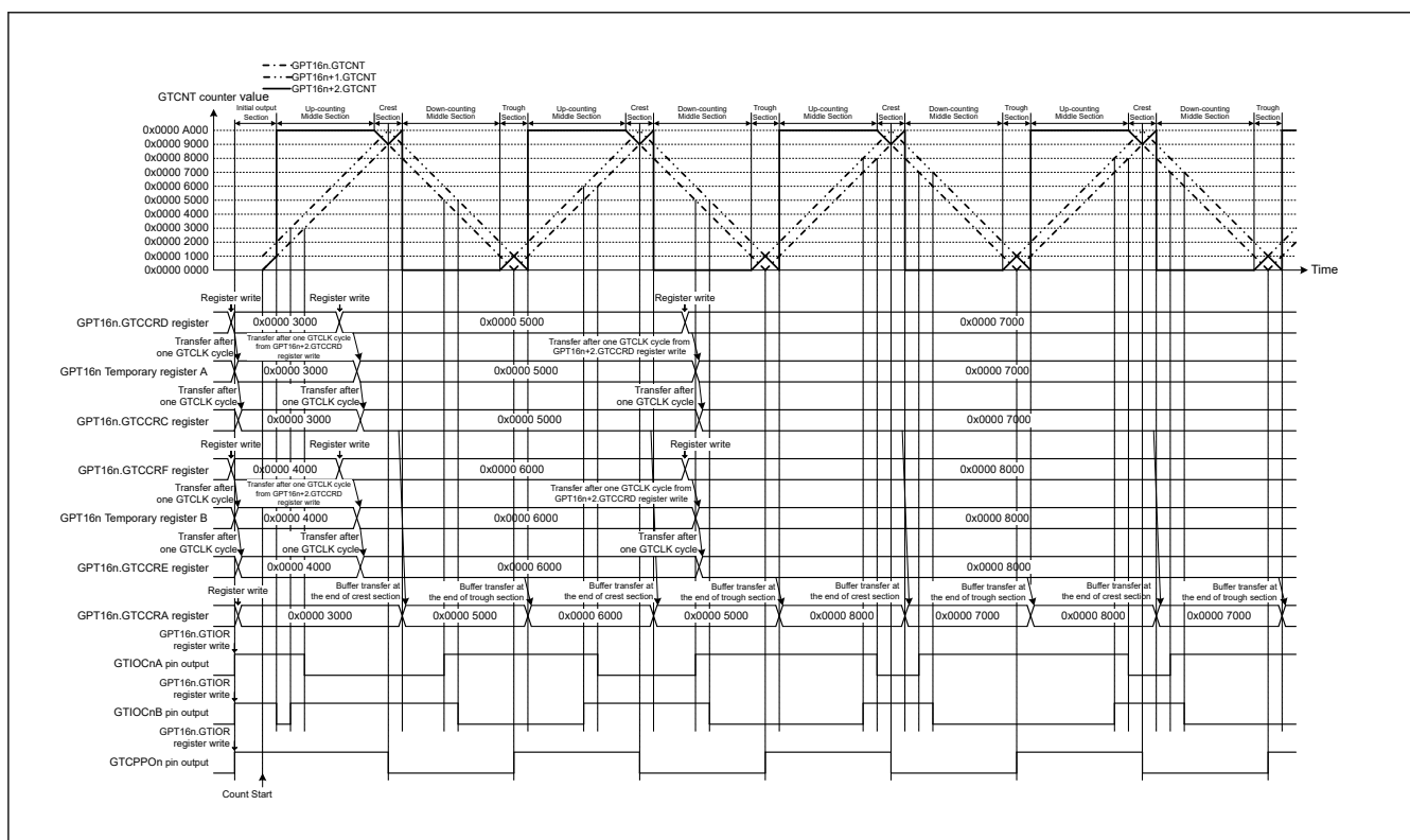
Figure 20.53 Example of complementary PWM mode 3 operation (double buffer operation, GTIOCnA pin = high/GTIOCnB pin = high as initial output, GTIOCnA pin = low/GTIOCnB pin = high at GTCCRA register compare match during up-counting, GTIOCnA pin = high/GTIOCnB pin = low at GTCCRA register compare match during down-counting, the dead time value is 0x0000 1000 and updating GTCRD register in middle section) (n = 0)
