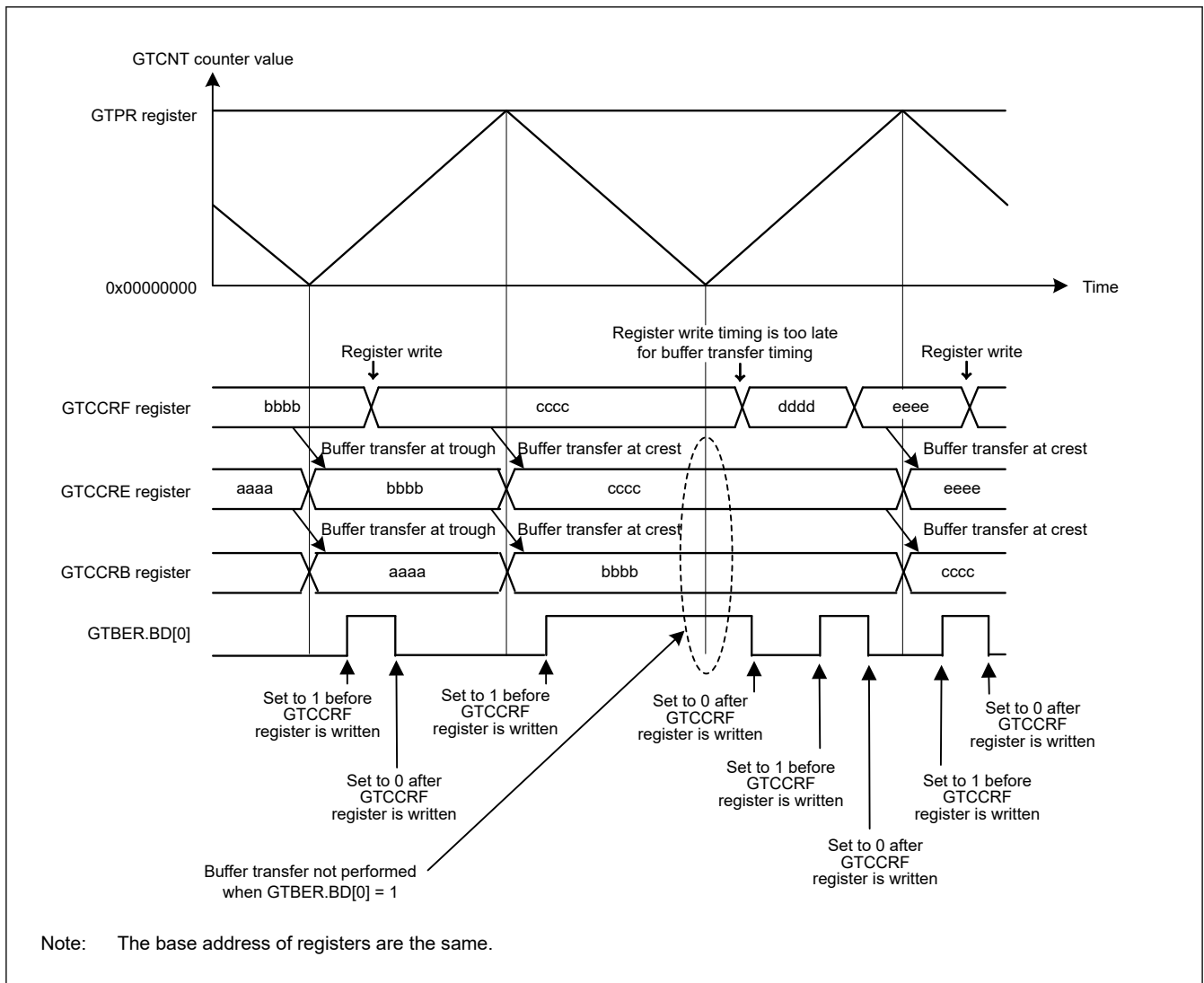
Figure 20.163 Example of operation for disabling buffer operation with triangle waves, double buffer operation, and buffer transfer at both troughs and crests
