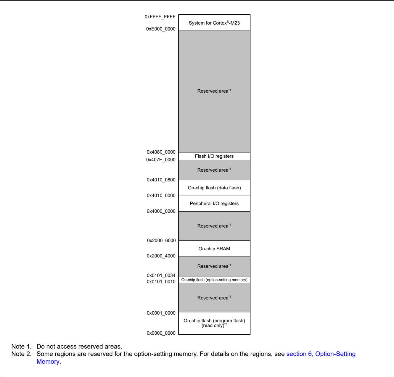
Figure 4.1 Memory map
