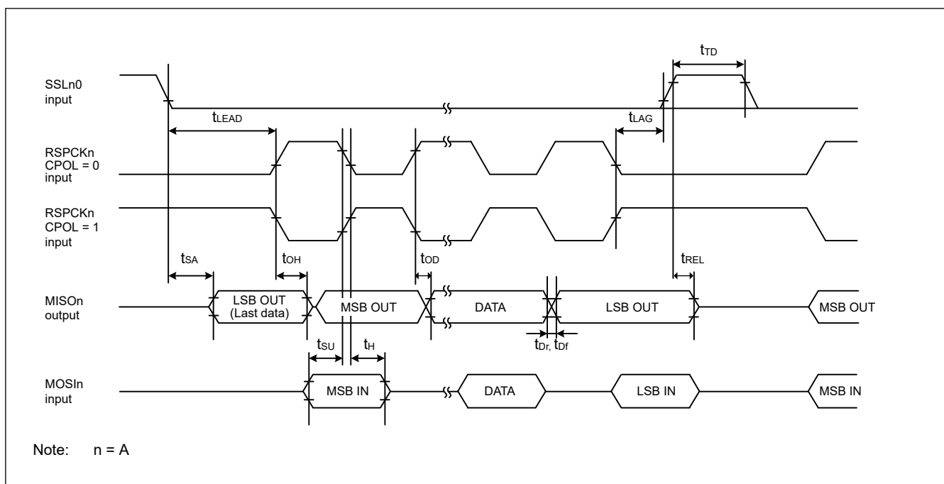
Figure 35.45 SPI timing (slave, CPHA = 1)
