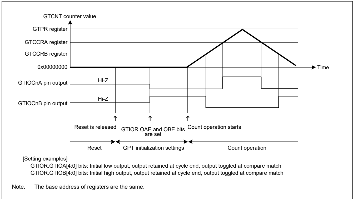
Figure 20.181 Example of pin settings after reset
