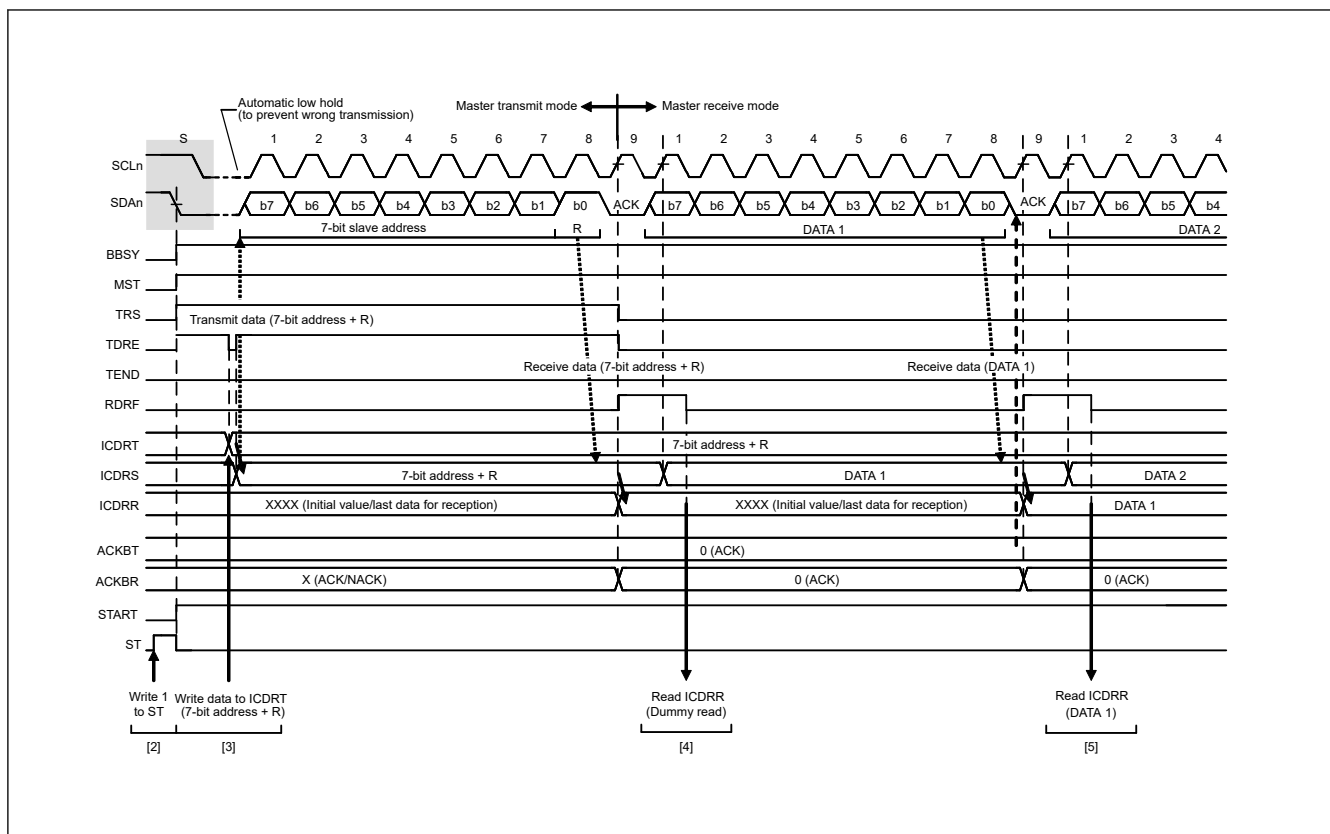
Figure 25.12 Master receive operation timing (1) with 7-bit address format when RDRFS = 0
