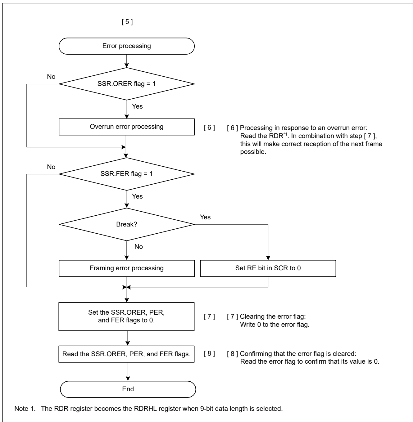
Figure 24.32 Example flow of multi-processor serial reception with non-FIFO selected (2)
