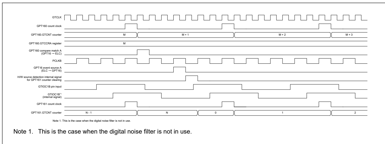
Figure 20.106 Examples of the timing of operations for counter clearing in response to event input from the ELC_GPTA (during counting triggered by hardware source)
