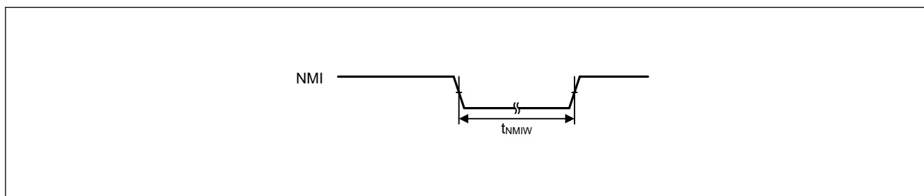
Figure 35.11 NMI interrupt input timing
