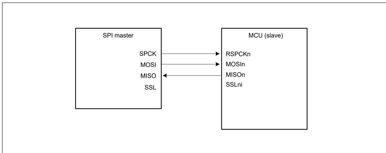
Figure 26.11 Clock synchronous master/slave configuration example with the MCU as a slave and CPHA = 1
