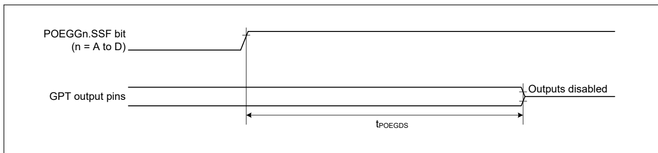
Figure 35.18 Output disable time for POEG in response to the register setting
