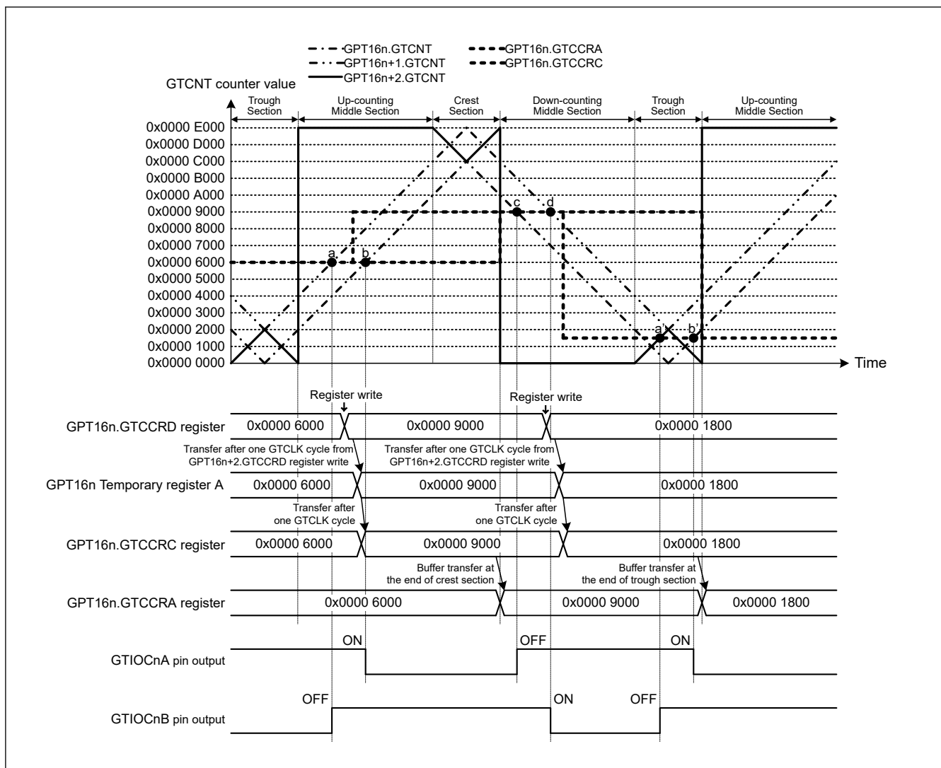
Figure 20.61 Example of compare match generation sequence operation in complementary PWM mode (complementary PWM mode 3 single buffer operation, GTIOCnA pin = low/GTIOCnB pin = high at GTCCRA register compare match during up-counting, GTIOCnA pin = high/GTIOCnB pin = low at GTCCRA register compare match during down-counting, the dead time value is 0x0000 2000, compare match generation order: c → d → a' → b') (n = 0)
