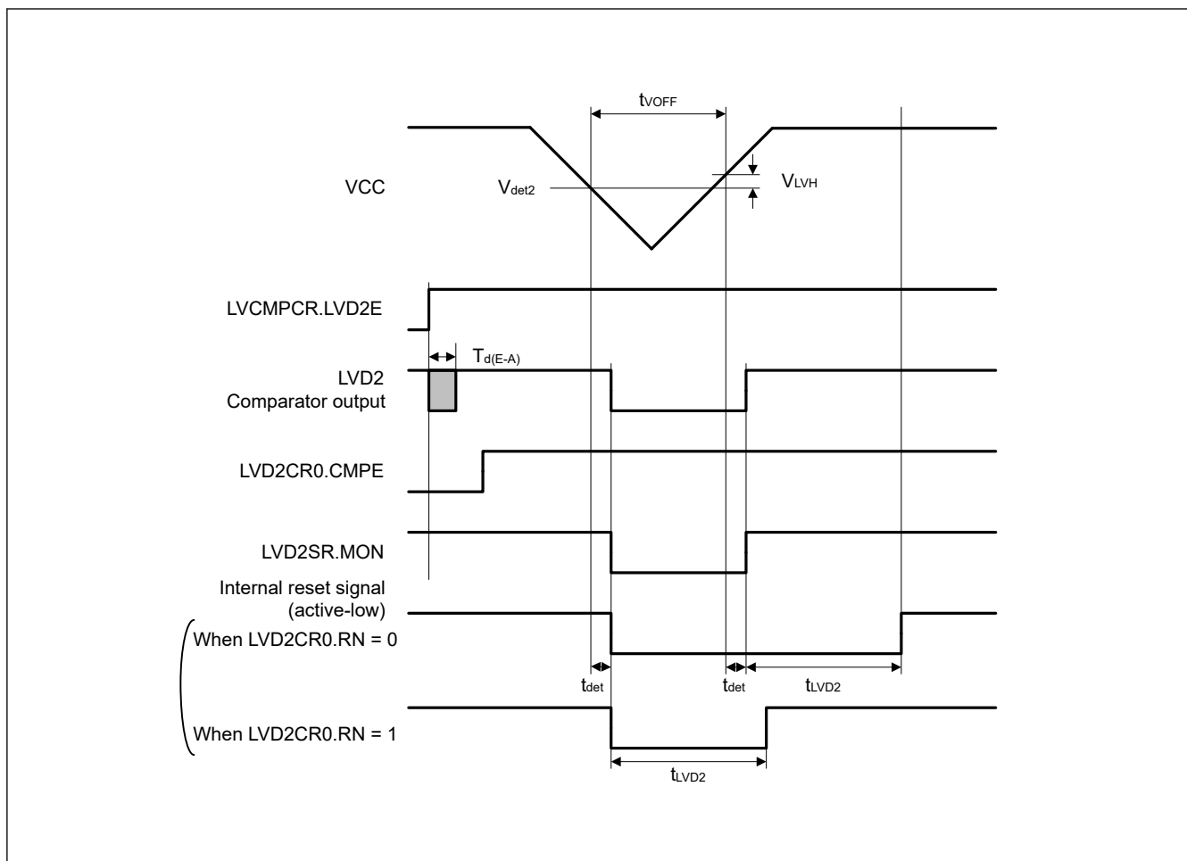
Figure 35.56 Voltage detection circuit timing ( V_{det2} )
