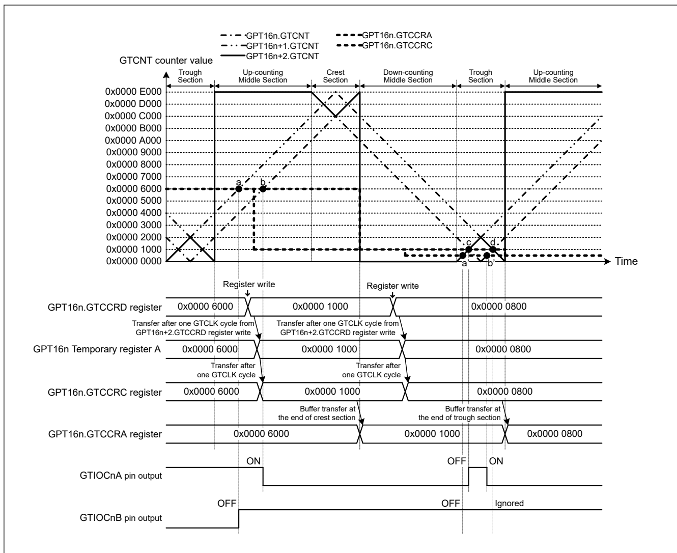
Figure 20.65 Example of compare match generation sequence operation in complementary PWM mode (complementary PWM mode 3 single buffer operation, GTIOCnA pin = low/GTIOCnB pin = high at GTCCRA register compare match during up-counting, GTIOCnA pin = high/GTIOCnB pin = low at GTCCRA register compare match during down-counting, the dead time value is 0x0000 2000, compare match generation order: a' → c → b' → d) (n=0)
