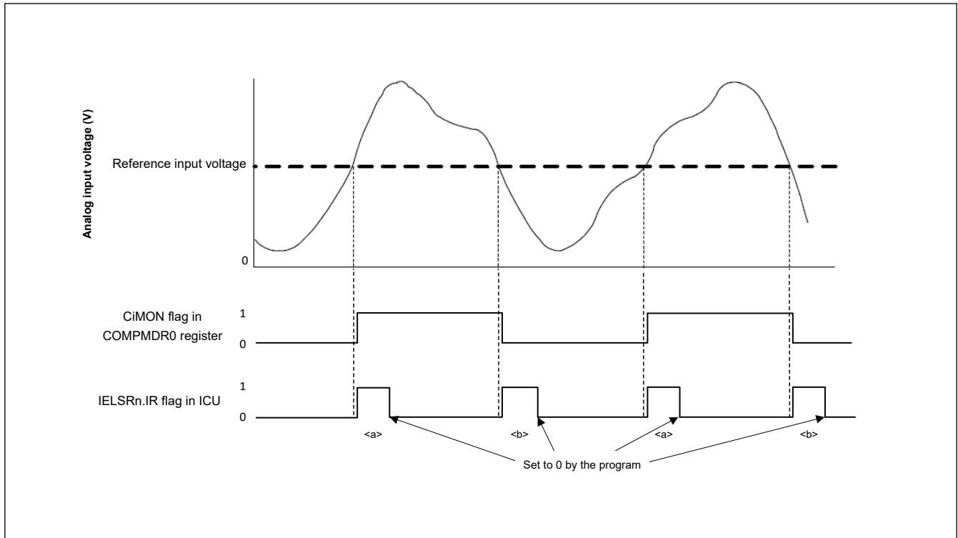
Figure 28.2 ACMPHS operation example
