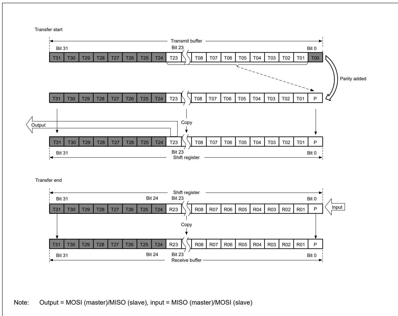
Figure 26.18 MSB-first transfer with 24-bit data and parity enabled
