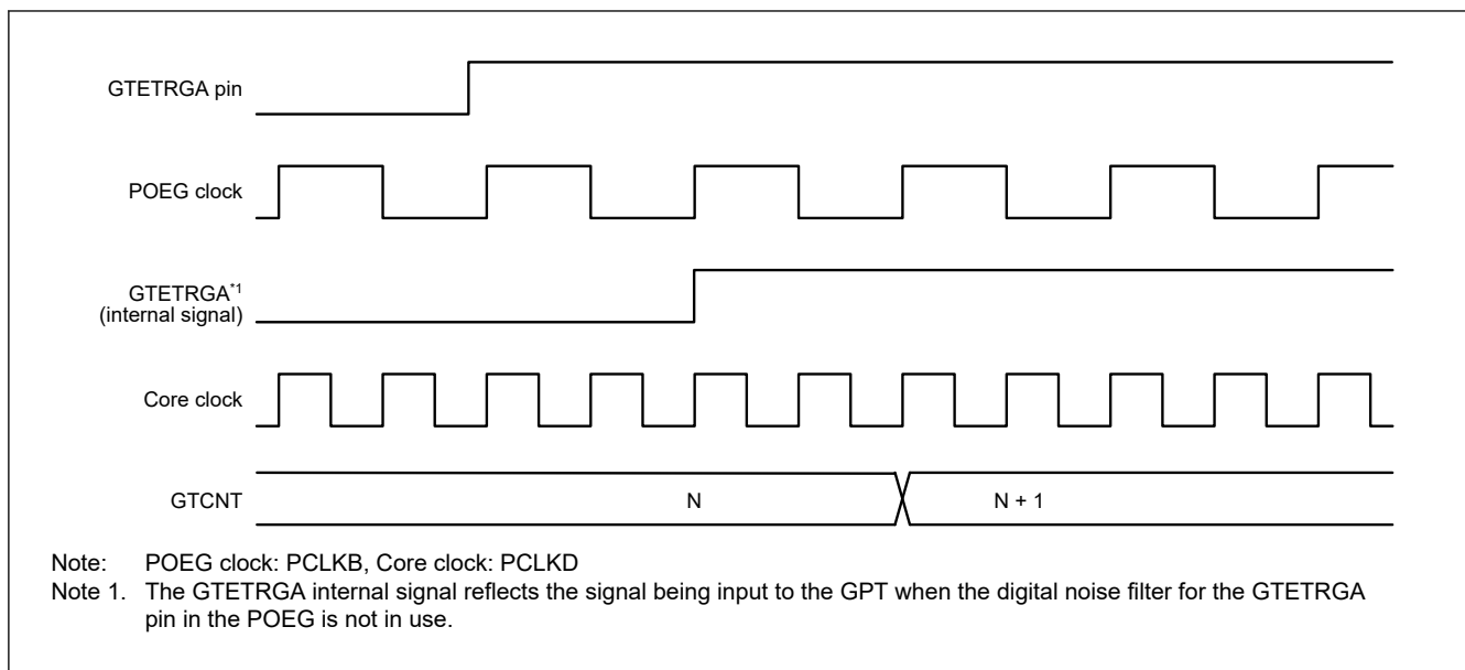
Figure 20.6 Example of event count operation in up-counting using hardware sources
