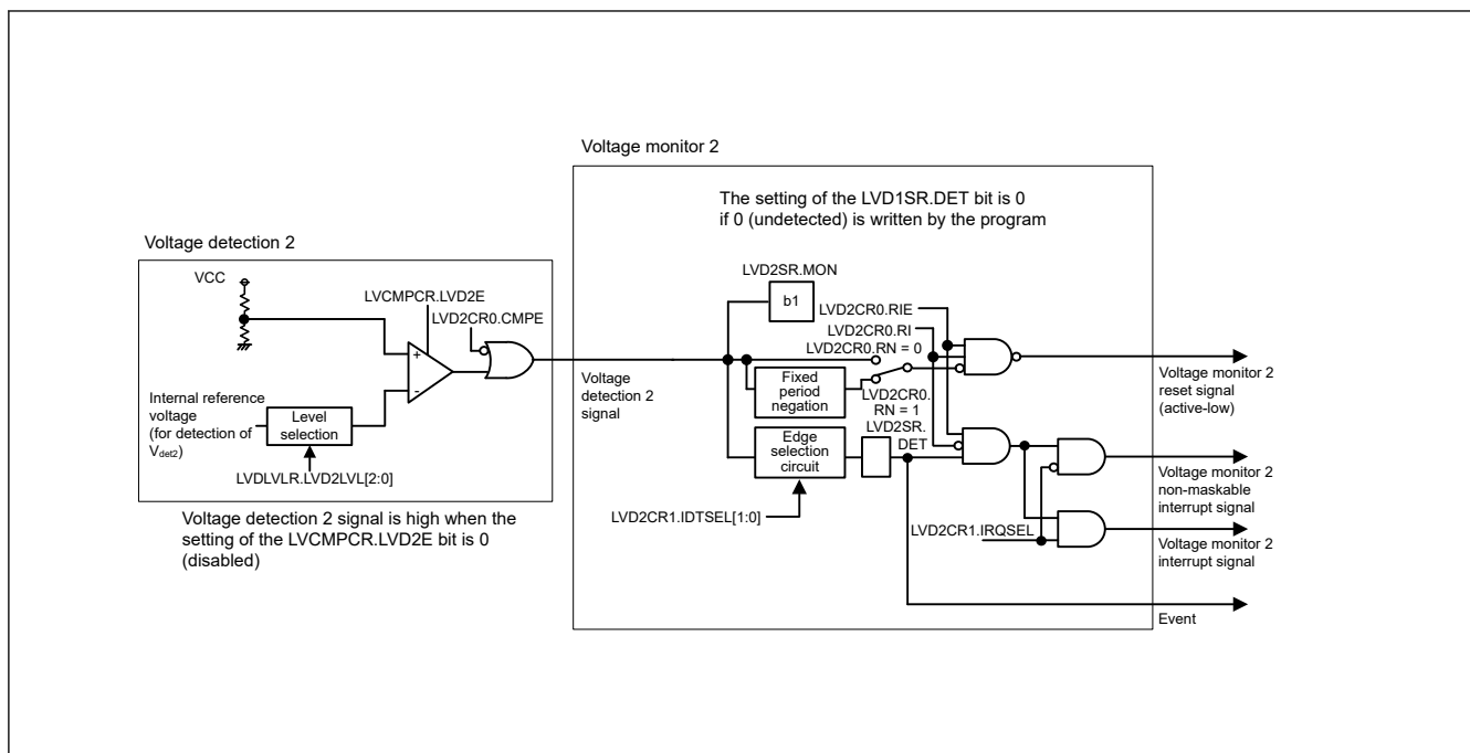
Figure 7.3 Block diagram of voltage monitor 2 interrupt and reset circuit
