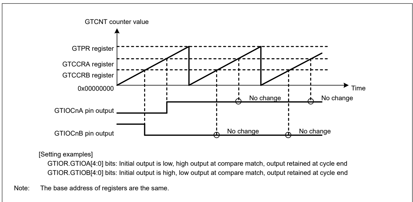
Figure 20.10 Example of low output and high output operation
