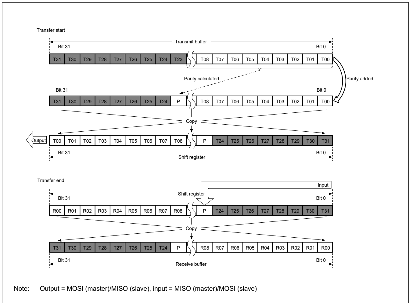
Figure 26.20 LSB-first transfer with 24-bit data and parity enabled
