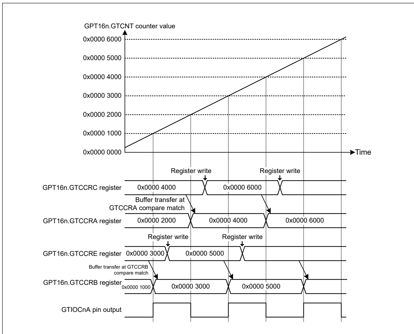
Figure 20.39 Example of saw-wave PWM mode 2 operation (low output at GTCCRA register compare match, high output at GTCCRB register compare match, single buffer operation, no clear setting) (n = 0 to 2)
