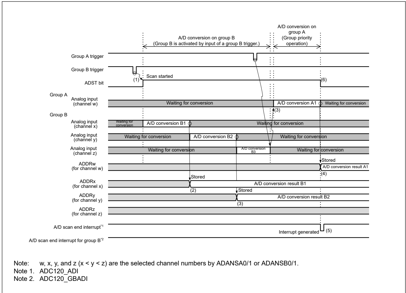
Figure 29.24 Group priority operation example 1-4: “Group A trigger is input during group B scan” when rescanning is disabled (when ADGSPCR.GBRSCN = 0, ADGSPCR.GBRP = 0)
