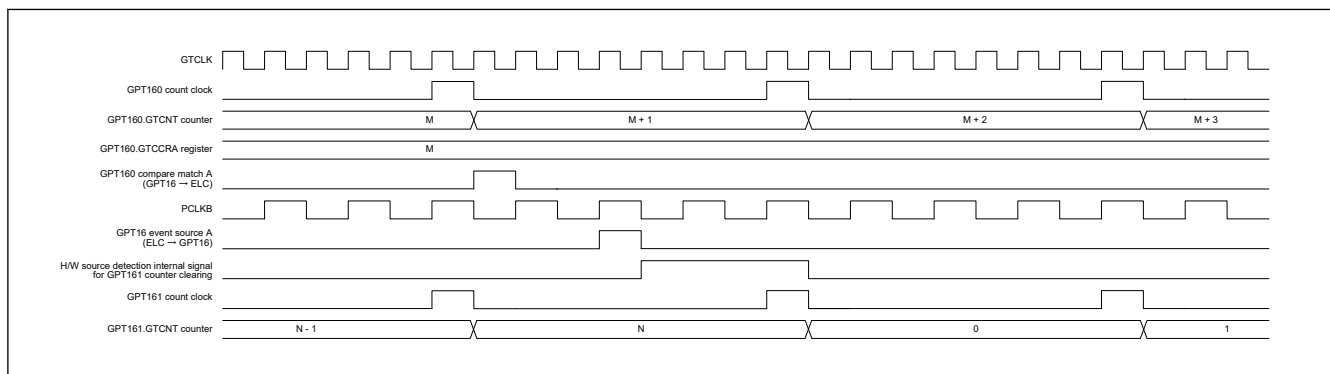
Figure 20.103 Examples of timing of operations for counter clearing in response to event input from the ELC_GPTA (during the counting of cycles of clock signal produced by dividing the GTCLK frequency)
