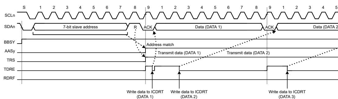
Figure 25.24 AASy flag set timing with 7-bit address format
