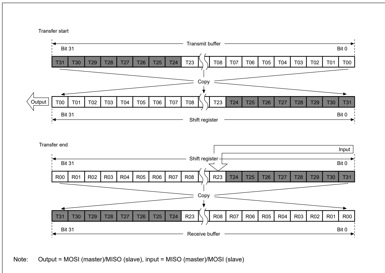
Figure 26.16 LSB-first transfer with 24-bit data and parity disabled
