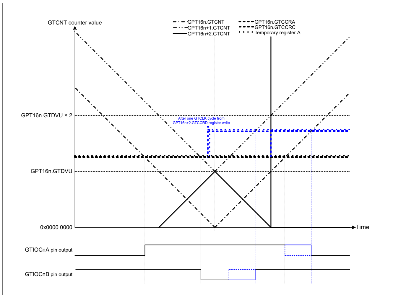
Figure 20.74 Example of complementary PWM mode 4 single buffer operation (down-counting trough section) (complementary PWM mode 4 single buffer operation, GTIOCnA pin = low/GTIOCnB pin = high at GTCCRA register compare match during up-counting, GTIOCnA pin = high/GTIOCnB pin = low at GTCCRC register compare match during down-counting, when a value larger than the GPT16n+2.GTCNT value is written to GTCCRD register after down-counting compare match) (n = 0)
