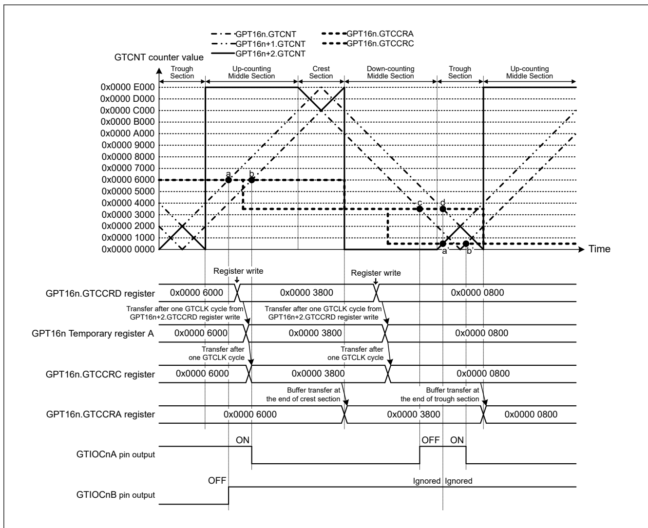
Figure 20.63 Example of compare match generation sequence operation in complementary PWM mode (complementary PWM mode 3 single buffer operation, GTIOCnA pin = low/GTIOCnB pin = high at GTCCRA register compare match during up-counting, GTIOCnA pin = high/GTIOCnB pin = low at GTCCRA register compare match during down-counting, the dead time value is 0x0000 2000, compare match generation order: c → a' → d → b' (n = 0))
