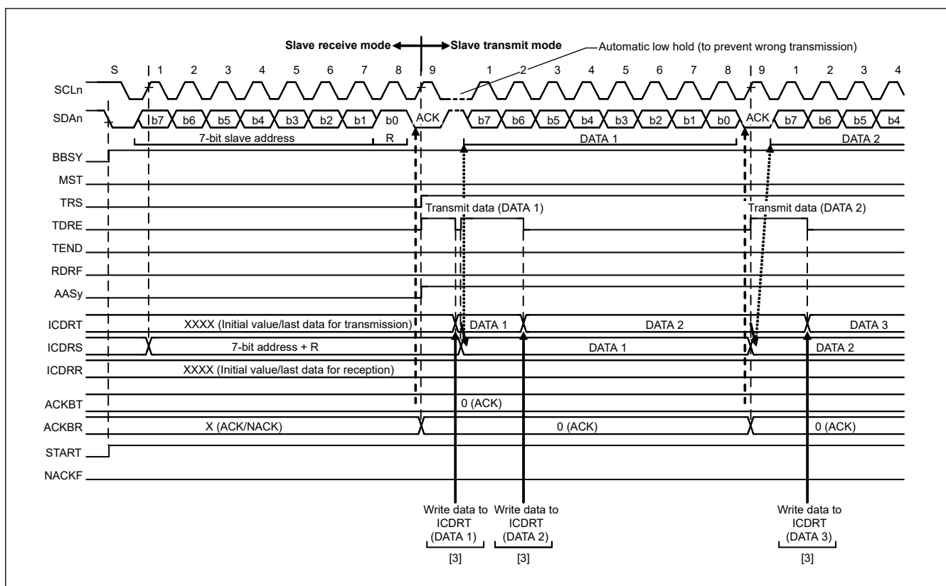
Figure 25.16 Slave transmit operation timing (1) with 7-bit address format
