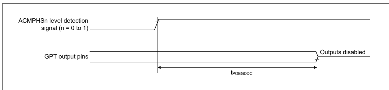
Figure 35.21 Output disable time for POEG in response to level detection signal from ACPHn
