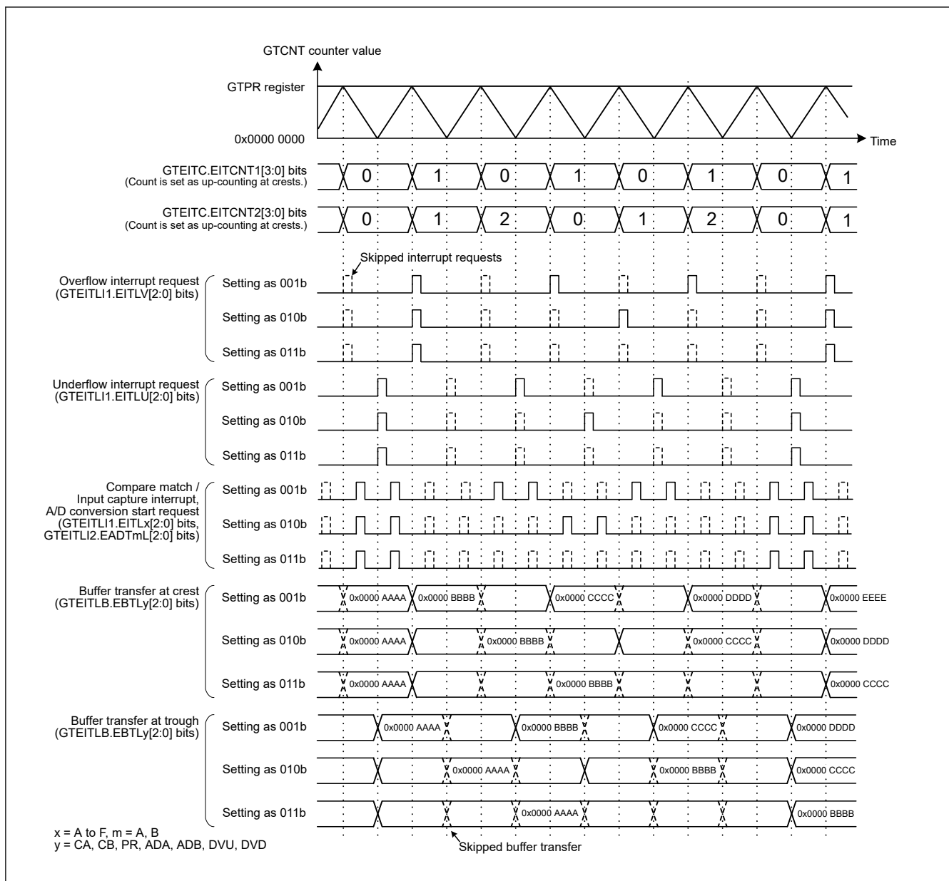
Figure 20.149 Example of extended interrupt skipping function operation (triangle-waves, counting crests, extended interrupt skipping 1 skipping count: 1, counting crests, extended interrupt skipping 2 skipping count: 2, extended interrupt skipping counter 2 initial value: 0, skipped in the period other than GTEITC.EITCNTk bits (k = 1, 2) as 0)
