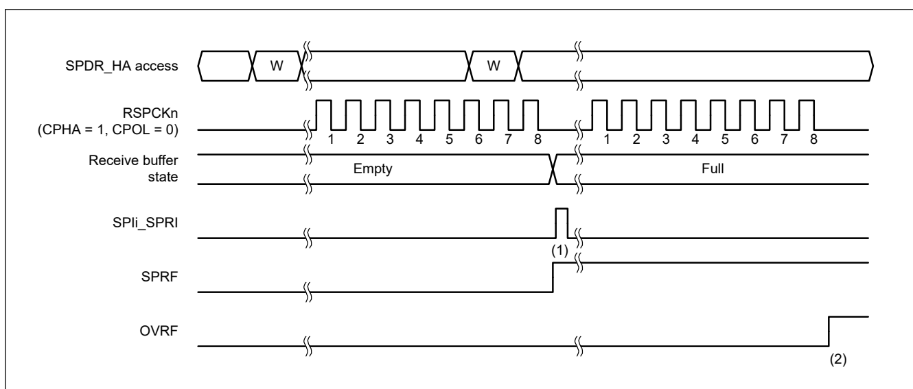
Figure 26.23 Operation example when SPCR.TXMD = 0
