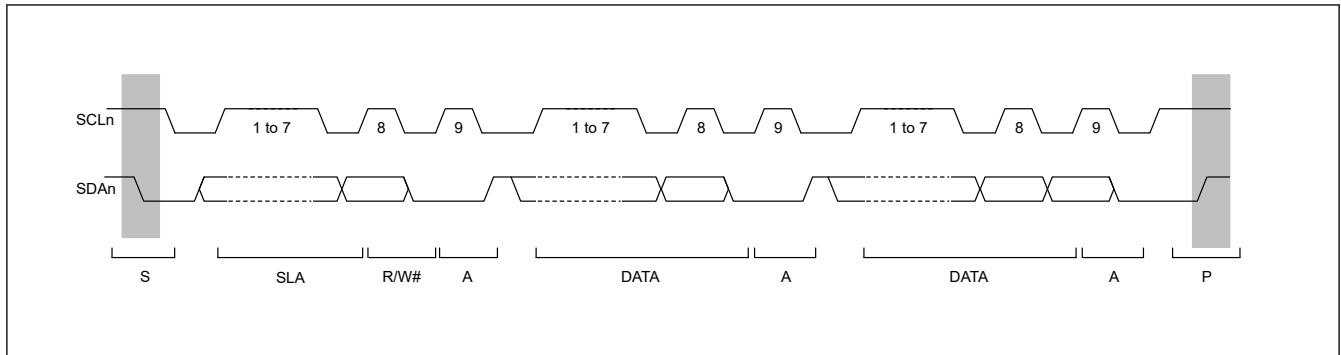
Figure 25.4 I 2 C bus timing when the SLA setting = 7 bits
