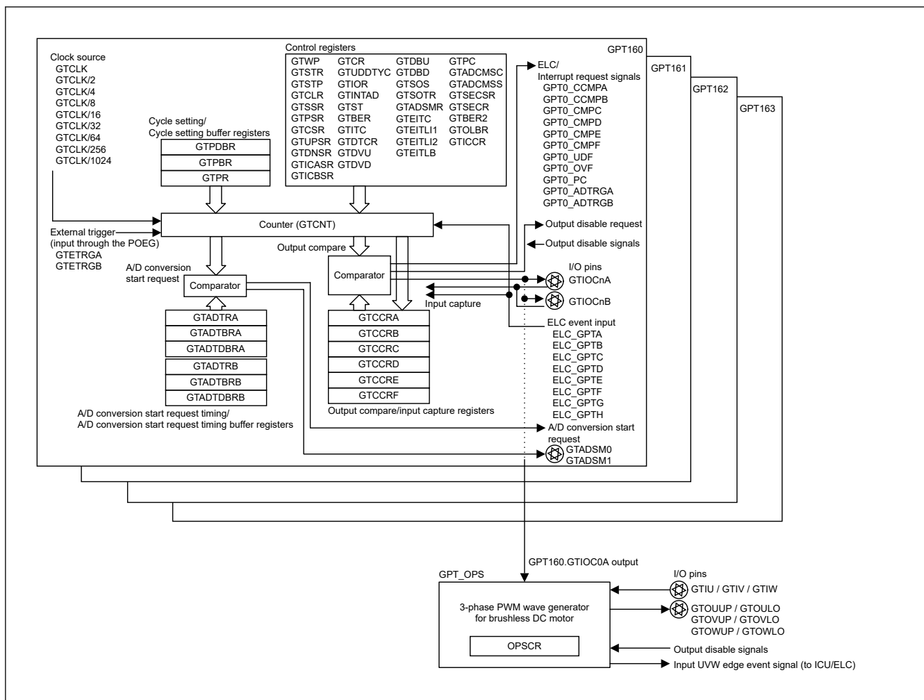
Figure 20.1 GPT block diagram (Saw-wave PWM mode 1, Saw-wave one-shot pulse mode, Triangle-wave PWM mode 1, 2, 3)
