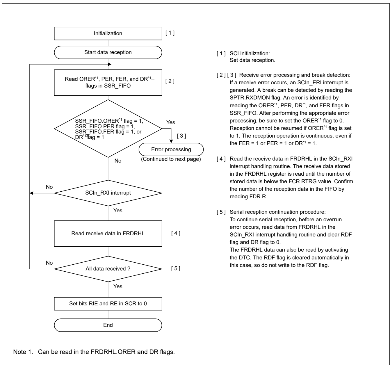
Figure 24.21 Example flow of serial reception in asynchronous mode with FIFO selected and Address Matching Enabled (1)
