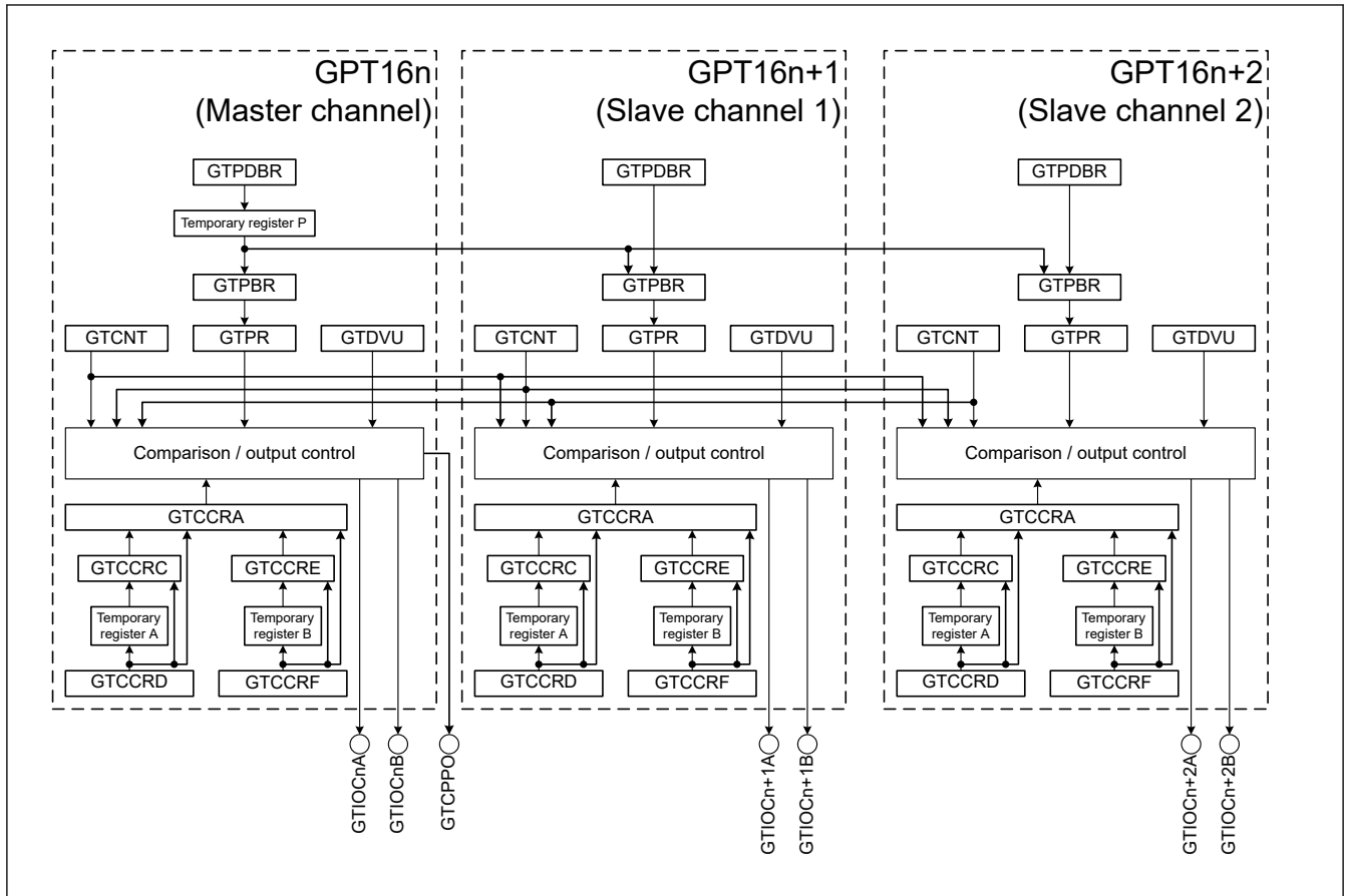
Figure 20.69 Block diagram in complementary PWM mode 4 ( n = 0 )
