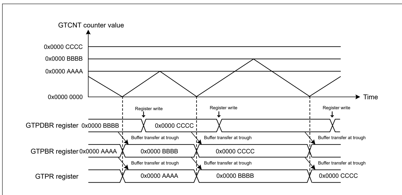
Figure 20.20 Example of GTPR double buffer operation with triangle waves
