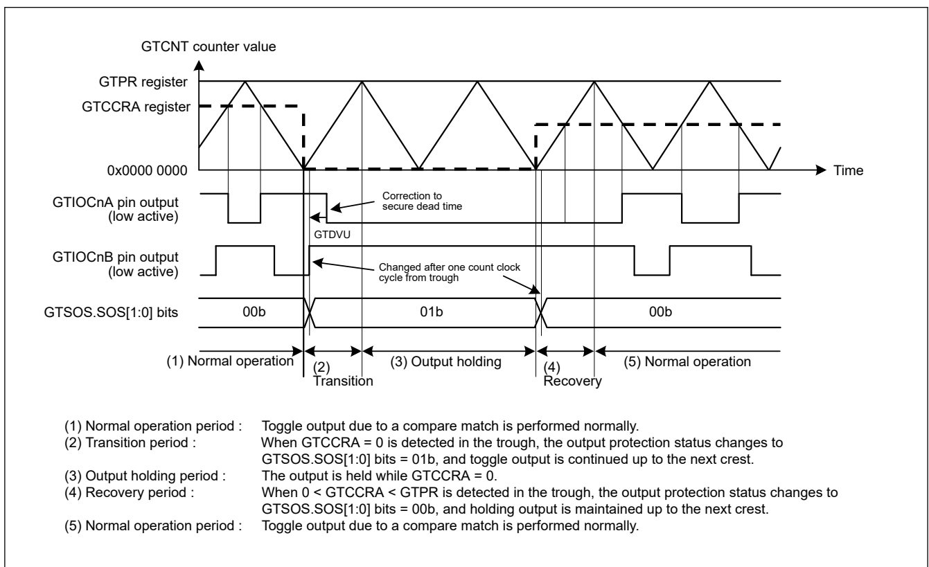
Figure 20.172 Example of output protection function operation when GTCCRA is set to 0x0000 0000 during buffer transfer at troughs (restored to 0 < GTCCRA < GTPR during buffer transfer at troughs, active level: low) (n = 0 to 2)
