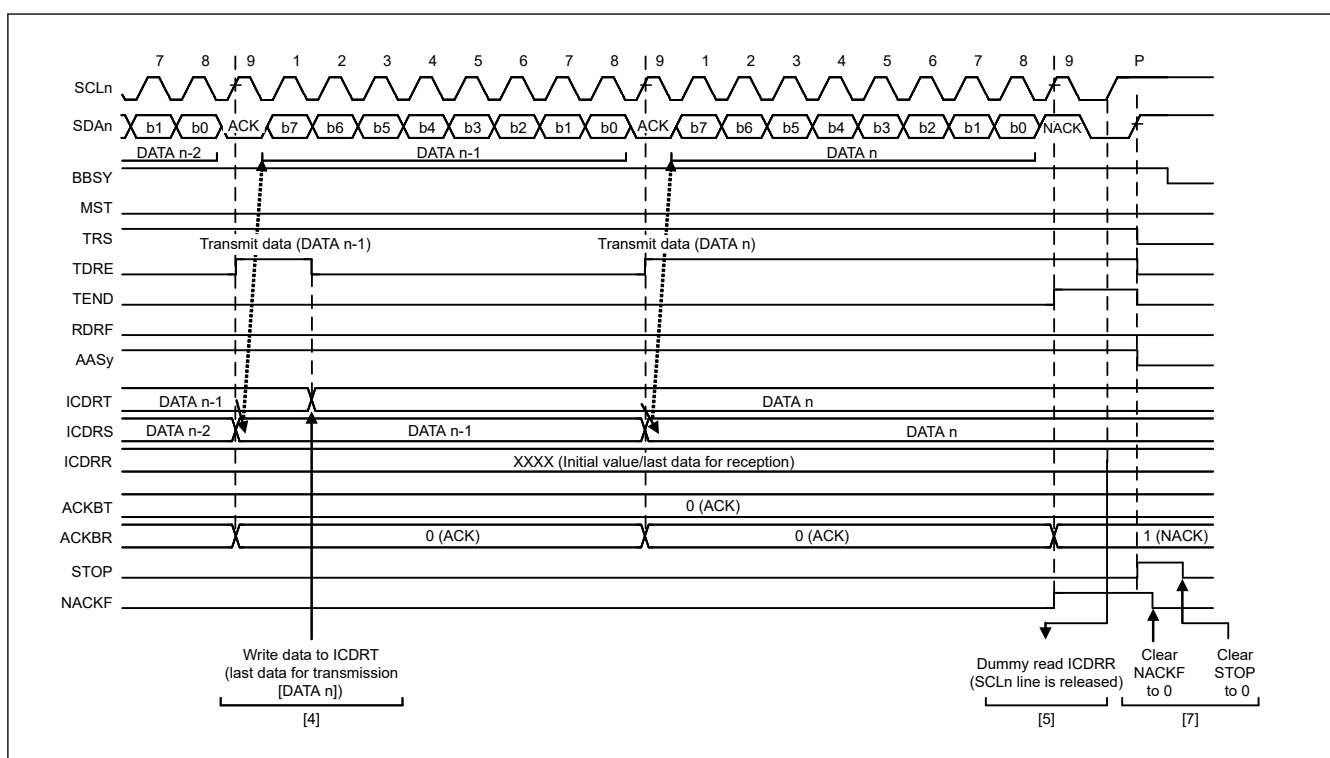
Figure 25.17 Slave transmit operation timing (2)
