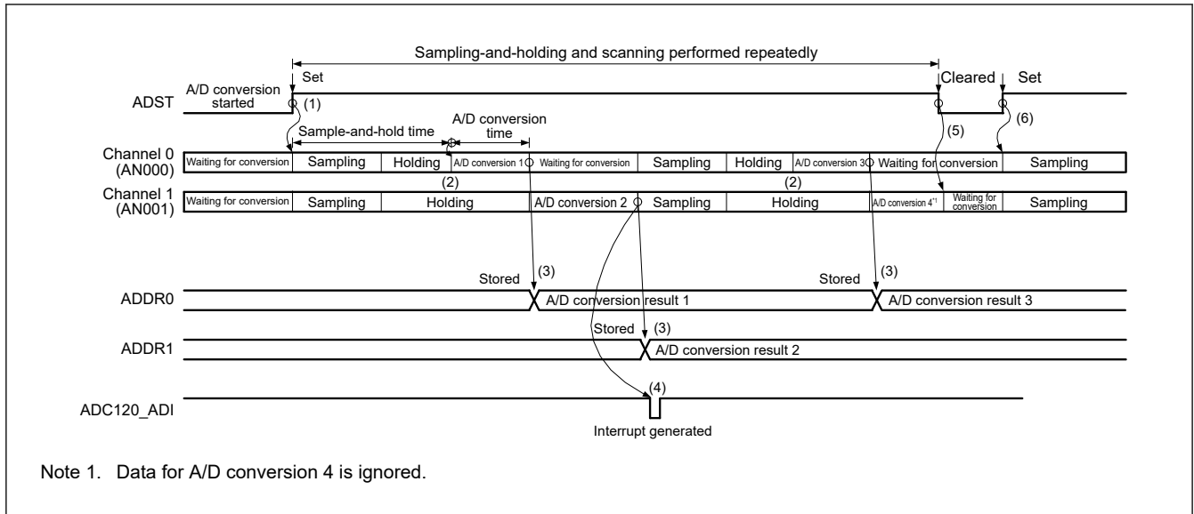
Figure 29.15 Example operation in continuous scan mode when channel-dedicated sample-and-hold circuits are used and AN000 and AN001 are selected
