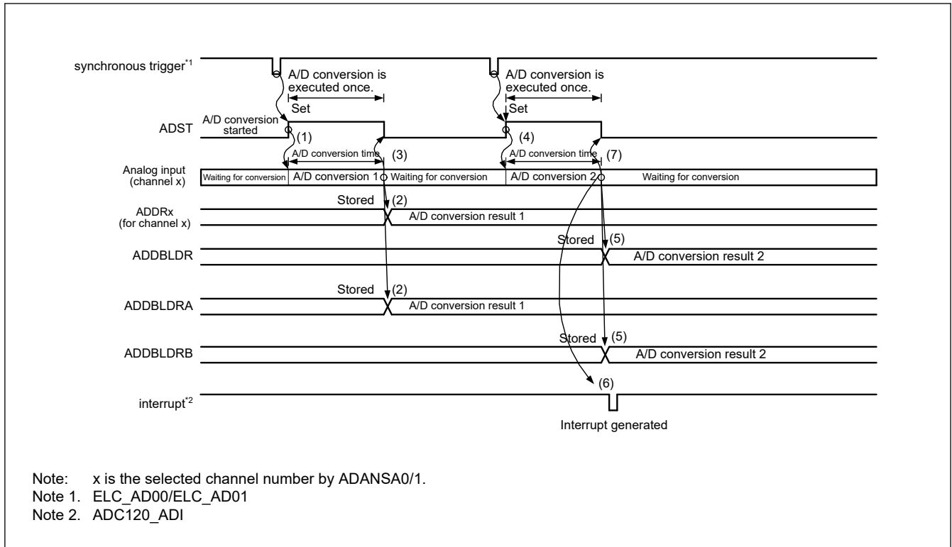
Figure 29.13 Example extended operation in double trigger mode with duplication selected for the analog input (channel x) and ELC_AD00/ELC_AD01
