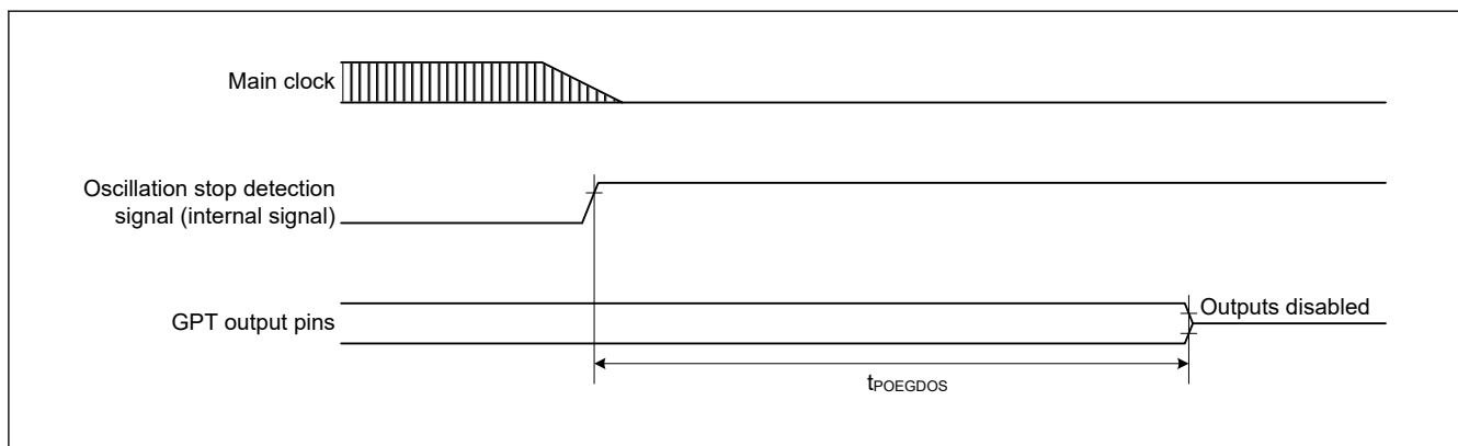
Figure 35.19 Output disable time of POEG in response to the oscillation stop detection
