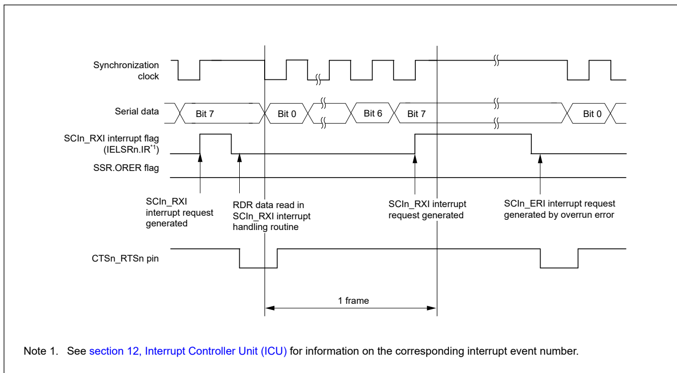
Figure 24.42 Example operation for serial reception in clock synchronous mode (2) when RTS function is used
