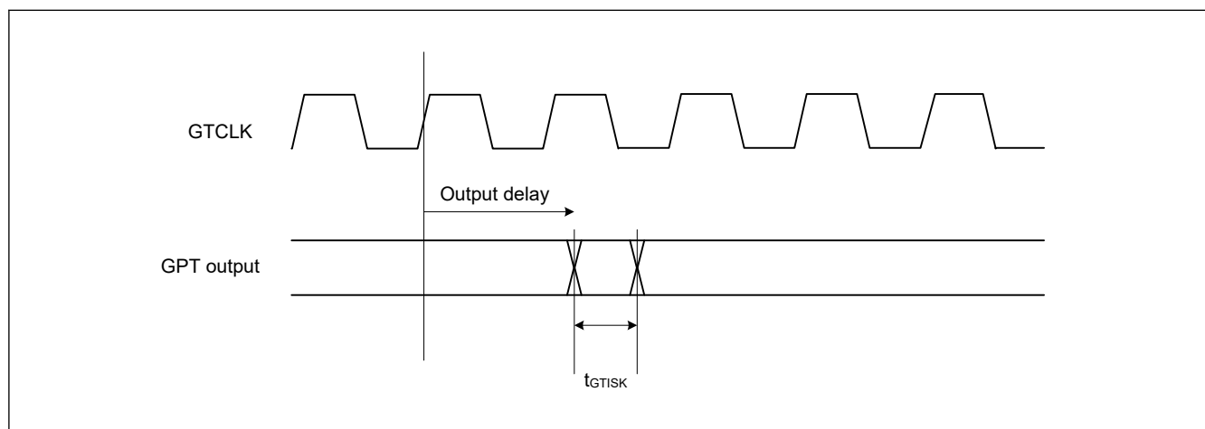
Figure 35.23 GPT output delay skew
