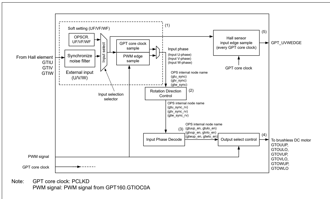
Figure 20.135 Conceptual diagram of GPT_OPS control flow
