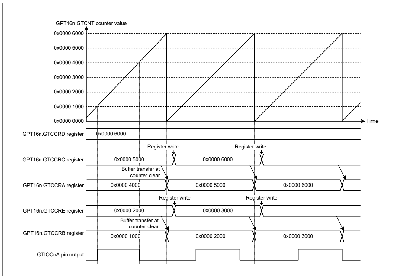
Figure 20.40 Example of saw-wave PWM mode 2 operation (low output at GTCCRA register compare match, high output at GTCCRB register compare match, low output at the end of cycle, single buffer operation, cleared at GTCCRD register compare match, GTIOR.OAEOCD bit = 0) (n = 0 to 2)
