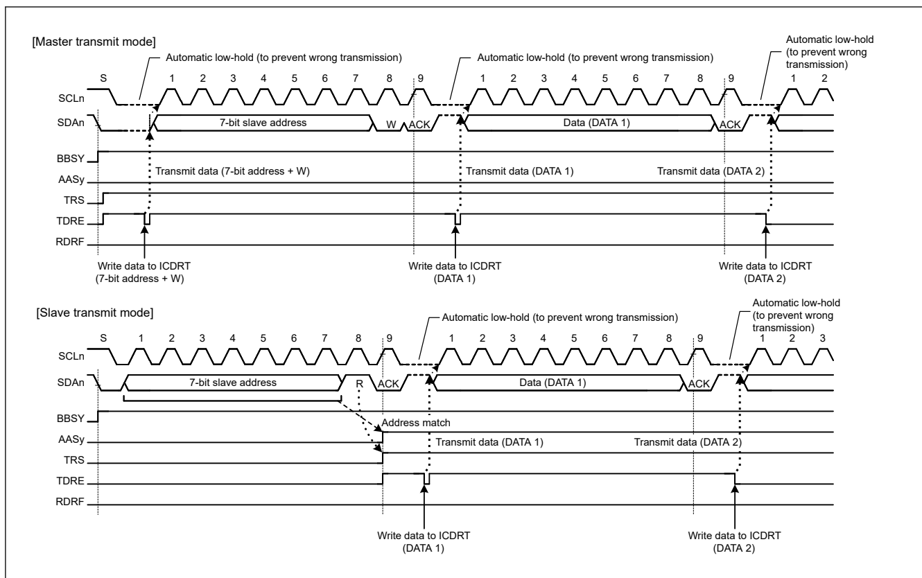
Figure 25.38 Automatic low-hold operation in transmit mode
