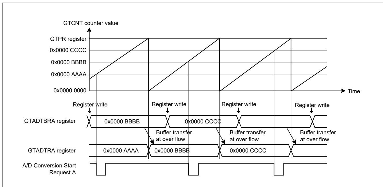
Figure 20.30 Example of buffer operation of the GTADTRA and GTADTRB registers (saw waves in up-counting, A/D conversion start request generated by up-counting)
