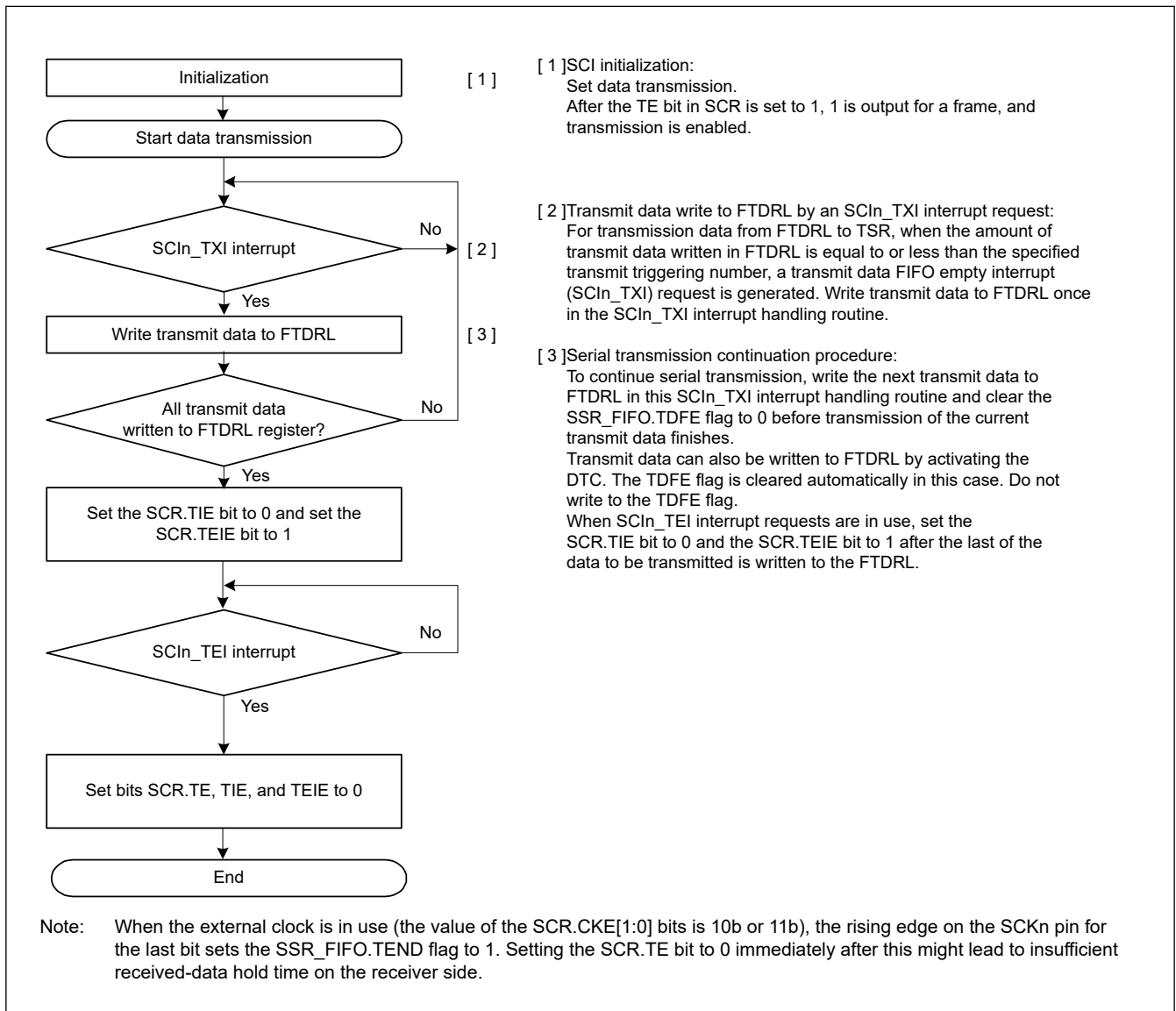
Figure 24.40 Example flow of serial transmission in clock synchronous mode with FIFO selected
