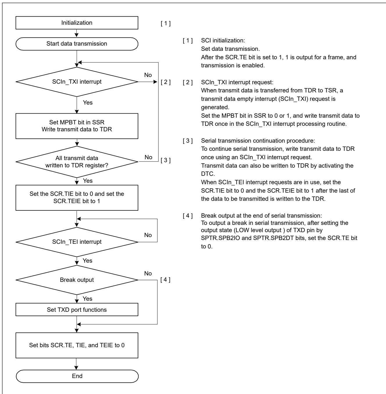
Figure 24.27 Example flow of multi-processor serial transmission with non-FIFO selected
