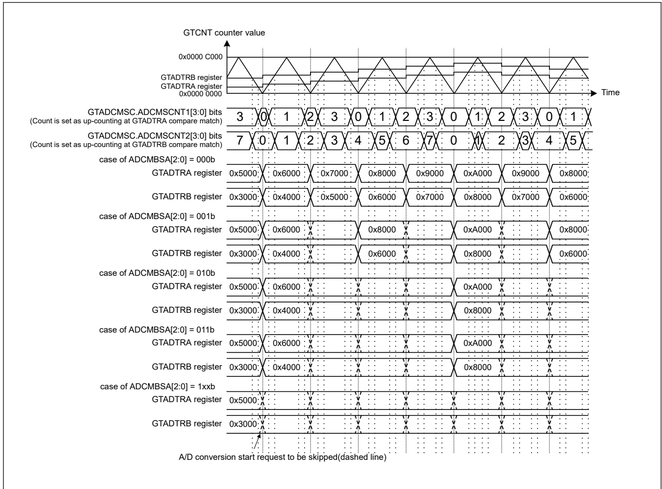
Figure 20.159 Example of A/D conversion start request compare match skipping function operation (triangle-wave, A/D conversion start request compare match skipping 1 skipping count: 3 counting GTADTRA compare match, A/D conversion start request compare match skipping 2 skipping count: 7 counting GTADTRB compare match, buffer transfer of GTADTRA and GTADTRB at trough)
