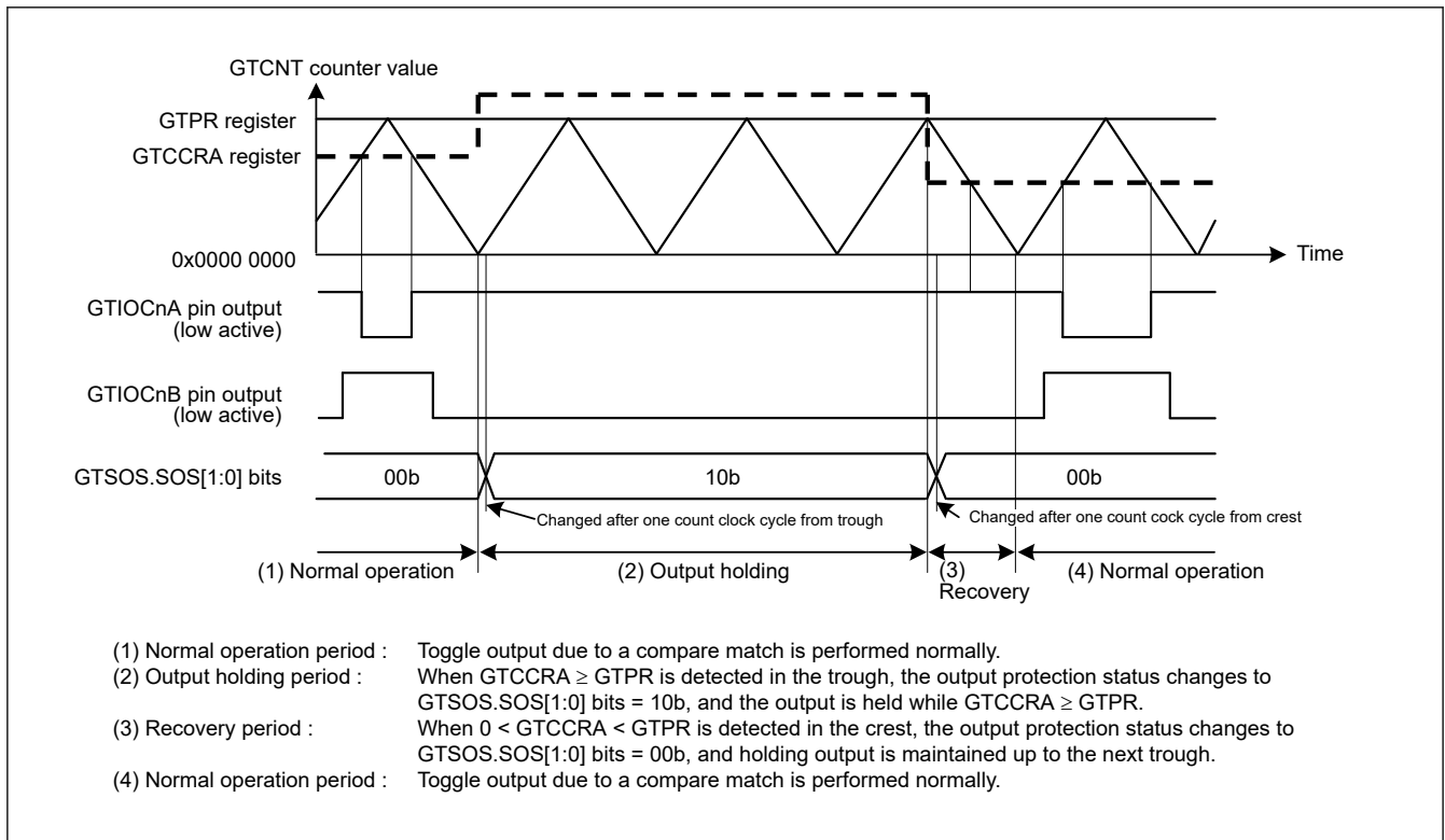
Figure 20.177 Example of output protection function operation when GTCCRA \geq GTPR is set during buffer transfer at troughs (restored to 0 < GTCCRA < GTPR during buffer transfer at crests, active level: low) (n = 0 to 2)
