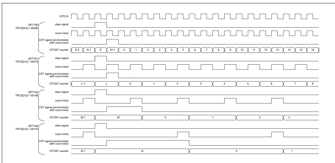
Figure 20.111 Example of simultaneous clearing operation by software (with different count period)
