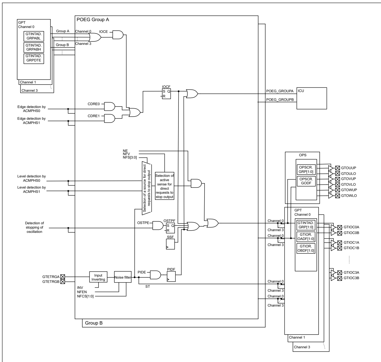
Figure 19.1 POEG block diagram
