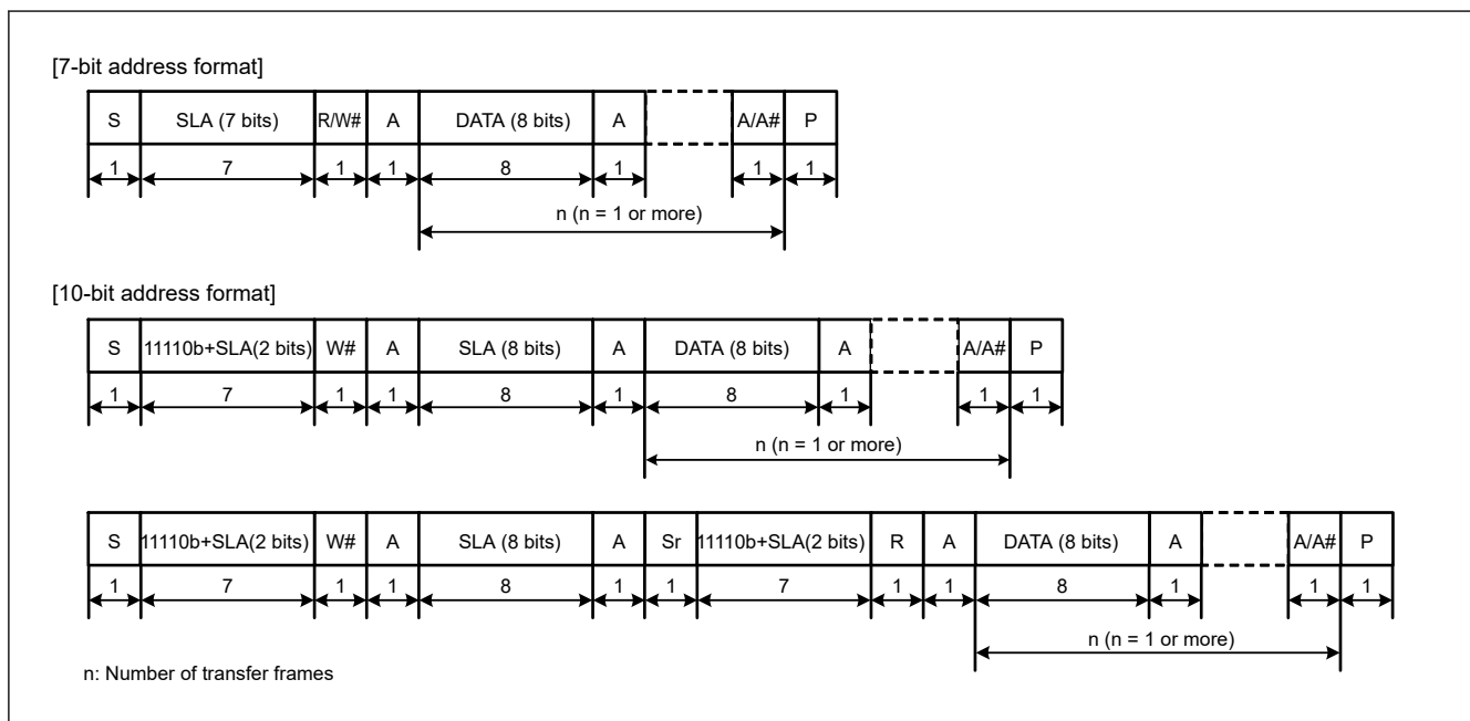
Figure 25.3 I 2 C bus format
