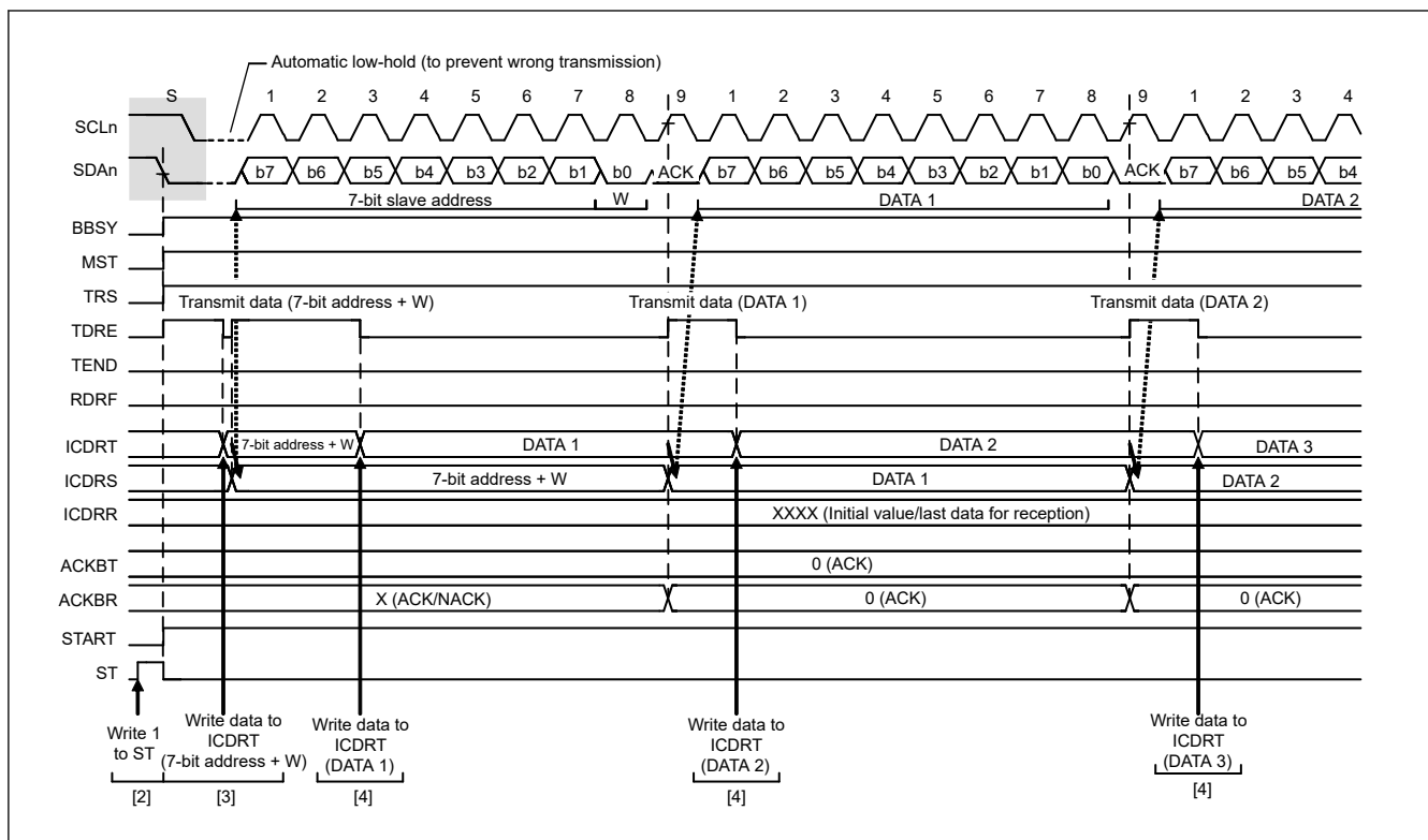
Figure 25.7 Master transmit operation timing (1) with 7-bit address format
