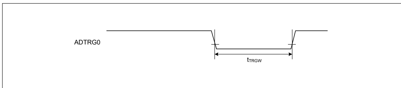
Figure 35.29 ADC12 trigger input timing
