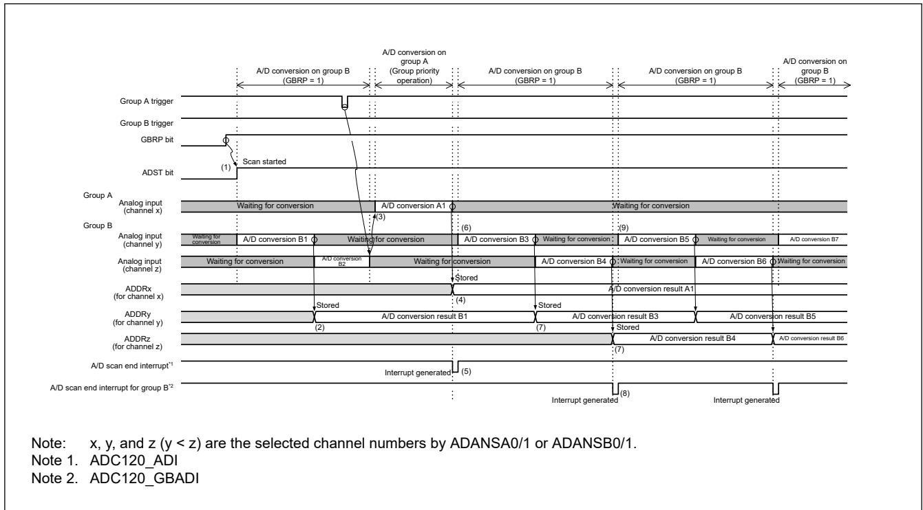
Figure 29.25 Group priority operation example 1-5: Continuously activating single scan for group B (when \text{ADGSPCR.GBRP} = 1 )
