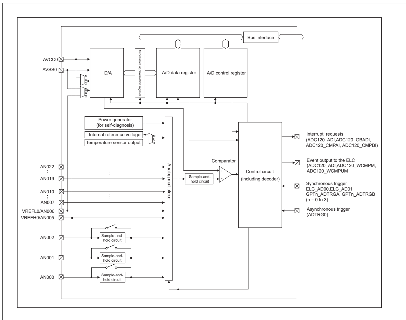
Figure 29.1 ADC12 block diagram
