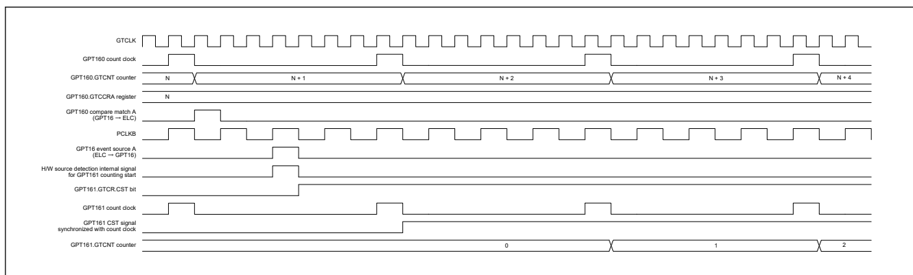
Figure 20.92 Example of timing of operations to start counting in response to event input from ELC_GPTA
