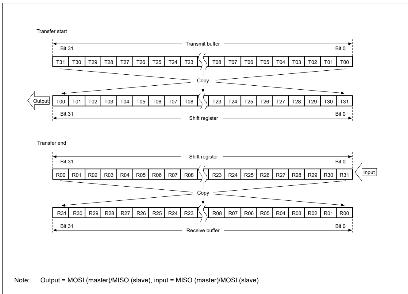
Figure 26.15 LSB-first transfer with 32-bit data and parity disabled
