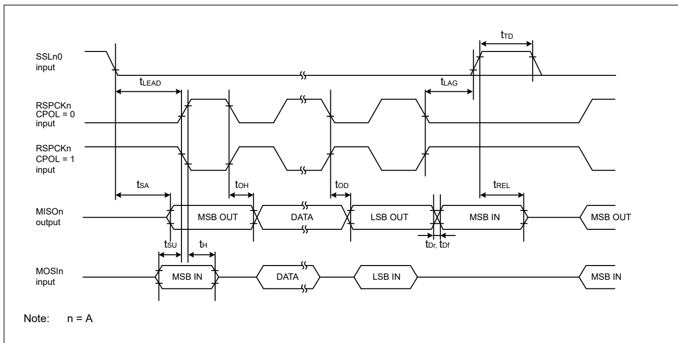
Figure 35.44 SPI timing (slave, CPHA = 0)
