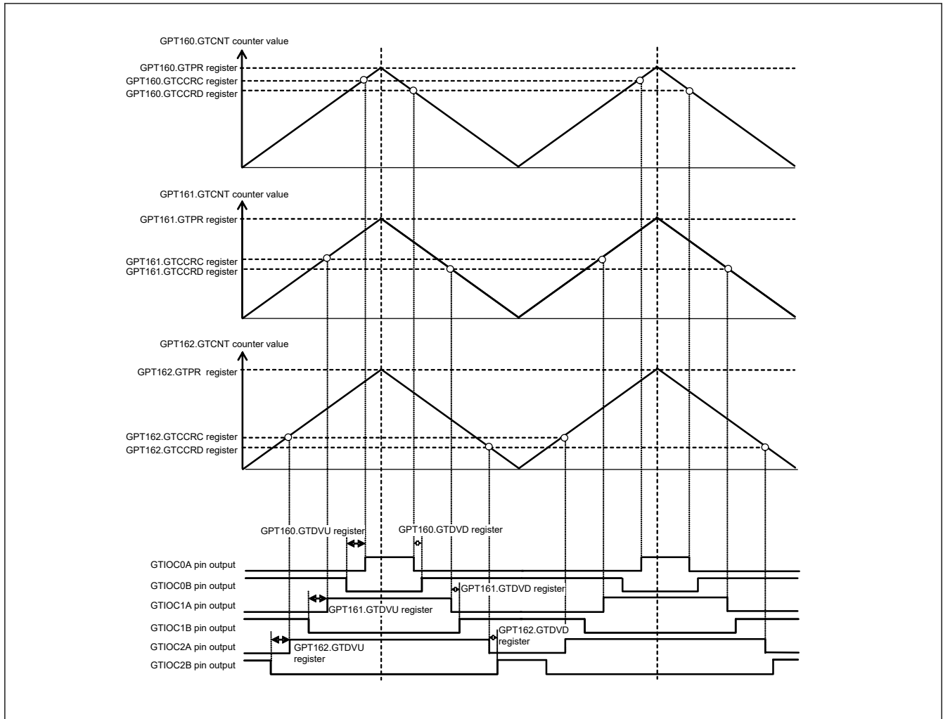
Figure 20.120 Example of 3-phase asymmetric triangle-wave complementary PWM output with automatic dead time setting
