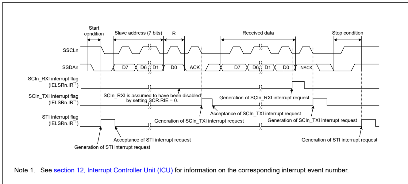
Figure 24.66 Example operations for master reception in simple IIC mode with 7-bit slave addresses, transmission interrupts, and reception interrupts
