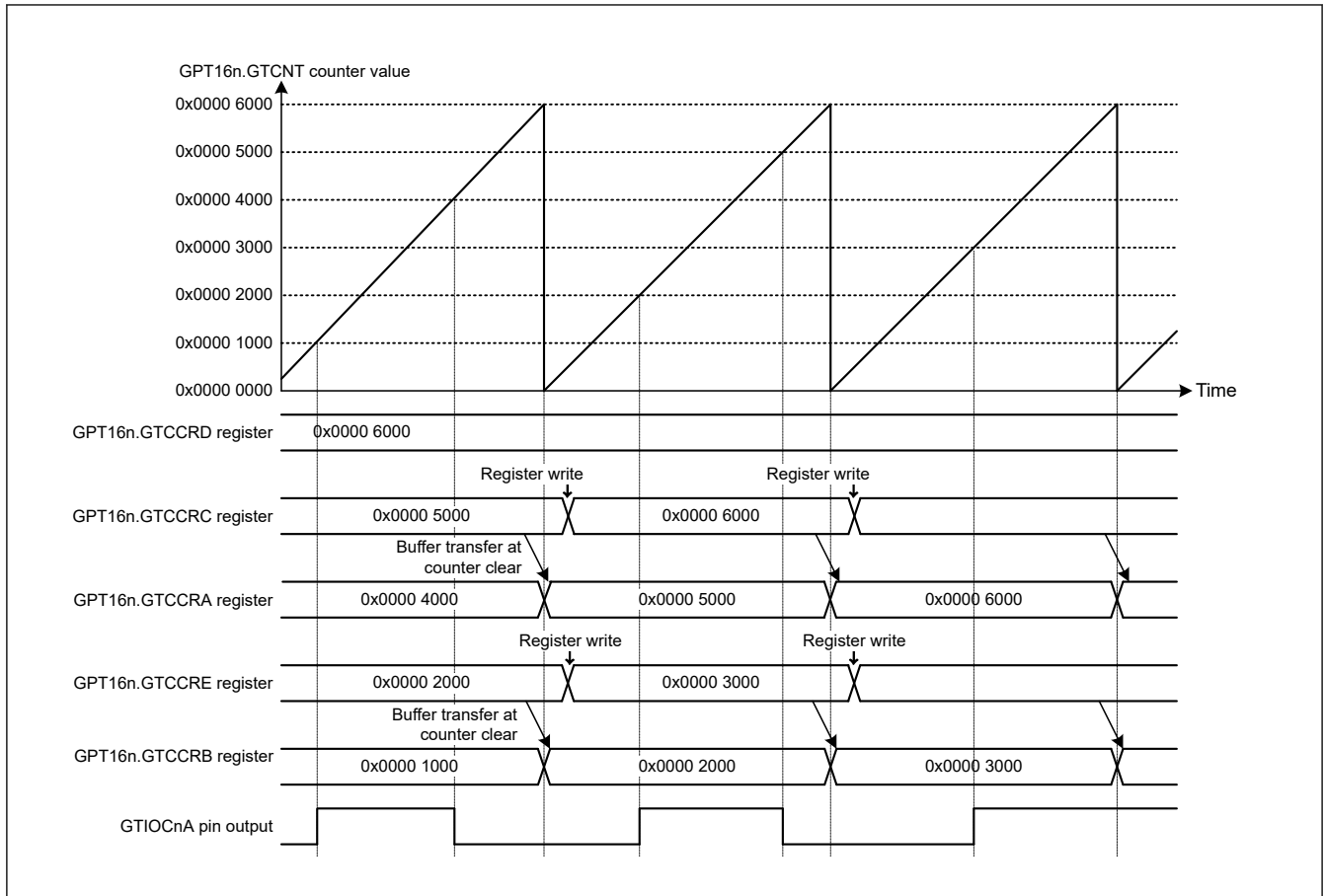
Figure 20.41 Example of saw-wave PWM mode 2 operation (low output at GTCCRA register compare match, high output at GTCCRB register compare match, low output at the end of cycle, single buffer operation, cleared at GTCCRD register compare match, GTIOR.OAEOCD bit = 1) (n = 0 to 2)
