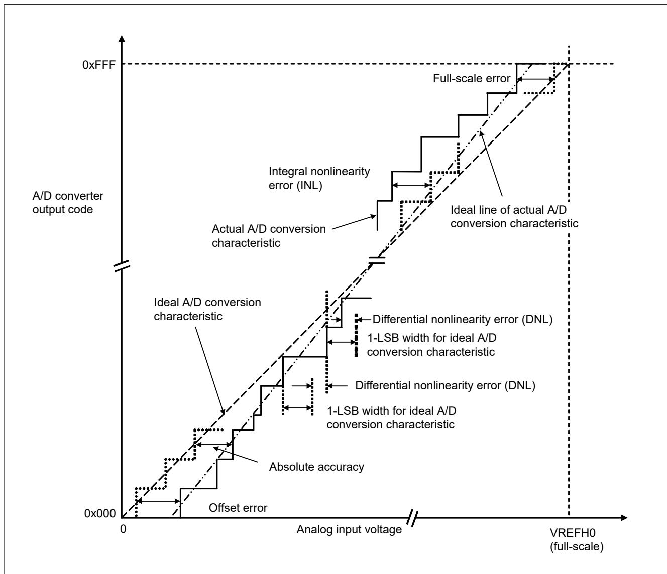
Figure 35.50 Illustration of 12-bit A/D converter characteristic terms
