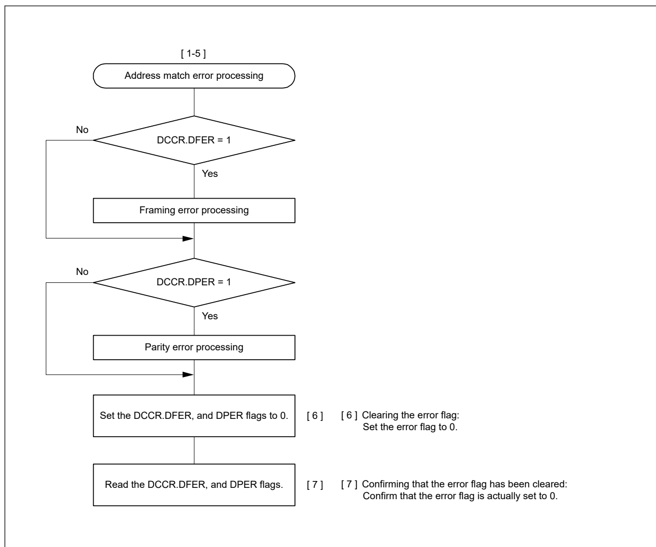
Figure 24.18 Example Flowchart of Serial Reception in Asynchronous Mode (FIFO not Selected and Address Matching Enabled) (2)
