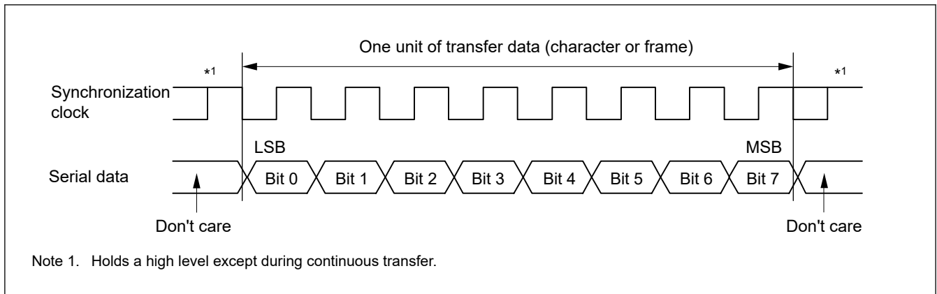
Figure 24.35 Data format in clock synchronous serial communications with LSB-first order
