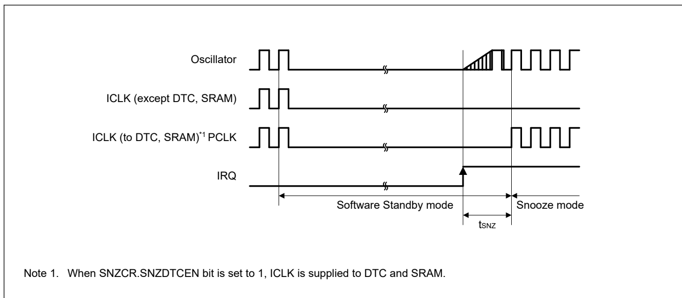
Figure 35.10 Recovery timing from Software Standby mode to Snooze mode
