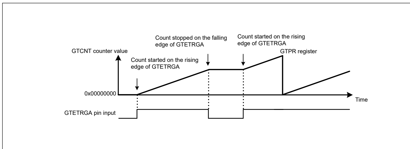
Figure 20.94 Example of count start/stop operation by a hardware source started on the rising edge of GTETRGA pin input, and stopped on the falling edge of GTETRGA pin input
