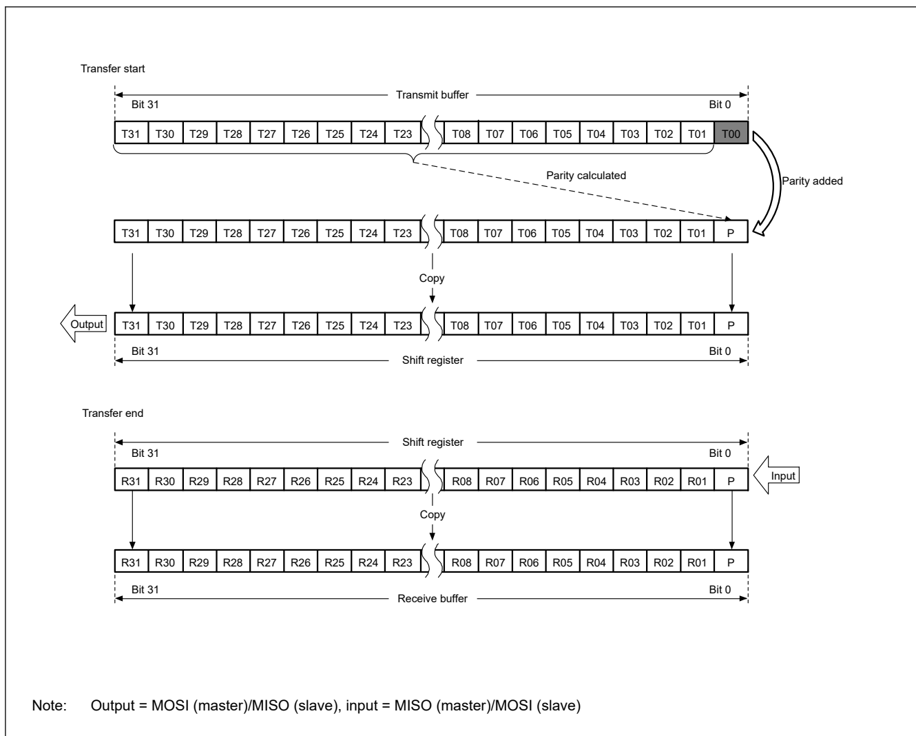
Figure 26.17 MSB-first transfer with 32-bit data and parity enabled
