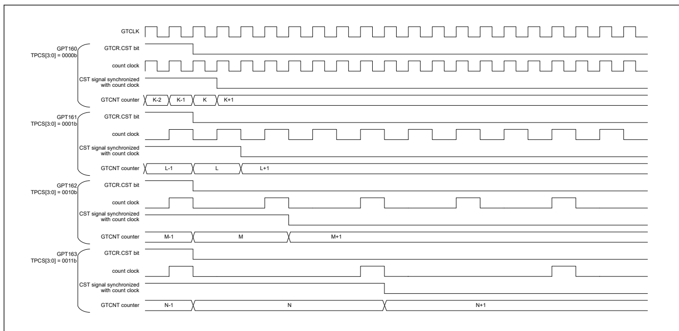
Figure 20.110 Example of simultaneous stop operation by software (with different count period)
