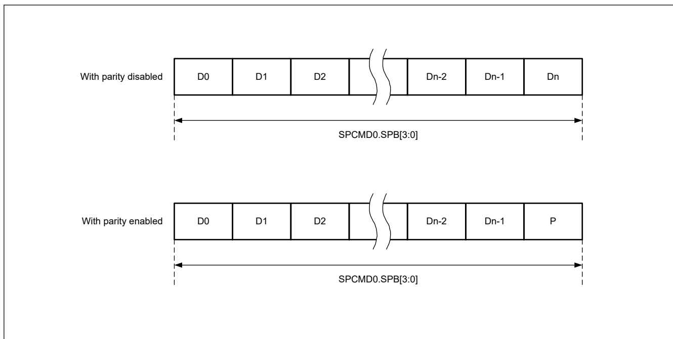
Figure 26.12 Data format with parity disabled and enabled
