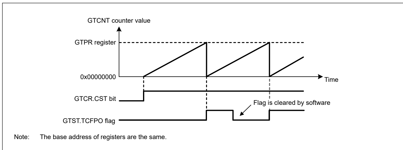
Figure 20.4 Example of periodic count operation in up-counting by the count clock
