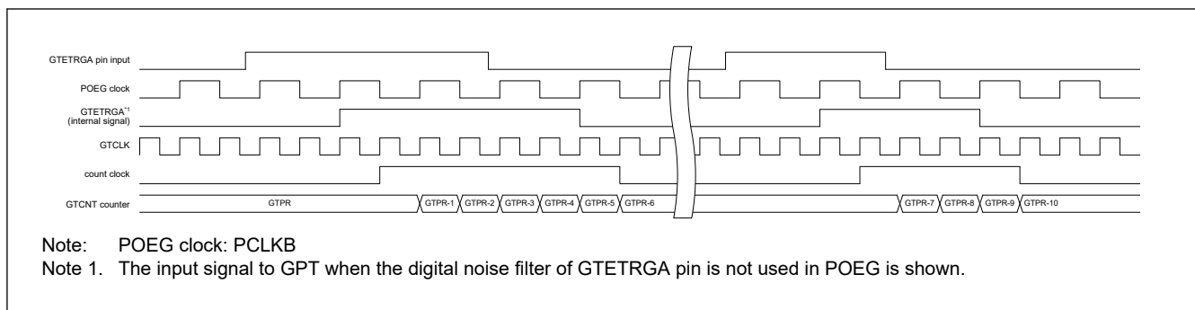
Figure 20.134 Example of external pulse width measuring function (down-counting)
