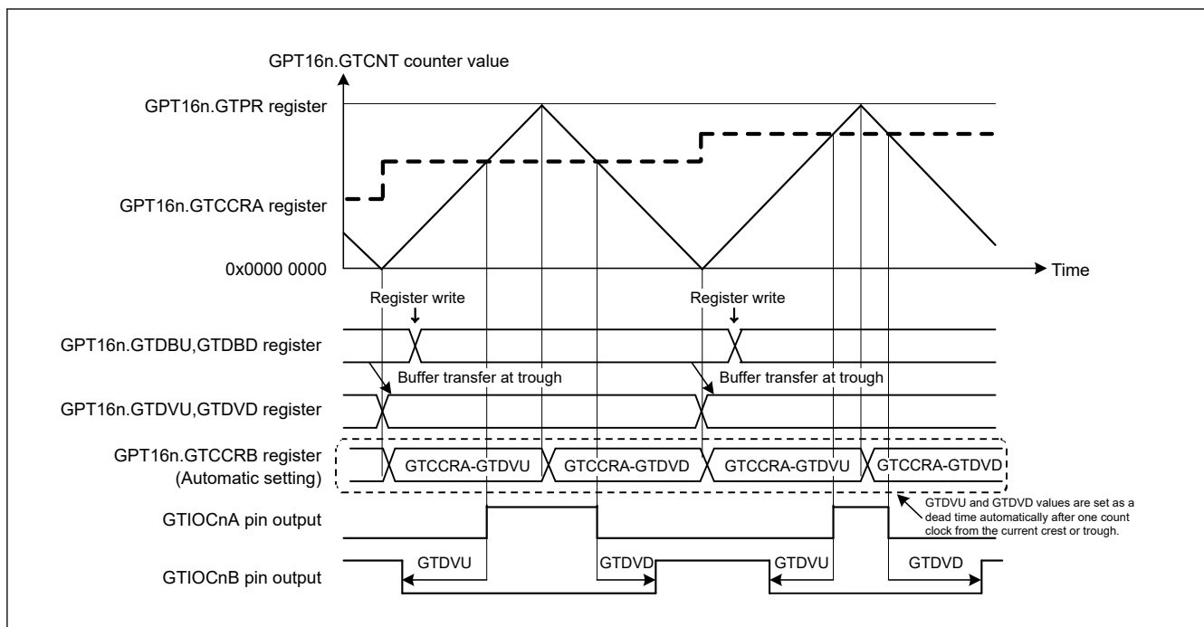
Figure 20.83 Example of automatic compare-match value setting function with dead time in triangle-wave PWM mode 1, GTDVU and GTDVD set to buffer operation, and active-high in GPT160 to GPT162
