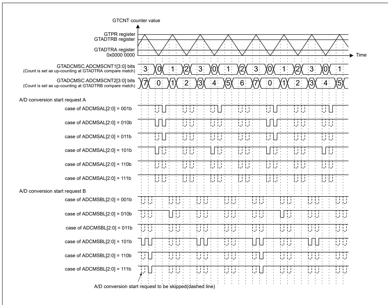
Figure 20.158 Example of A/D conversion start request compare match skipping function operation (triangle-wave, A/D conversion start request compare match skipping 1 skipping count: 3 counting GTADTRA compare match, A/D conversion start request compare match skipping 2 skipping count: 7 counting GTADTRB compare match)
