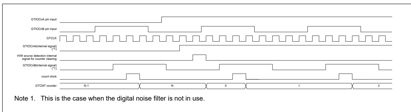
Figure 20.105 Examples of the timing of operations for counter clearing in response to a rising edge of the input on the GTIOcNA pin (during counting triggered by hardware source)
