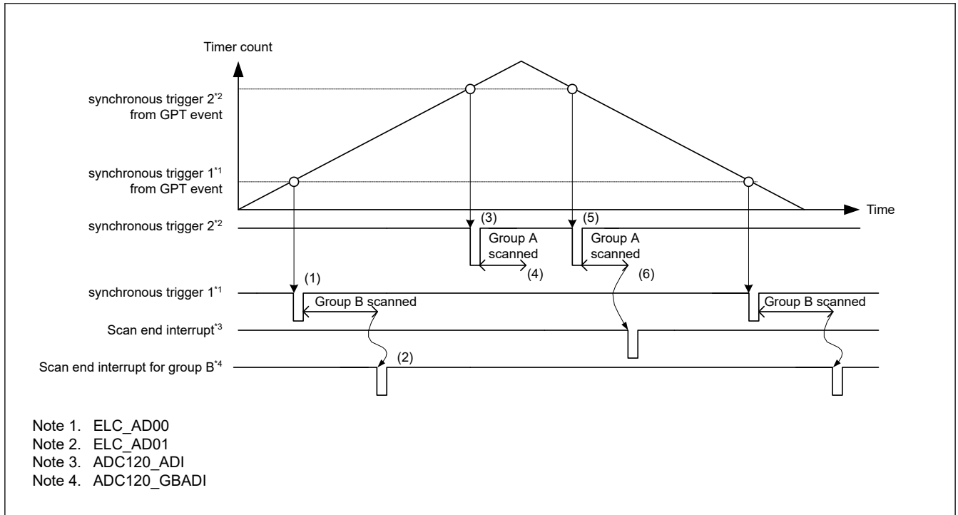
Figure 29.19 Example basic operation in group scan mode with double-trigger mode when synchronous triggers from the ELC are used
