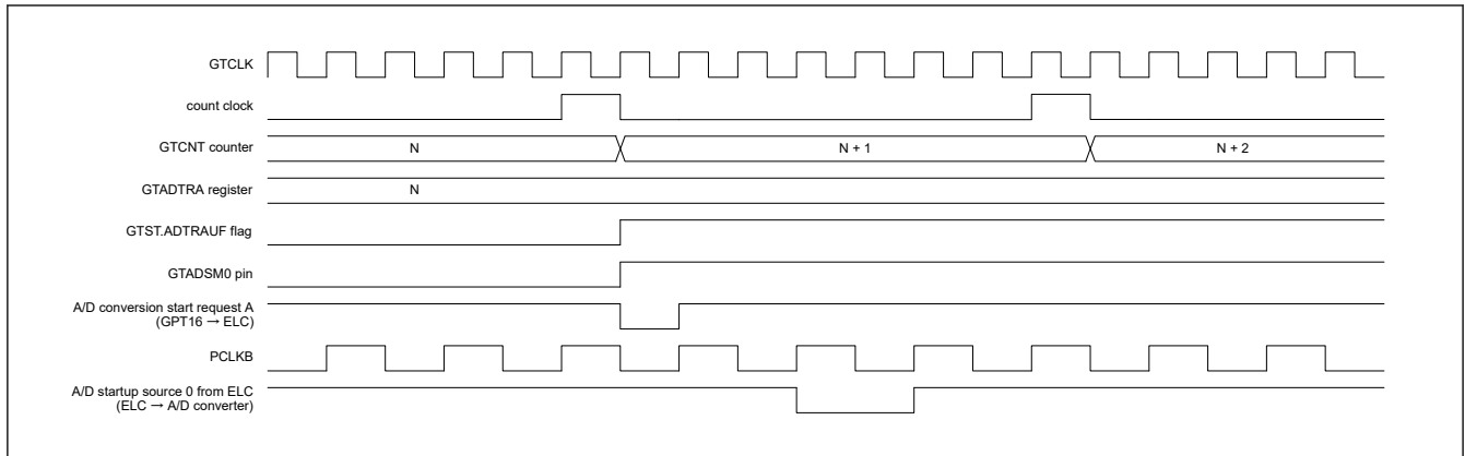
Figure 20.161 Example of A/D conversion start request timing operation
