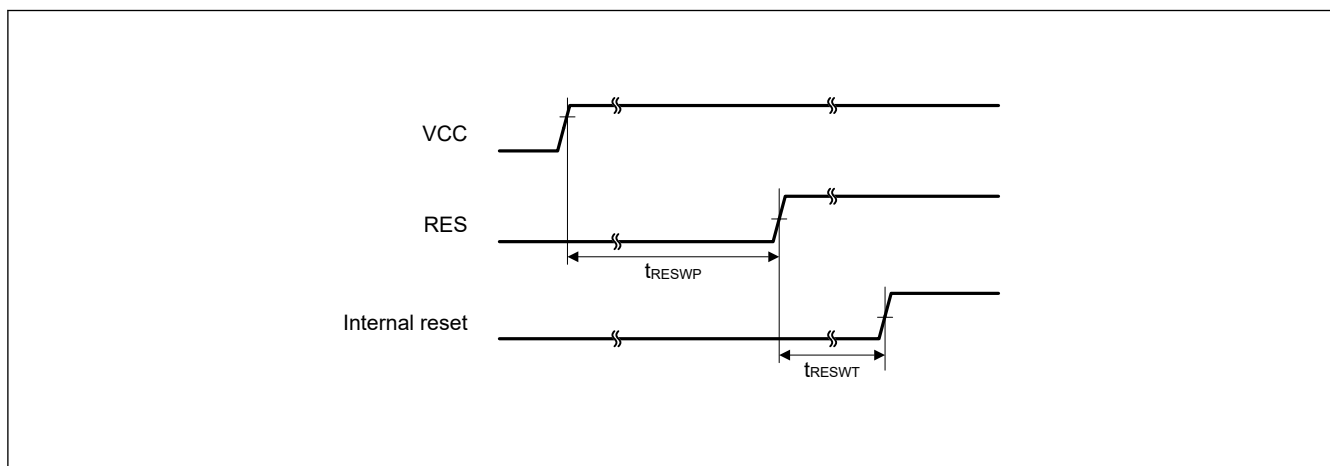
Figure 35.6 Reset input timing at power-on
