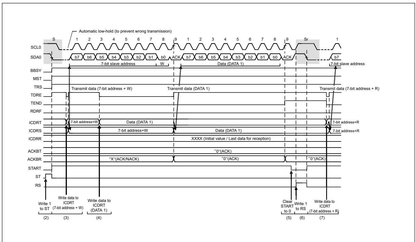
Figure 25.46 Restart condition issue timing after master transmission.
