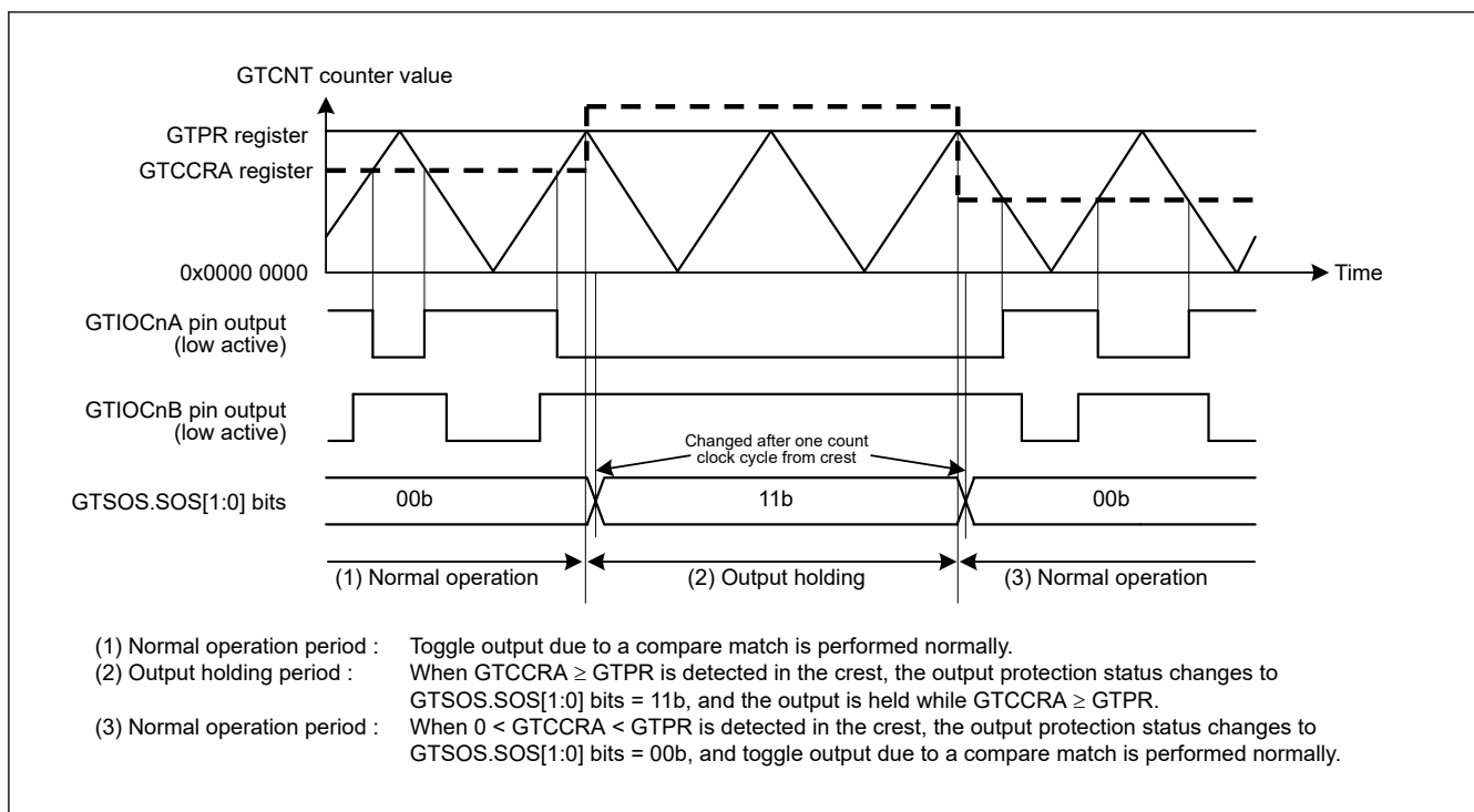
Figure 20.178 Example of output protection function operation when GTCCRA \geq GTPR is set during buffer transfer at crests (restored to 0 < GTCCRA < GTPR during buffer transfer at crests, active level: low) (n = 0 to 2)
