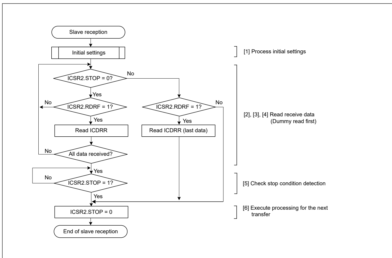
Figure 30.18 Example slave reception flow
