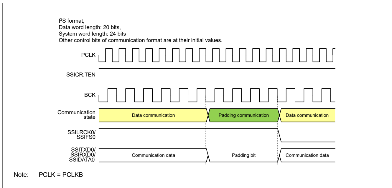
Figure 34.49 Transition from data communication to padding communication
