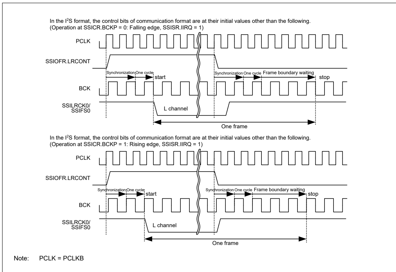
Figure 34.44 Example of disabling LR clock/frame synchronization continuation by SSIOFR.LRCONT
