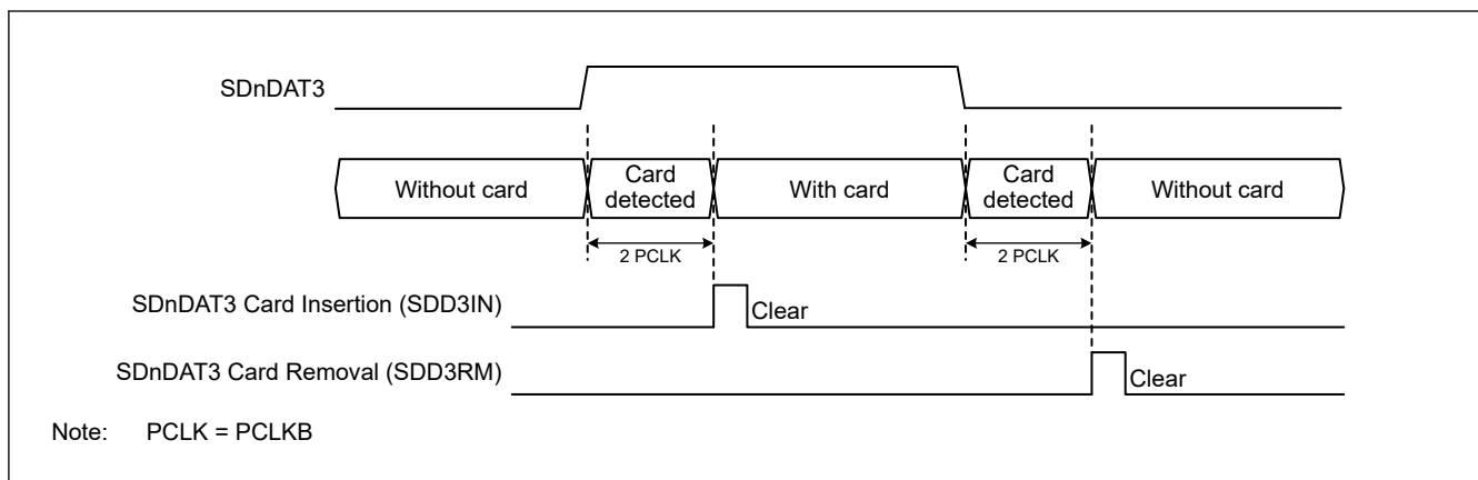
Figure 35.7 SD card detection with SDnDAT3
