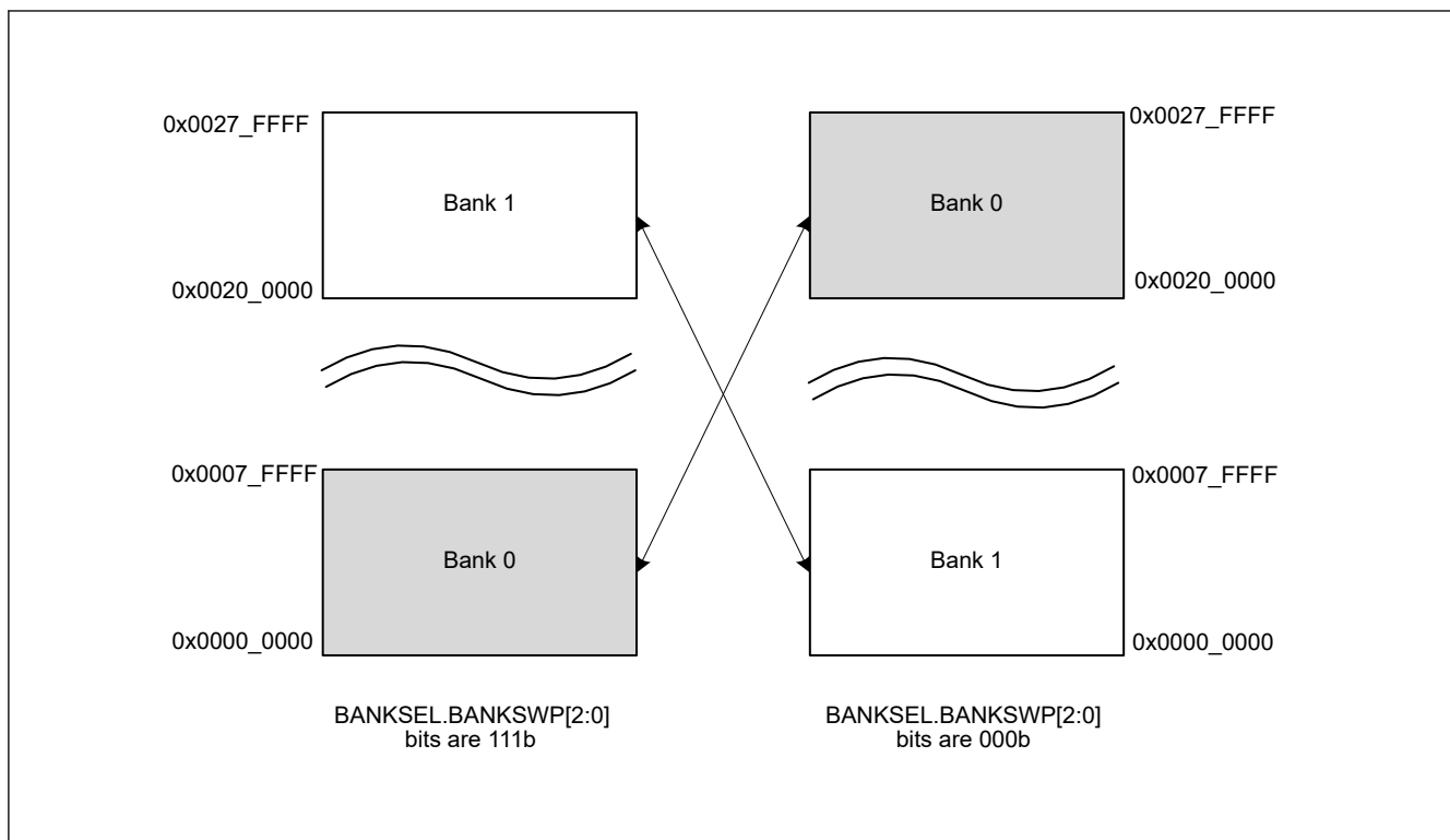
Figure 44.31 Example of Startup Bank Selection (For Products with 1 MB of Code Flash Memory)
