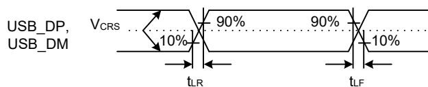
Figure 47.54 USB_DP and USB_DM output timing in low-speed mode
