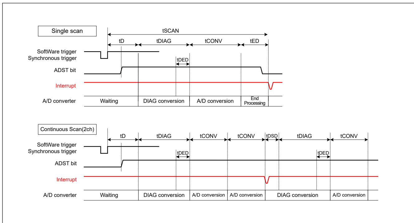
Figure 39.26 Scan conversion timing when activated by software or a synchronous trigger input (ELC)
