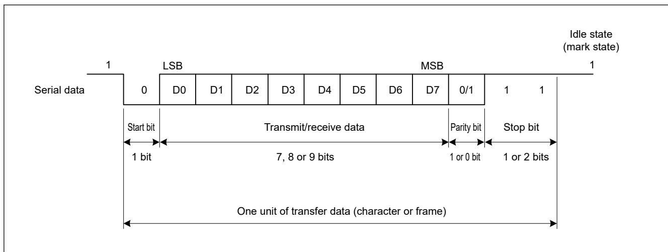
Figure 29.6 Data format in asynchronous serial communications with 8-bit data, parity bit, and 2 stop bits
