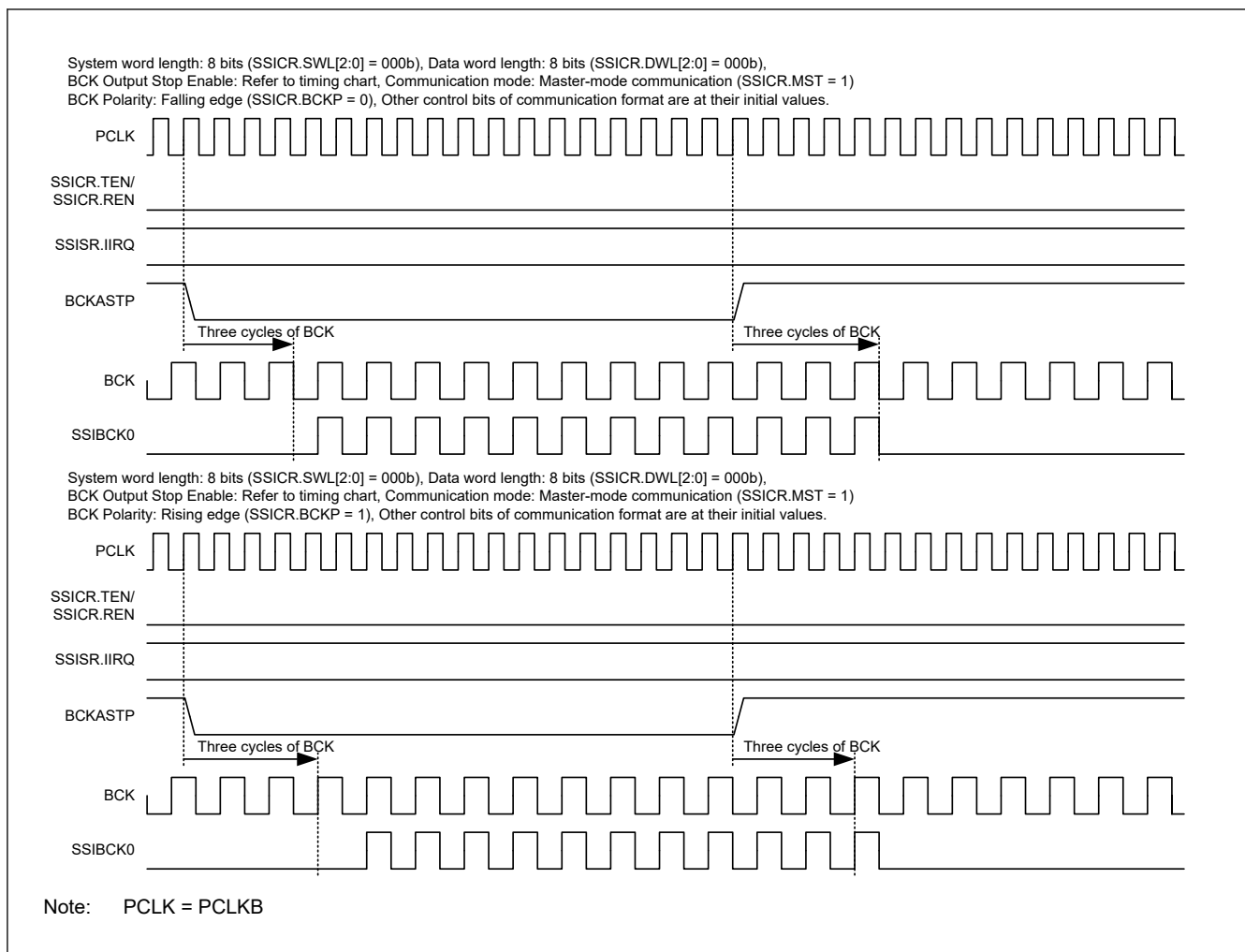
Figure 34.34 Example operation of the BCKASTP bit (idle state)
