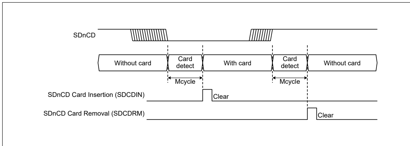
Figure 35.6 Example of card detection with SDnCD
