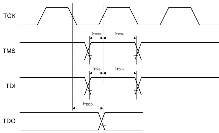
Figure 47.68 Boundary scan input/output timing
