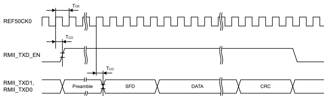
Figure 47.50 RMII transmission timing
