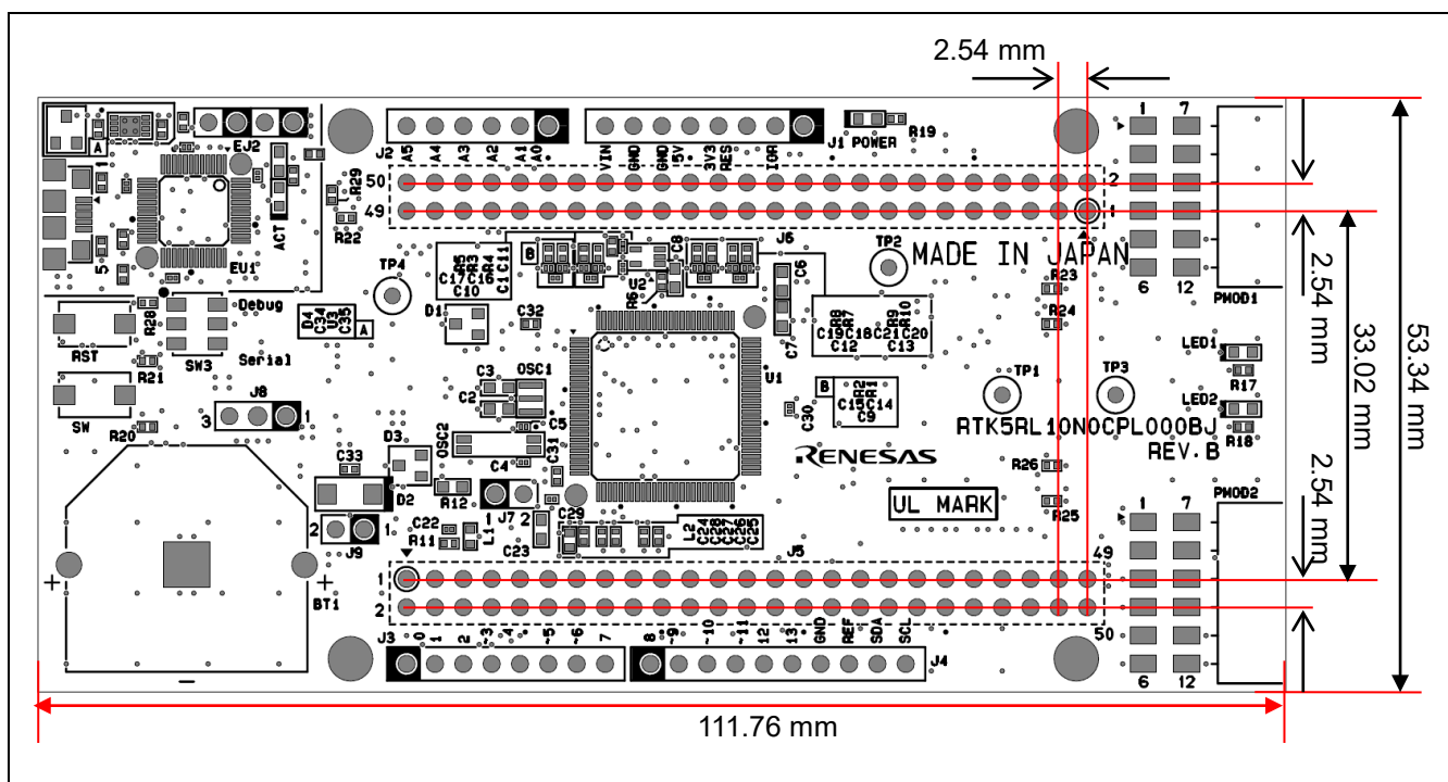
Figure 3-1 Parts Layout
