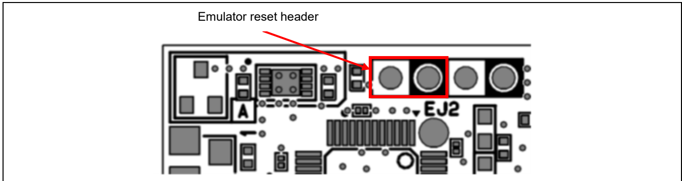
Figure 5-15 Position of the Emulator Reset Header (Top Side)
