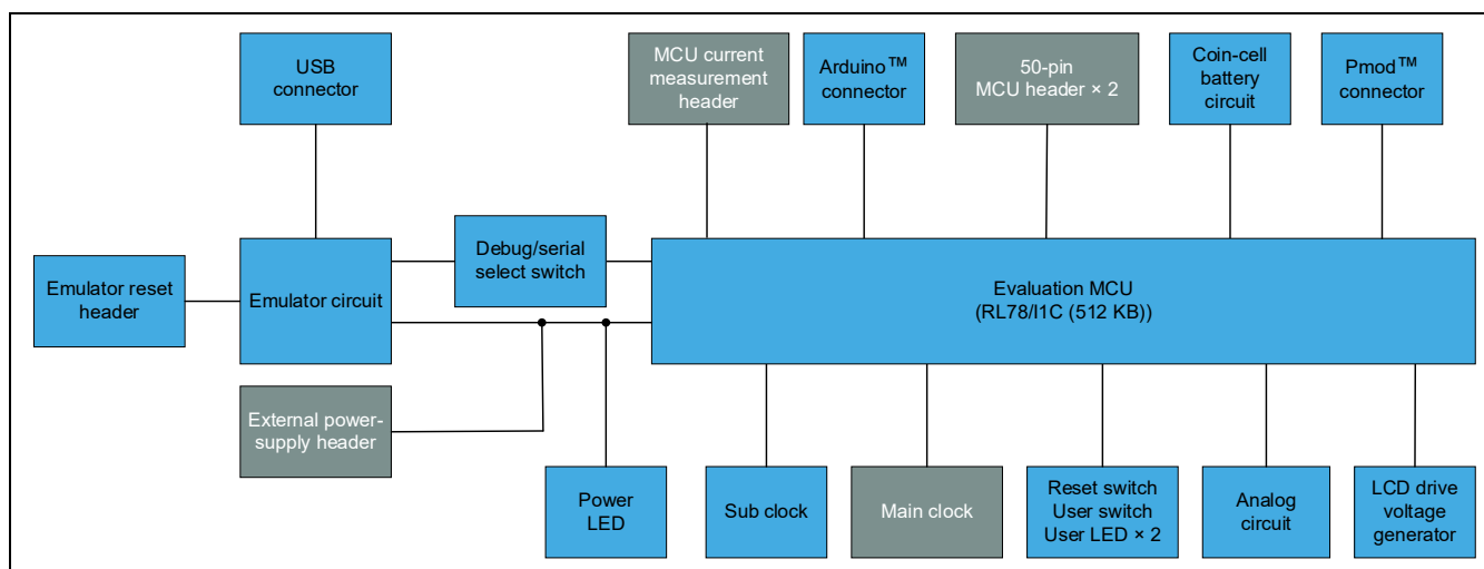
Figure 1-1 Block Diagram
