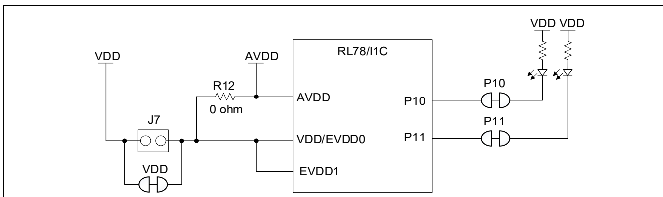
Figure 5-23 Block Diagram of the Headers Related to MCU Current Measurement
