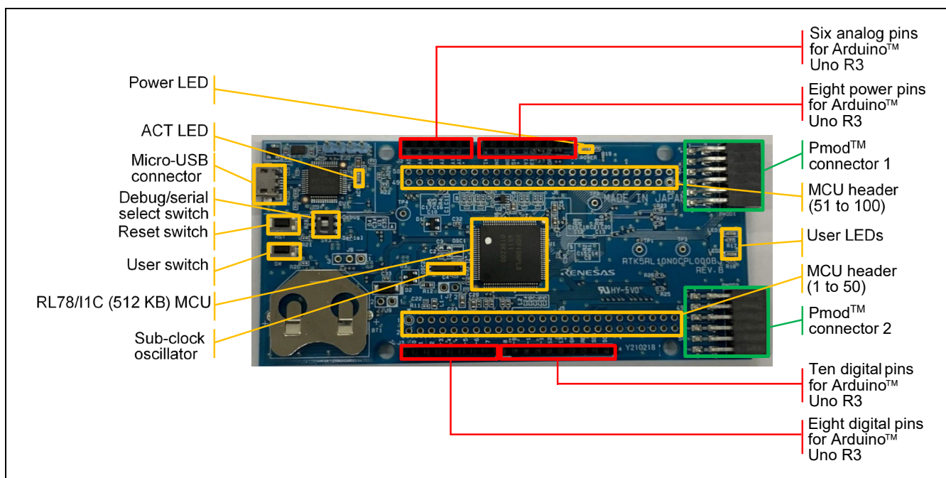
Figure 2-1 Board Layout (Top Side)
