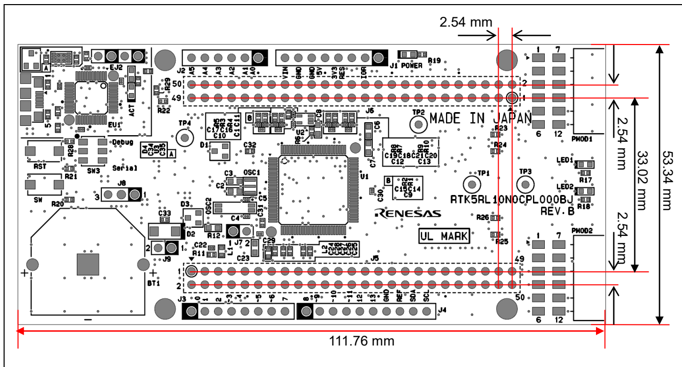
Figure 3-1 Parts Layout
