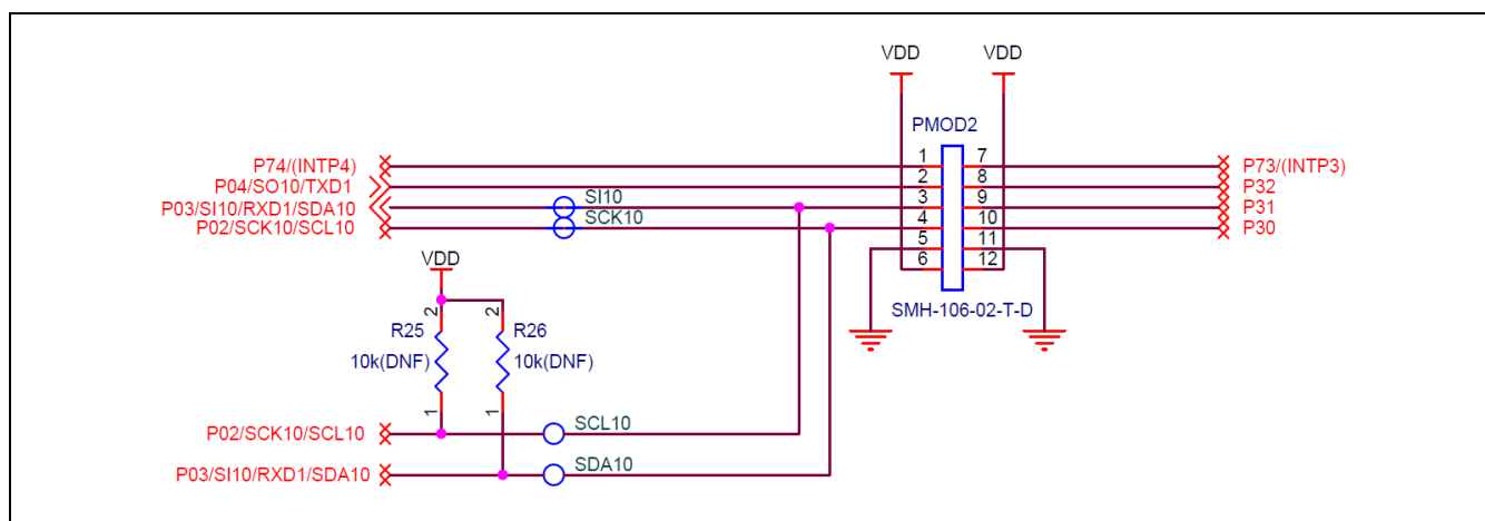
Figure 5-5 Circuit Schematic of Pmod™ 2
