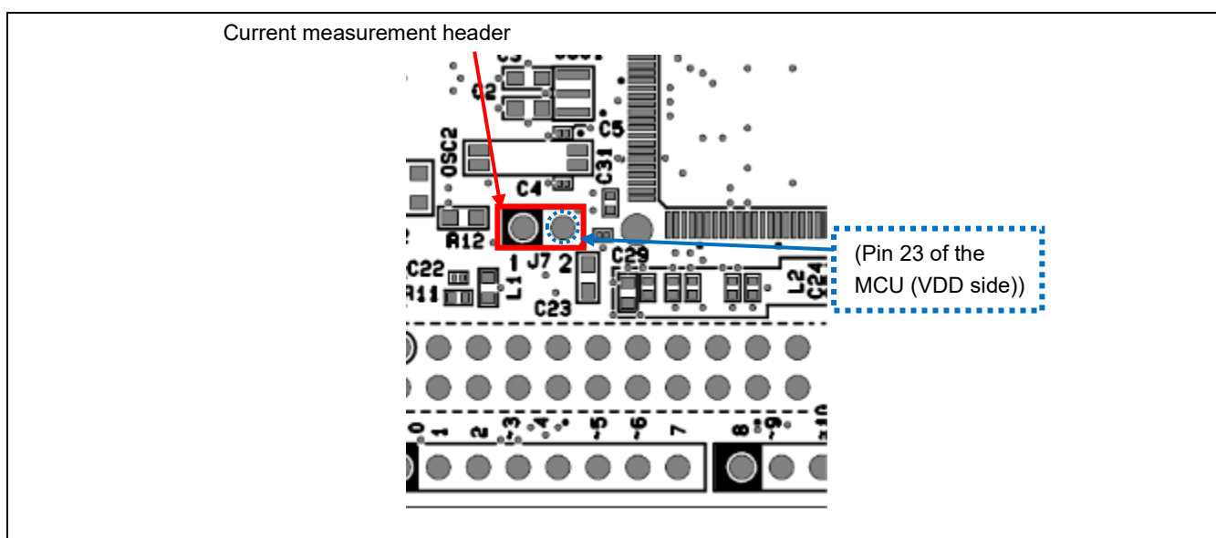
Figure 5-21 Position of the Current Measurement Header (Top Side)
