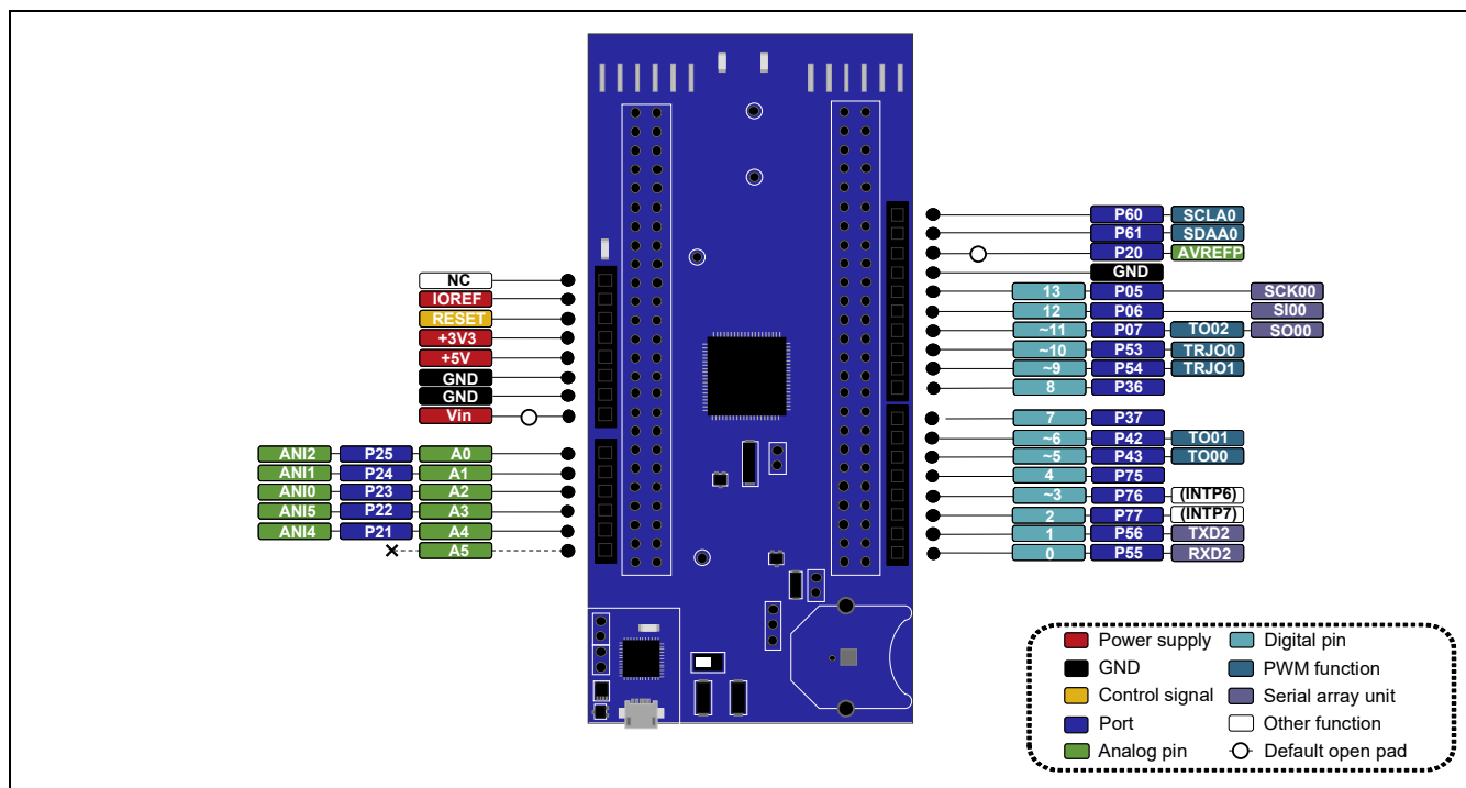
Figure 5-6 Pin Assignments of the Arduino™ Connectors
