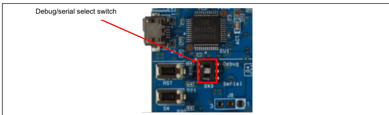
Figure 5-14 Position of the Debug/Serial Select Switch (Top Side)
