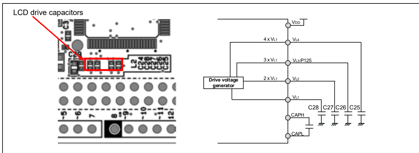
Figure 5-28 Positions of Capacitors (C25 to C28) (Top Side) and Circuit Schematic
