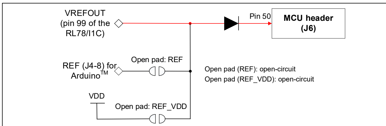
Figure 5-25 Circuit Schematic when VREFOUT for the RL78/I1C is Selected (Setting as Shipped)
