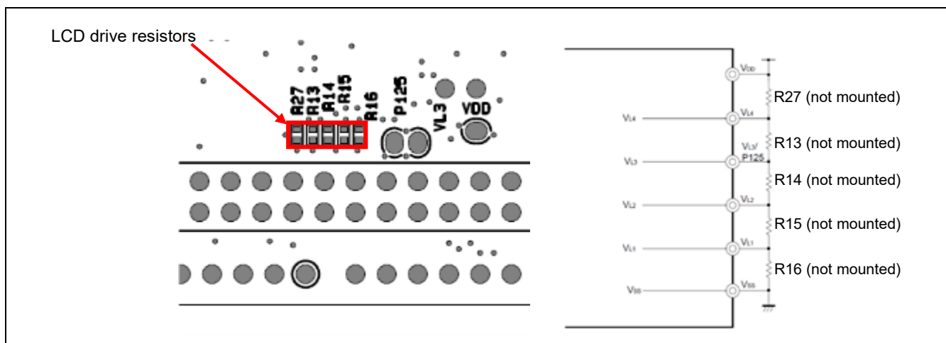
Figure 5-29 Positions of Resistors (R13 to R16 and R27) (Soldered Side) and Circuit Schematic
