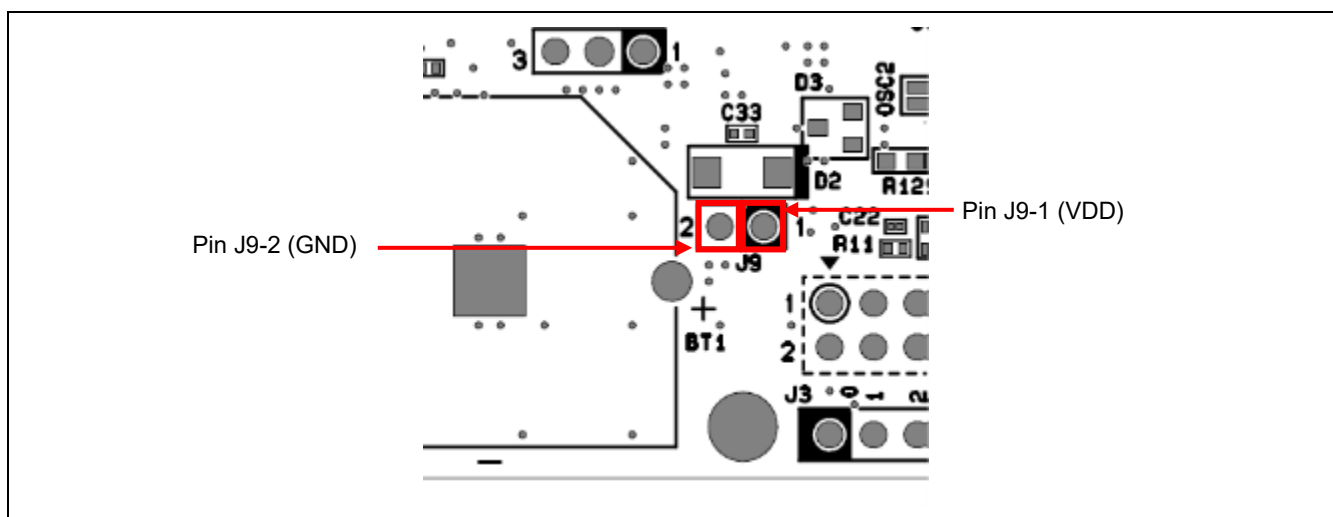
Figure 5-19 Positions of the External Power-Supply Header (Top Side)
