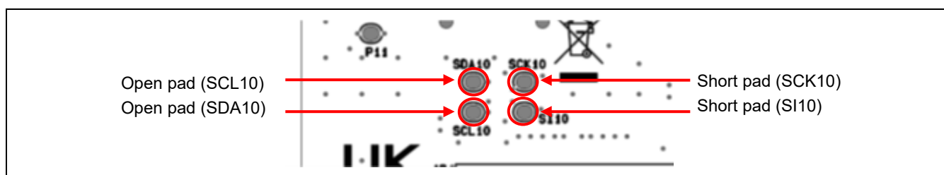
Figure 5-4 Positions of Open and Short Pads (Pmod™ 2) (Soldered Side)
