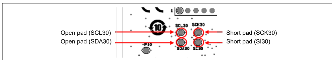
Figure 5-2 Positions of Open and Short Pads (Pmod™ 1) (Soldered Side)
