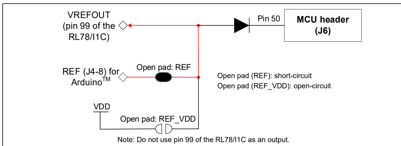
Figure 5-26 Circuit Schematic when REF for Arduino™ is Selected
