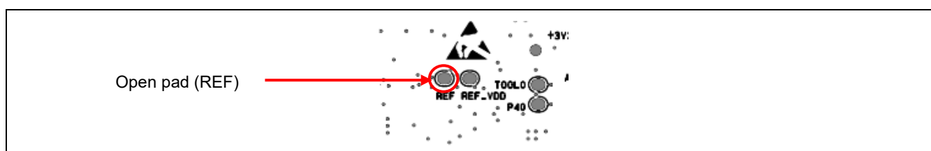
Figure 5-7 Position of the Open Pad (REF) (Soldered Side)
