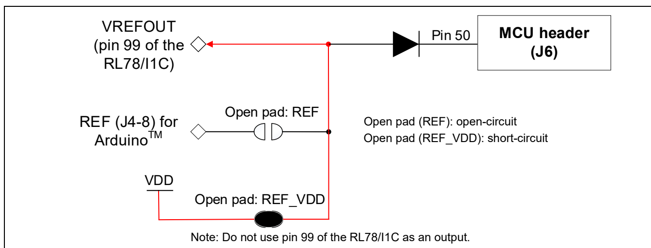
Figure 5-27 Circuit Schematic when VDD is Selected
