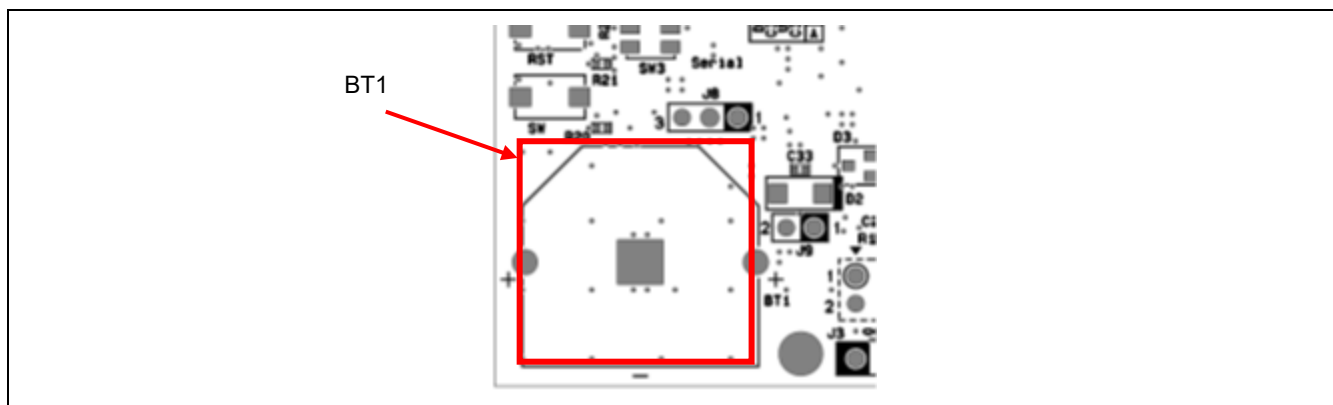
Figure 5-20 Position of BT1 (Top Side)
