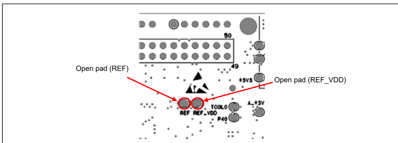
Figure 5-24 Positions of the Open Pads (REF_VDD and REF) (Soldered Side)
