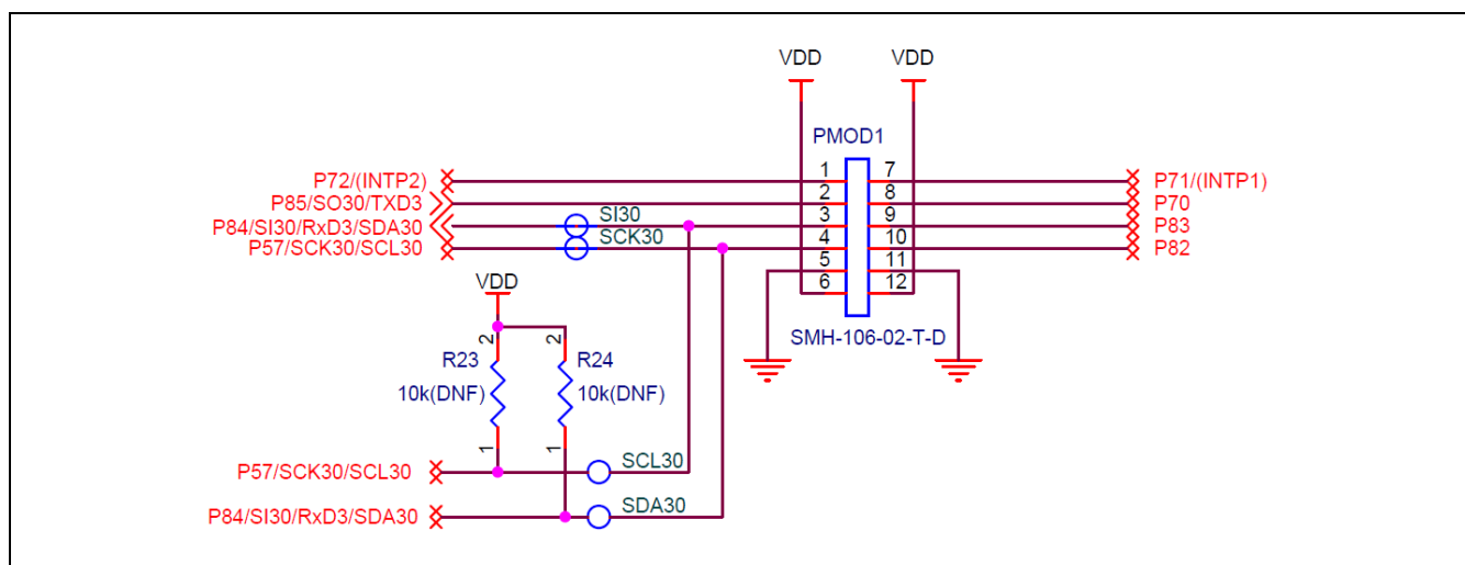
Figure 5-3 Circuit Schematic of Pmod™ 1
