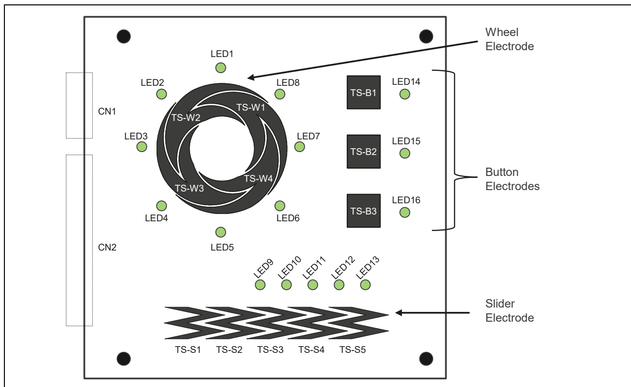
Figure 2. Application Board
