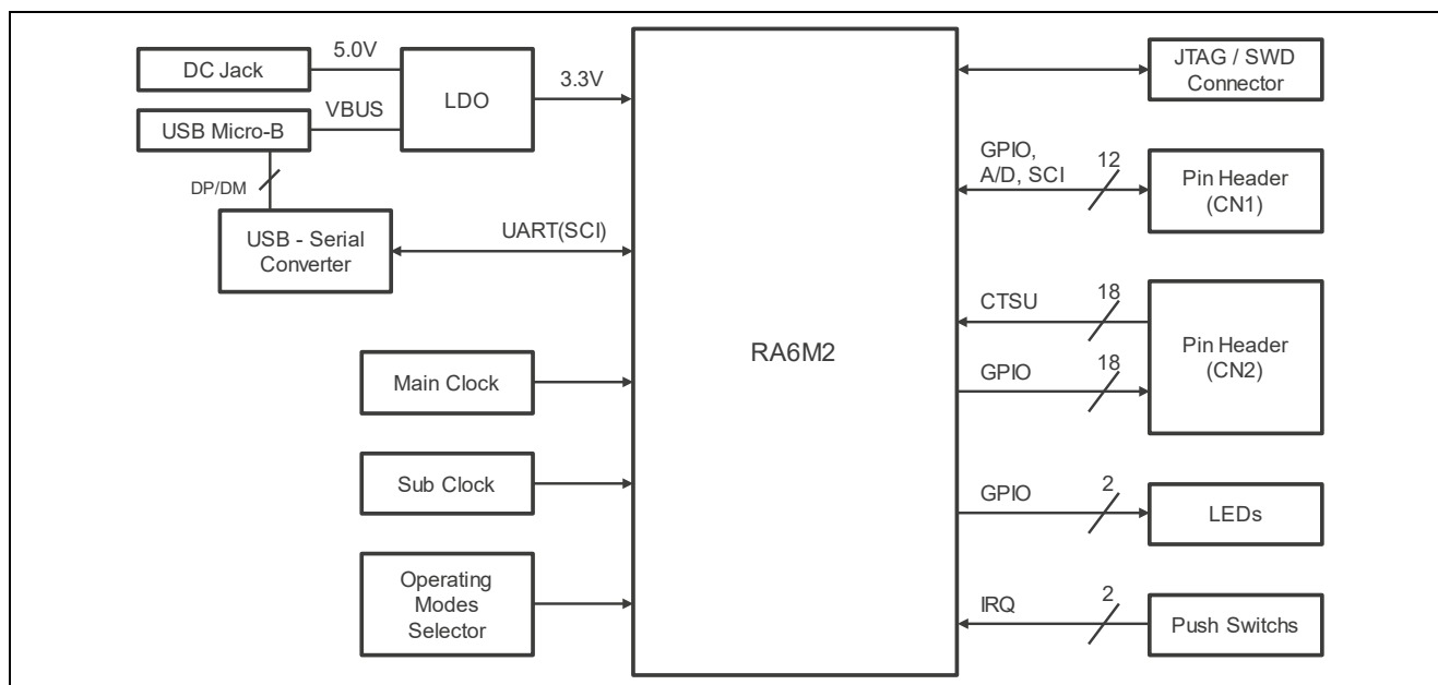
Figure 3. RA6M2 Cap Touch CPU Board Block Diagram
