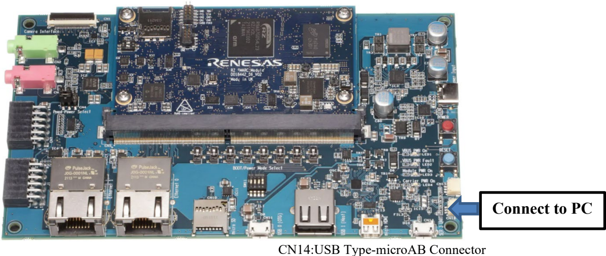
Figure 3. Connecting console for debug
