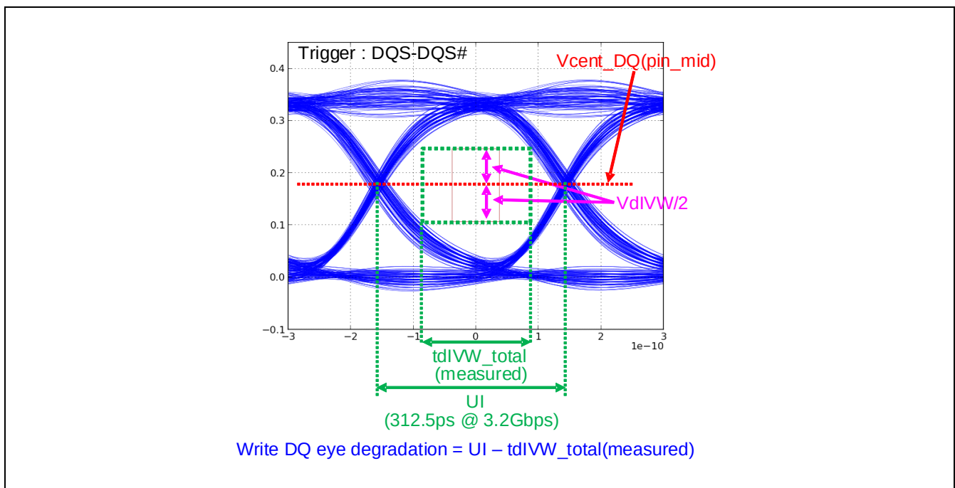
Figure 4.17 Measurement example of DQ Eye pattern
