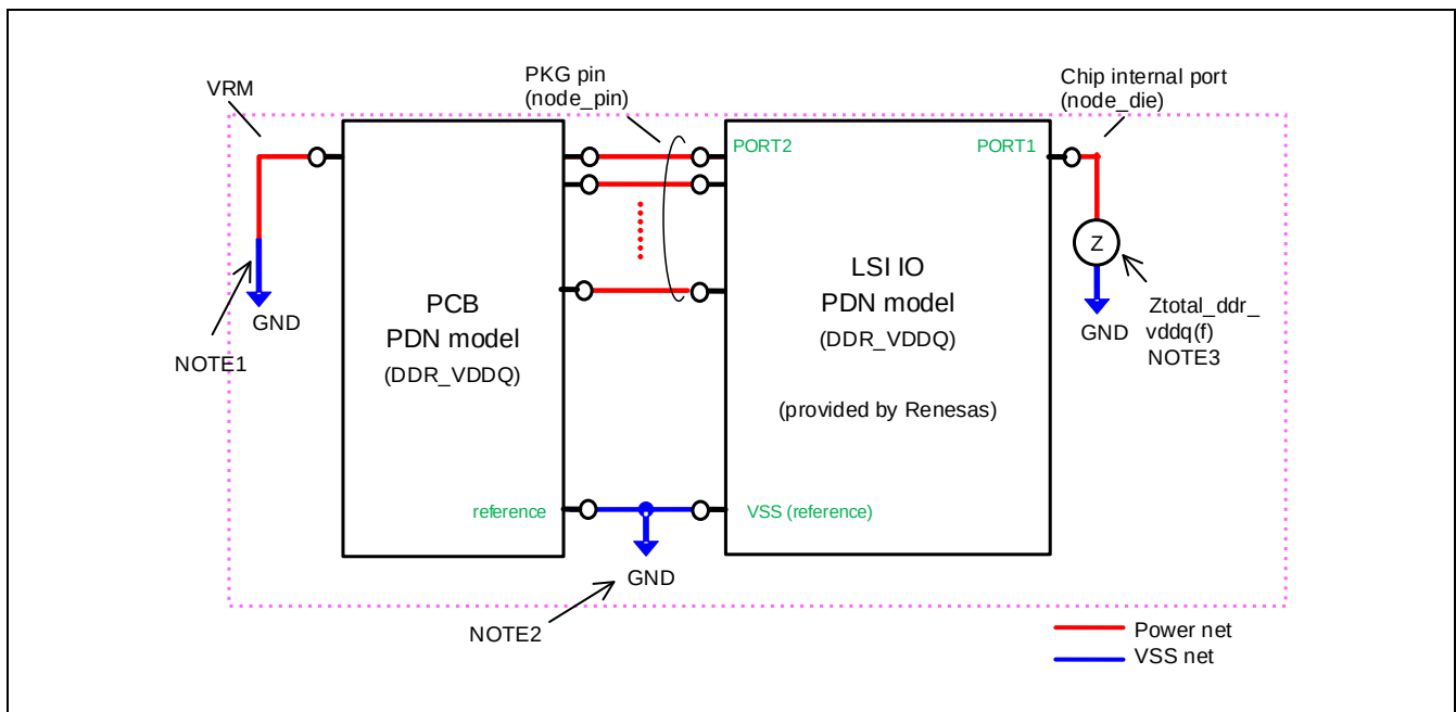
Figure 5.1 Connection for Z_{\text{total\_DDR\_vddq}}(f) calculation
