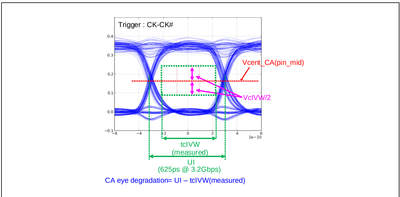
Figure 4.18 Measurement example of CA Eye pattern
