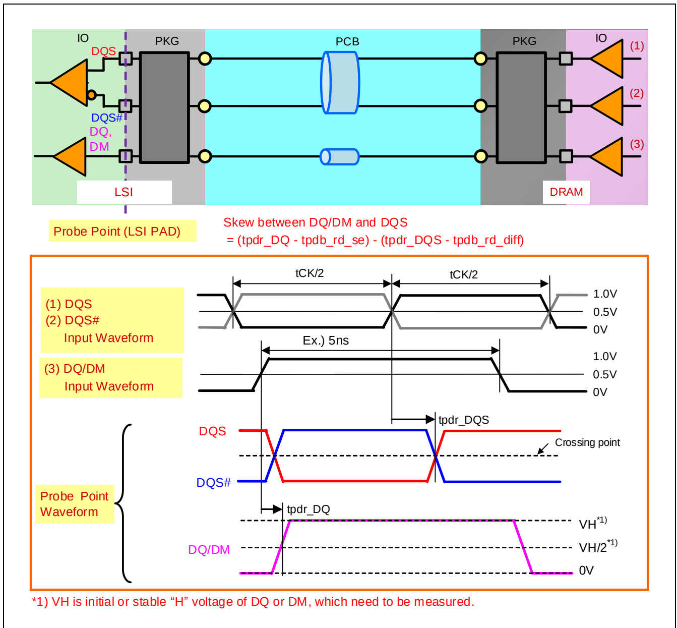
Figure 4.13 Measurement method of skew between DQ/DM and DQS (Read)
