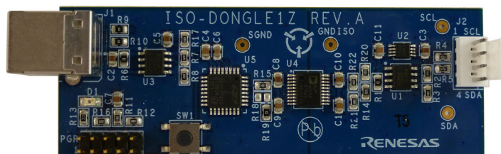
Figure 2. ISO-DONGLE1Z Board
