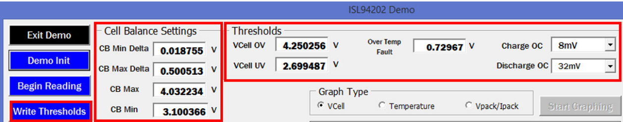
Figure 52. Demonstration Fault and Cell Balance Thresholds
