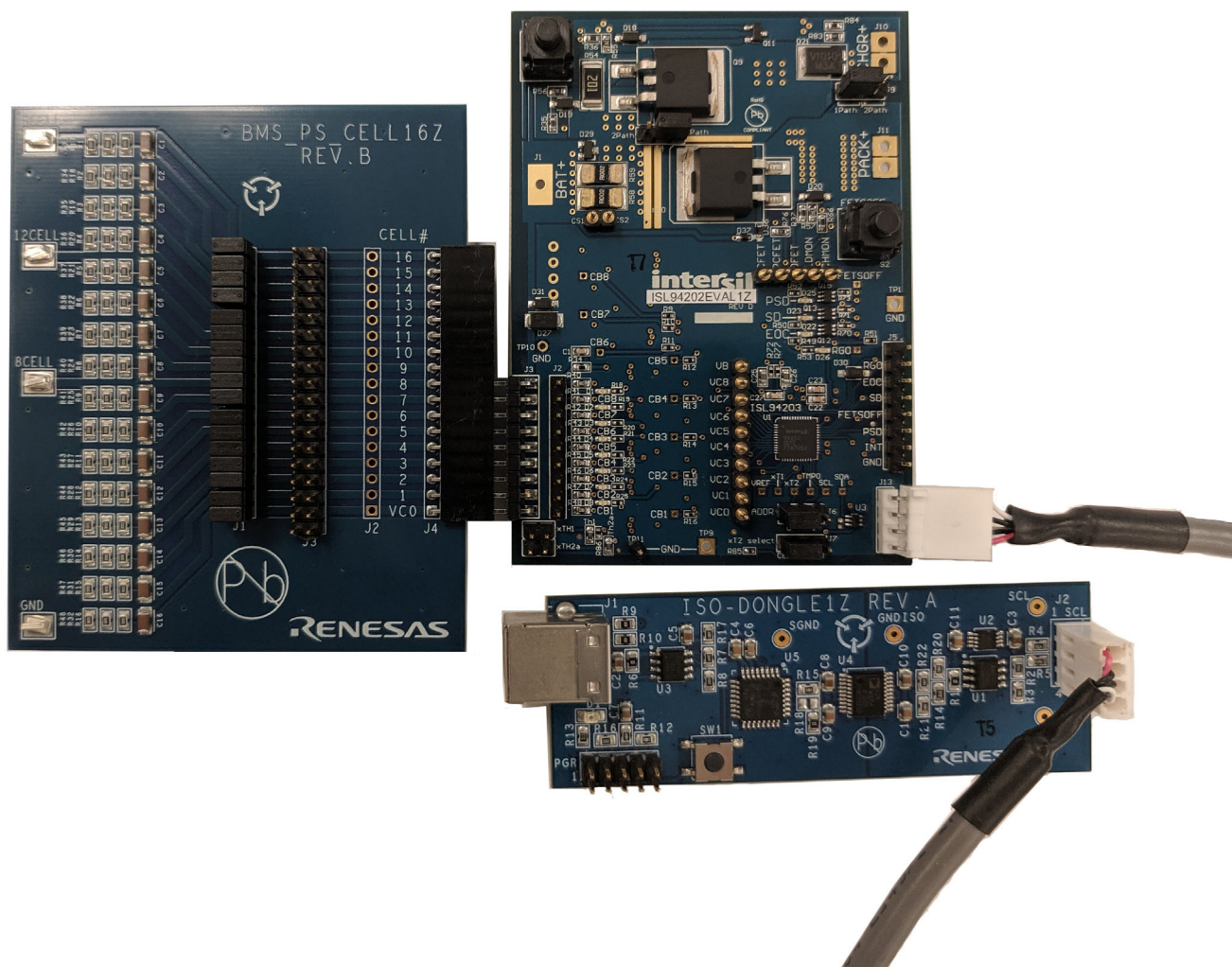
Figure 4. Board Connection
