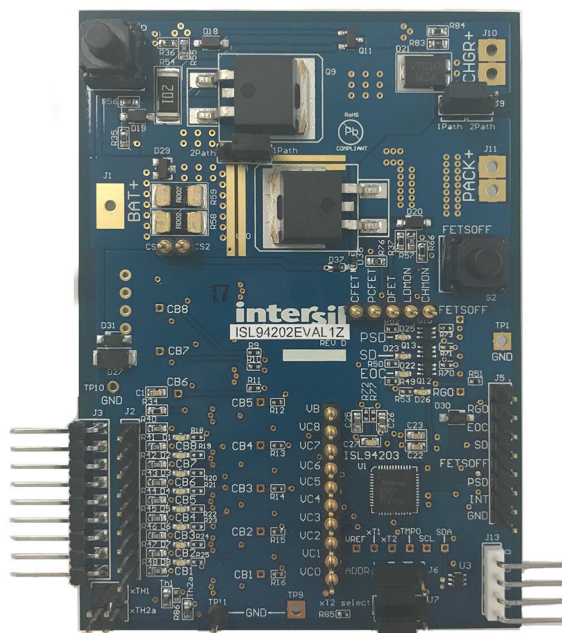
Figure 1. ISL94202EVAL1Z Board
