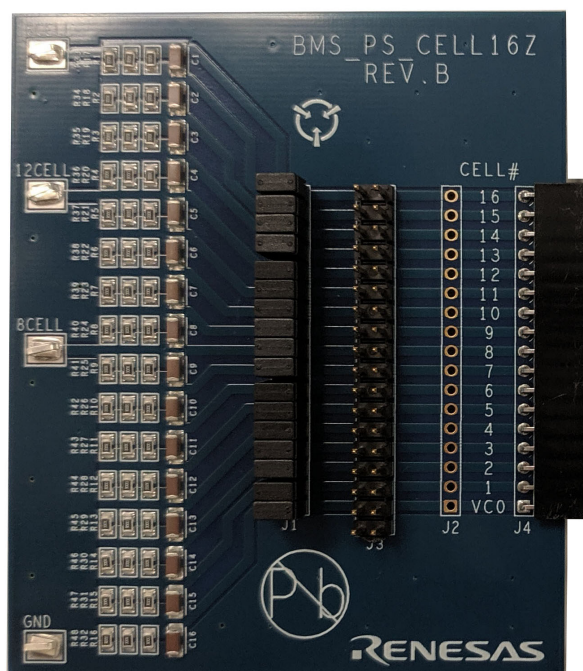
Figure 3. Resistor Ladder
