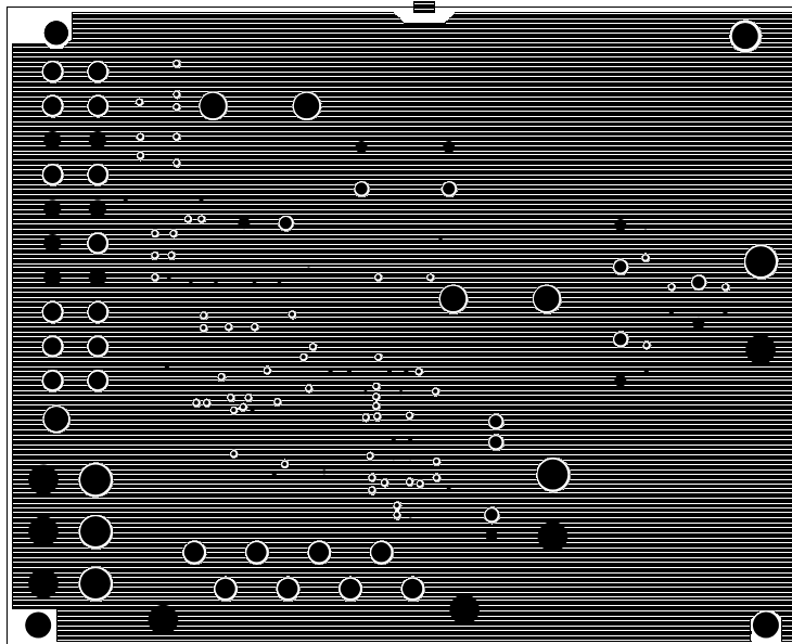
FIGURE 13. INTERNAL 1 GROUND
