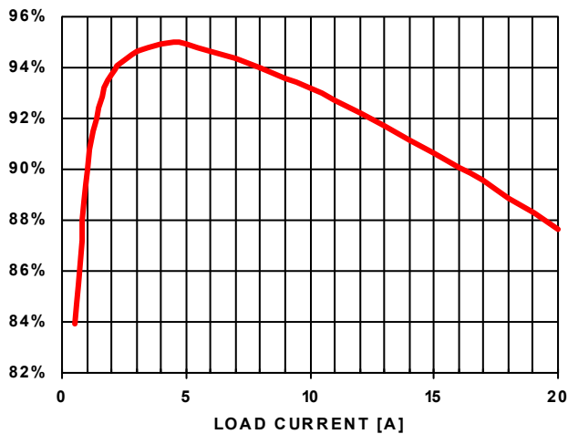
FIGURE 10. V DDQ EFFICIENCY
