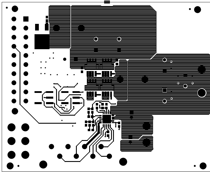
FIGURE 12. TOP
