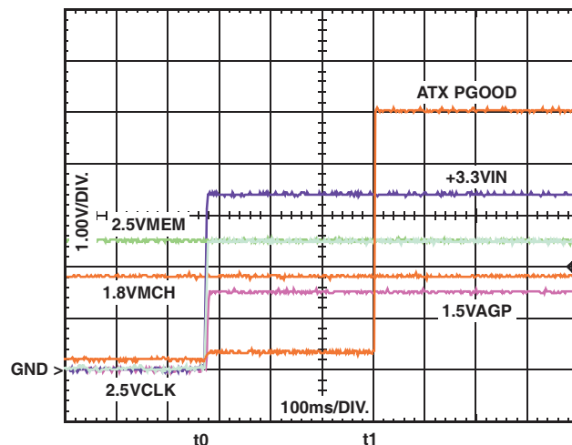
FIGURE 4. S3 STANDBY TO ACTIVE STATE TRANSITION
