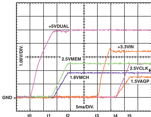
FIGURE 2. ISL6432EVAL1 START-UP
