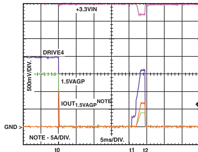
FIGURE 7. ISL6432EVAL1 VOUT4 HICUP MODE UNDER APPLIED SHORT CIRCUIT
