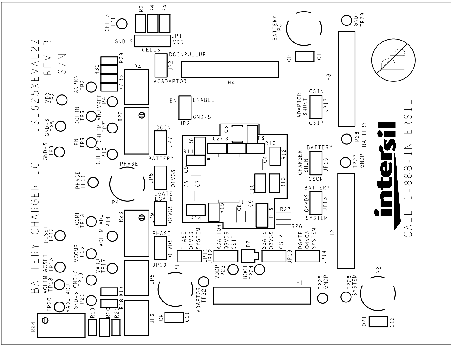
FIGURE 1. TOP SILK
