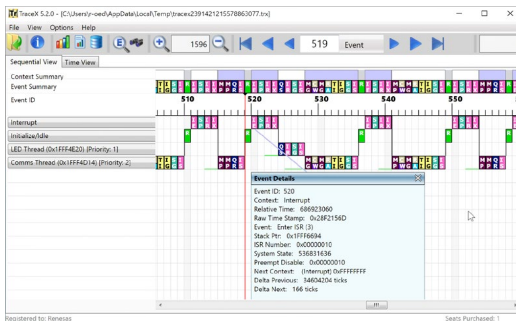
Figure 11-5: The sequence of events as visualized by TraceX®
