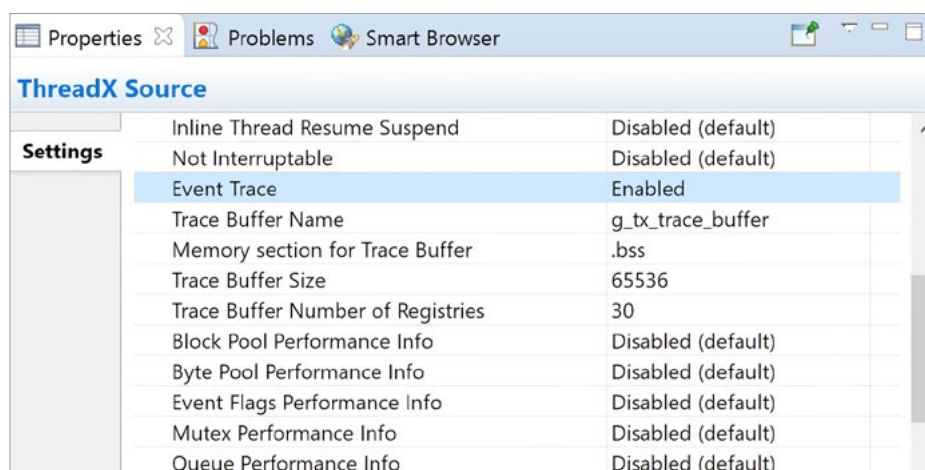
Figure 11-3: The event trace needs to be enabled in the properties of the ThreadX®
