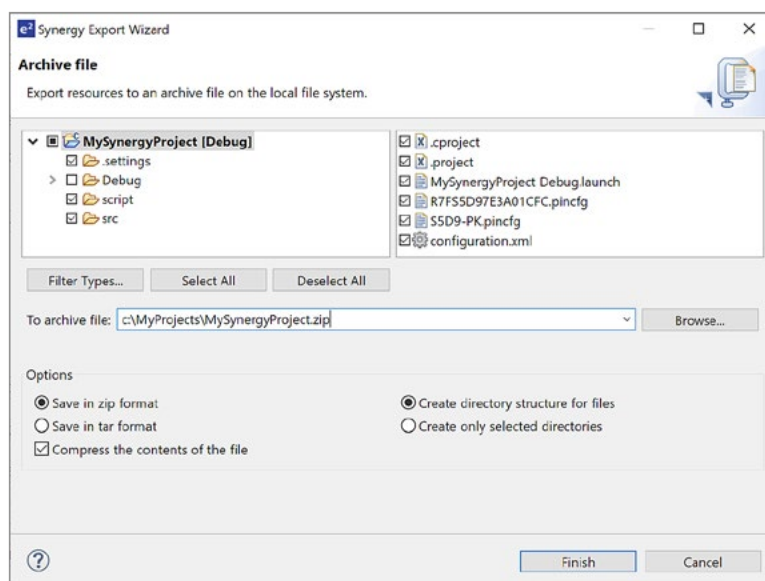
Figure 5-5: The Export Wizard in e 2 studio
