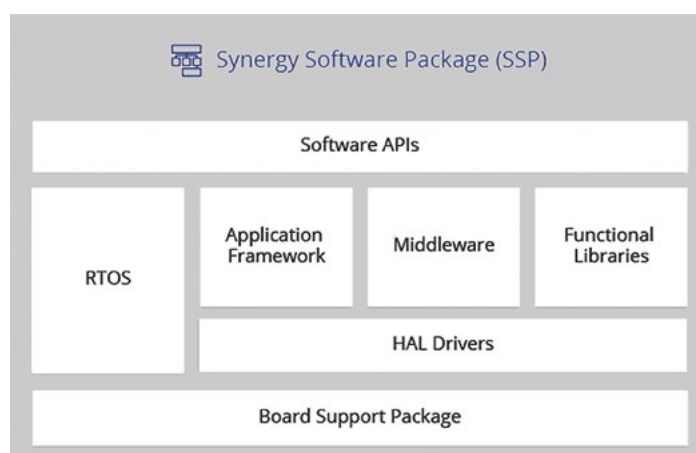
Figure 2-2: Everything in the Synergy software ecosystem is built in layers
