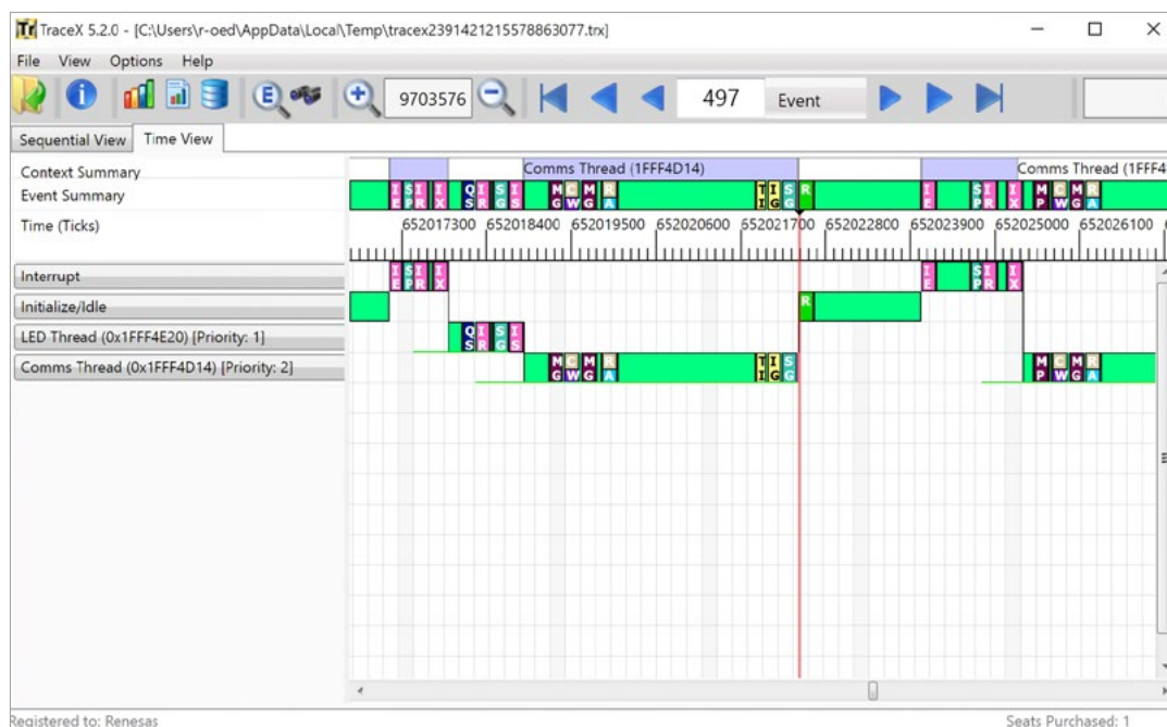
Figure 11-6: When in Time View, TraceX® displays the exact timings between the different events
