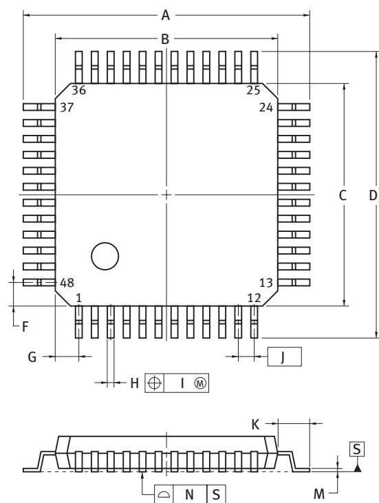
48-PIN PLASTIC LQFP (FINE PITCH) (7x7)
