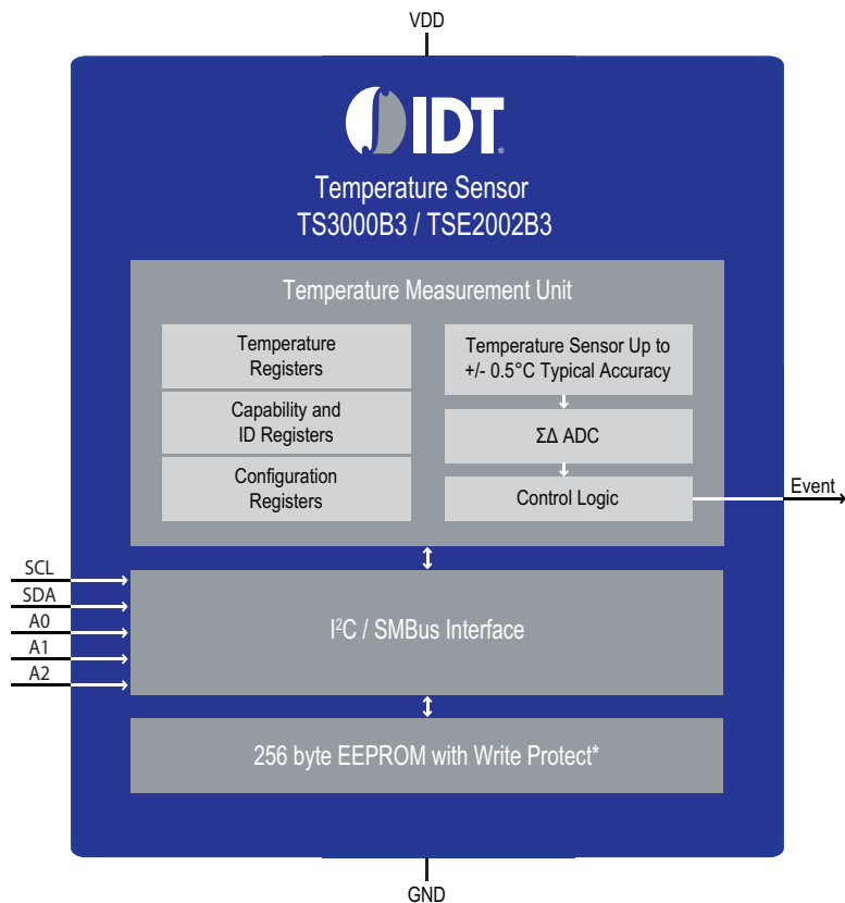
Figure 1. TS3000B3 / TSE2002B3 Functional block diagram
