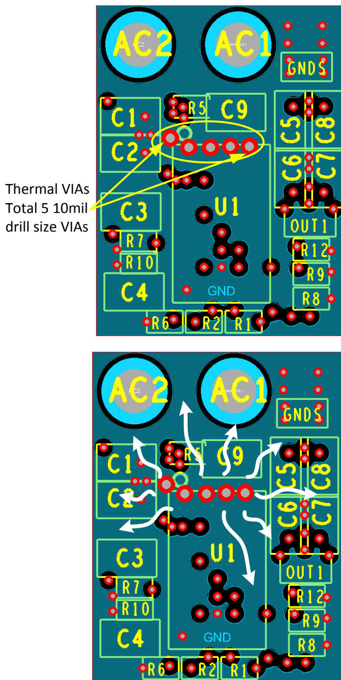
Figure 10. P9027LP-R QFN Bottom Layer layout.
