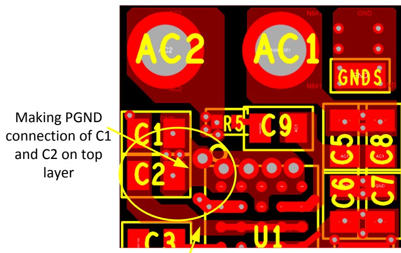
Figure 7. Recommended layout for rectifier capacitors.
