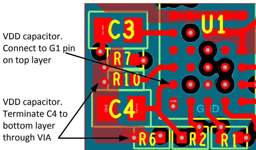
(b) VDD capacitor layout
