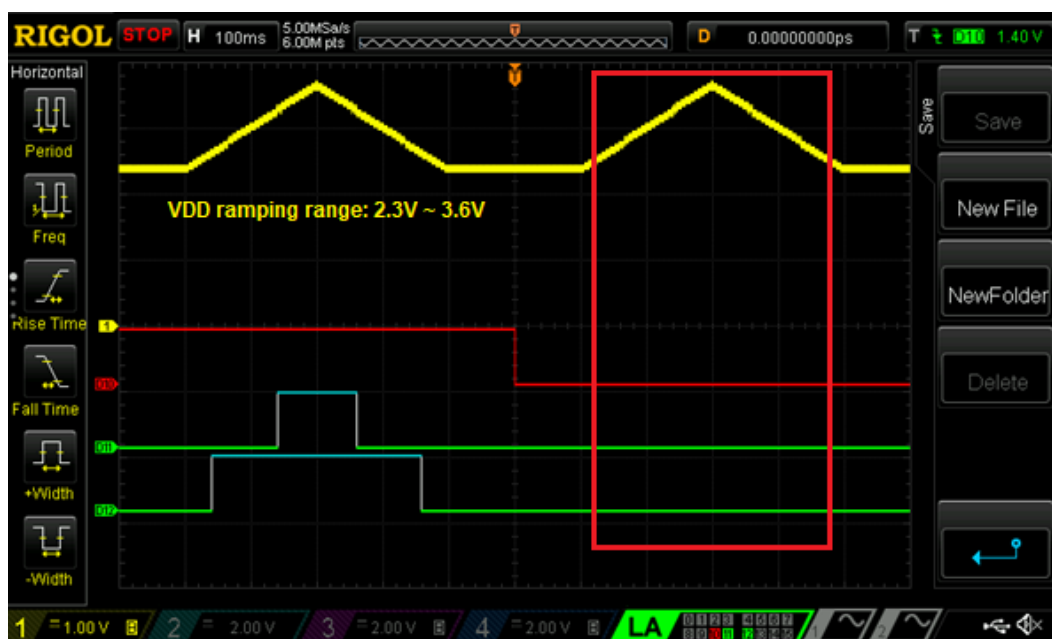
Figure 2 ACMPs Output Behavior
