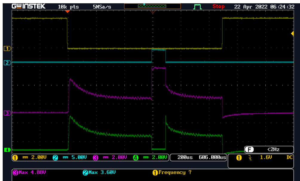
Figure 7 Glitch at HV_GPOx, decay = 0 (Fast decay)
