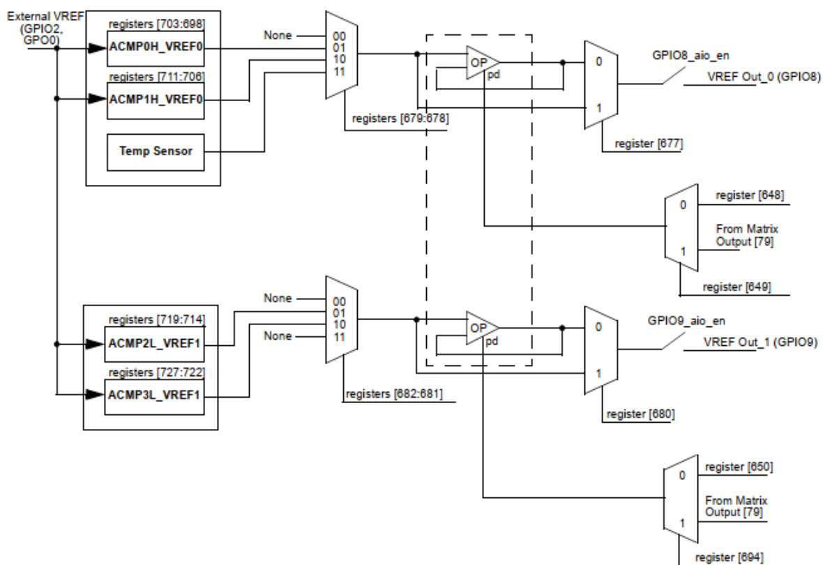
Figure 2: Voltage Reference Block Diagram
