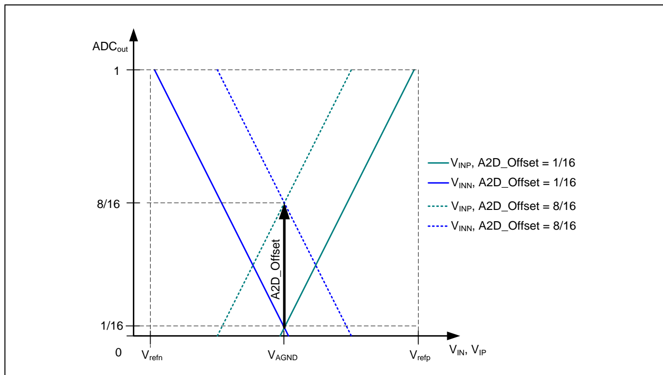
Figure 2.2 ADC Offset
