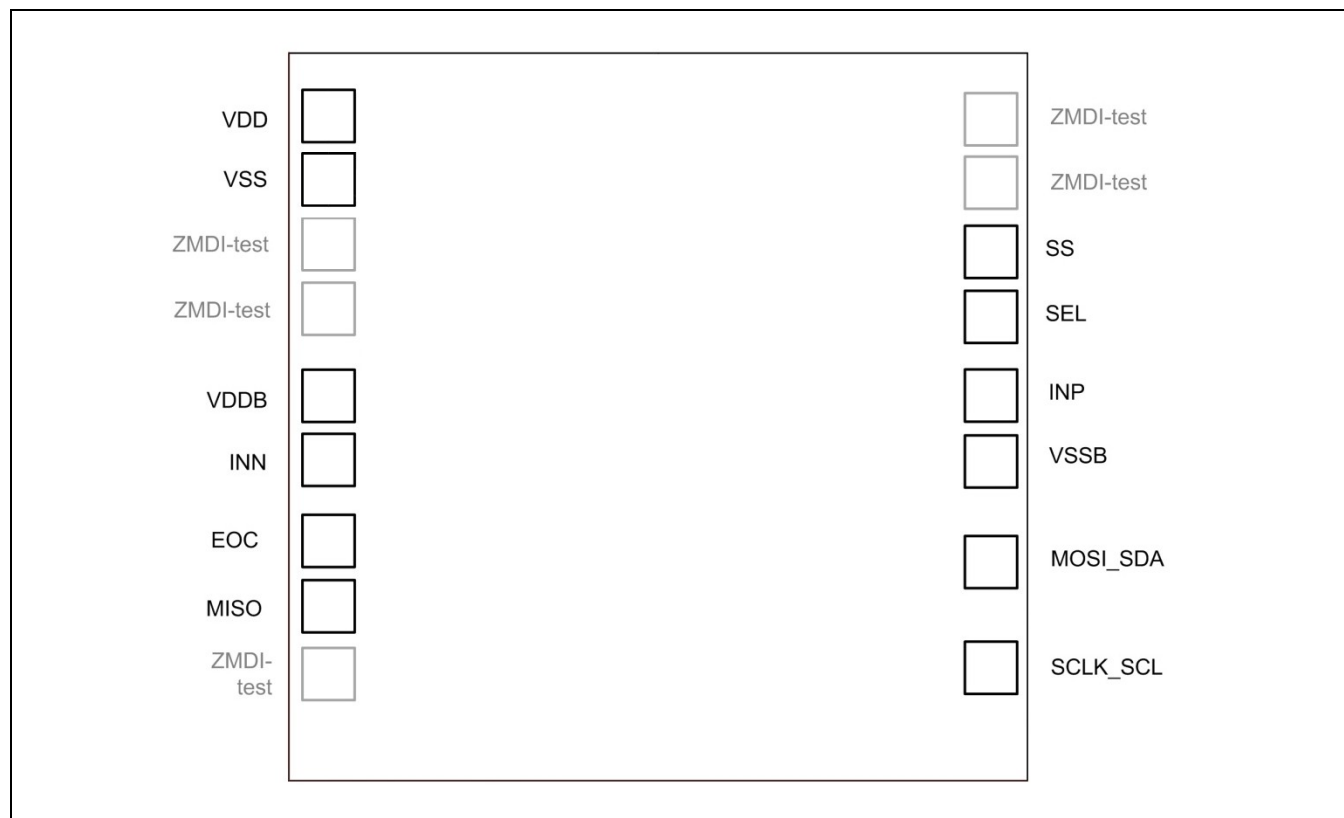
Figure 4.1 ZSSC3027 Pad Assignments
