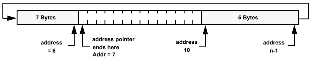
FIGURE 15. WRITING 12 BYTES TO A 16-BYTE PAGE STARTING AT LOCATION 10
