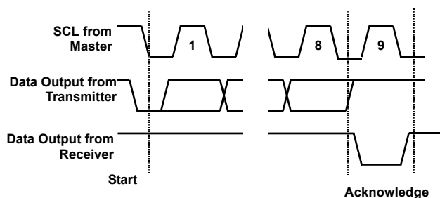
FIGURE 12. ACKNOWLEDGE RESPONSE FROM RECEIVER
