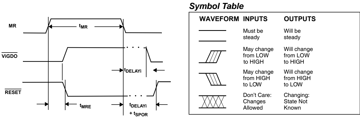
FIGURE 2. MANUAL RESET (MR)
