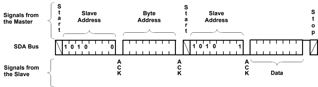
FIGURE 16. RANDOM ADDRESS READ SEQUENCE
