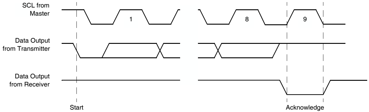
FIGURE 5. ACKNOWLEDGE RESPONSE FROM RECEIVER
