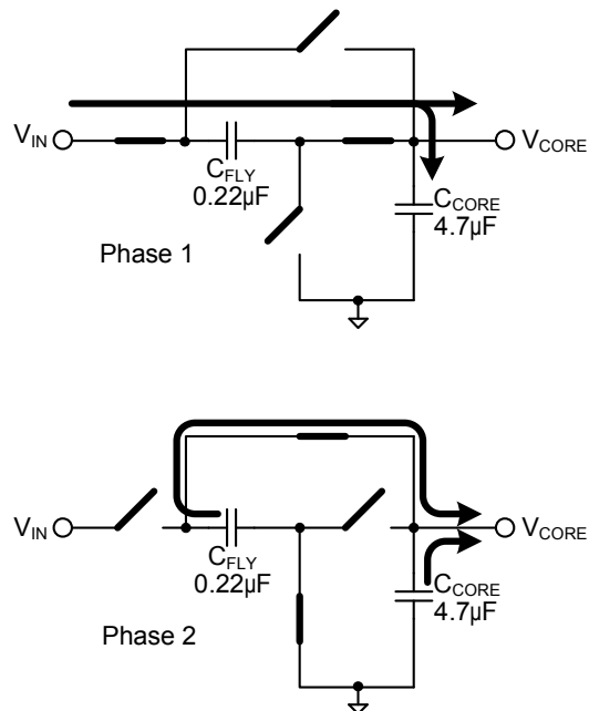
Figure 32. 0.5x Charge Pump 2 Phase Operation
