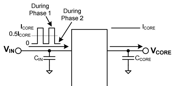
Figure 33. Input Current flowing Diagram
