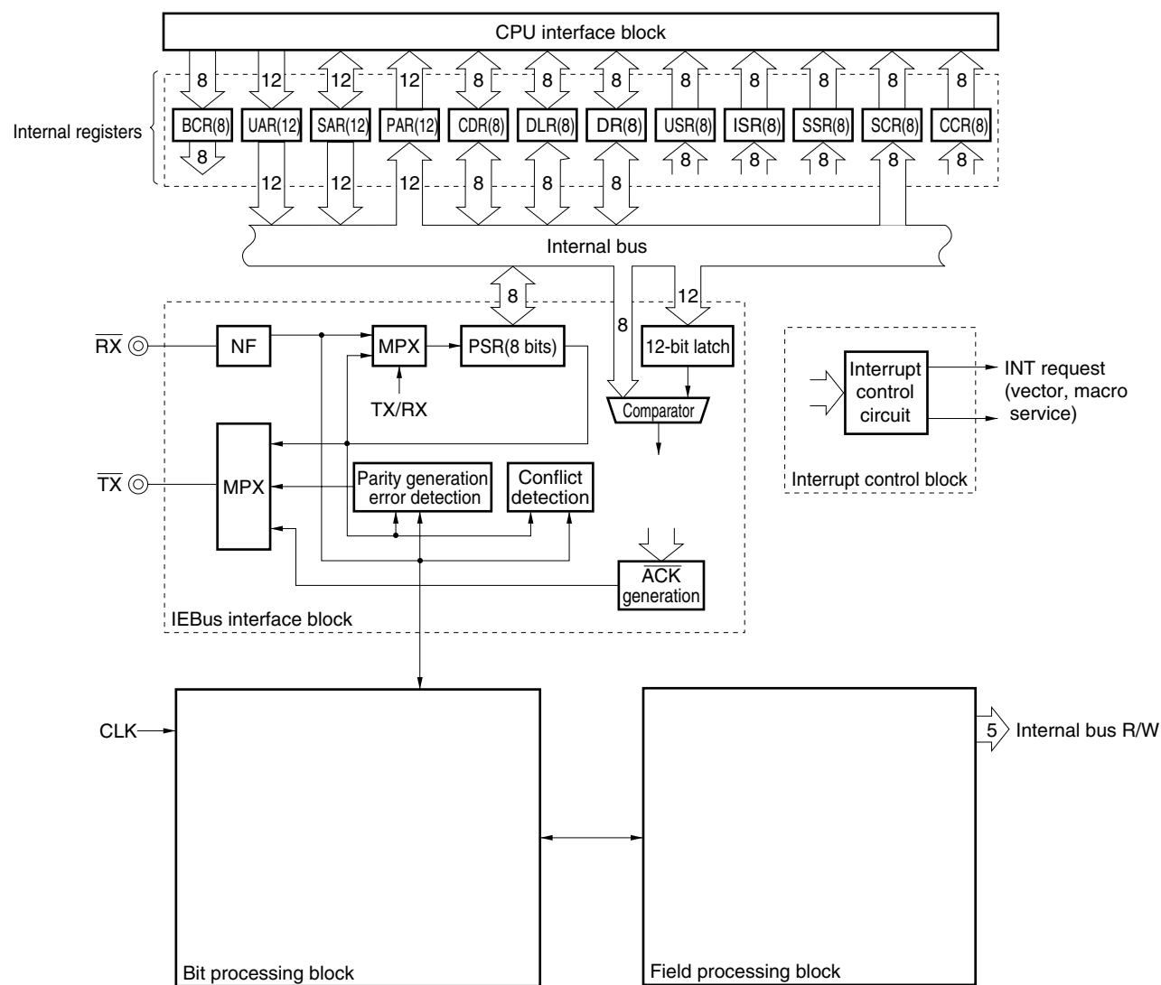
Figure 8-16. Block Diagram of IEBus Controller
