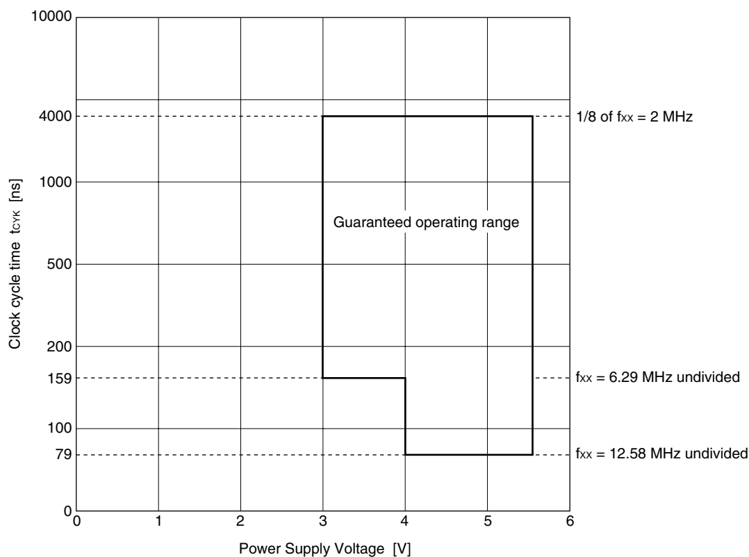
Figure 16-1. Power Supply Voltage and Clock Cycle Time
