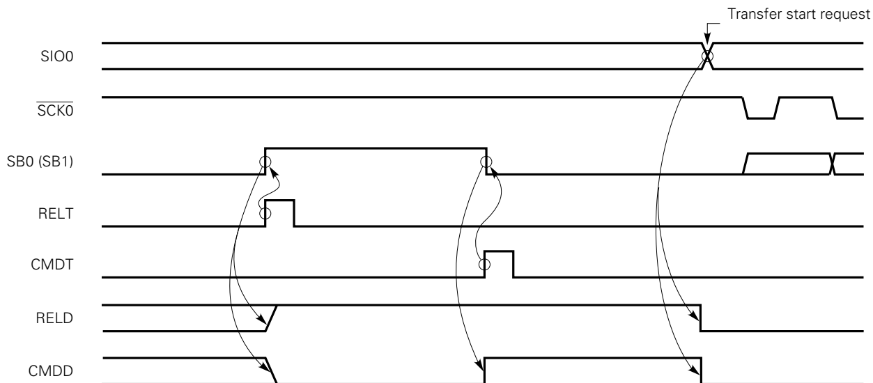
Fig. 4-38 Operations of RELT, CMDT, RELD, and CMDD (Master)
