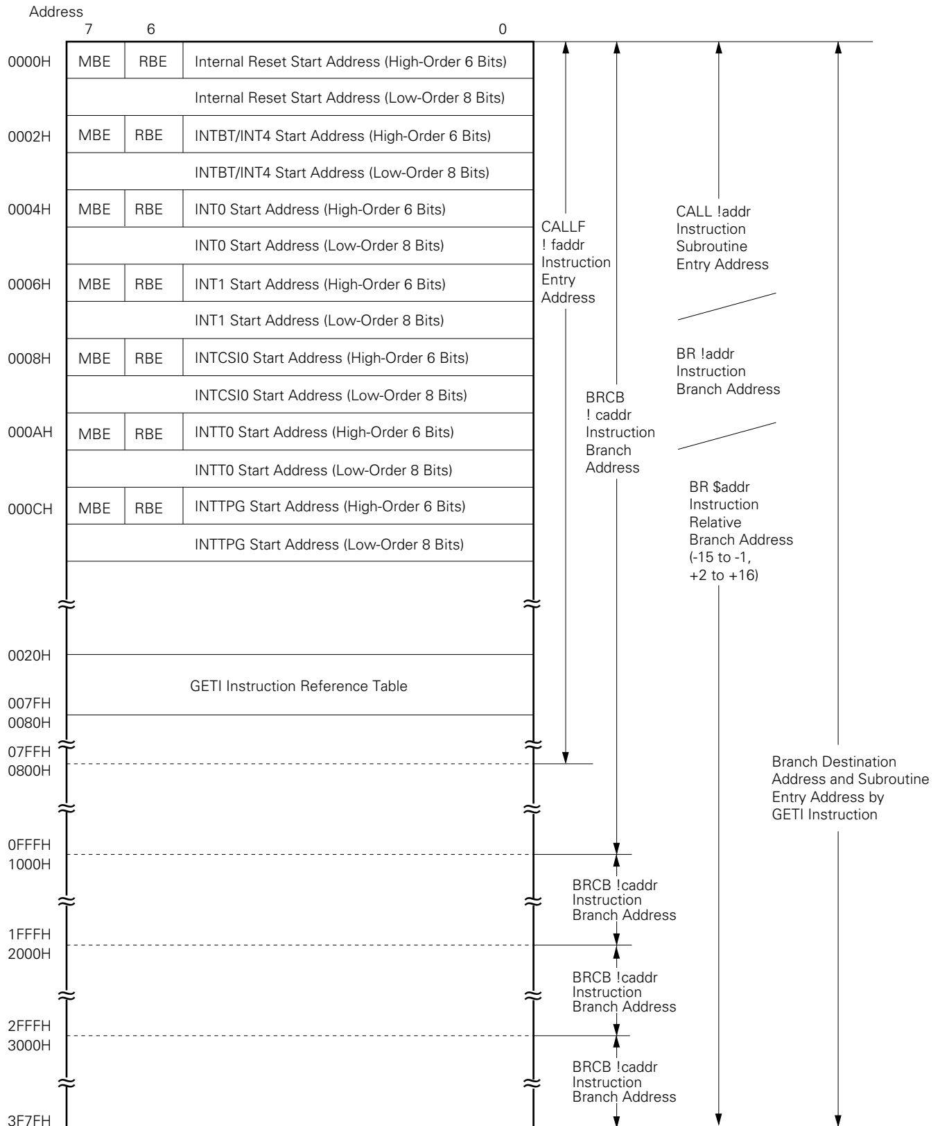
Fig. 5-1 Program Memory Map
