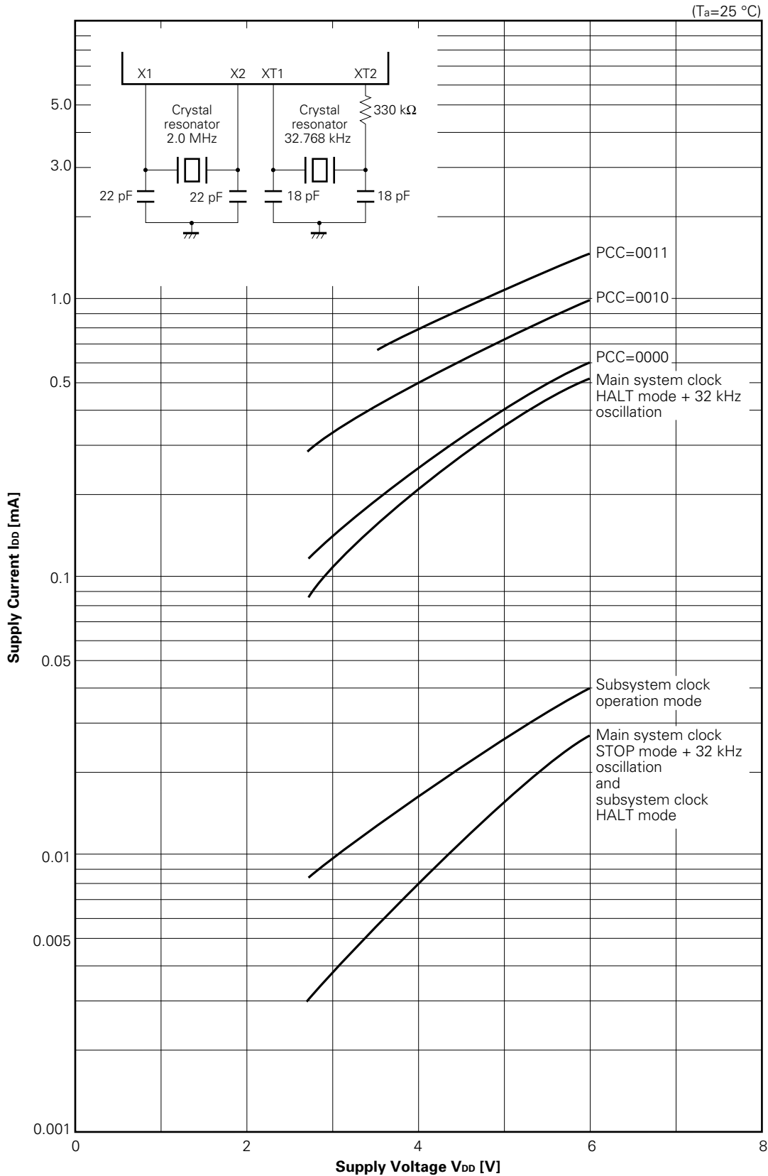
I DD vs V DD (Main system clock: 2.0-MHz crystal resonator)
