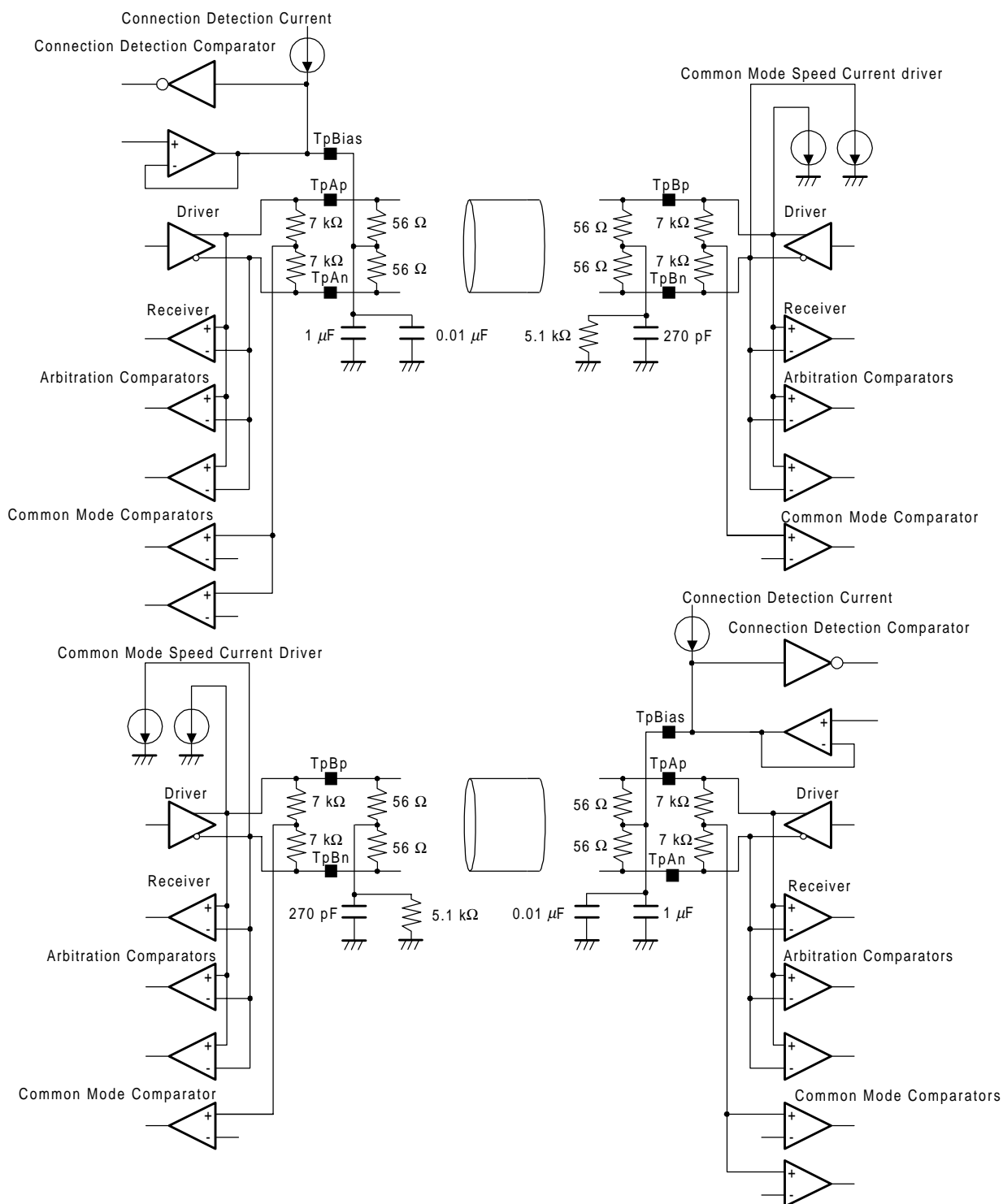
Figure 3-4. Cable Interface
