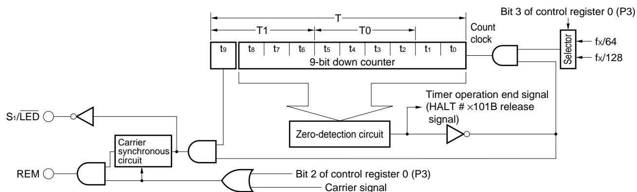
Figure 4-1. Timer Configuration
