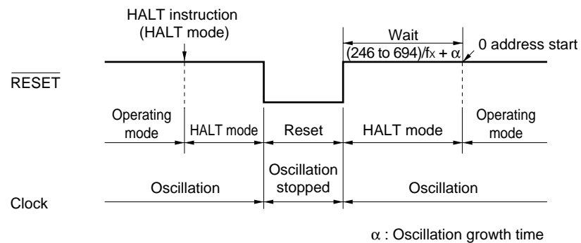
Figure 5-4. HALT Mode Release by RESET Input
