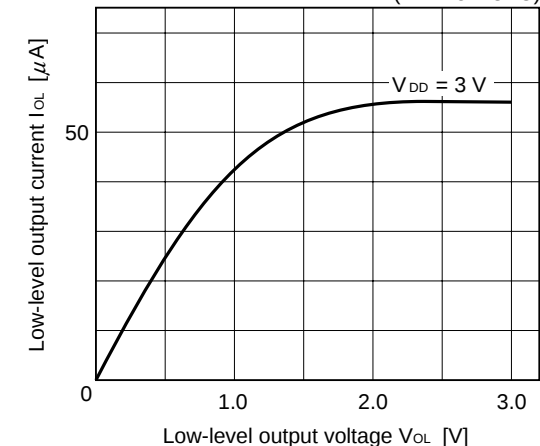
I_{OL} vs V_{OL} characteristic examples (K I/O0 -K I/O7 )
