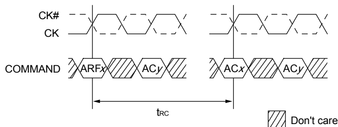
Figure 2-21. AUTO REFRESH Cycle
